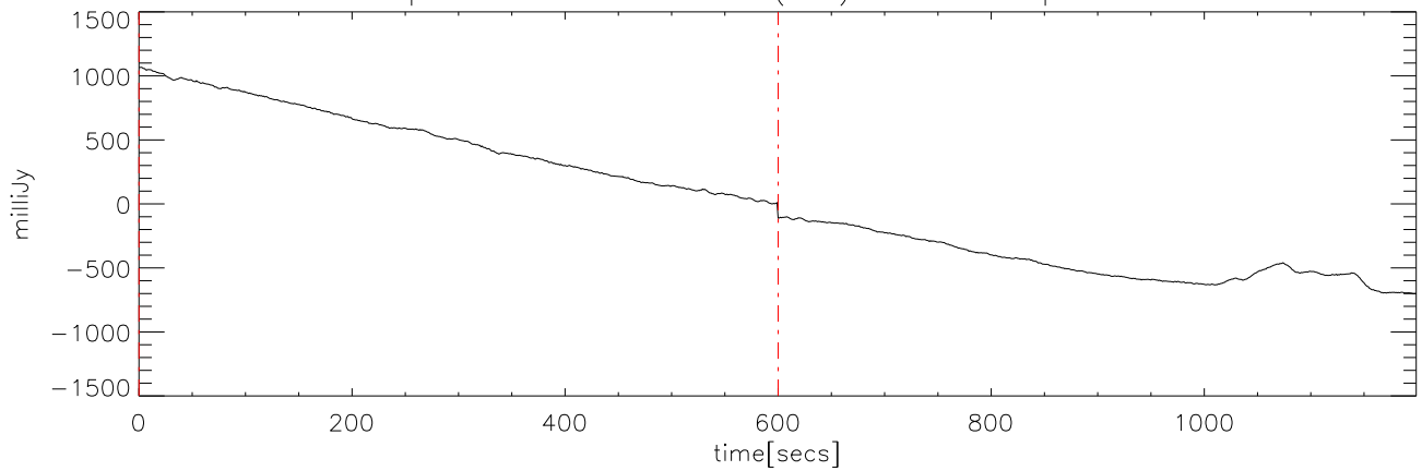
p2111 file:12 28dec08 (AST) StokesI freq:5125.
