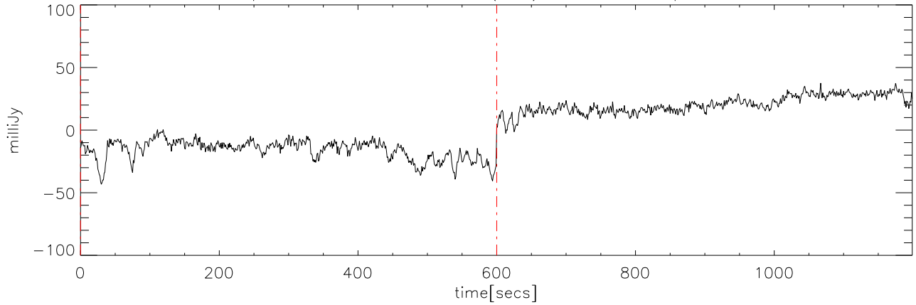
p2111 file:12 28dec08 (AST) StokesQ freq:5250.
