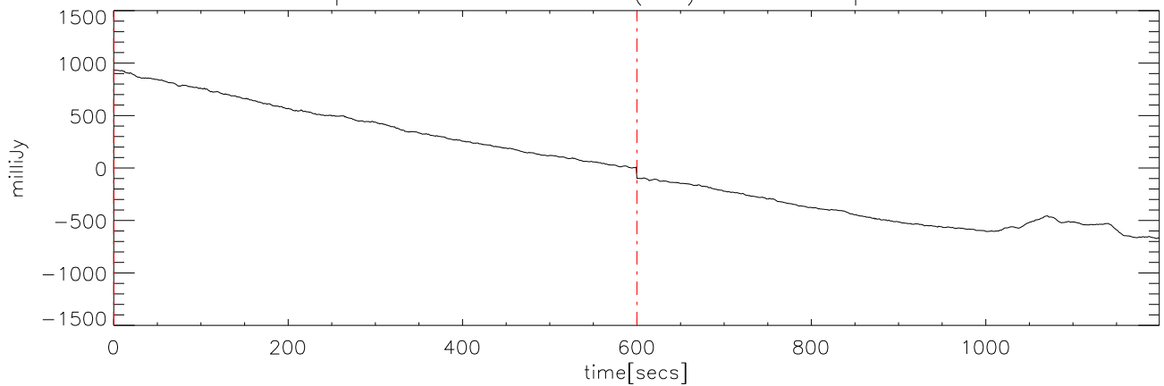
p2111 file:12 28dec08 (AST) StokesI freq:4725.
