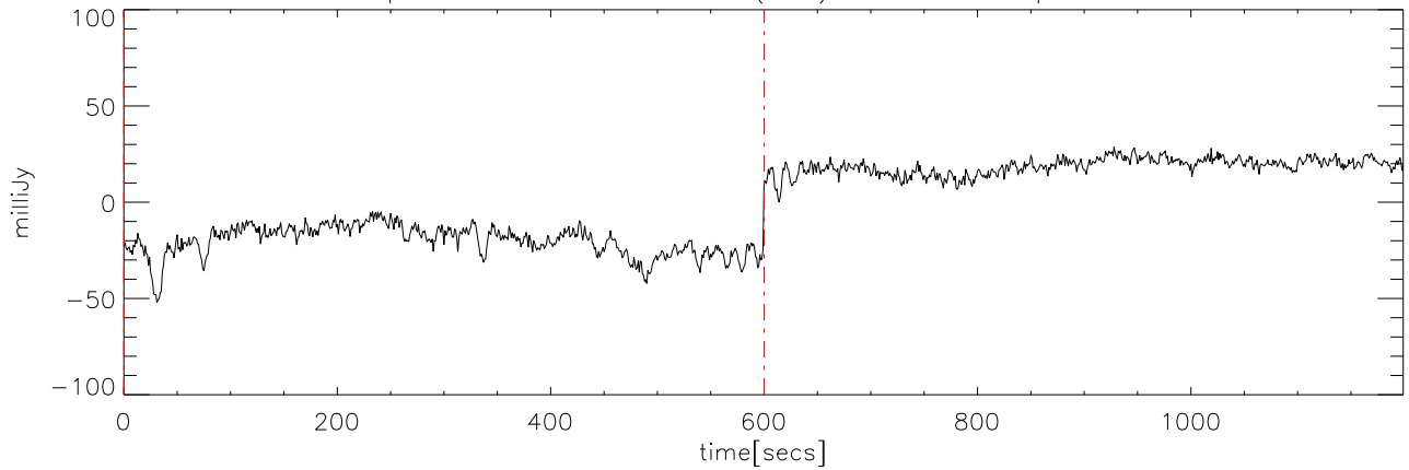
p2111 file:12 28dec08 (AST) StokesQ freq:5125.
