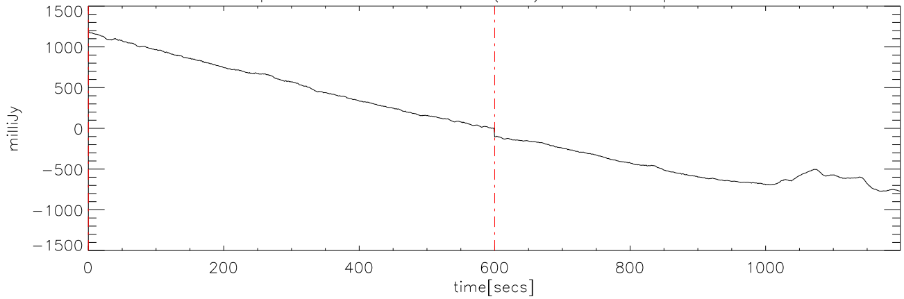
p2111 file:12 28dec08 (AST) StokesI freq:5250.
