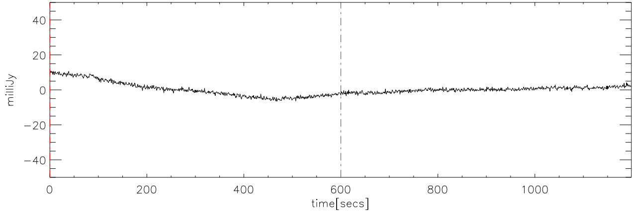
p2111 file:12 28dec08 (AST) StokesU freq:4475.
