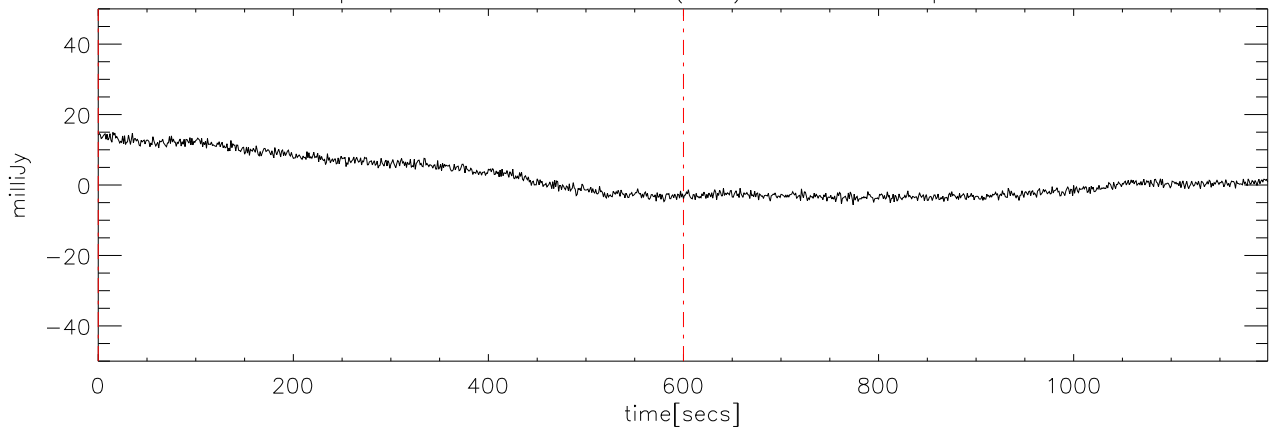
p2111 file:12 28dec08 (AST) StokesU freq:5125.
