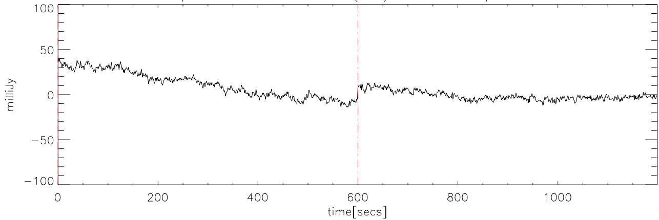
p2111 file:12 28dec08 (AST) StokesQ freq:4600.
