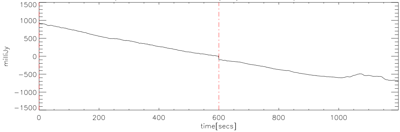
p2111 file:12 28dec08 (AST) StokesI freq:4475.
