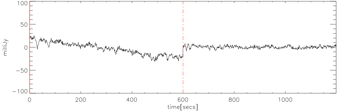
p2111 file:12 28dec08 (AST) StokesQ freq:4475.
