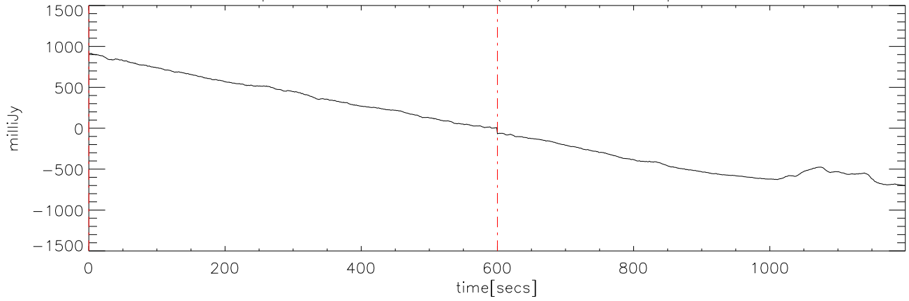
p2111 file:12 28dec08 (AST) StokesI freq:5000.
