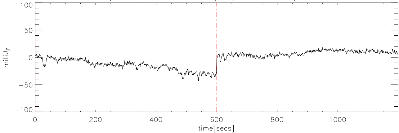
p2111 file:12 28dec08 (AST) StokesQ freq:4725.
