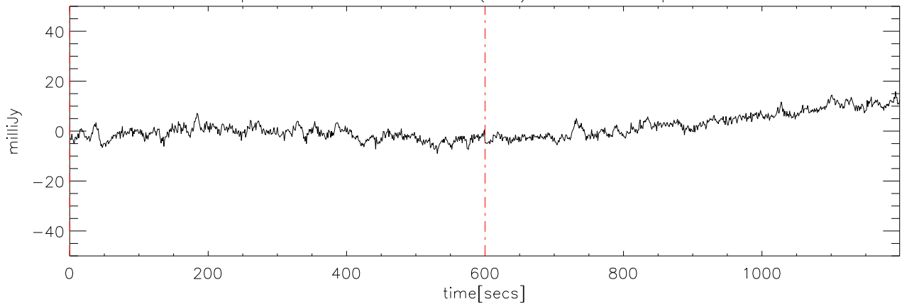
p2111 file:12 28dec08 (AST) StokesU freq:5250.
