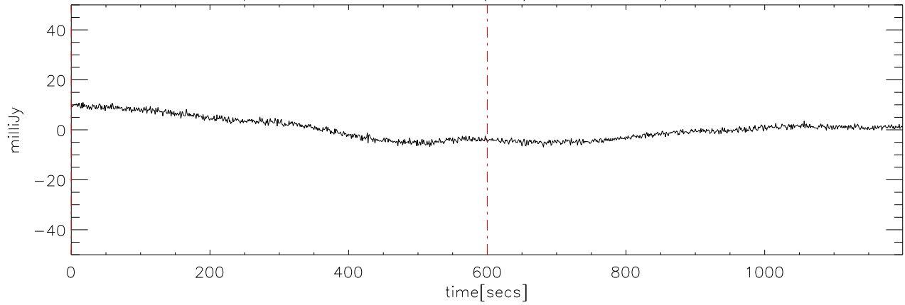
p2111 file:12 28dec08 (AST) StokesU freq:4725.
