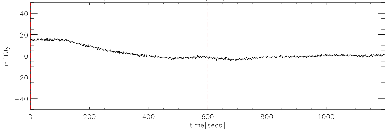
p2111 file:12 28dec08 (AST) StokesU freq:4600.
