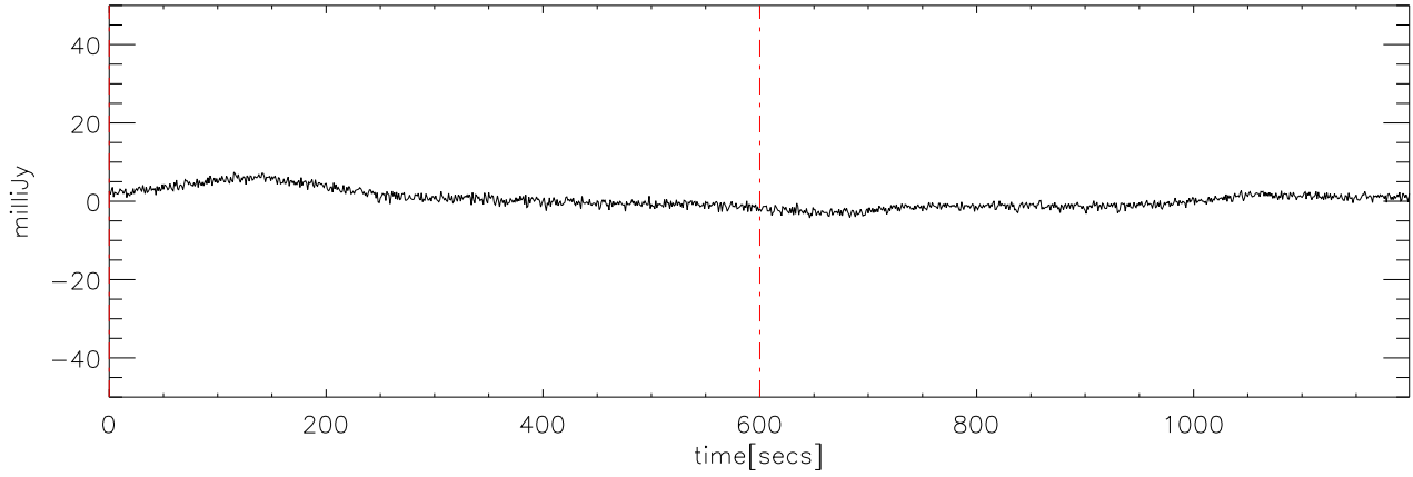
p2111 file:12 28dec08 (AST) StokesU freq:5000.
