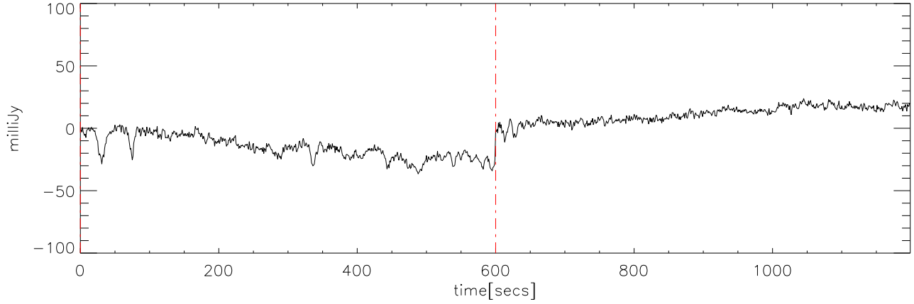
p2111 file:12 28dec08 (AST) StokesQ freq:5000.
