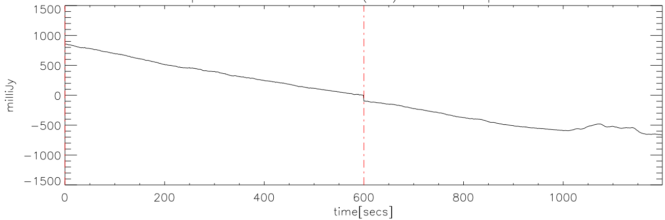
p2111 file:12 28dec08 (AST) StokesI freq:4600.
