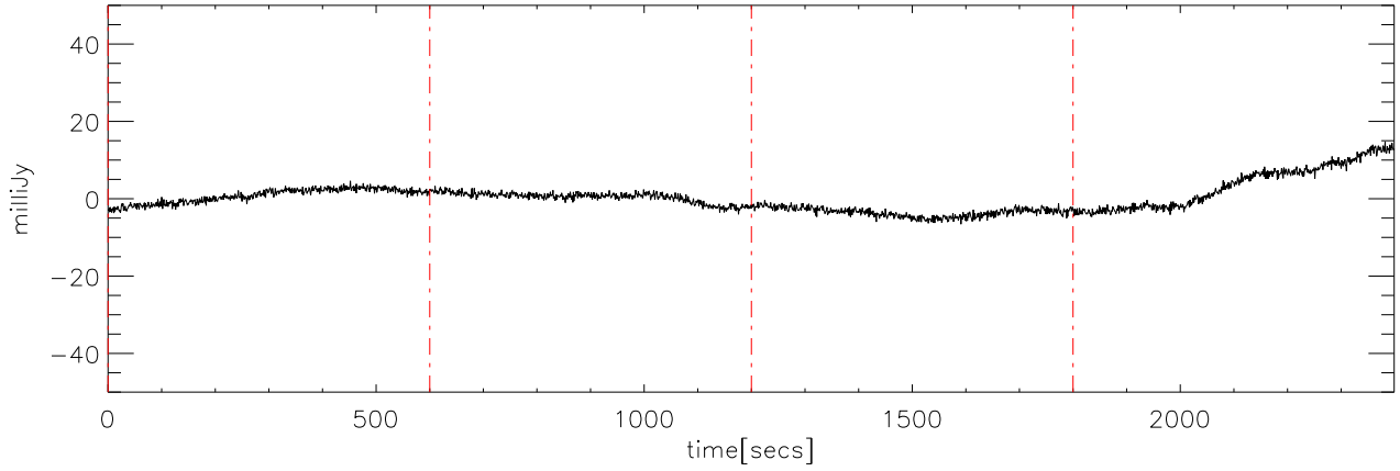
p2111 file:08 28dec08 (AST) StokesU freq:5000.
