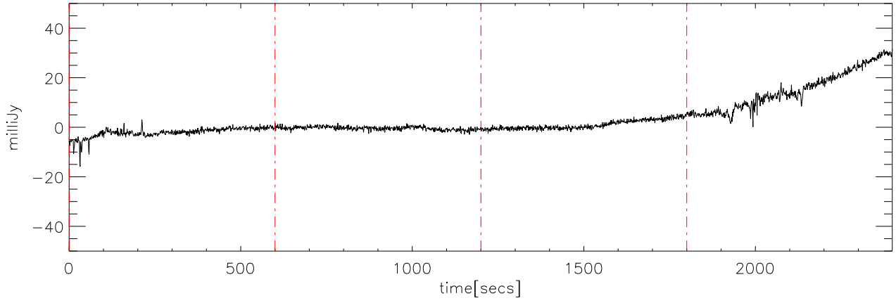
p2111 file:08 28dec08 (AST) StokesU freq:4475.
