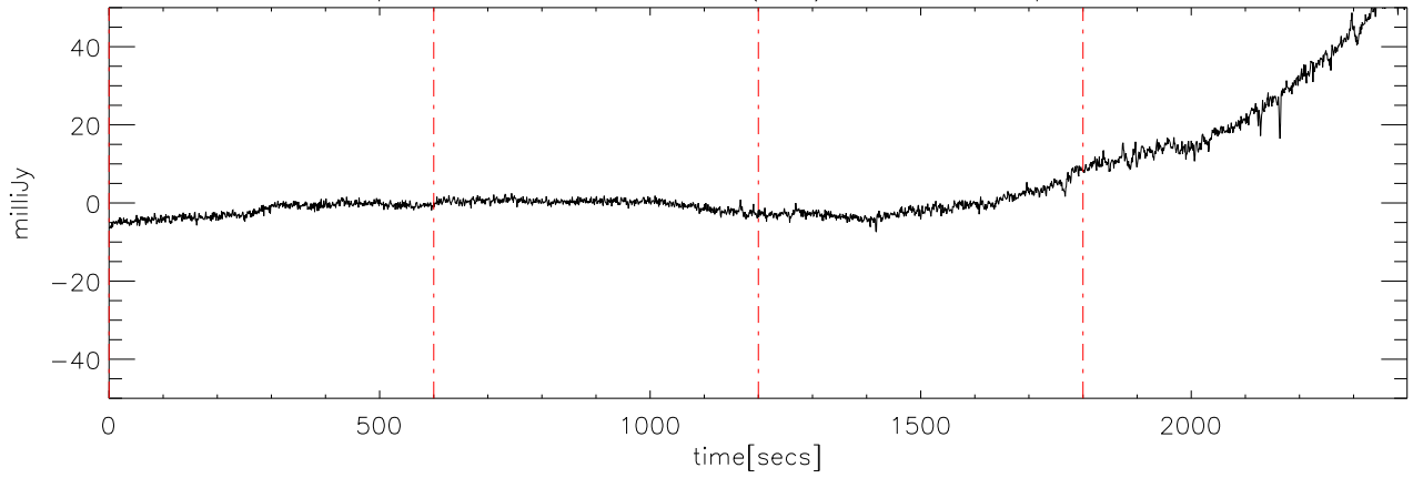
p2111 file:08 28dec08 (AST) StokesU freq:4725.
