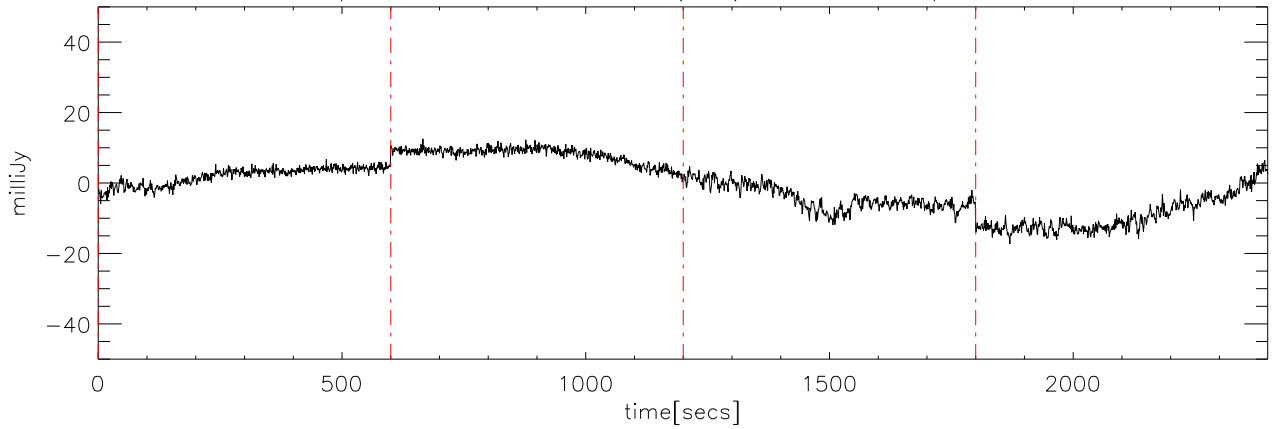
p2111 file:08 28dec08 (AST) StokesU freq:5250.
