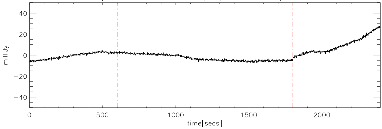
p2111 file:08 28dec08 (AST) StokesU freq:5125.
