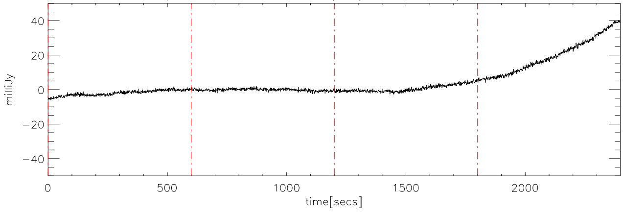
p2111 file:08 28dec08 (AST) StokesU freq:4600.
