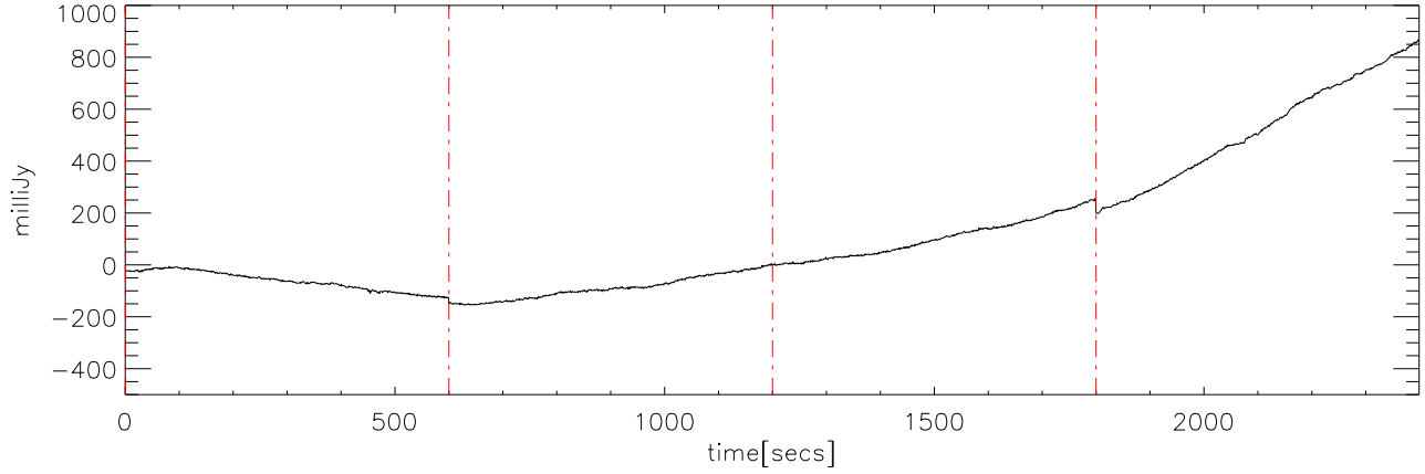
p2111 file:04 29dec08 (AST) StokesI freq:5000.
