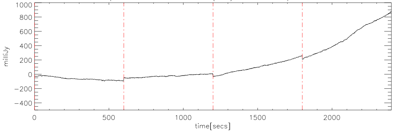
p2111 file:04 29dec08 (AST) StokesI freq:5125.
