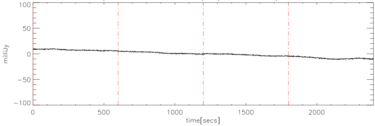
p2111 file:04 29dec08 (AST) StokesU freq:5125.
