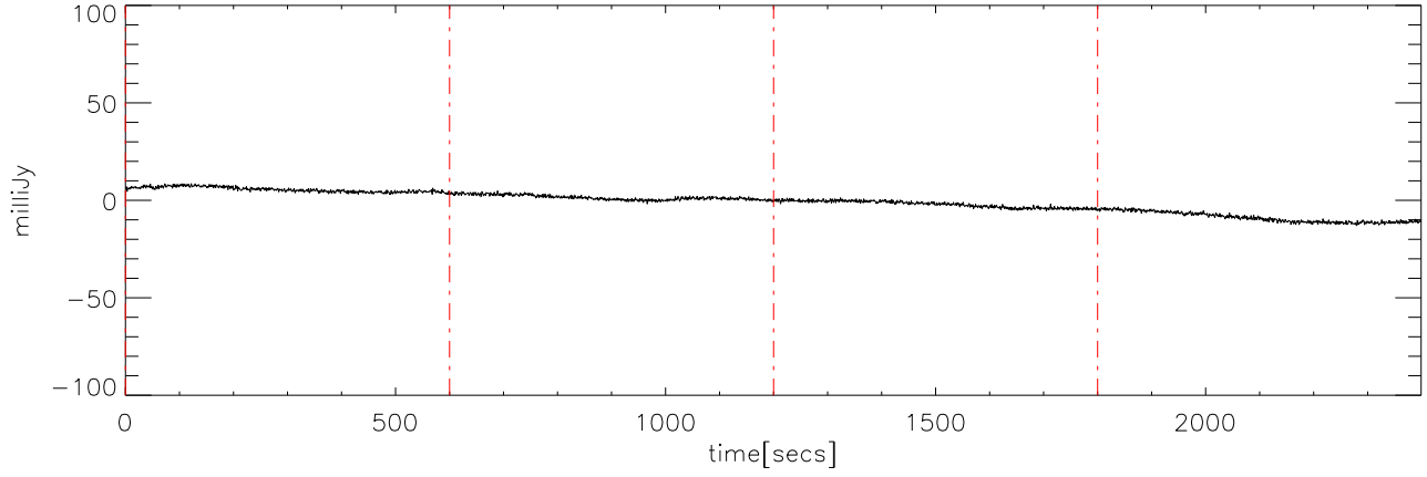
p2111 file:04 29dec08 (AST) StokesU freq:5000.
