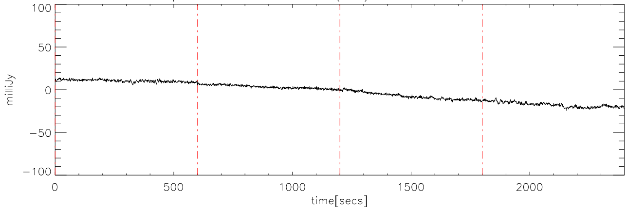
p2111 file:04 29dec08 (AST) StokesU freq:5250.
