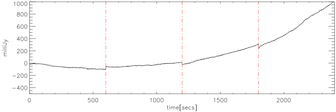
p2111 file:04 29dec08 (AST) StokesI freq:5250.
