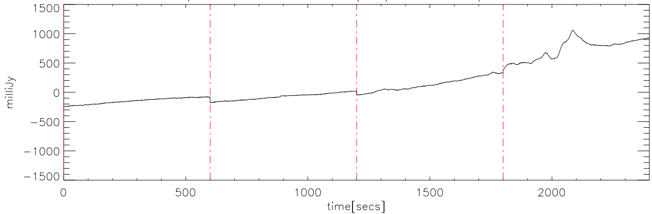
p2111 file:00 28dec08 (AST) StokesI freq:5250.
