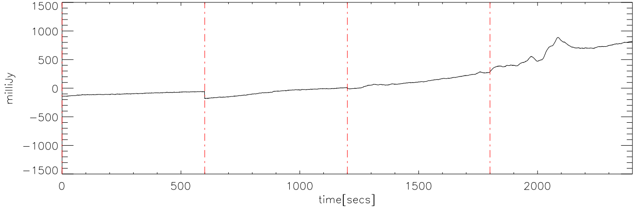
p2111 file:00 28dec08 (AST) StokesI freq:5000.
