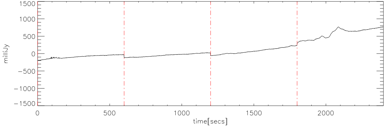
p2111 file:00 28dec08 (AST) StokesI freq:4475.
