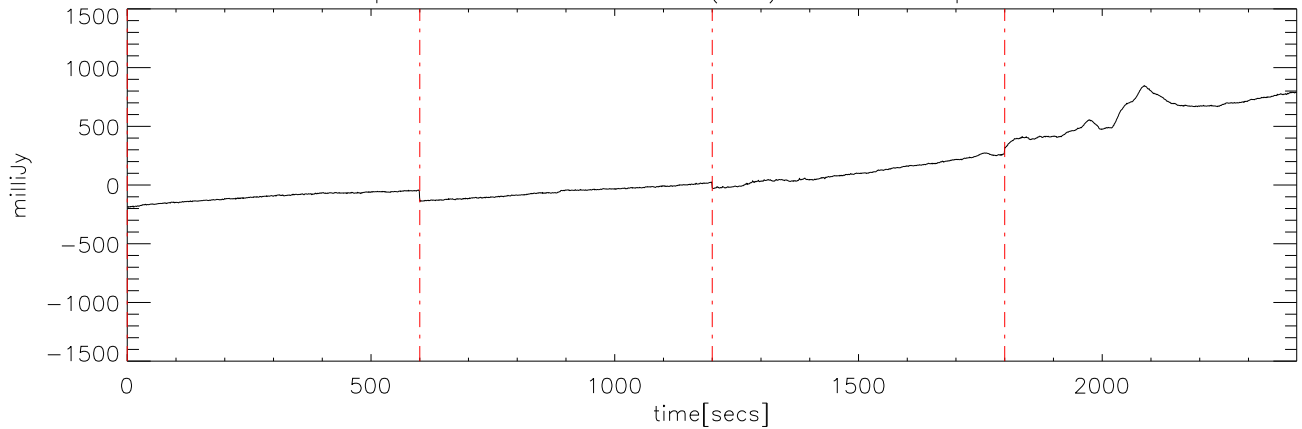
p2111 file:00 28dec08 (AST) StokesI freq:4725.
