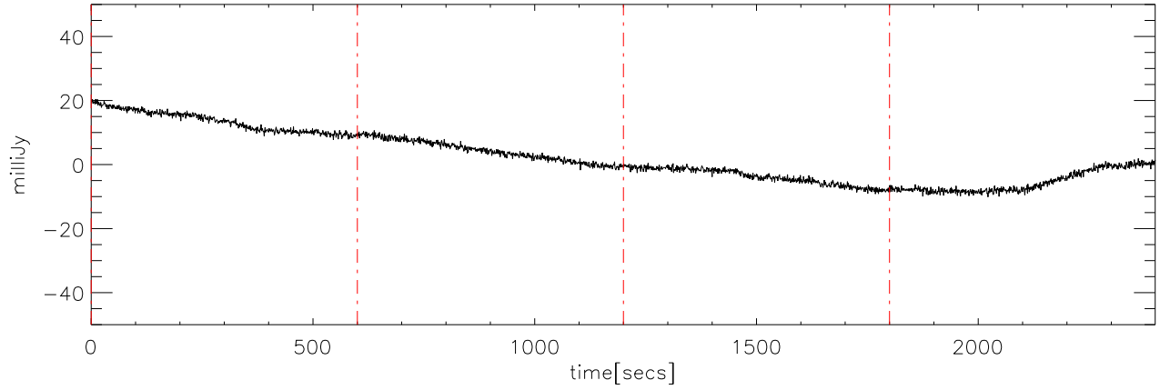
p2111 file:00 28dec08 (AST) StokesU freq:5000.
