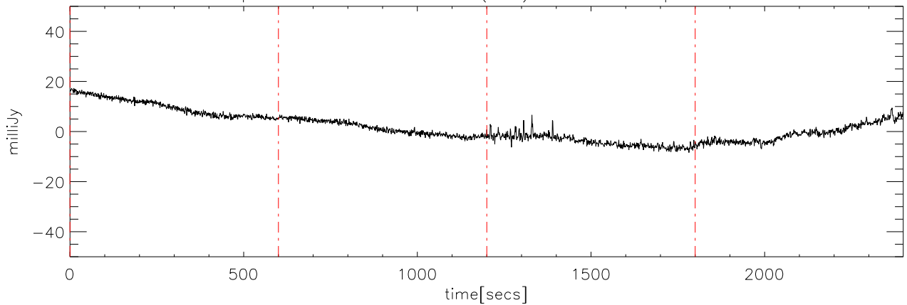
p2111 file:00 28dec08 (AST) StokesU freq:4725.
