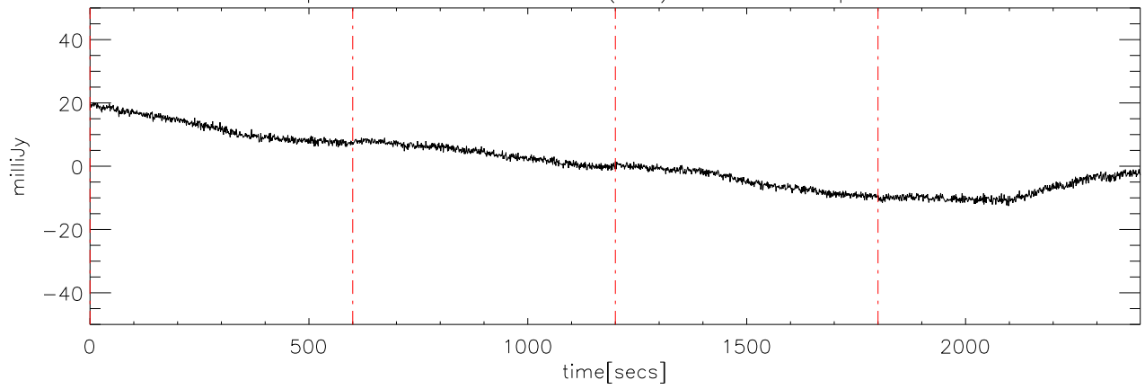
p2111 file:00 28dec08 (AST) StokesU freq:5125.
