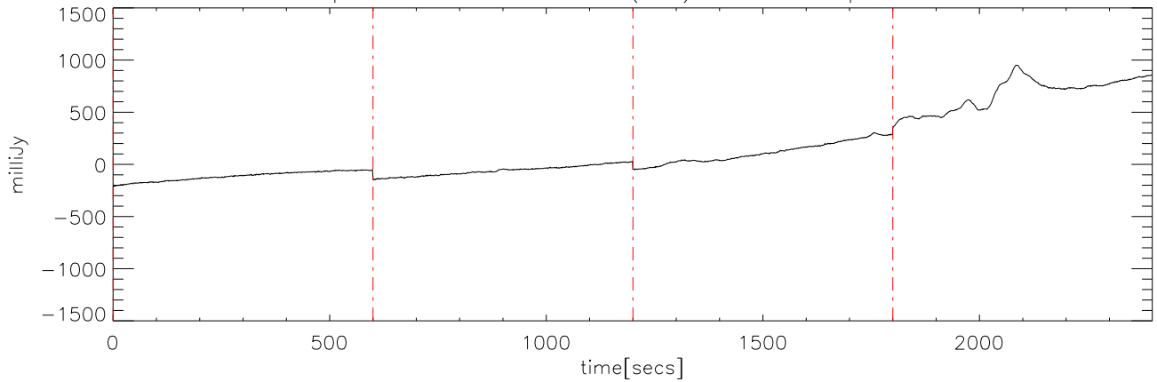
p2111 file:00 28dec08 (AST) StokesI freq:5125.
