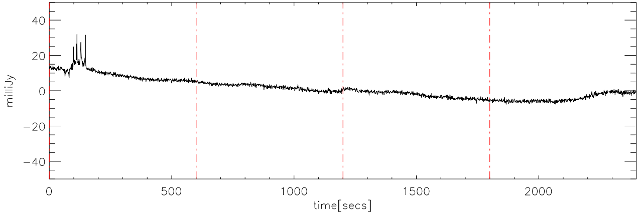
p2111 file:00 28dec08 (AST) StokesU freq:4475.
