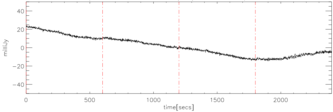
p2111 file:00 28dec08 (AST) StokesU freq:5250.
