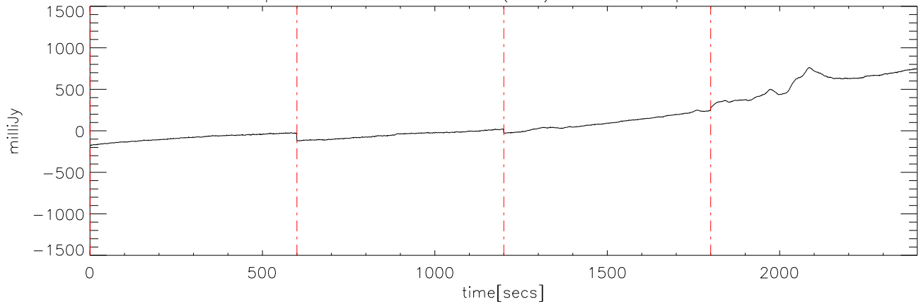
p2111 file:00 28dec08 (AST) StokesI freq:4600.
