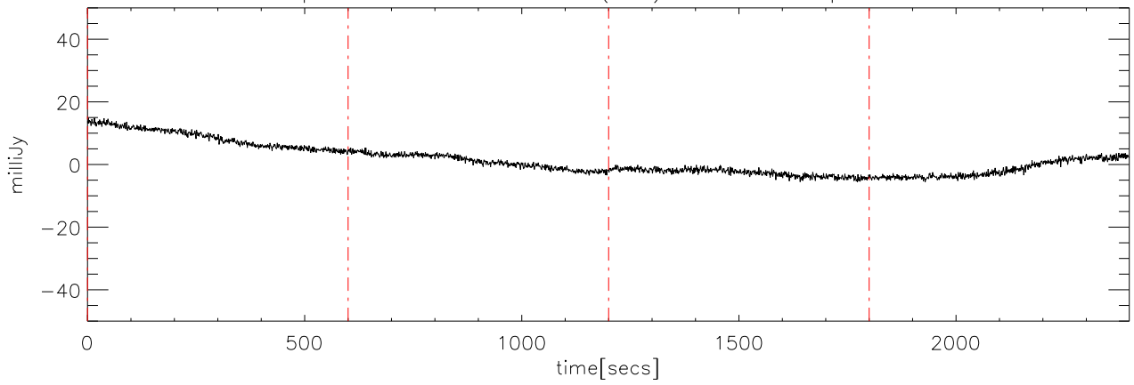
p2111 file:00 28dec08 (AST) StokesU freq:4600.
