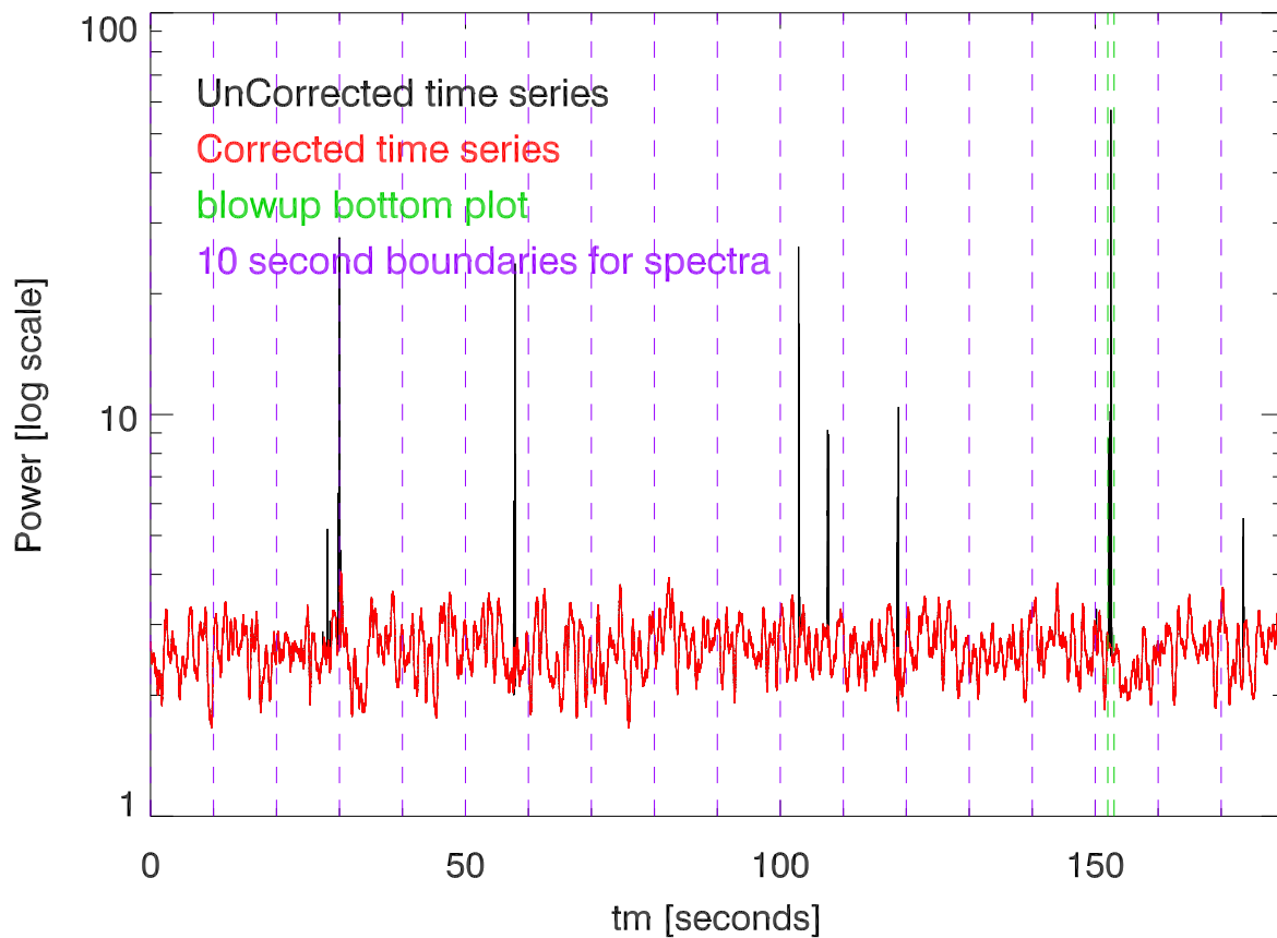
190808 327 B1005+077. PoIA TotPwr vs time on Source.
