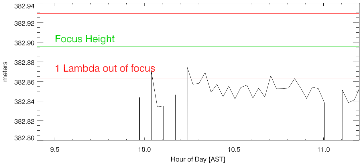
Platform average height during bm440
