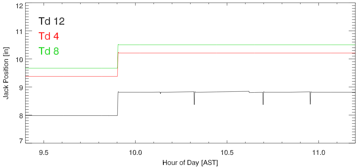
180617 tiedown position during bm440
