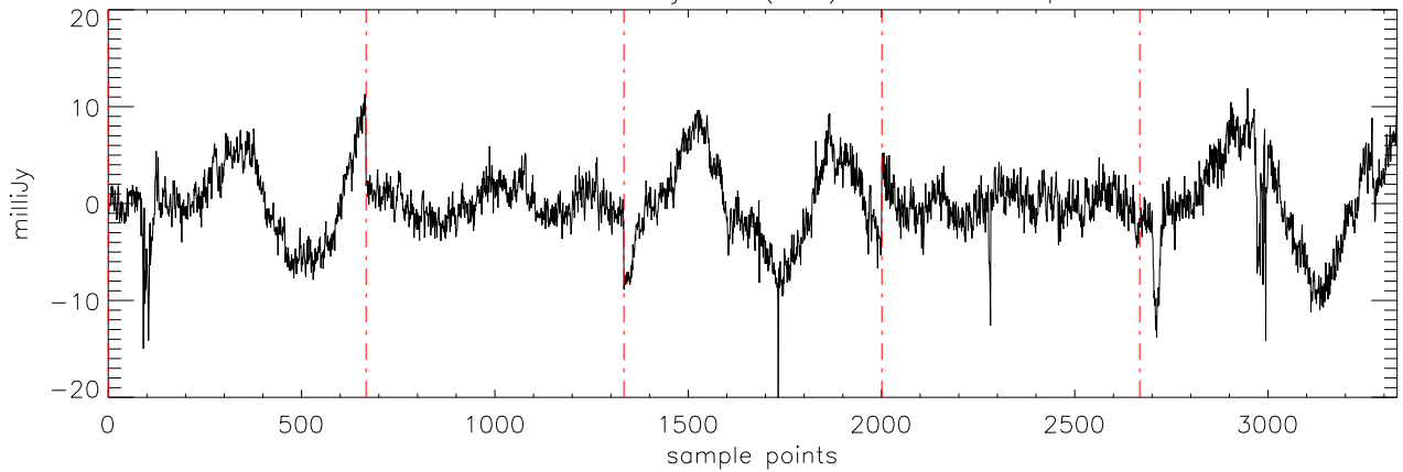
a2471 J1841086 18jul11 (AST) StokesQ freq:4750.
