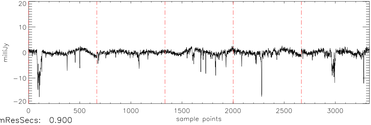
a2471 J1841086 18jul11 (AST) StokesU freq:5034.
