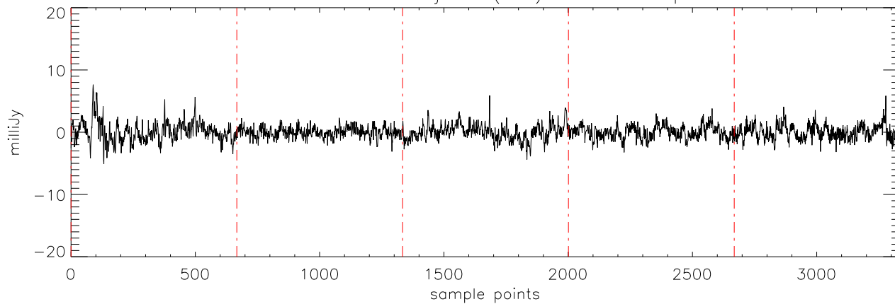
a2471 J1841086 18jul11 (AST) StokesV freq:5176.
