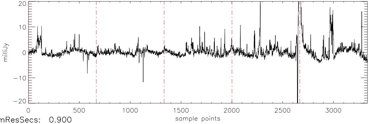
a2471 J1841086 18jul11 (AST) StokesU freq:4466.
