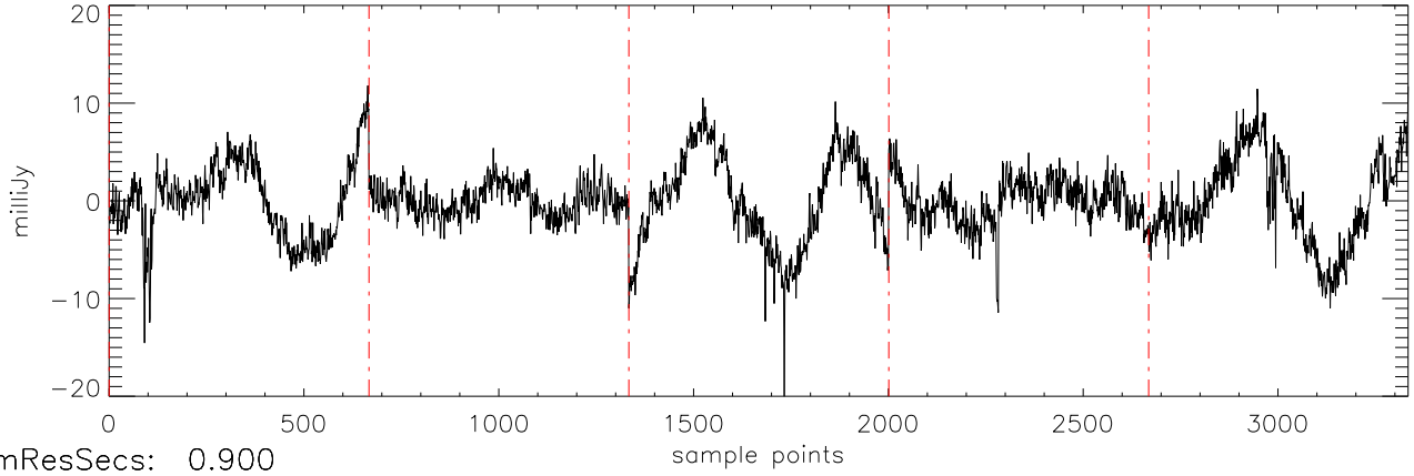
a2471 J1841086 18jul11 (AST) StokesQ freq:5034.
