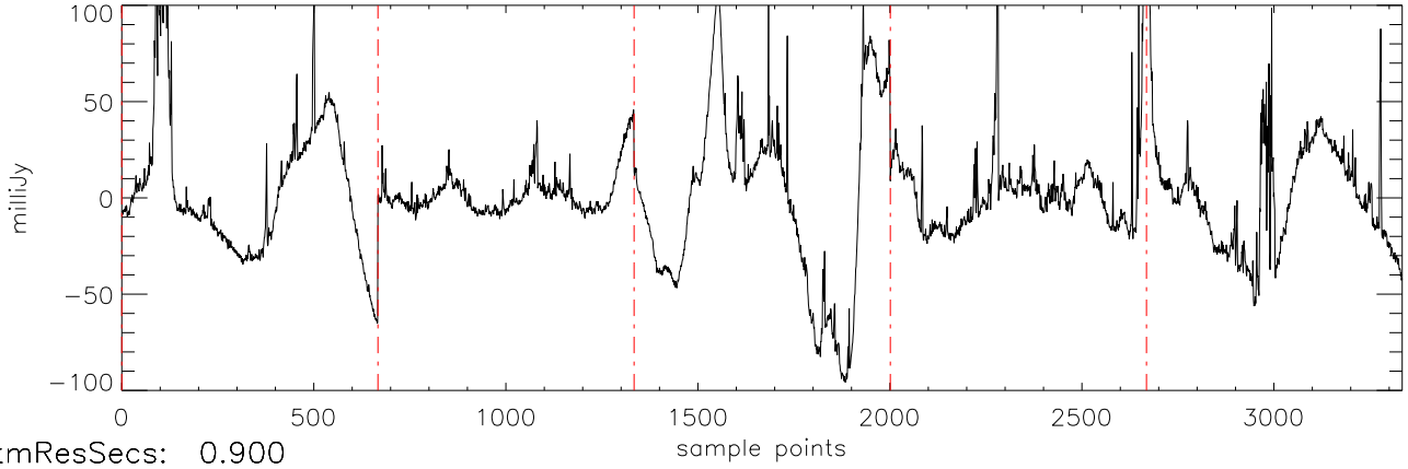
\alpha 2471 J1841086 18jul11 (AST) StokesI freq:4466.
