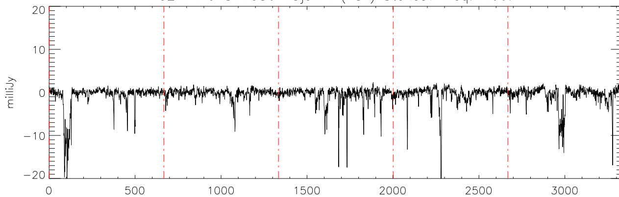
a2471 J1841086 18jul11 (AST) StokesV freq:4466.
