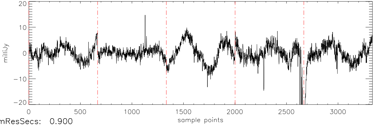
a2471 J1841086 18jul11 (AST) StokesQ freq:4466.
