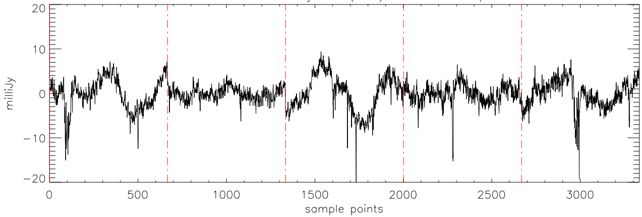
a2471 J1841086 18jul11 (AST) StokesQ freq:4608.
