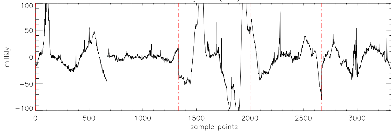
\alpha 2471 J1841086 18jul11 (AST) StokesI freq:5176.
