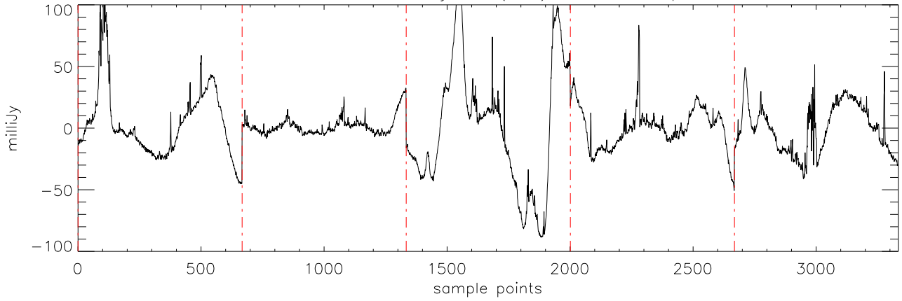
\alpha 2471 J1841086 18jul11 (AST) StokesI freq:4750.
