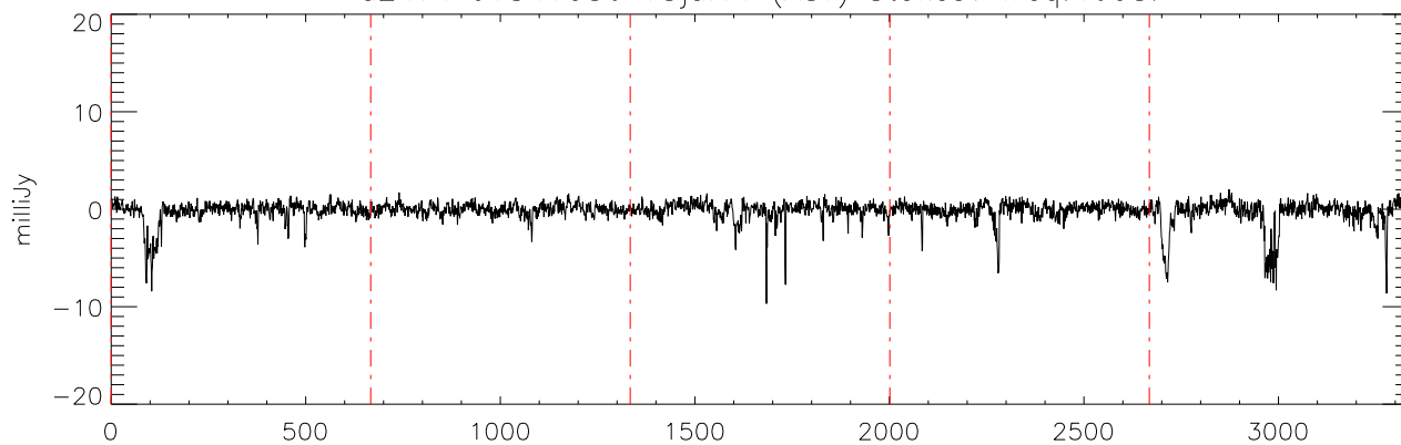
a2471 J1841086 18jul11 (AST) StokesV freq:4608.
