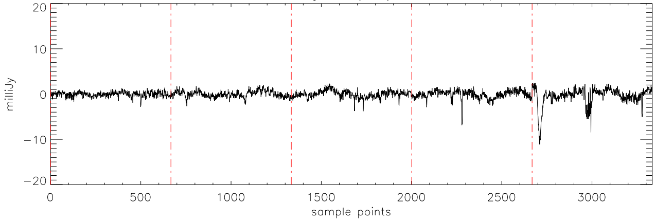
a2471 J1841086 18jul11 (AST) StokesU freq:4750.
