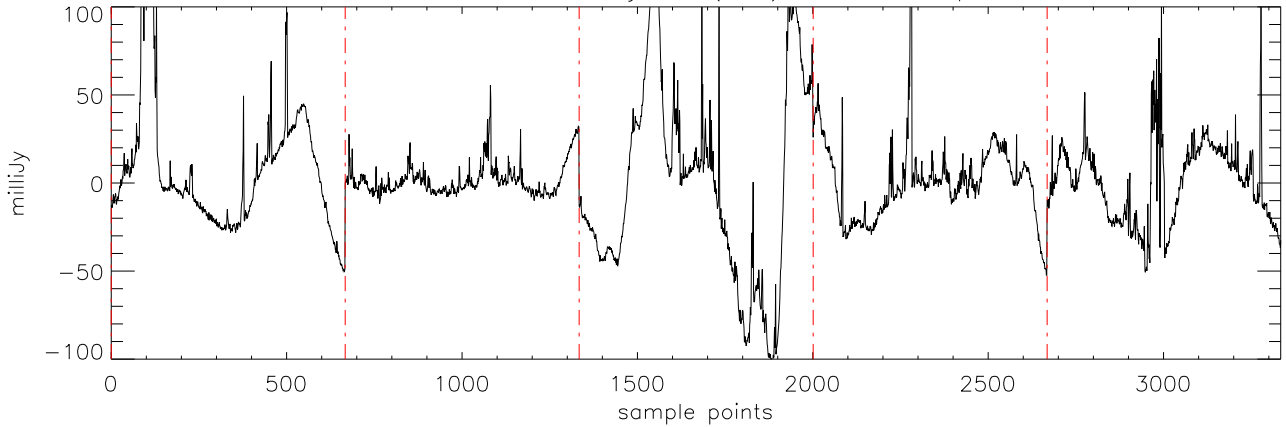
\alpha 2471 J1841086 18jul11 (AST) StokesI freq:4750.
