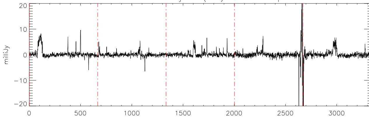
a2471 J1841086 18jul11 (AST) StokesV freq:4325.
