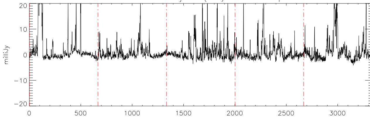
a2471 J1841086 18jul11 (AST) StokesV freq:4750.
