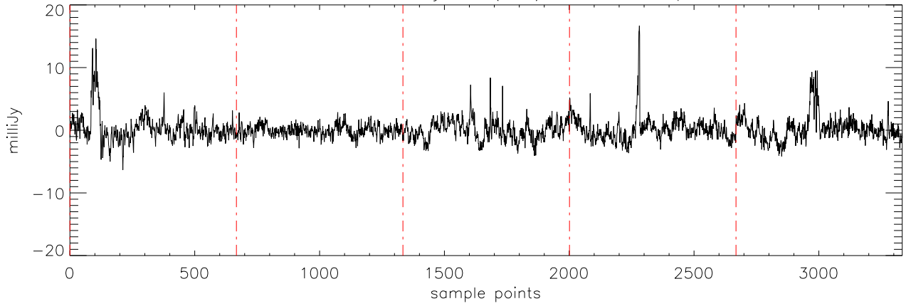
a2471 J1841086 18jul11 (AST) StokesU freq:5176.
