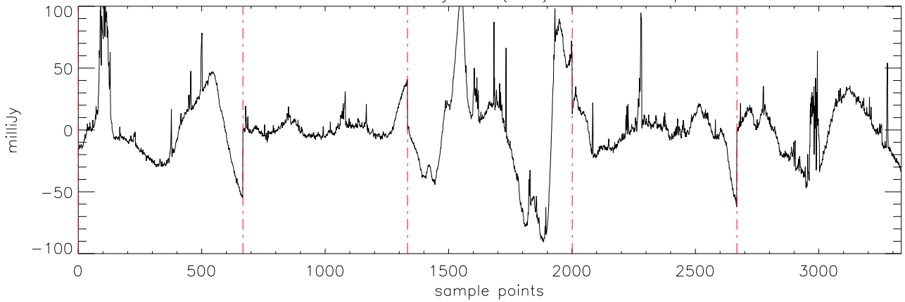
\alpha 2471 J1841086 18jul11 (AST) StokesI freq:4608.
