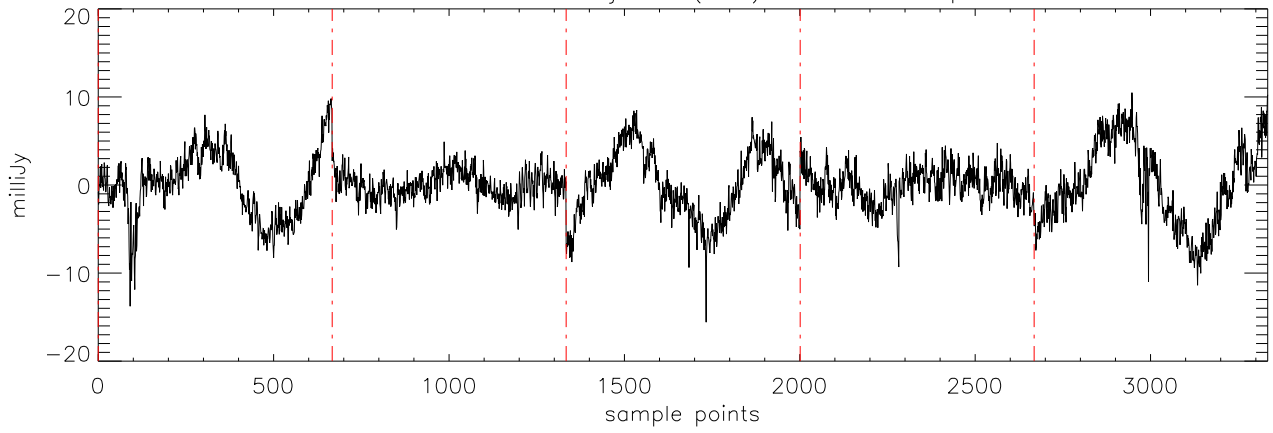
a2471 J1841086 18jul11 (AST) StokesQ freq:5176.
