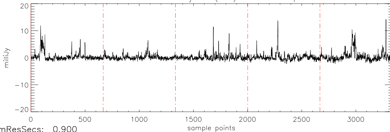
a2471 J1841086 18jul11 (AST) StokesV freq:5034.
