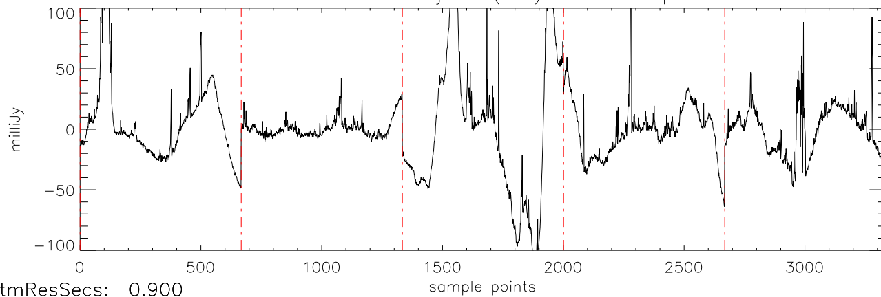
\alpha 2471 J1841086 18jul11 (AST) StokesI freq:5034.
