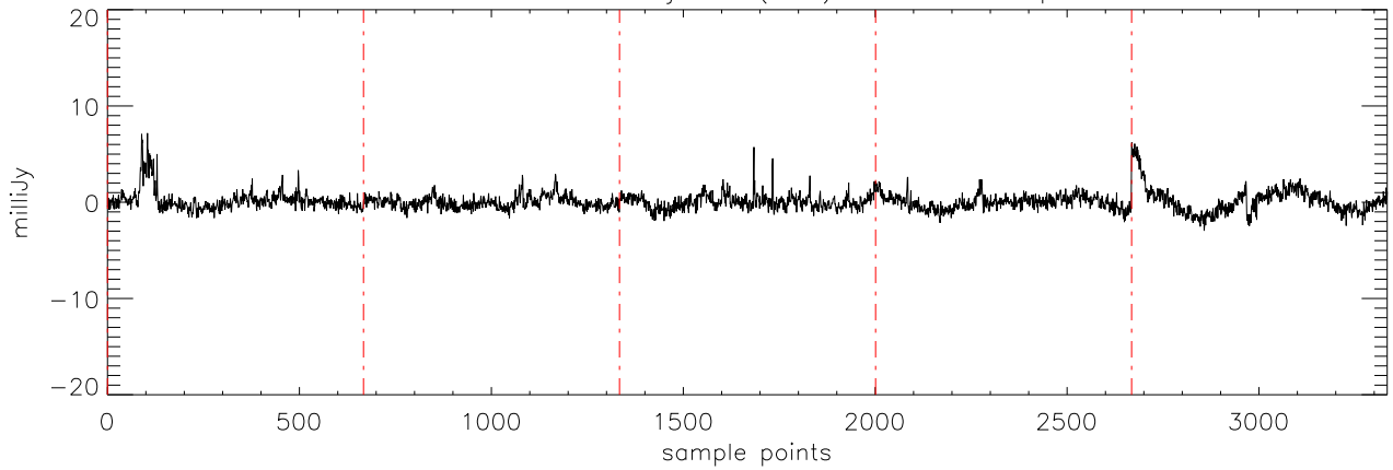
a2471 J1841086 18jul11 (AST) StokesU freq:4608.
