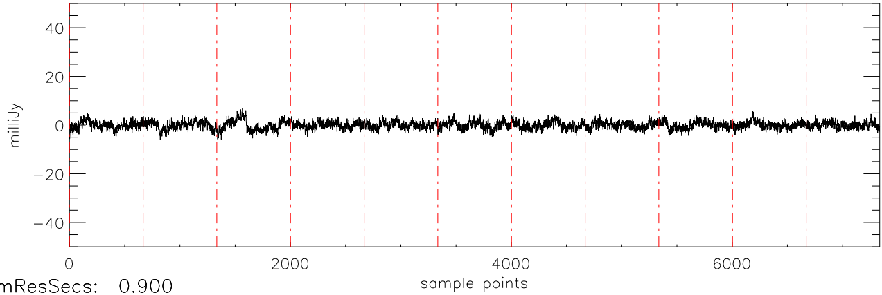
a2471 J10475385 30nov10 (AST) StokesQ freq:5034.
