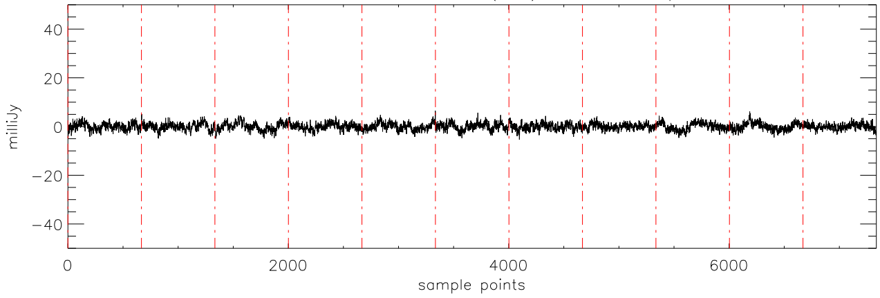
a2471 J10475385 30nov10 (AST) StokesQ freq:4608.
