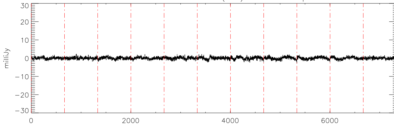
a2471 J10475385 30nov10 (AST) StokesU freq:5176.
