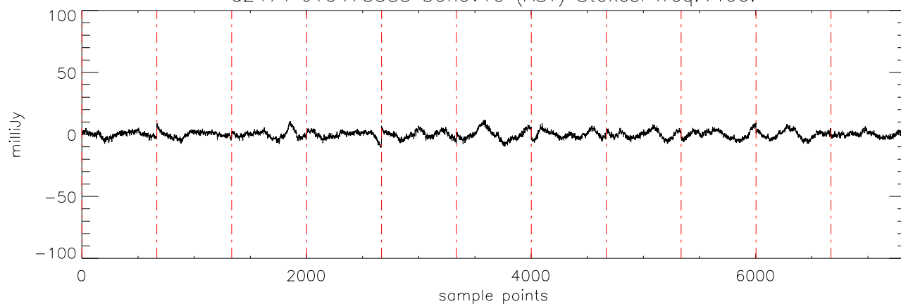
a2471 J10475385 30nov10 (AST) StokesI freq:4608.
