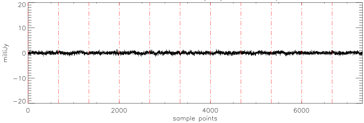
a2471 J10475385 30nov10 (AST) StokesV freq:4608.
