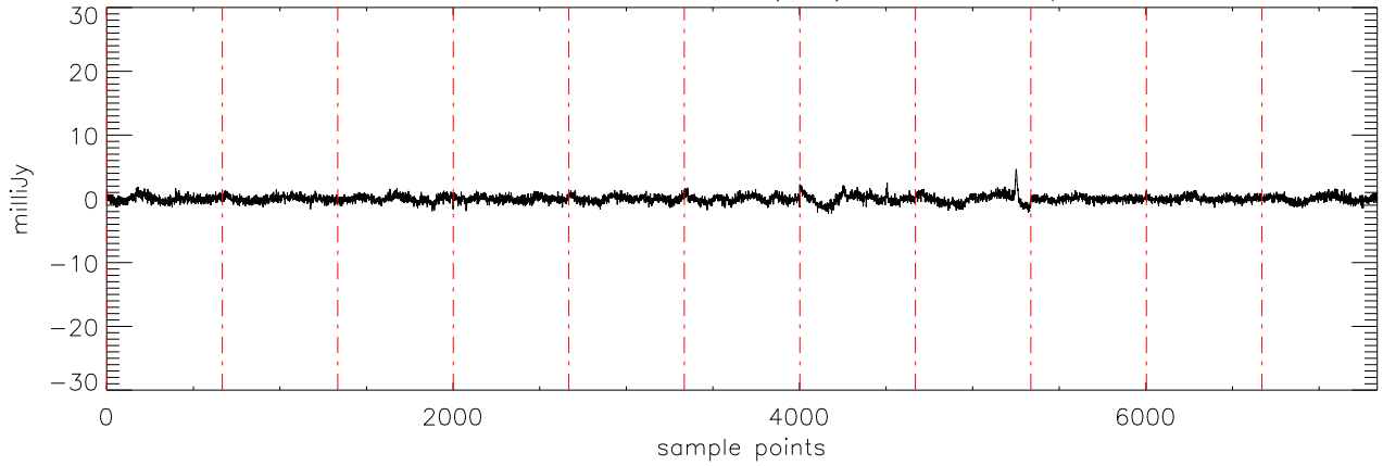
a2471 J10475385 30nov10 (AST) StokesU freq:4750.
