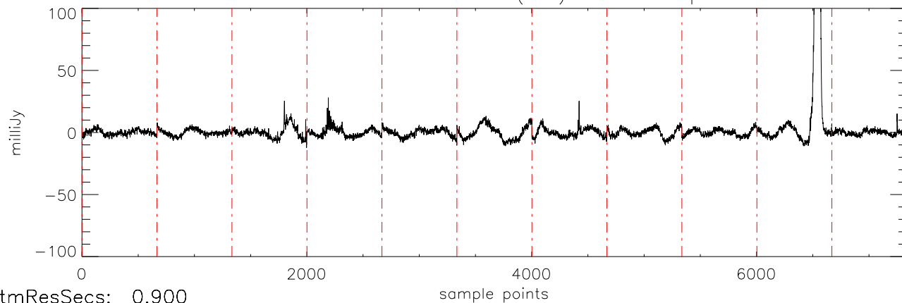
a2471 J10475385 30nov10 (AST) StokesI freq:4466.
