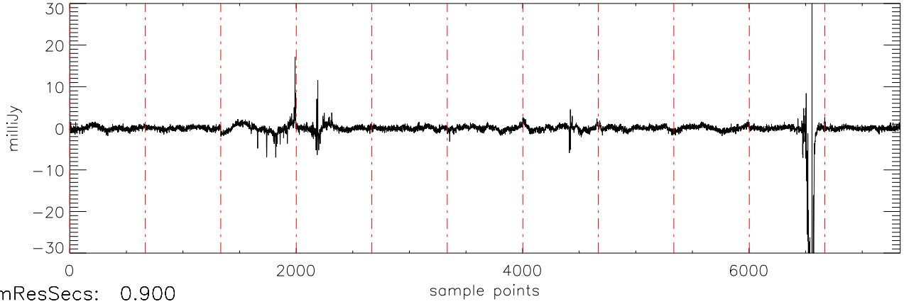
a2471 J10475385 30nov10 (AST) StokesU freq:4466.
