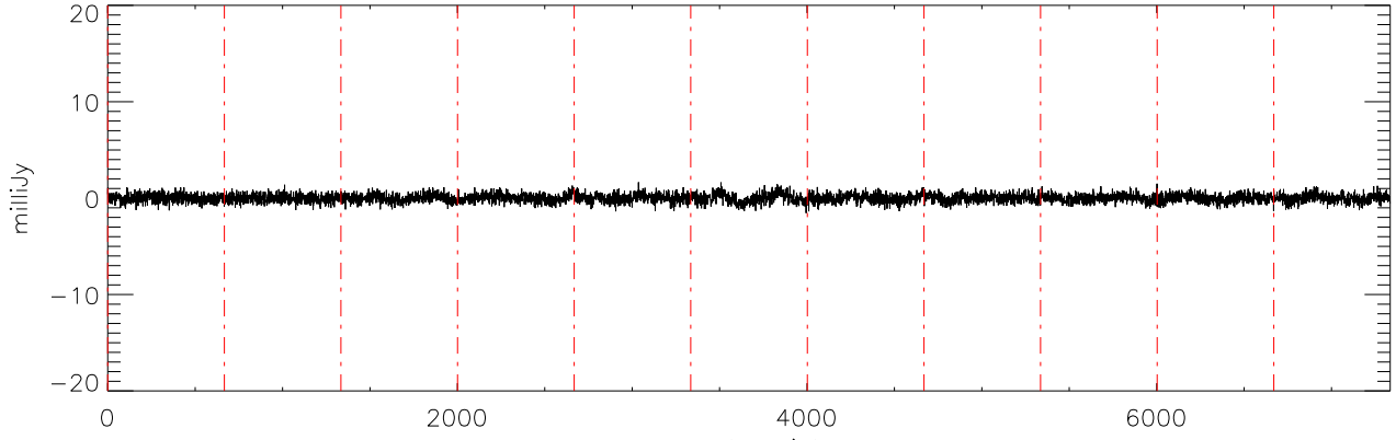
a2471 J10475385 30nov10 (AST) StokesV freq:4892.
