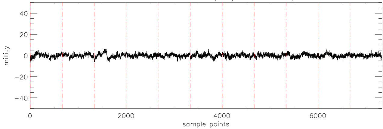
a2471 J10475385 30nov10 (AST) StokesQ freq:5176.
