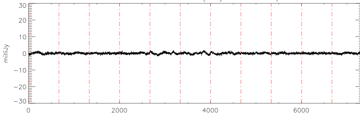
a2471 J10475385 30nov10 (AST) StokesU freq:4892.
