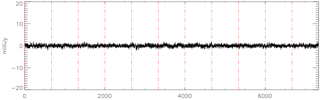
a2471 J10475385 30nov10 (AST) StokesV freq:5176.
