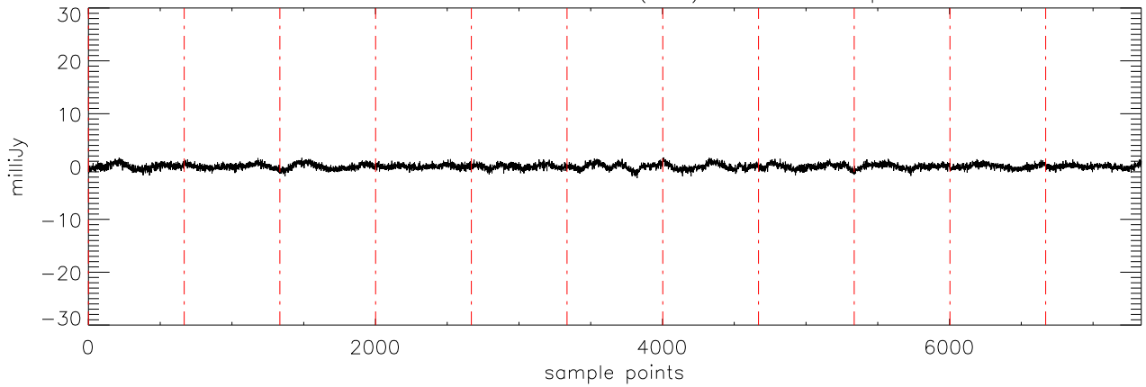
a2471 J10475385 30nov10 (AST) StokesU freq:4608.
