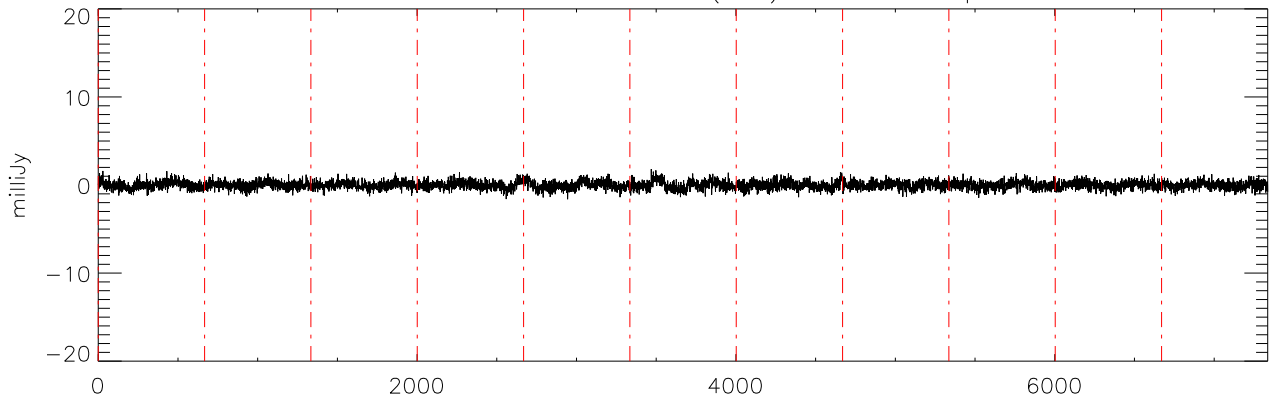
a2471 J10475385 30nov10 (AST) StokesV freq:5034.
