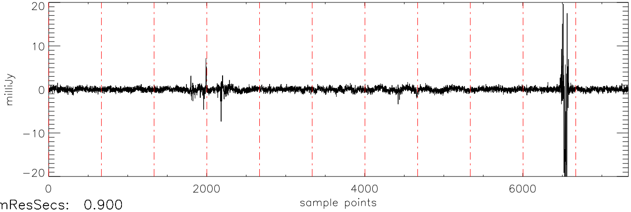
a2471 J10475385 30nov10 (AST) StokesV freq:4466.
