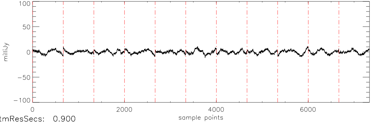
a2471 J10475385 30nov10 (AST) StokesI freq:5034.
