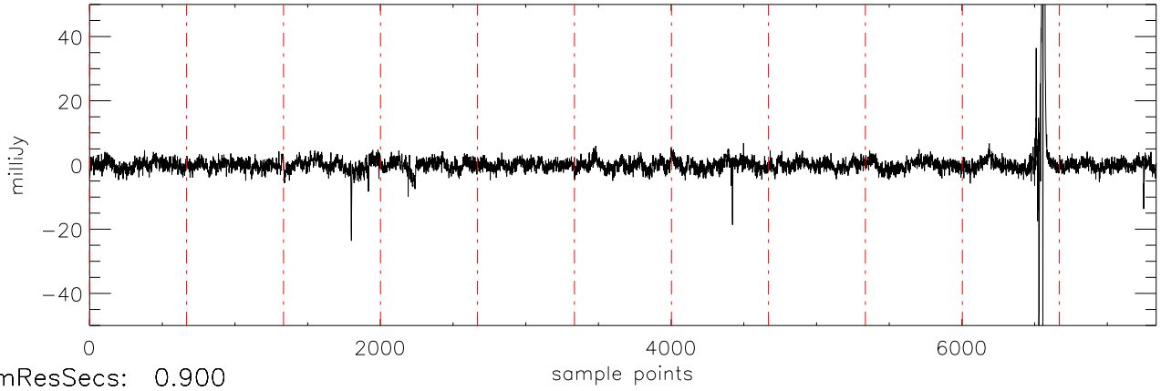
a2471 J10475385 30nov10 (AST) StokesQ freq:4466.
