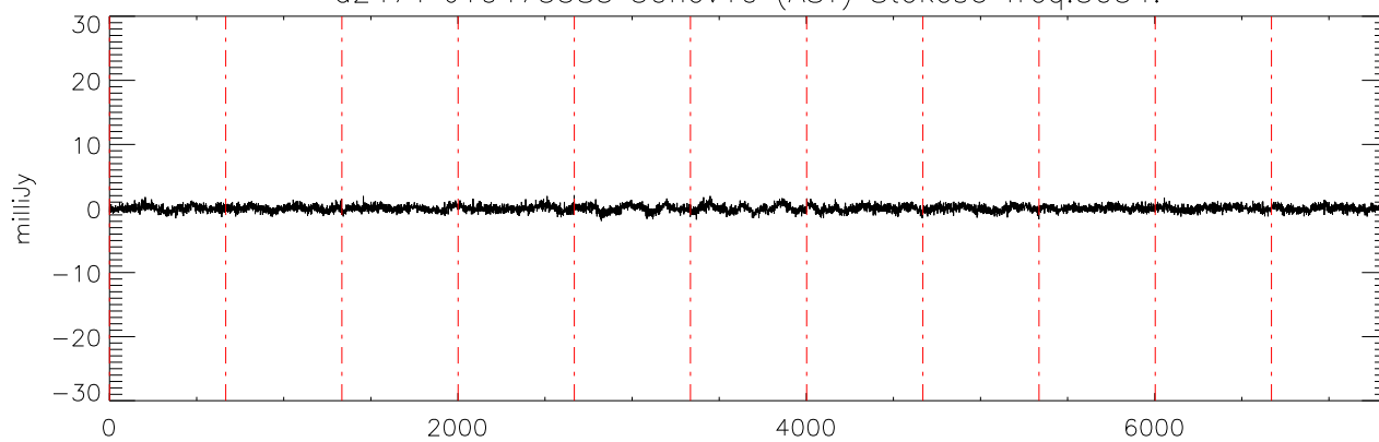
a2471 J10475385 30nov10 (AST) StokesU freq:5034.
