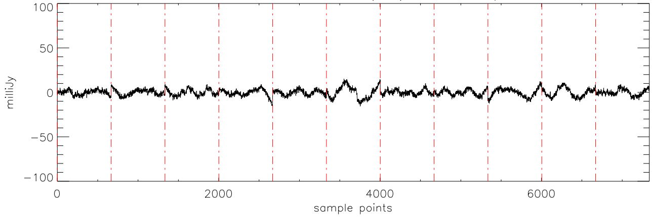
a2471 J10475385 30nov10 (AST) StokesI freq:5176.
