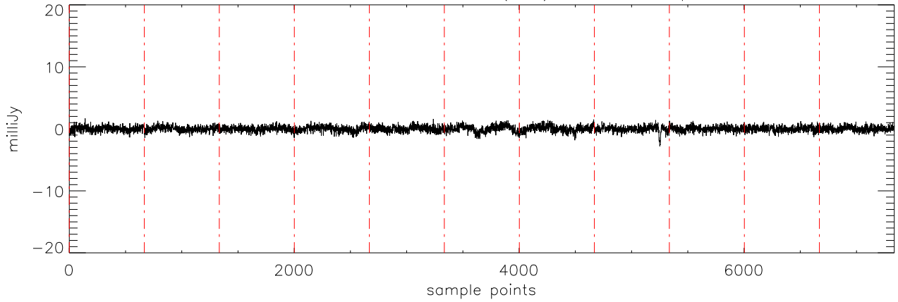
a2471 J10475385 30nov10 (AST) StokesV freq:4750.
