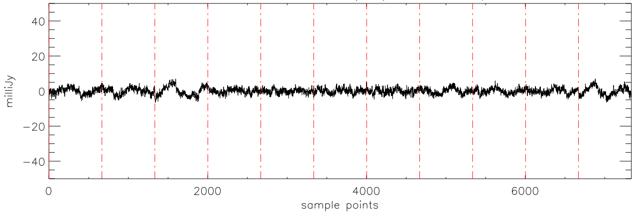
a2471 J10475385 30nov10 (AST) StokesQ freq:4750.
