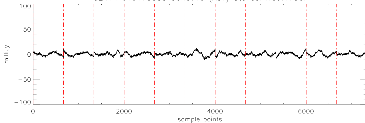
a2471 J10475385 30nov10 (AST) StokesI freq:4750.
