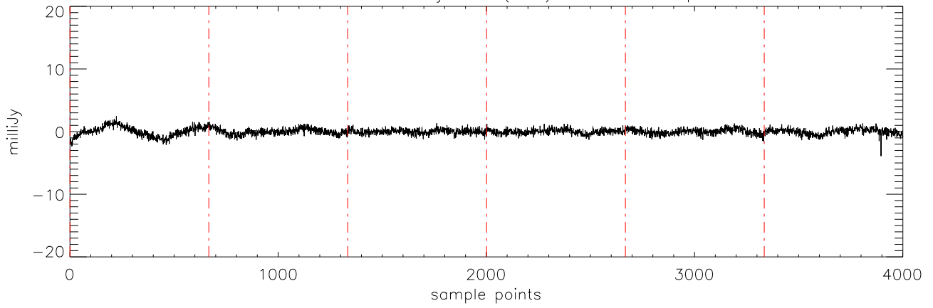
a2471 J10475385 11jan11 (AST) StokesU freq:4608.
