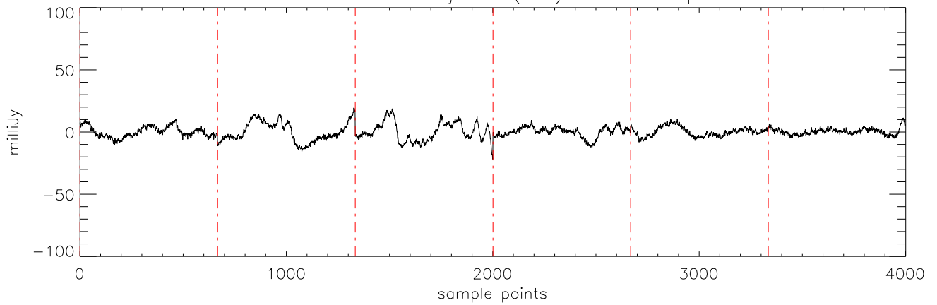
a2471 J10475385 11jan11 (AST) StokesI freq:5176.
