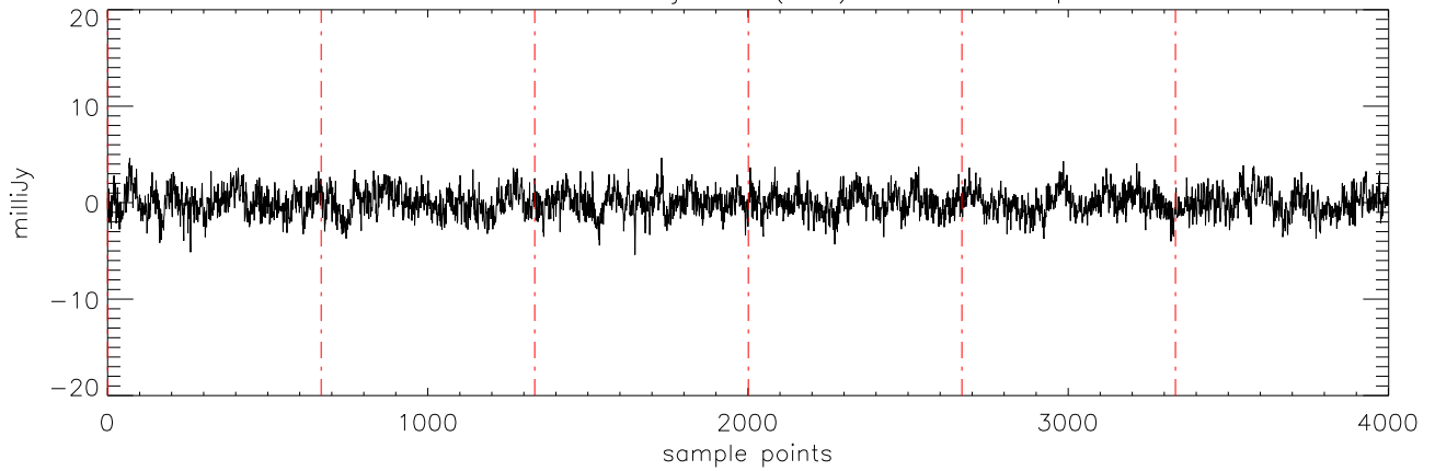
a2471 J10475385 11jan11 (AST) StokesQ freq:4608.
