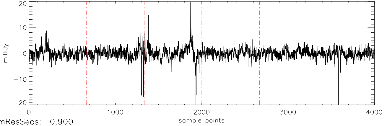
a2471 J10475385 11jan11 (AST) StokesQ freq:4466.
