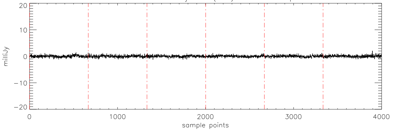
a2471 J10475385 11jan11 (AST) StokesV freq:4608.
