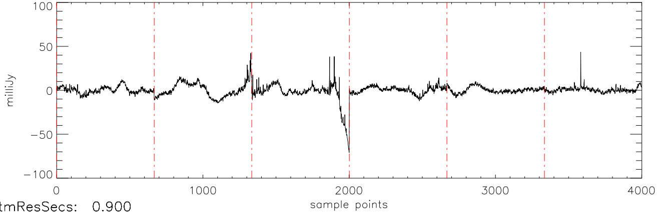
a2471 J10475385 11jan11 (AST) StokesI freq:4466.
