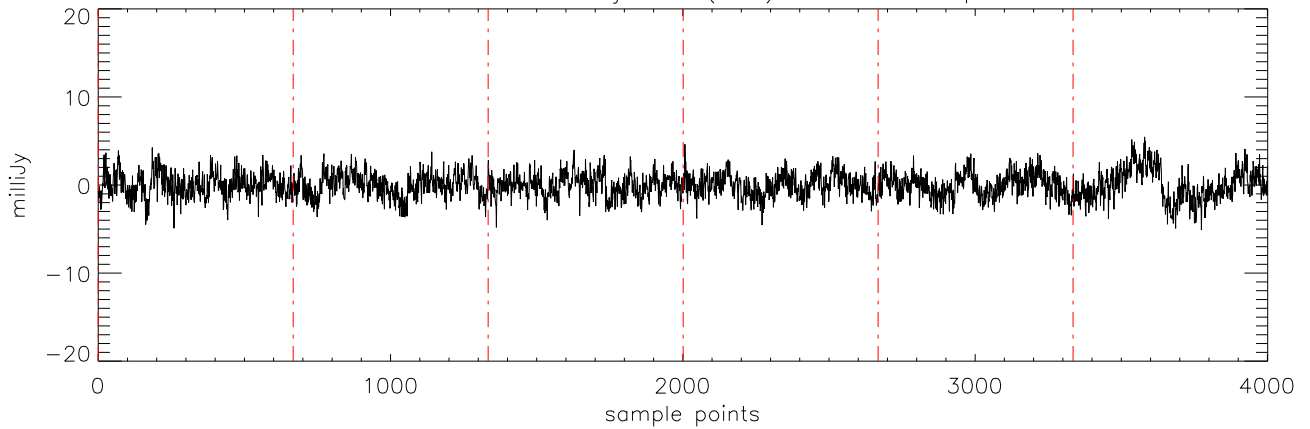
a2471 J10475385 11jan11 (AST) StokesQ freq:4750.
