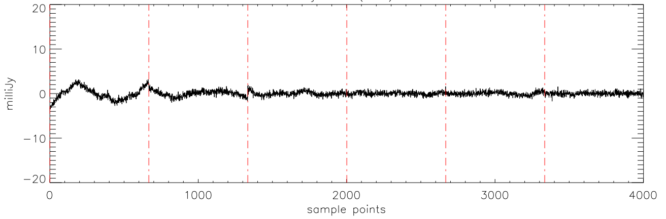
a2471 J10475385 11jan11 (AST) StokesU freq:5176.
