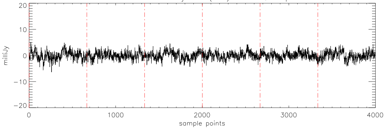
a2471 J10475385 11jan11 (AST) StokesQ freq:5176.
