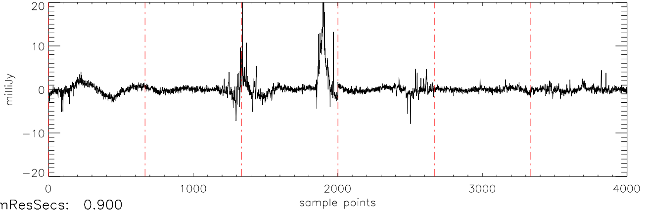
a2471 J10475385 11jan11 (AST) StokesU freq:4466.
