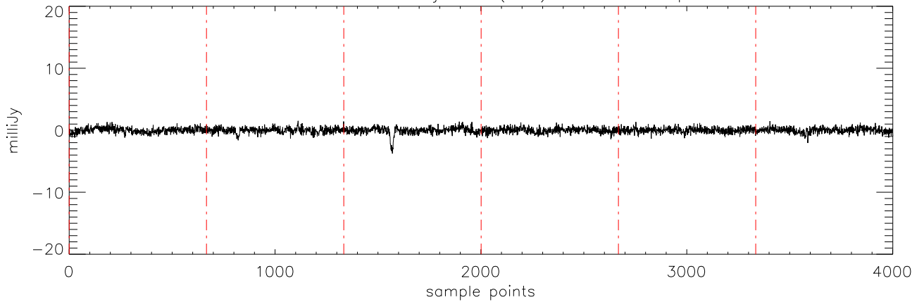
a2471 J10475385 11jan11 (AST) StokesV freq:4750.
