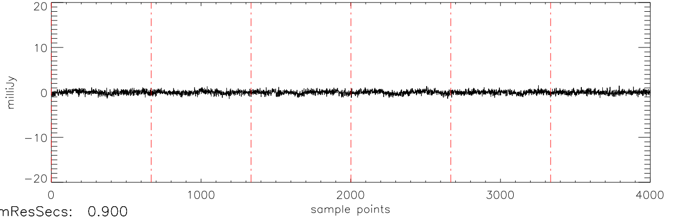
a2471 J10475385 11jan11 (AST) StokesV freq:5034.
