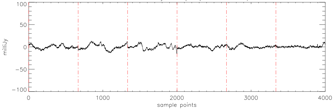
a2471 J10475385 11jan11 (AST) StokesI freq:4608.
