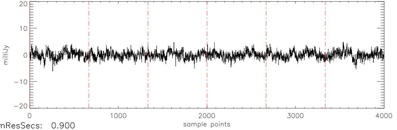
a2471 J10475385 11jan11 (AST) StokesQ freq:5034.
