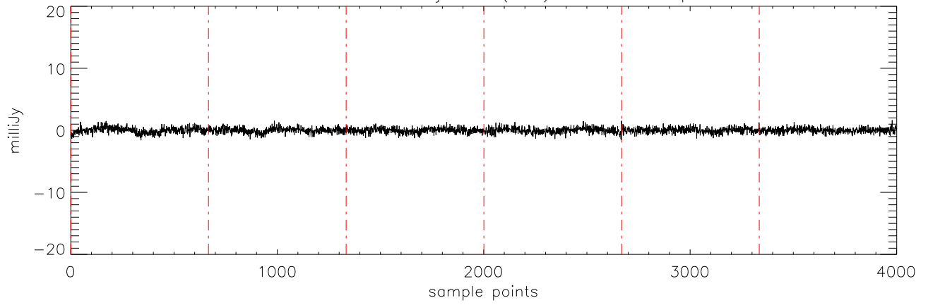
a2471 J10475385 11jan11 (AST) StokesV freq:5176.
