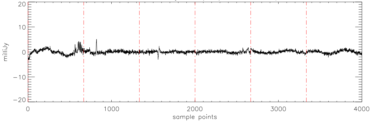
a2471 J10475385 11jan11 (AST) StokesU freq:4750.
