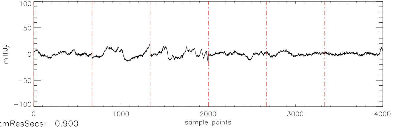
a2471 J10475385 11jan11 (AST) StokesI freq:5034.
