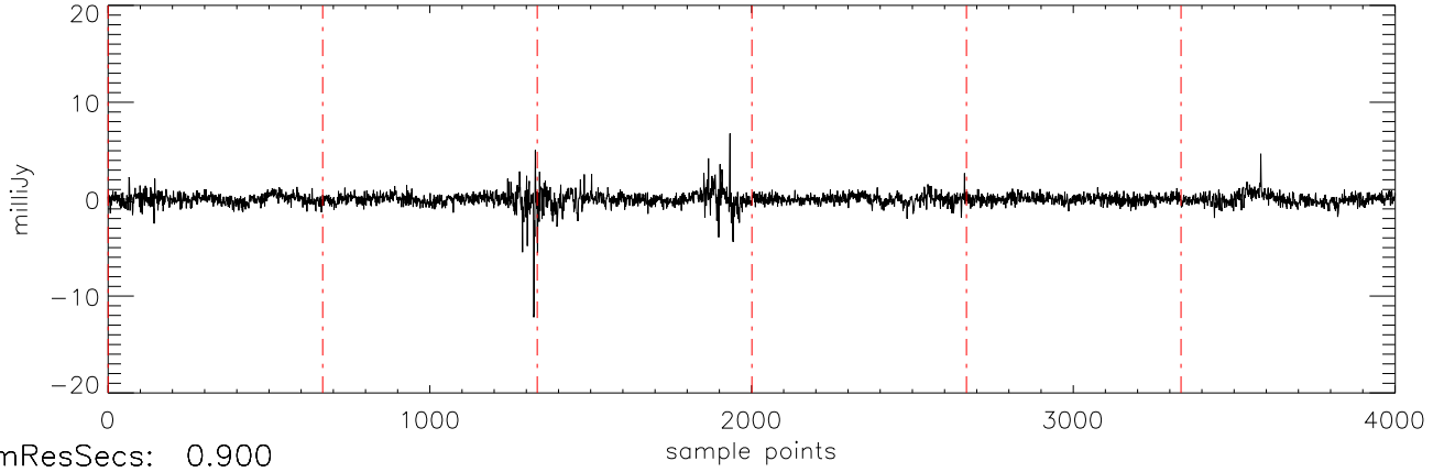
a2471 J10475385 11jan11 (AST) StokesV freq:4466.
