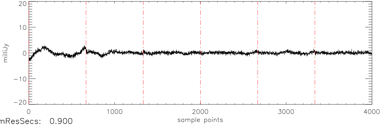
a2471 J10475385 11jan11 (AST) StokesU freq:5034.
