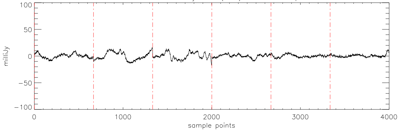
a2471 J10475385 11jan11 (AST) StokesI freq:4750.
