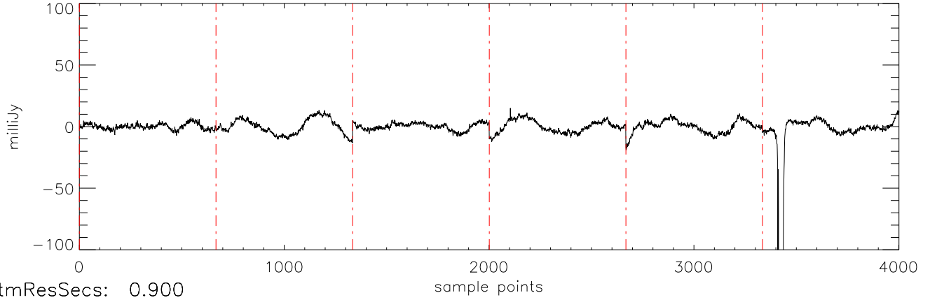
a2471 J09373487 03jan11 (AST) StokesI freq:5034.
