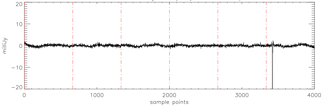
a2471 J09373487 03jan11 (AST) StokesU freq:4608.
