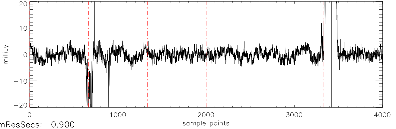
a2471 J09373487 03jan11 (AST) StokesQ freq:4466.
