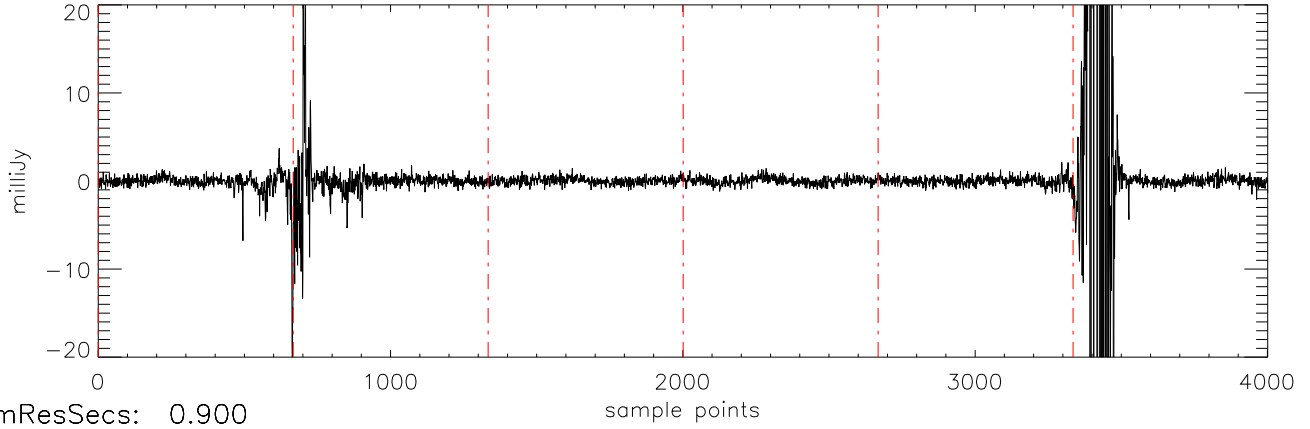
a2471 J09373487 03jan11 (AST) StokesV freq:4466.
