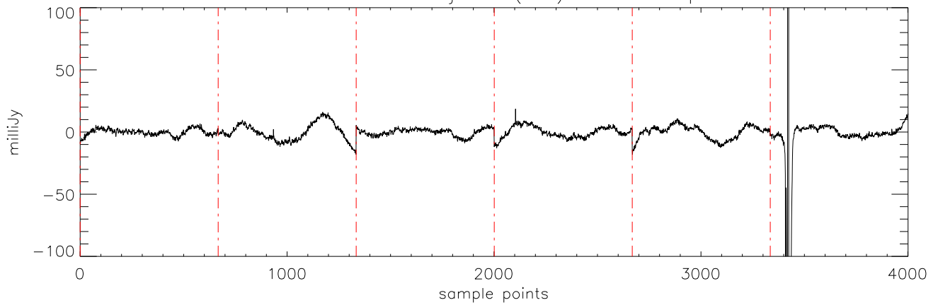
a2471 J09373487 03jan11 (AST) StokesI freq:4608.
