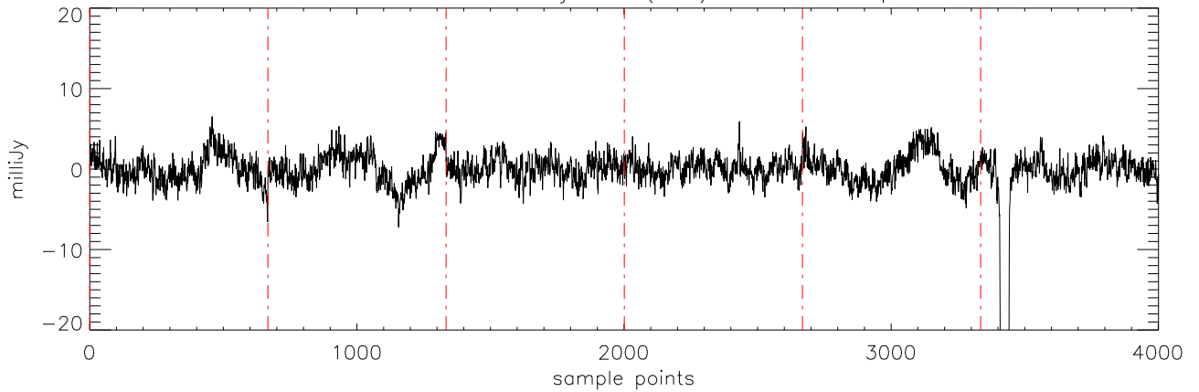
a2471 J09373487 03jan11 (AST) StokesQ freq:4750.
