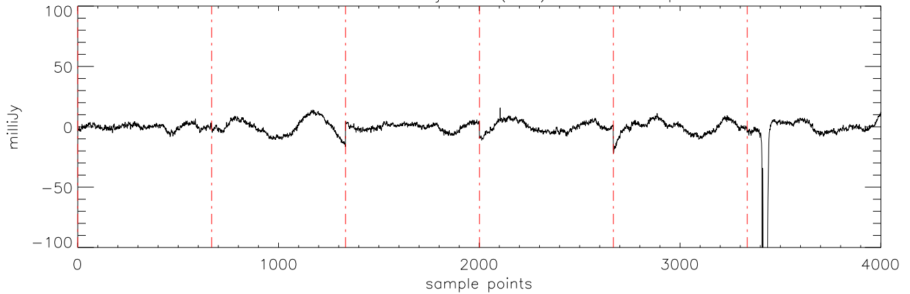
a2471 J09373487 03jan11 (AST) StokesI freq:4750.
