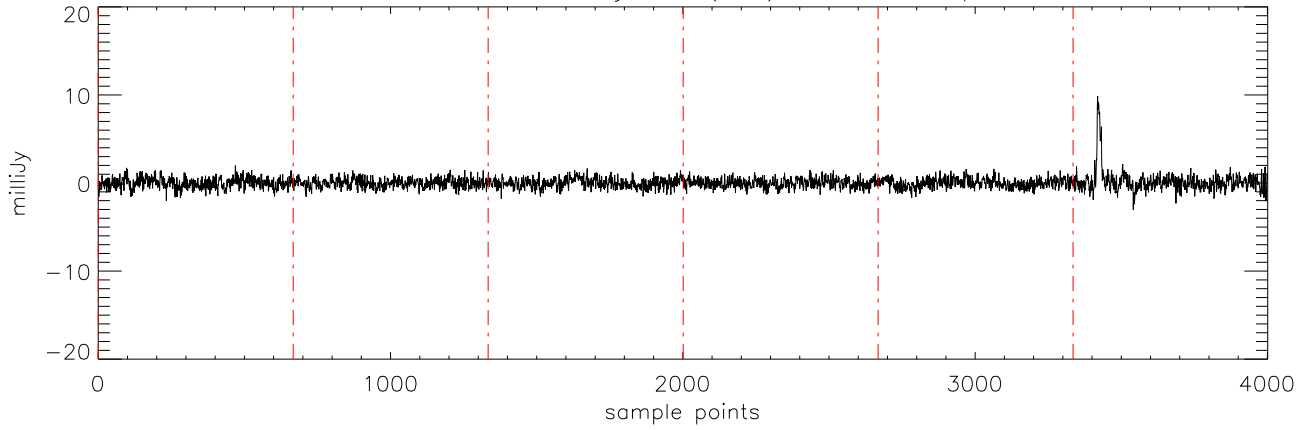
a2471 J09373487 03jan11 (AST) StokesV freq:5176.
