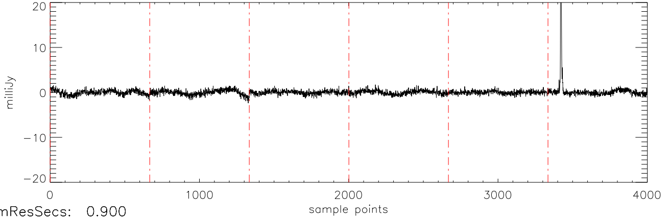
a2471 J09373487 03jan11 (AST) StokesU freq:5034.
