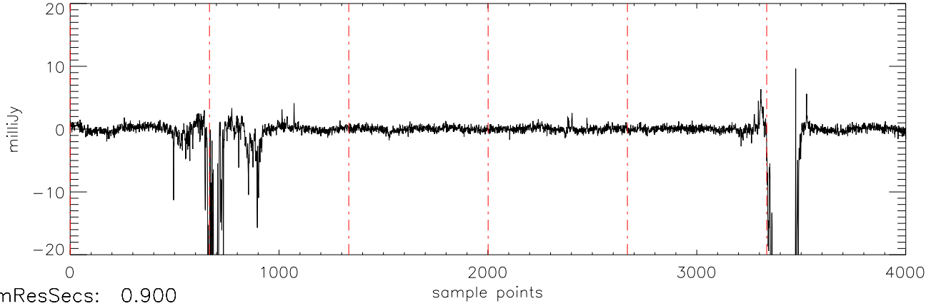
a2471 J09373487 03jan11 (AST) StokesU freq:4466.
