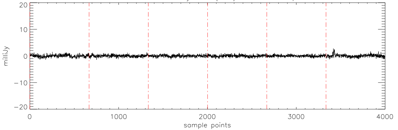
a2471 J09373487 03jan11 (AST) StokesV freq:4750.
