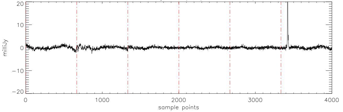
a2471 J09373487 03jan11 (AST) StokesU freq:4750.
