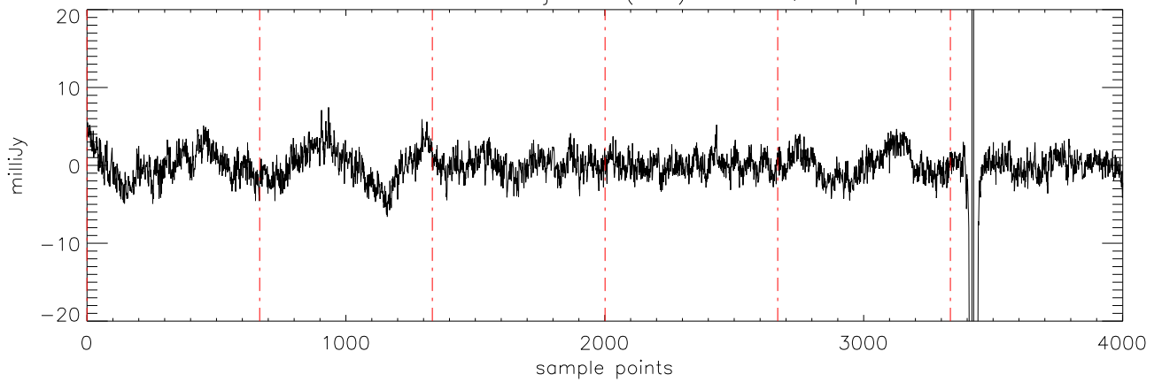
a2471 J09373487 03jan11 (AST) StokesQ freq:4608.
