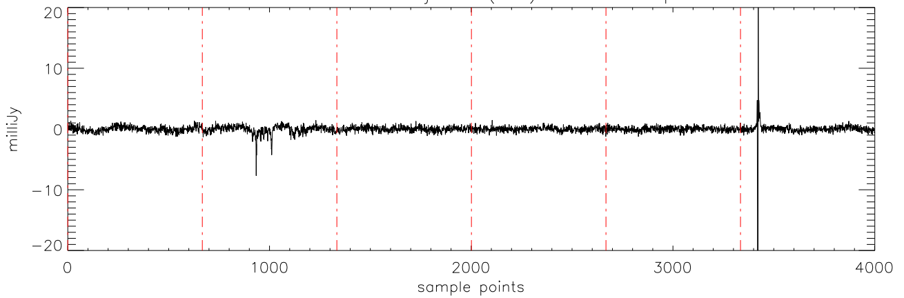
a2471 J09373487 03jan11 (AST) StokesV freq:4608.
