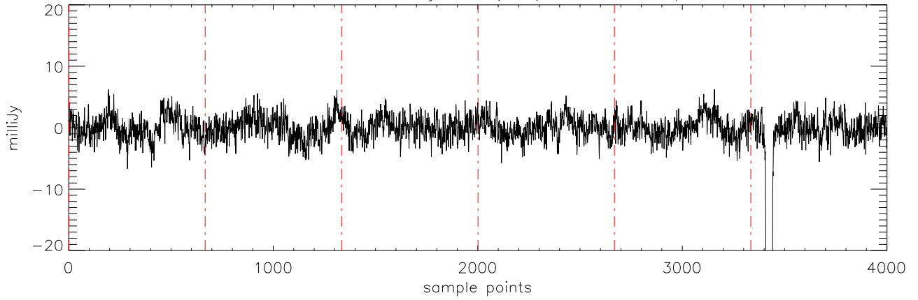
a2471 J09373487 03jan11 (AST) StokesQ freq:5176.
