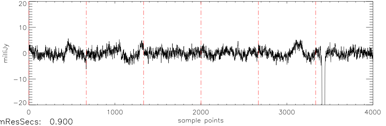
a2471 J09373487 03jan11 (AST) StokesQ freq:5034.
