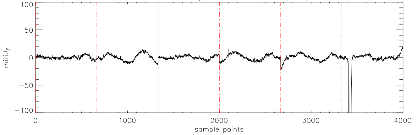
a2471 J09373487 03jan11 (AST) StokesI freq:5176.
