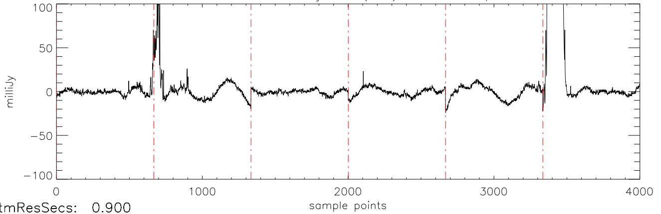
a2471 J09373487 03jan11 (AST) StokesI freq:4466.
