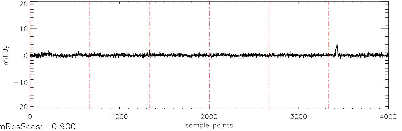
a2471 J09373487 03jan11 (AST) StokesV freq:5034.
