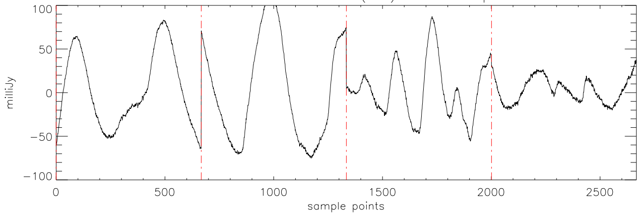
α2471 J09121469 09feb12 (AST) StokesI freq:4608.
