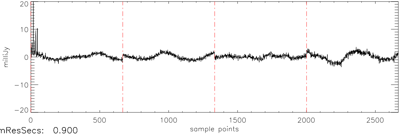
a2471 J09121469 09feb12 (AST) StokesU freq:4466.
