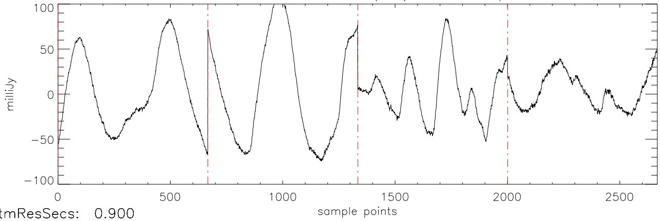
α2471 J09121469 09feb12 (AST) StokesI freq:5034.
