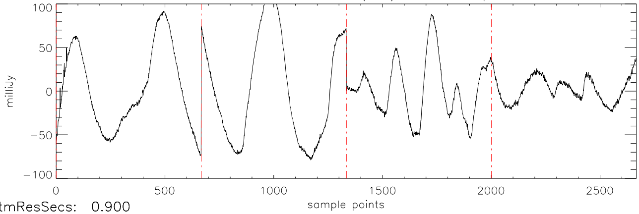
α2471 J09121469 09feb12 (AST) StokesI freq:4466.
