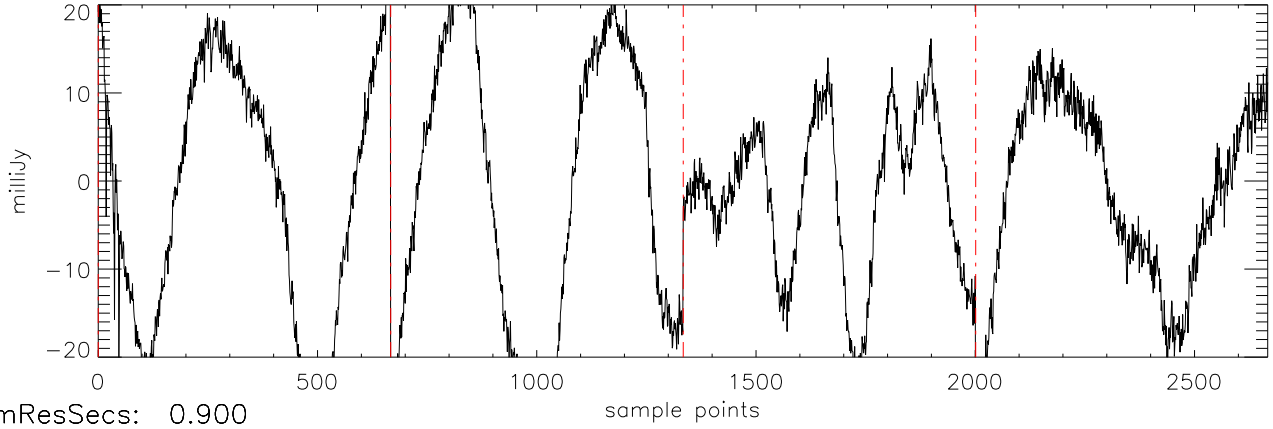
a2471 J09121469 09feb12 (AST) StokesQ freq:4466.
