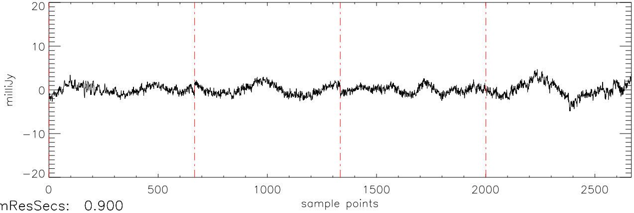
a2471 J09121469 09feb12 (AST) StokesU freq:5034.
