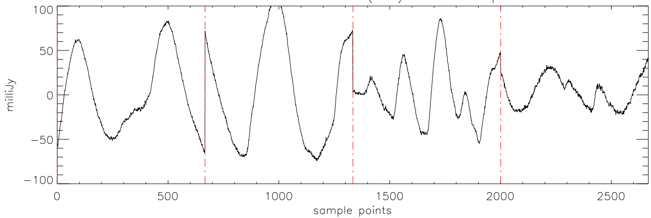
α2471 J09121469 09feb12 (AST) StokesI freq:4750.
