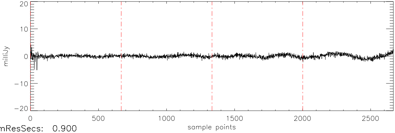
a2471 J09121469 09feb12 (AST) StokesV freq:4466.
