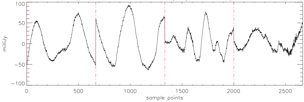
α2471 J09121469 09feb12 (AST) StokesI freq:5176.
