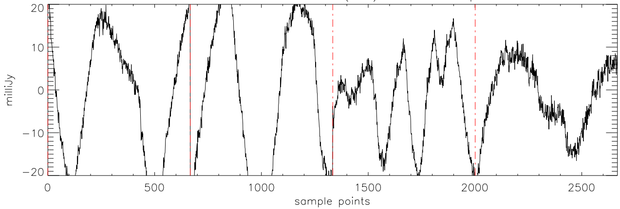
a2471 J09121469 09feb12 (AST) StokesQ freq:4608.
