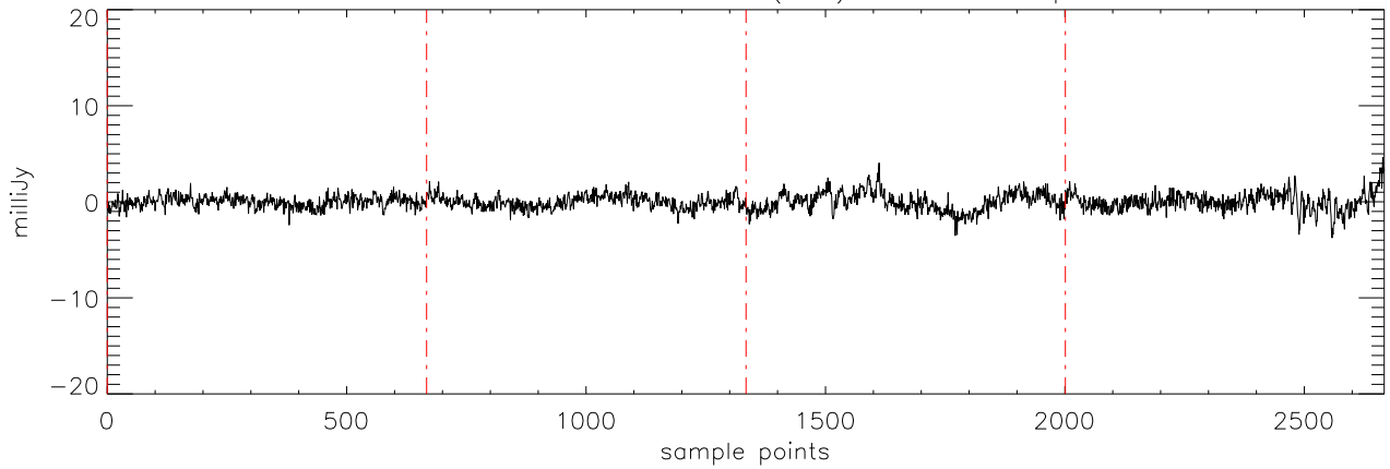
a2471 J09121469 09feb12 (AST) StokesU freq:5176.
