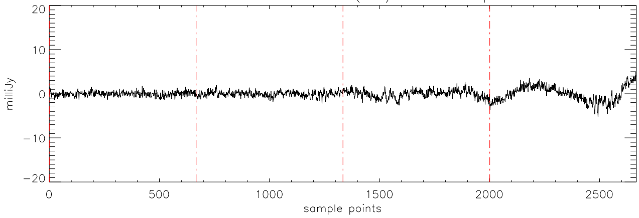
a2471 J09121469 09feb12 (AST) StokesV freq:5176.
