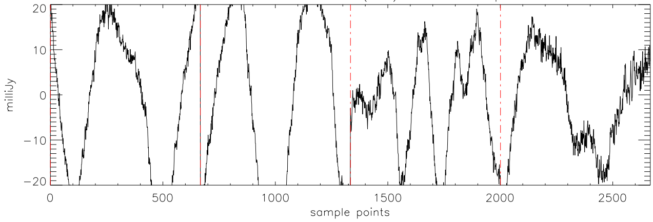
a2471 J09121469 09feb12 (AST) StokesQ freq:5176.
