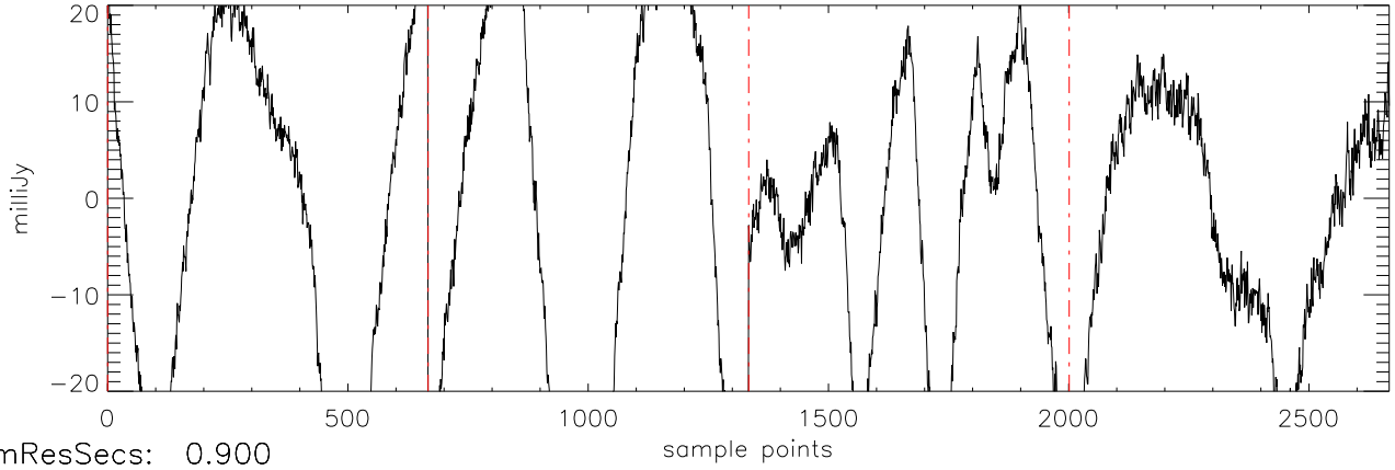
a2471 J09121469 09feb12 (AST) StokesQ freq:5034.
