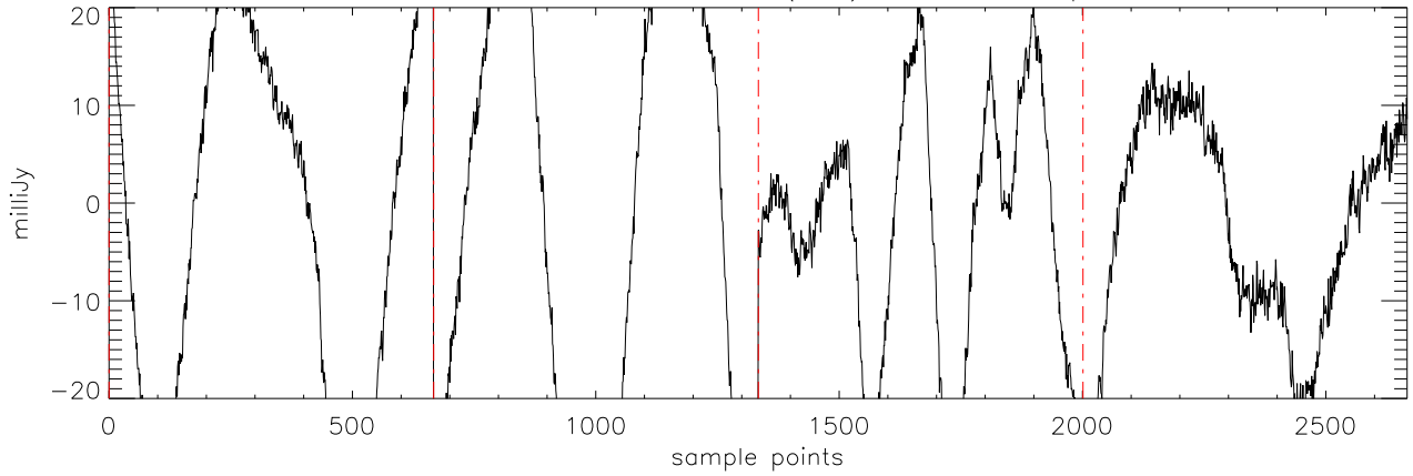
a2471 J09121469 09feb12 (AST) StokesQ freq:4750.
