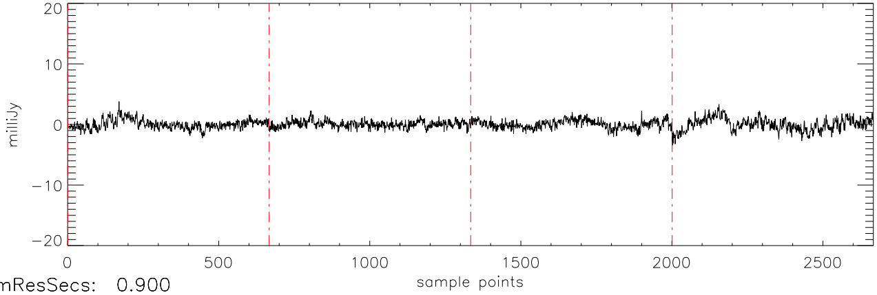
a2471 J09121469 09feb12 (AST) StokesV freq:5034.
