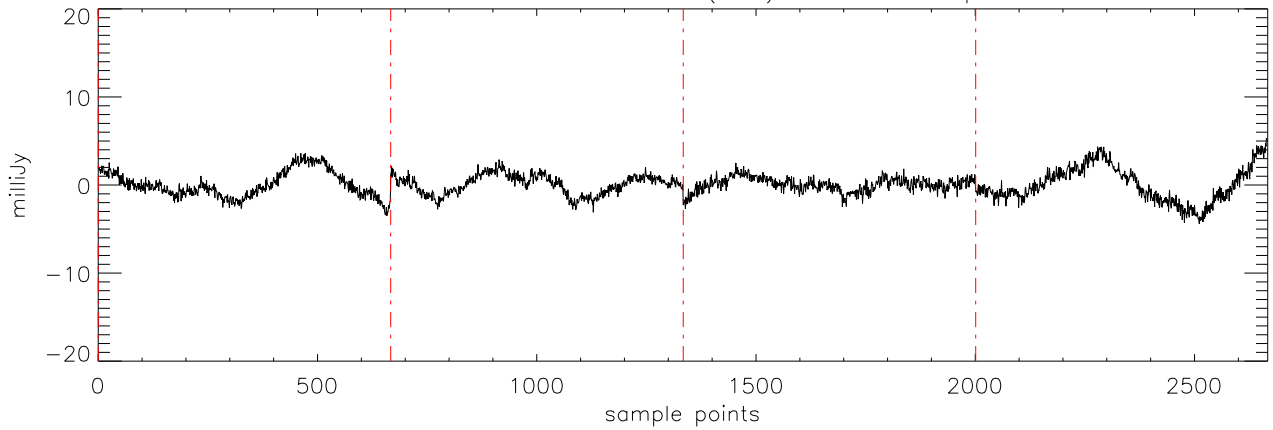
a2471 J09121469 09feb12 (AST) StokesU freq:4608.
