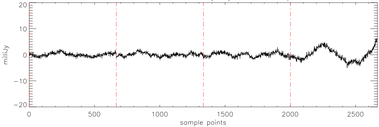
a2471 J09121469 09feb12 (AST) StokesU freq:4750.
