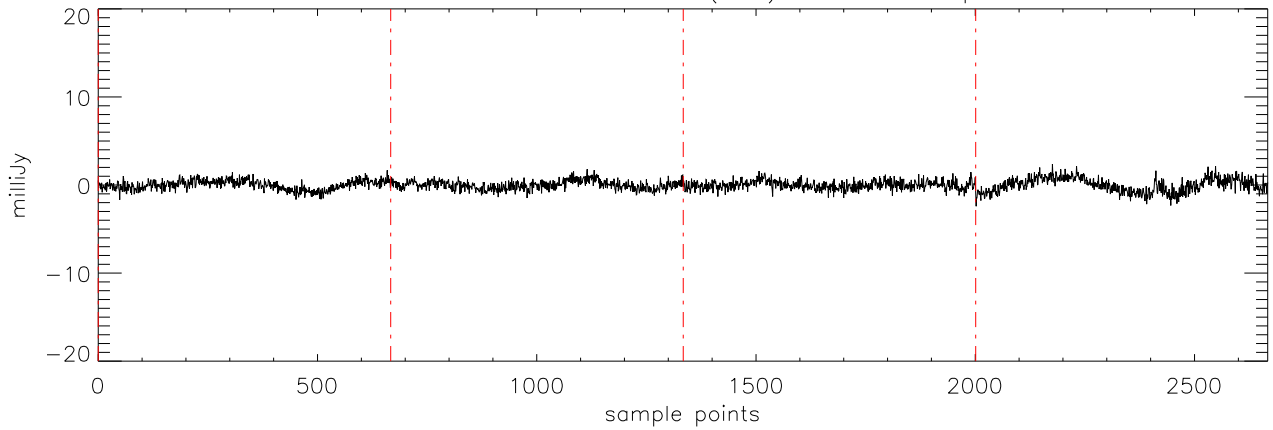
a2471 J09121469 09feb12 (AST) StokesV freq:4608.
