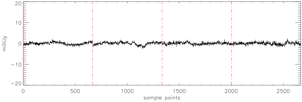
a2471 J09121469 09feb12 (AST) StokesV freq:4750.
