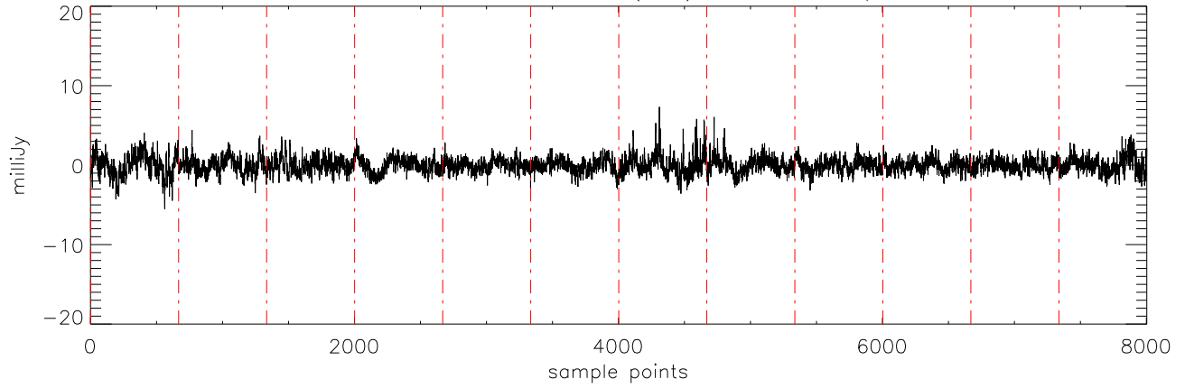
a2471 J0850359 09feb12 (AST) StokesU freq:5176.
