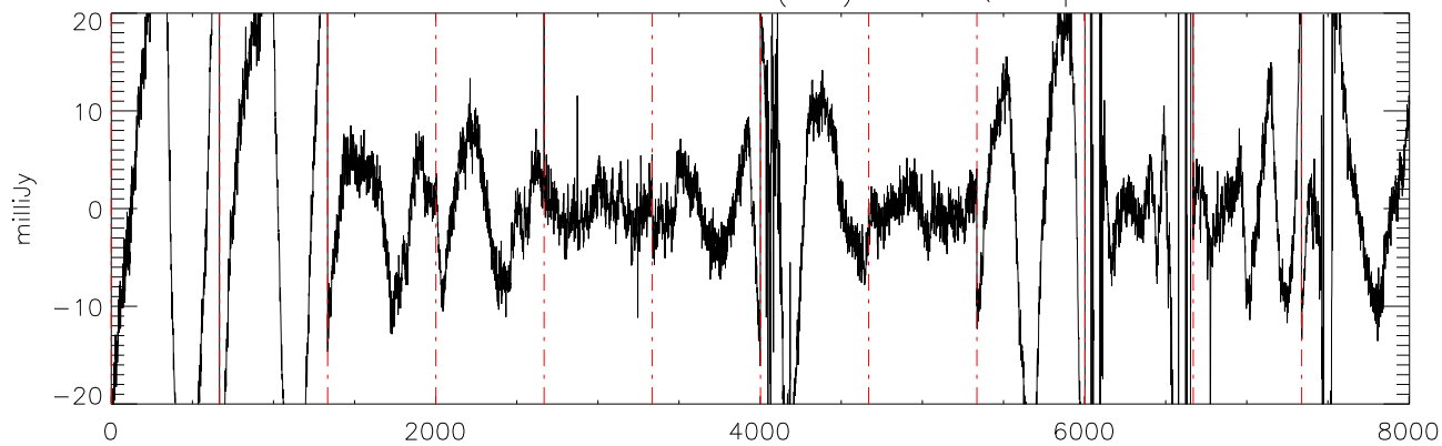
a2471 J0850359 09feb12 (AST) StokesQ freq:4325.
