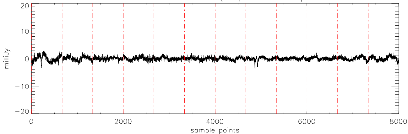
a2471 J0850359 09feb12 (AST) StokesU freq:4608.
