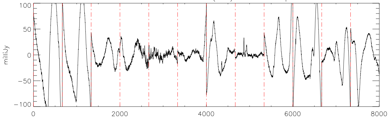
a2471 J0850359 09feb12 (AST) StokesI freq:4608.
