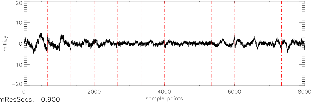
a2471 J0850359 09feb12 (AST) StokesU freq:5034.
