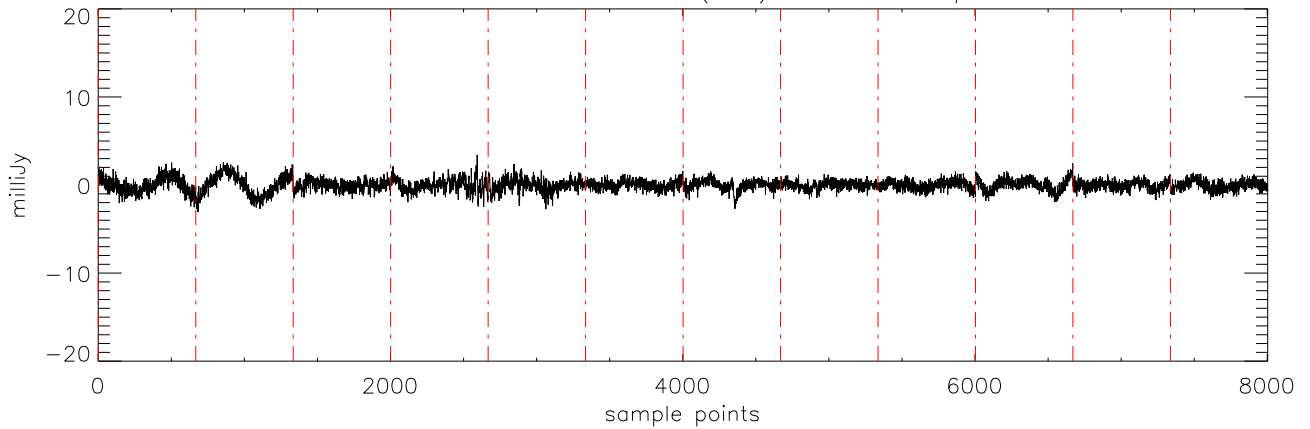
a2471 J0850359 09feb12 (AST) StokesV freq:4750.
