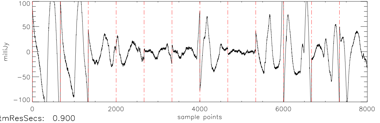
a2471 J0850359 09feb12 (AST) StokesI freq:5034.
