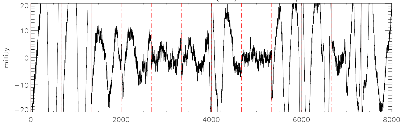
a2471 J0850359 09feb12 (AST) StokesQ freq:4608.
