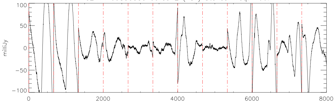
a2471 J0850359 09feb12 (AST) StokesI freq:4466.
