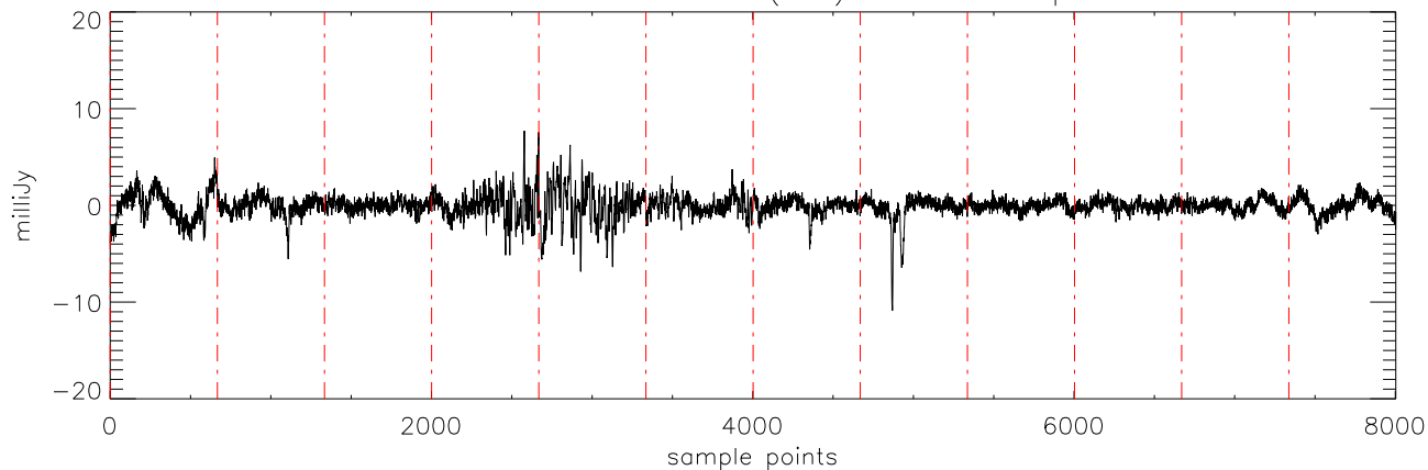
a2471 J0850359 09feb12 (AST) StokesU freq:4750.
