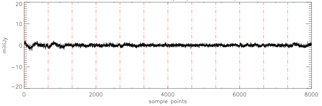
a2471 J0850359 09feb12 (AST) StokesV freq:4608.
