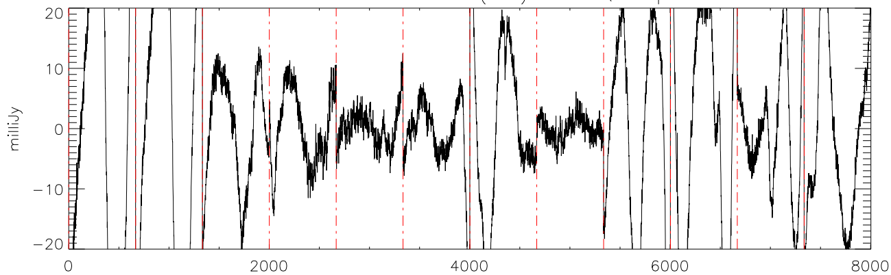
a2471 J0850359 09feb12 (AST) StokesQ freq:4750.
