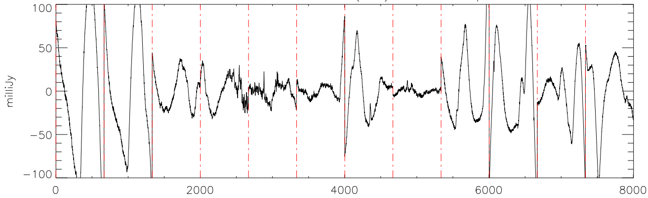
a2471 J0850359 09feb12 (AST) StokesI freq:4750.
