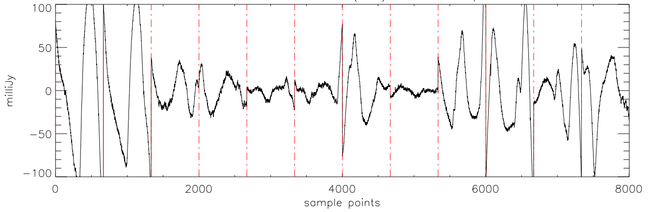
a2471 J0850359 09feb12 (AST) StokesI freq:5176.
