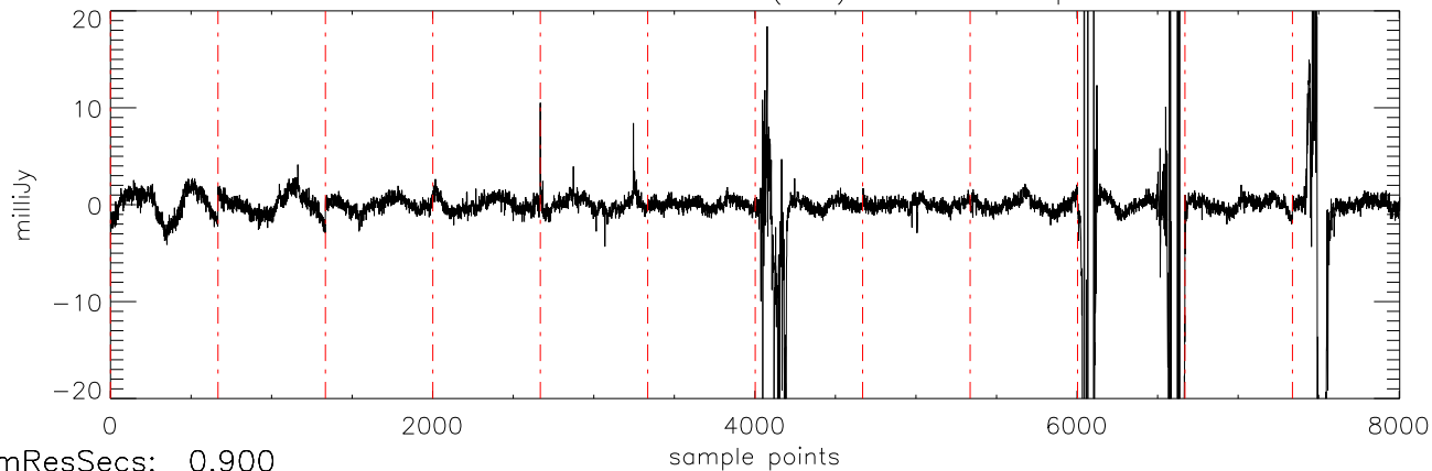
a2471 J0850359 09feb12 (AST) StokesU freq:4466.
