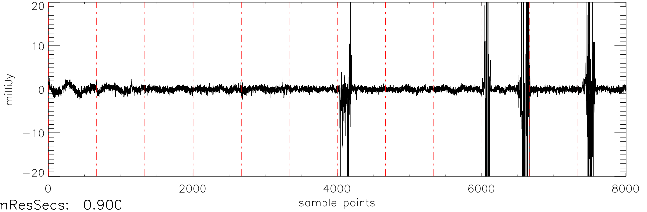
a2471 J0850359 09feb12 (AST) StokesV freq:4466.
