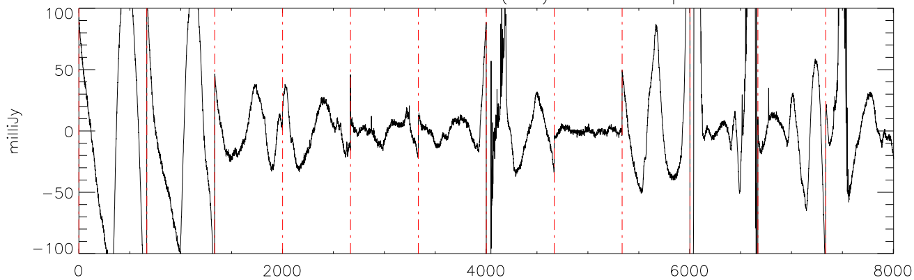
a2471 J0850359 09feb12 (AST) StokesI freq:4325.
