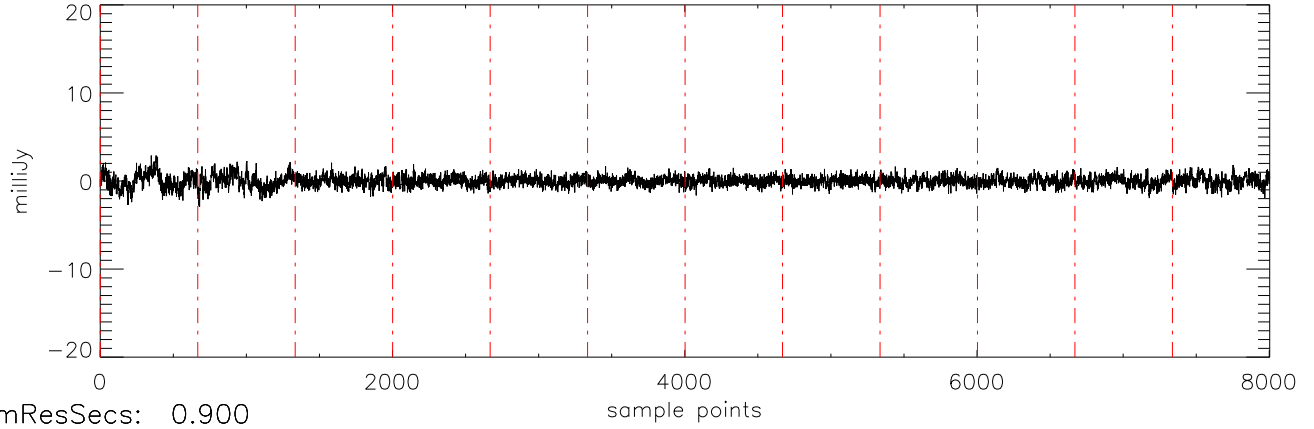
a2471 J0850359 09feb12 (AST) StokesV freq:5034.
