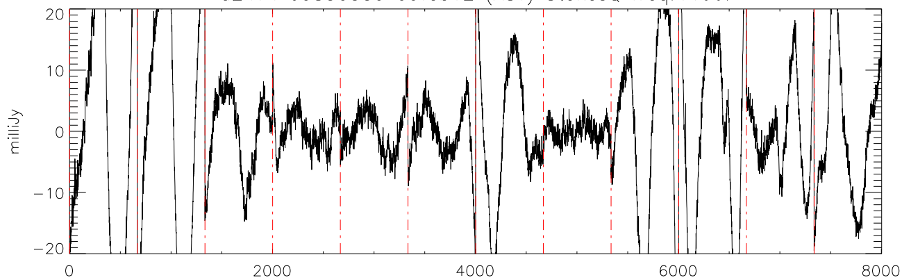
a2471 J0850359 09feb12 (AST) StokesQ freq:4466.
