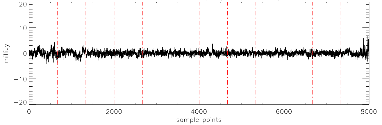
a2471 J0850359 09feb12 (AST) StokesV freq:5176.
