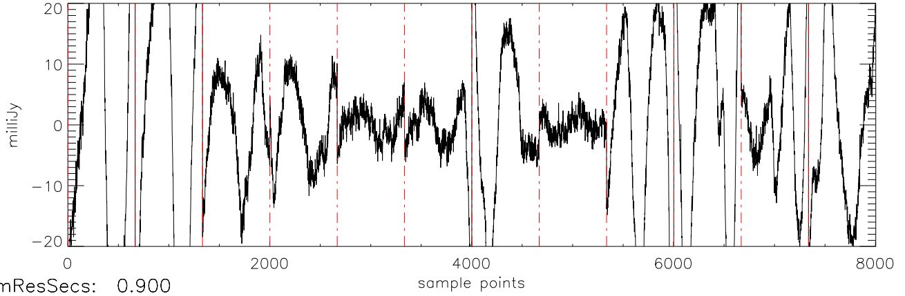
a2471 J0850359 09feb12 (AST) StokesQ freq:5034.
