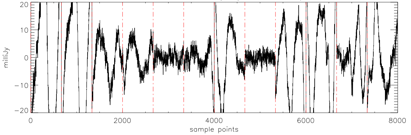
a2471 J0850359 09feb12 (AST) StokesQ freq:5176.
