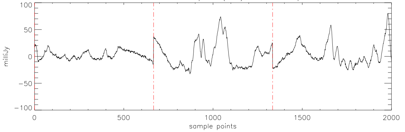
a2471 J07464256 05apr12 (AST) StokesI freq:5176.
