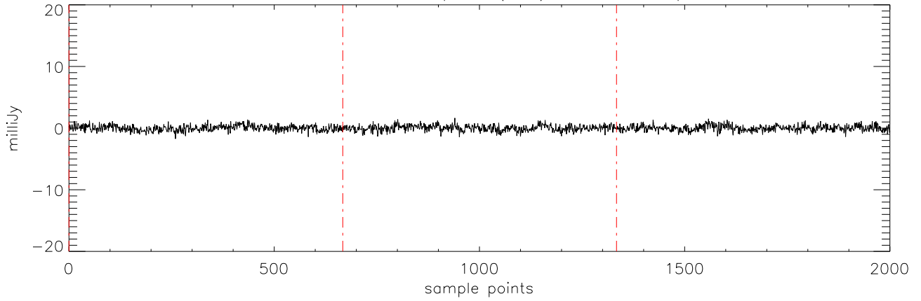
a2471 J07464256 05apr12 (AST) StokesV freq:4750.
