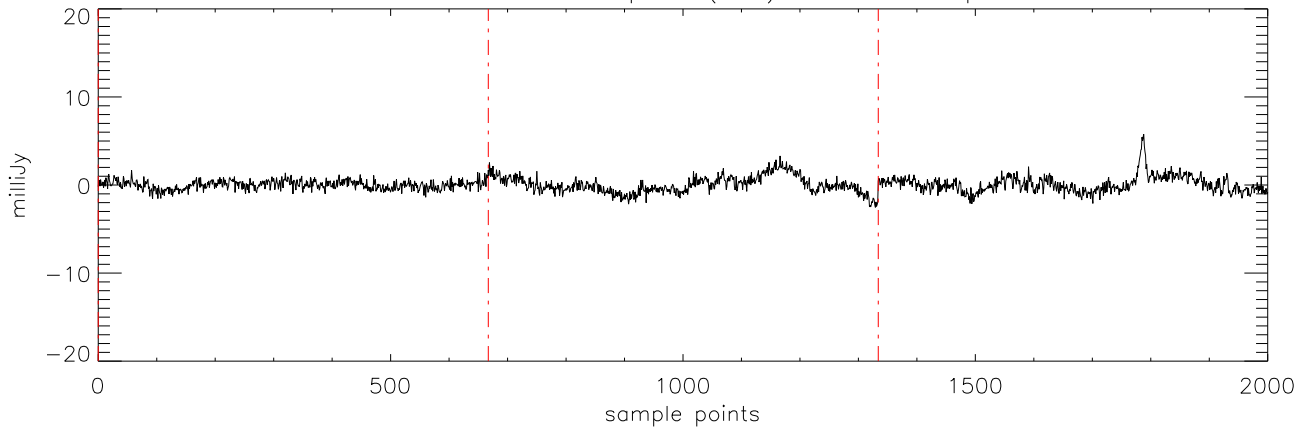
a2471 J07464256 05apr12 (AST) StokesU freq:4608.
