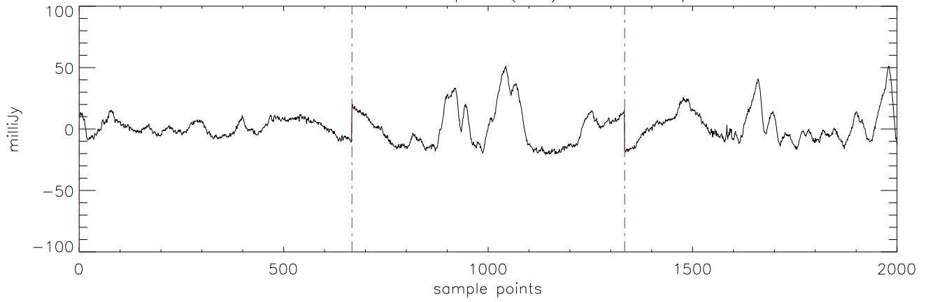
a2471 J07464256 05apr12 (AST) StokesI freq:4608.
