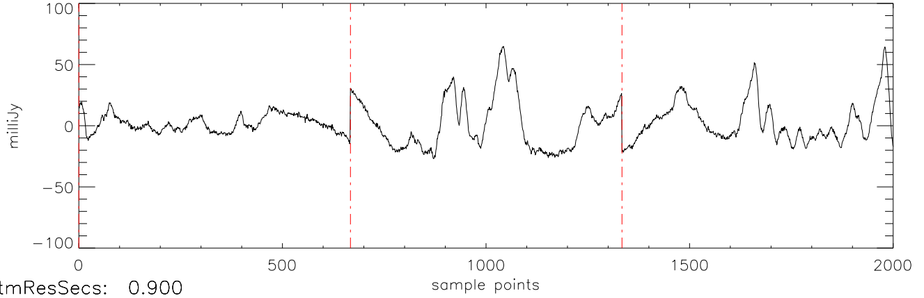
a2471 J07464256 05apr12 (AST) StokesI freq:5034.
