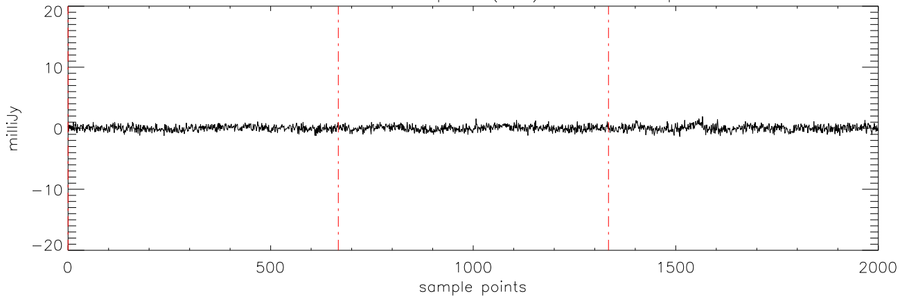
a2471 J07464256 05apr12 (AST) StokesV freq:4608.
