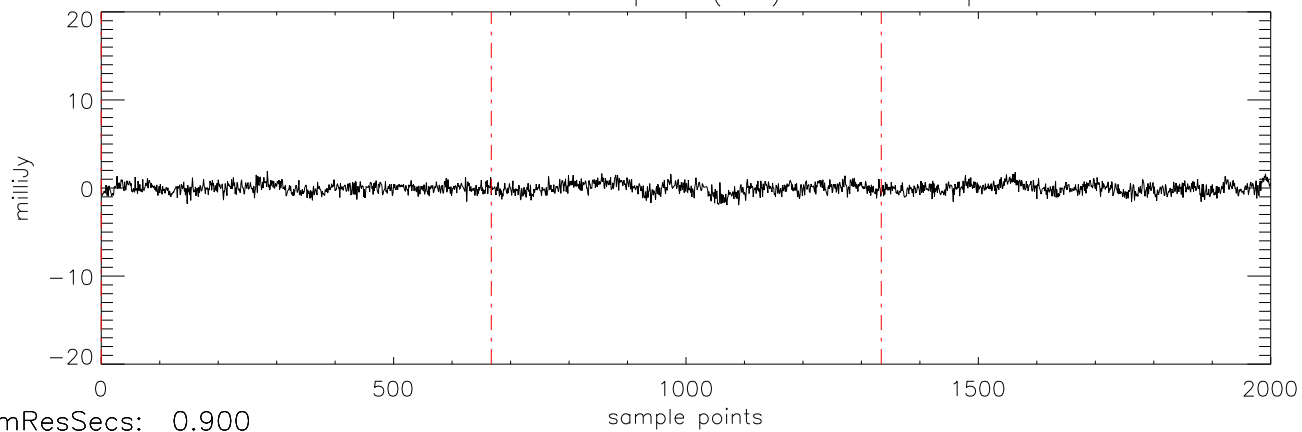
a2471 J07464256 05apr12 (AST) StokesV freq:5034.
