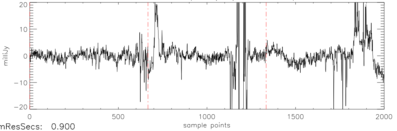
a2471 J07464256 05apr12 (AST) StokesQ freq:4466.
