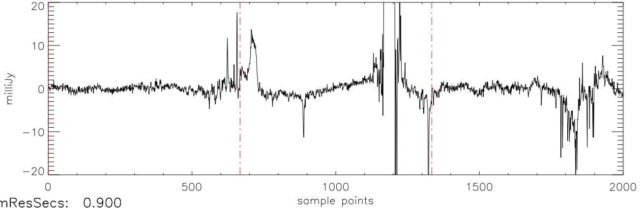
a2471 J07464256 05apr12 (AST) StokesU freq:4466.
