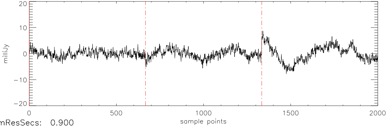
a2471 J07464256 05apr12 (AST) StokesQ freq:5034.
