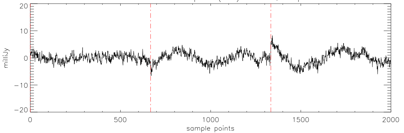
a2471 J07464256 05apr12 (AST) StokesQ freq:4750.
