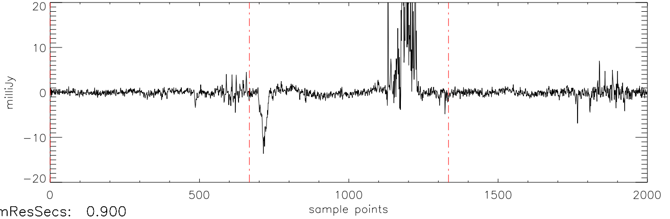
a2471 J07464256 05apr12 (AST) StokesV freq:4466.
