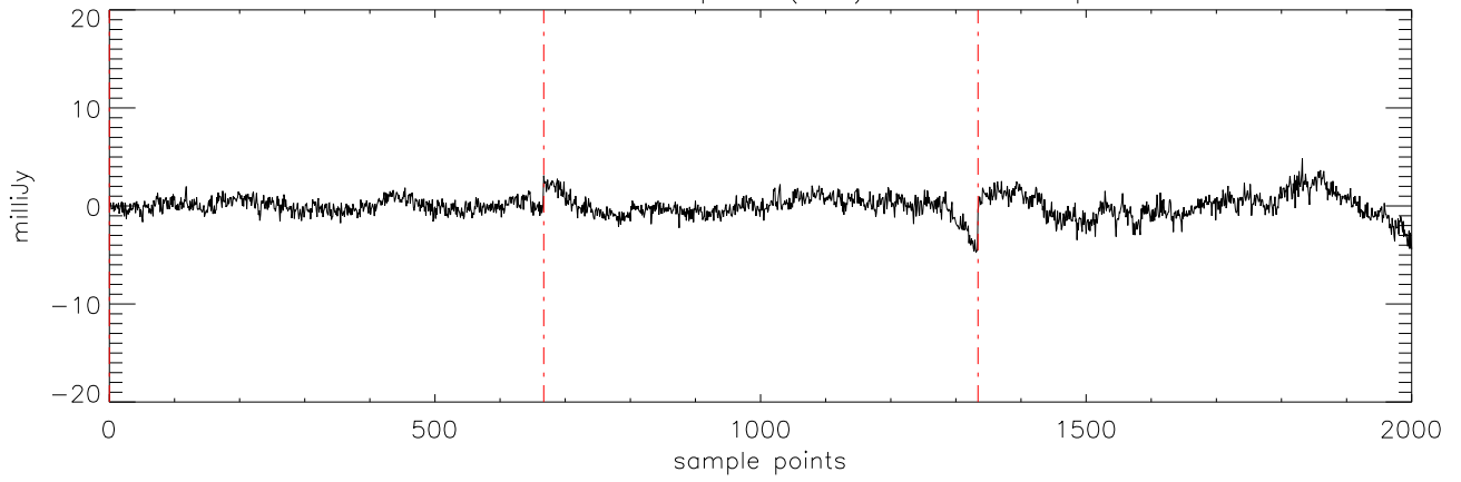
a2471 J07464256 05apr12 (AST) StokesU freq:5176.
