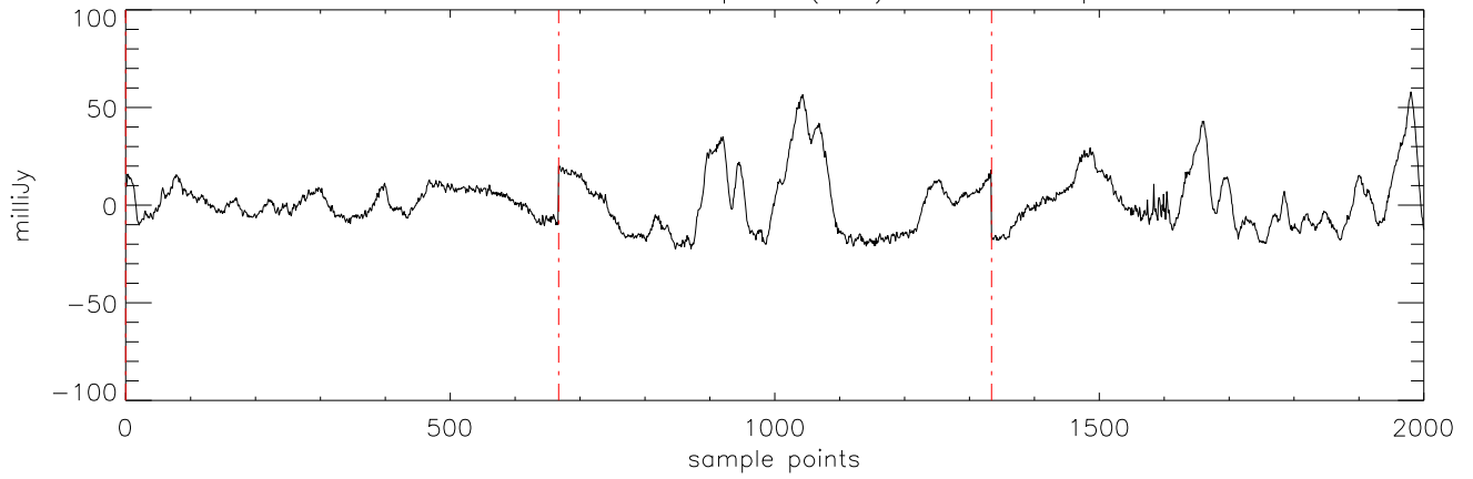
a2471 J07464256 05apr12 (AST) StokesI freq:4750.
