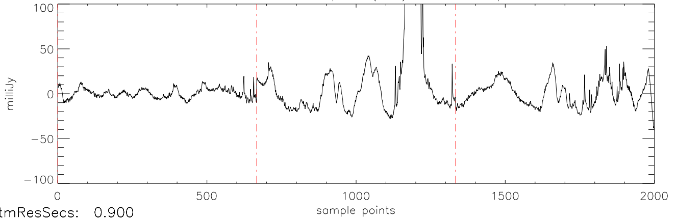
a2471 J07464256 05apr12 (AST) StokesI freq:4466.
