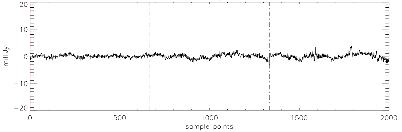
a2471 J07464256 05apr12 (AST) StokesU freq:4750.
