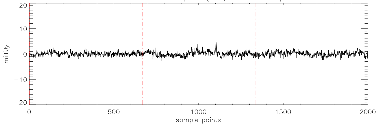
a2471 J07464256 05apr12 (AST) StokesV freq:5176.
