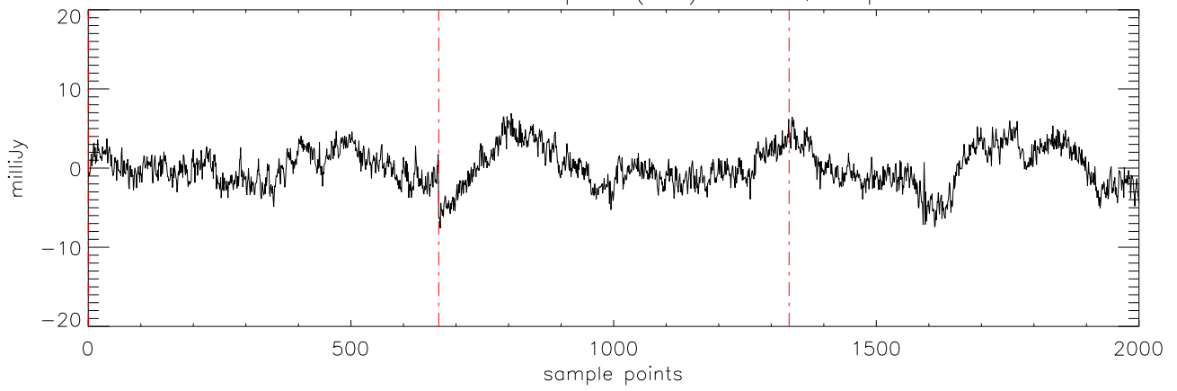
a2471 J07464256 05apr12 (AST) StokesQ freq:4608.
