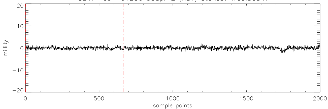
a2471 J07464256 05apr12 (AST) StokesV freq:5176.
