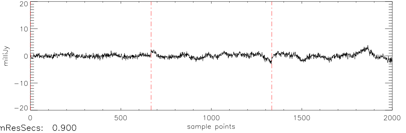
a2471 J07464256 05apr12 (AST) StokesU freq:5034.
