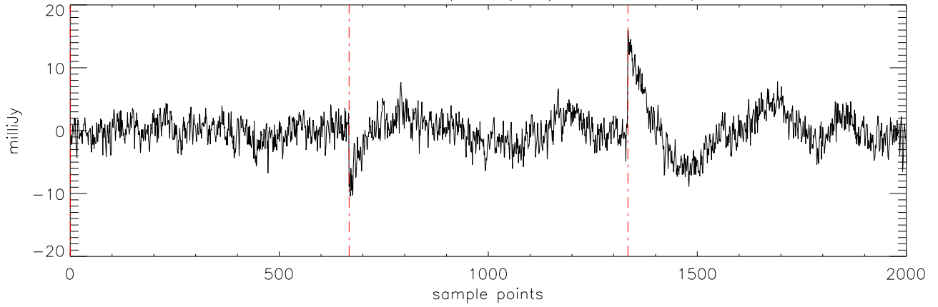
a2471 J07464256 05apr12 (AST) StokesQ freq:5176.
