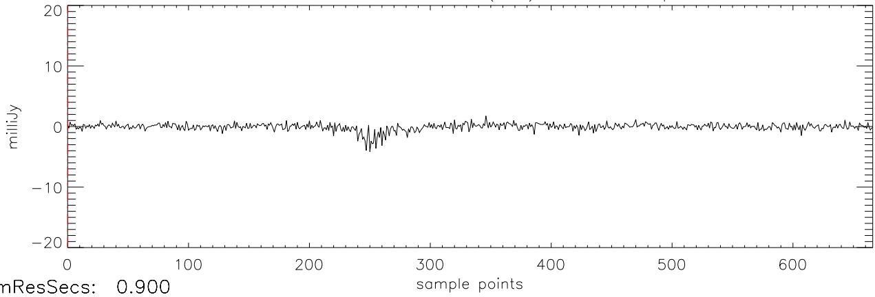
a2471 J03284265 27oct11 (AST) StokesV freq:4466.
