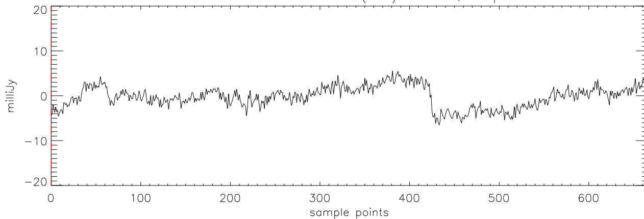
a2471 J03284265 27oct11 (AST) StokesQ freq:4750.
