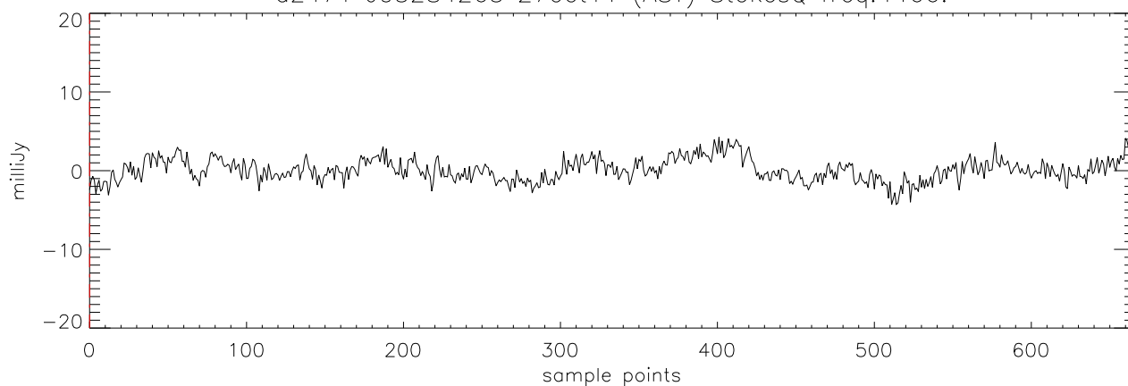
a2471 J03284265 27oct11 (AST) StokesQ freq:4608.
