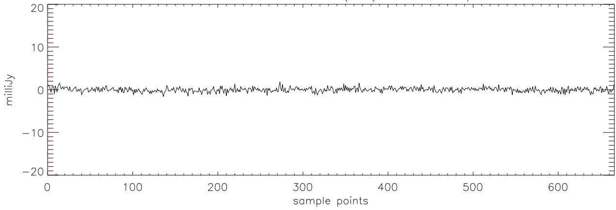
a2471 J03284265 27oct11 (AST) StokesV freq:5176.
