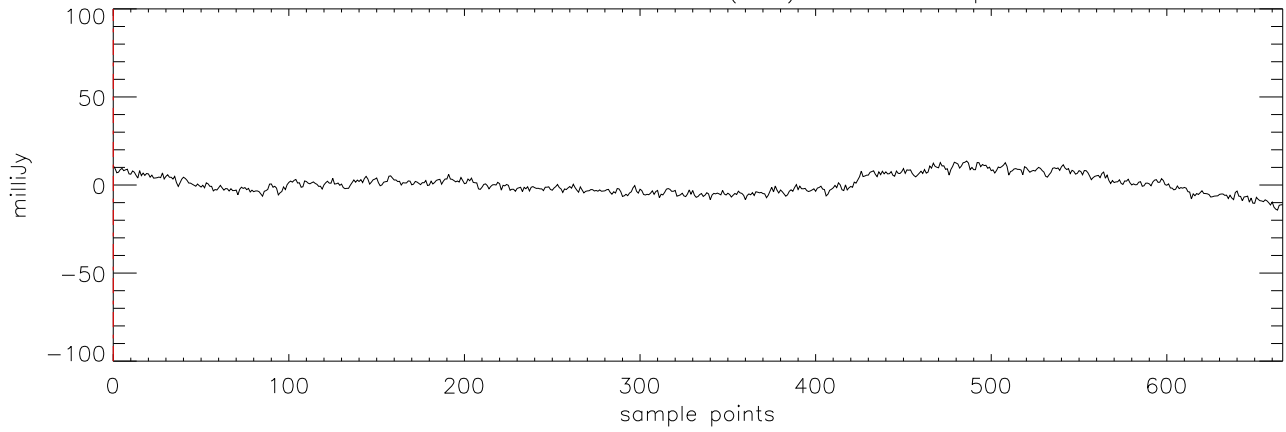
a2471 J03284265 27oct11 (AST) StokesI freq:5176.
