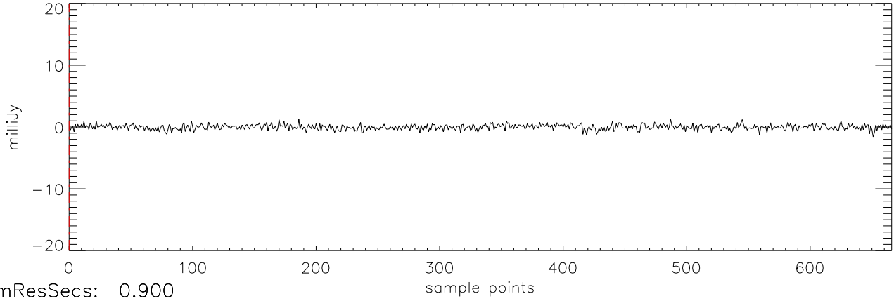
a2471 J03284265 27oct11 (AST) StokesV freq:5034.
