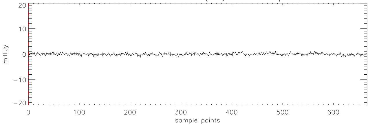
a2471 J03284265 27oct11 (AST) StokesV freq:4750.
