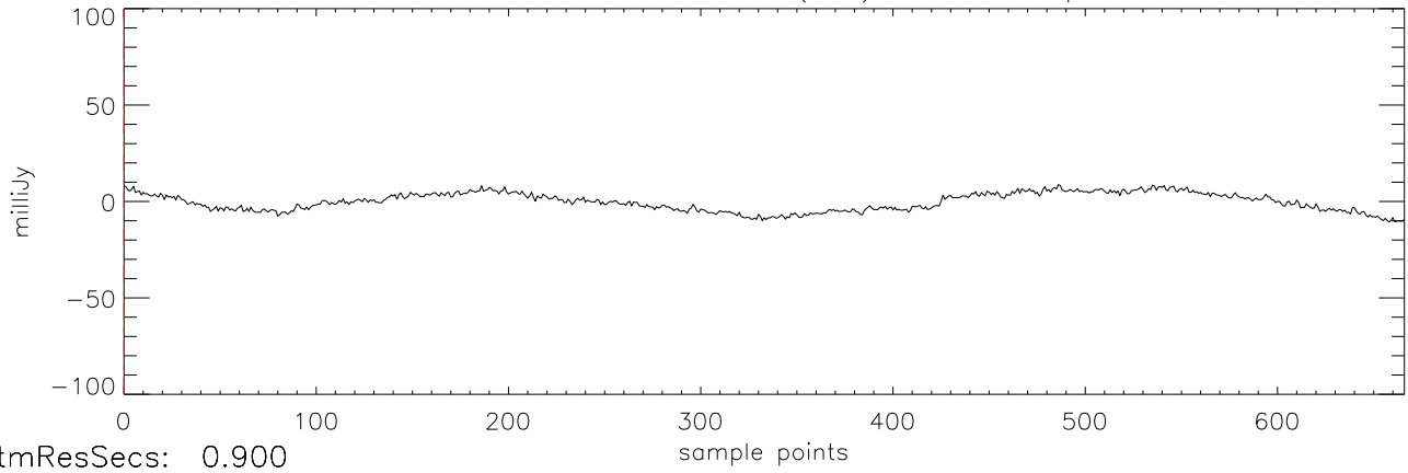
a2471 J03284265 27oct11 (AST) StokesI freq:5034.
