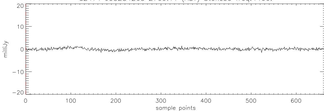
a2471 J03284265 27oct11 (AST) StokesU freq:4608.
