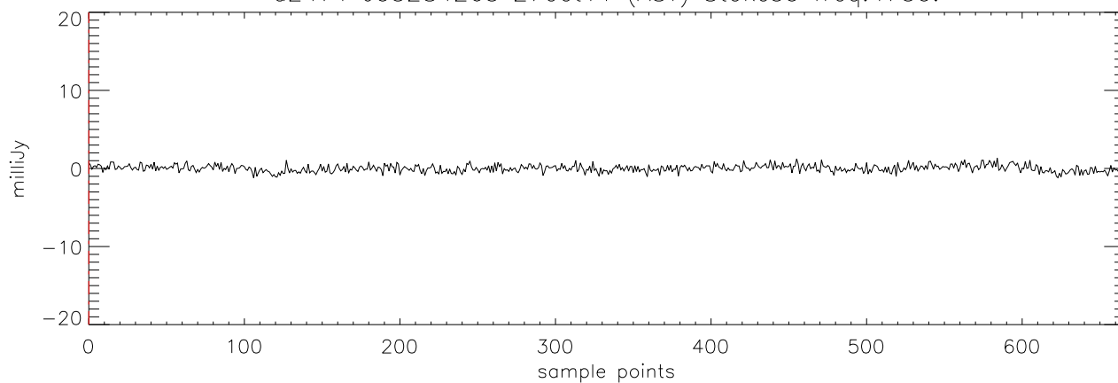
a2471 J03284265 27oct11 (AST) StokesU freq:4750.
