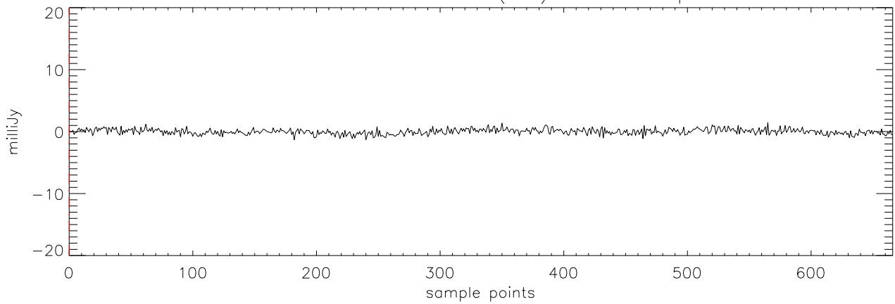
a2471 J03284265 27oct11 (AST) StokesV freq:4608.
