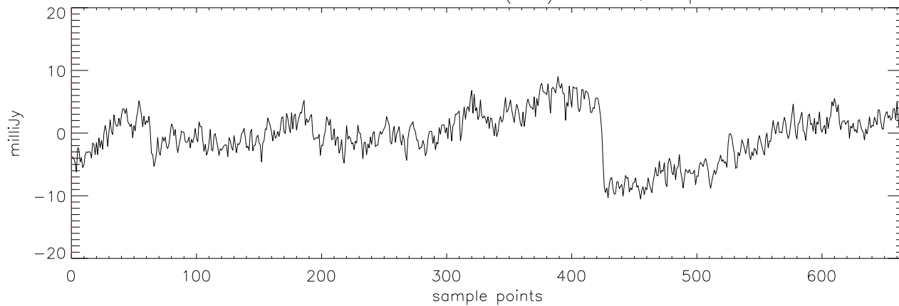
a2471 J03284265 27oct11 (AST) StokesQ freq:5176.
