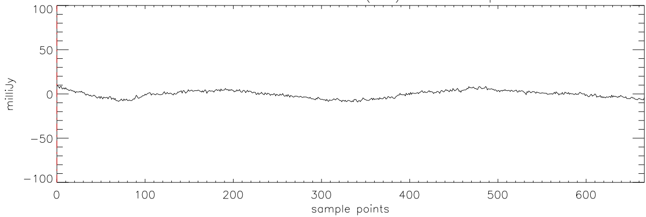
a2471 J03284265 27oct11 (AST) StokesI freq:4608.
