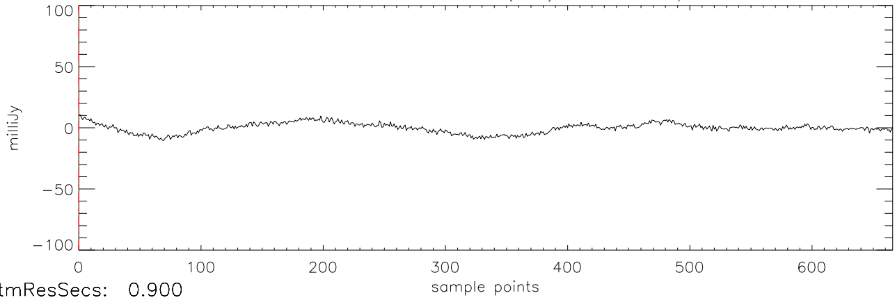
a2471 J03284265 27oct11 (AST) StokesI freq:4466.
