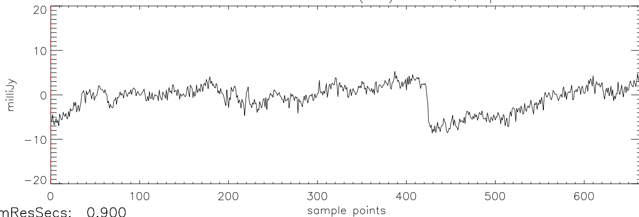
a2471 J03284265 27oct11 (AST) StokesQ freq:5034.
