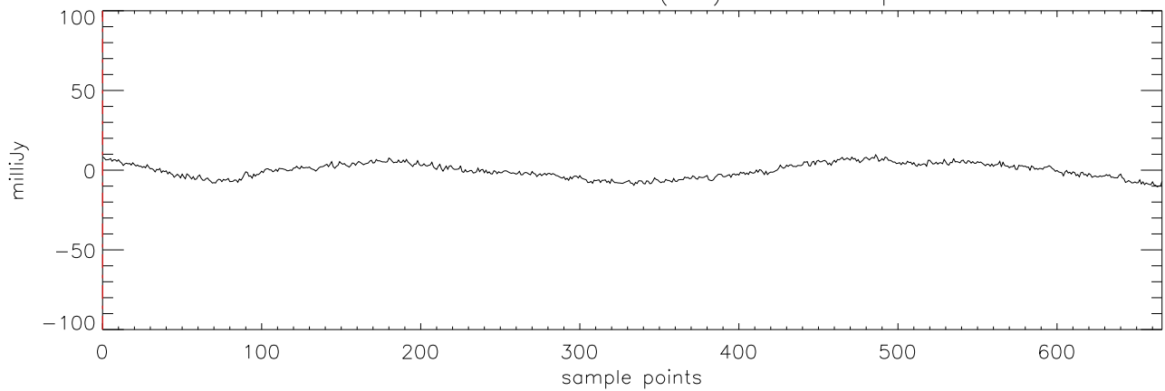
a2471 J03284265 27oct11 (AST) StokesI freq:4750.
