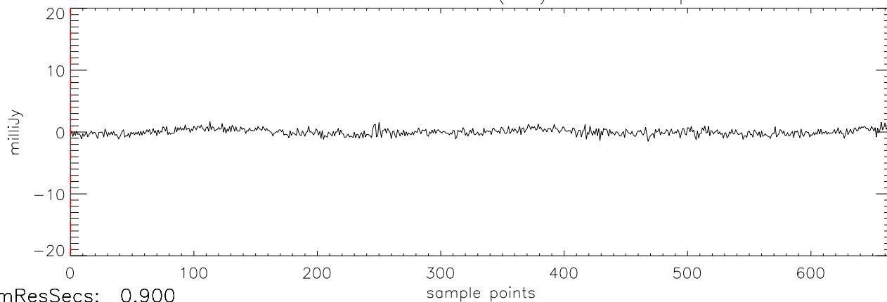
a2471 J03284265 27oct11 (AST) StokesU freq:4466.
