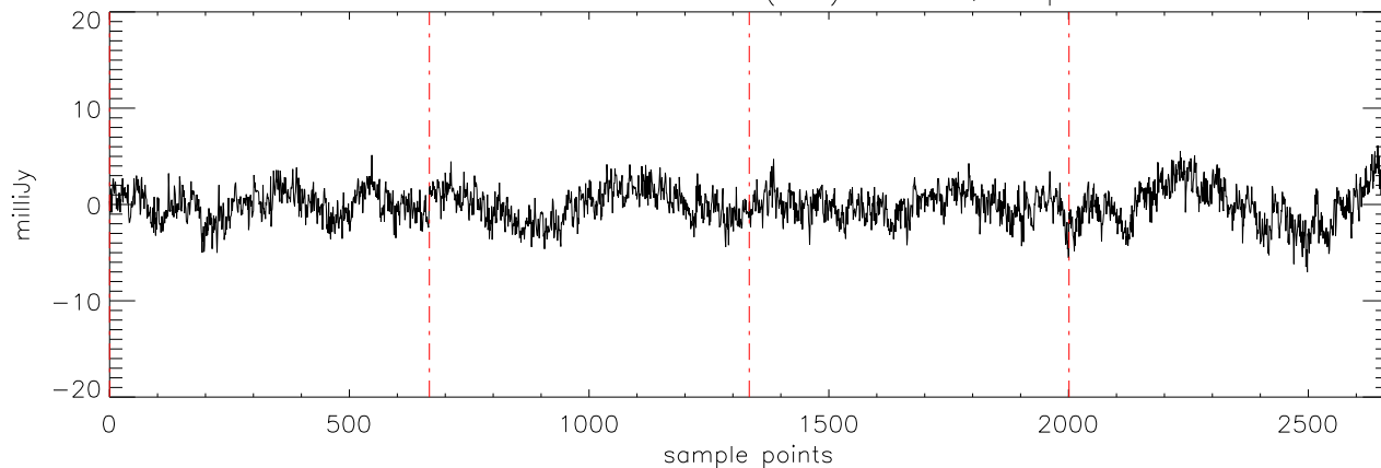
a2471 J0326137 22oct11 (AST) StokesQ freq:5176.
