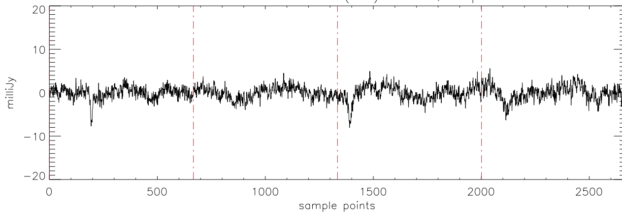
a2471 J0326137 22oct11 (AST) StokesQ freq:4750.
