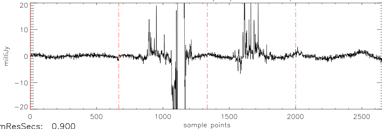
a2471 J0326137 22oct11 (AST) StokesU freq:4466.
