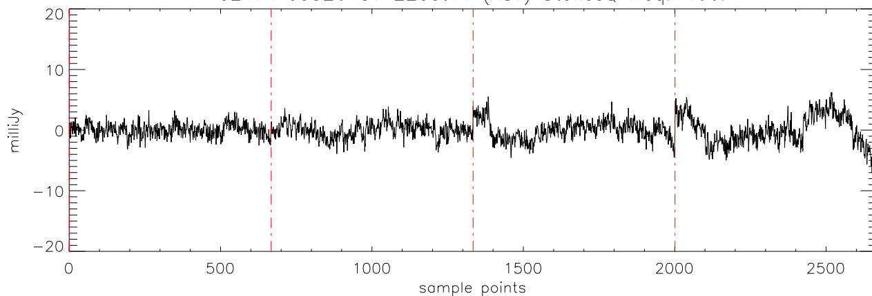
a2471 J0326137 22oct11 (AST) StokesQ freq:4608.
