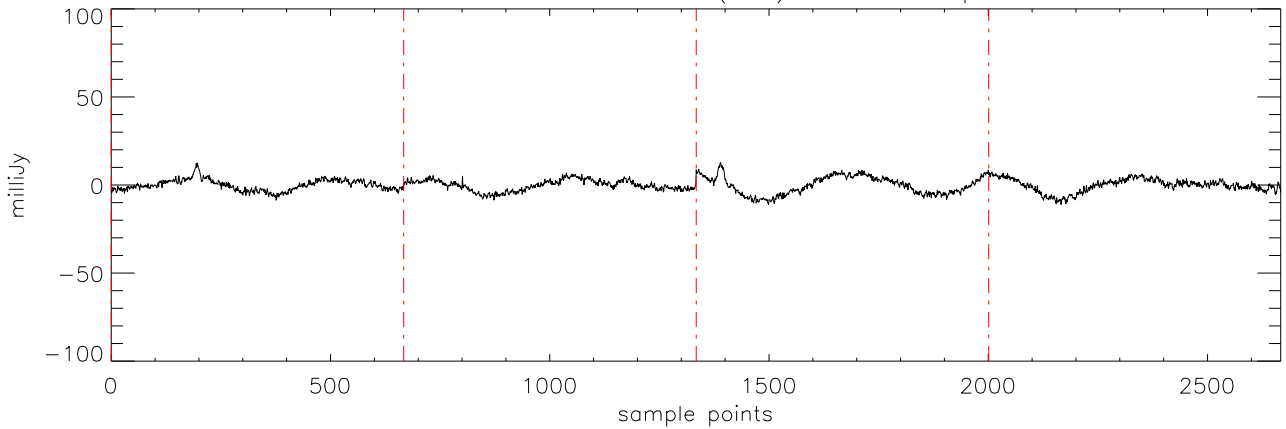
a2471 J0326137 22oct11 (AST) StokesI freq:4750.
