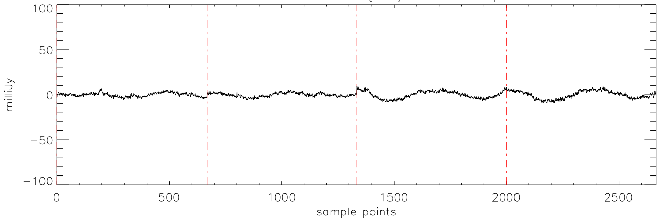
a2471 J0326137 22oct11 (AST) StokesI freq:4608.
