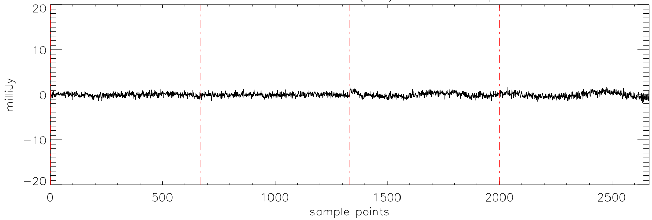
a2471 J0326137 22oct11 (AST) StokesV freq:4608.
