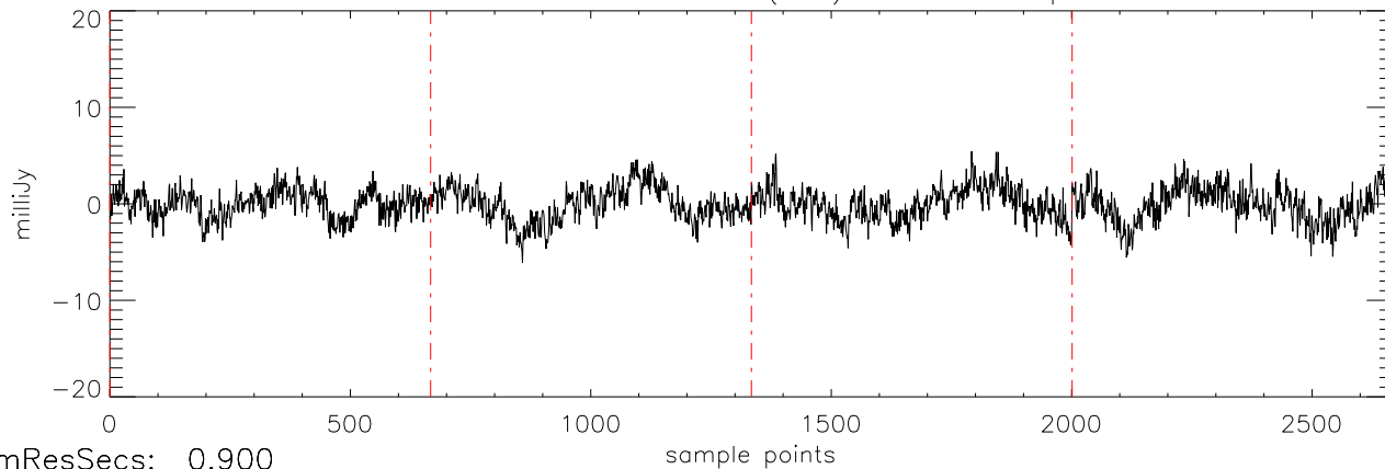
a2471 J0326137 22oct11 (AST) StokesQ freq:5034.
