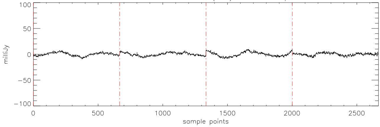
a2471 J0326137 22oct11 (AST) StokesI freq:5176.
