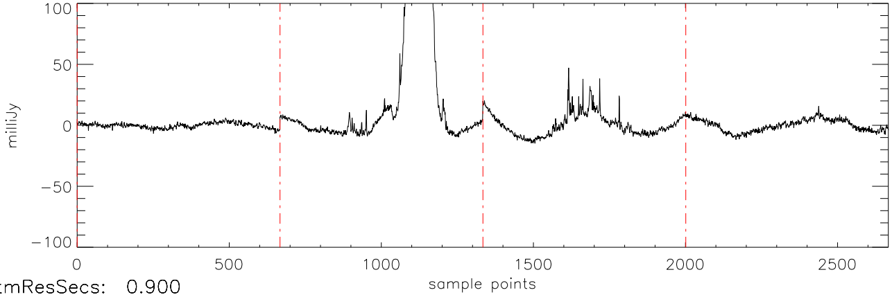
a2471 J0326137 22oct11 (AST) StokesI freq:4466.
