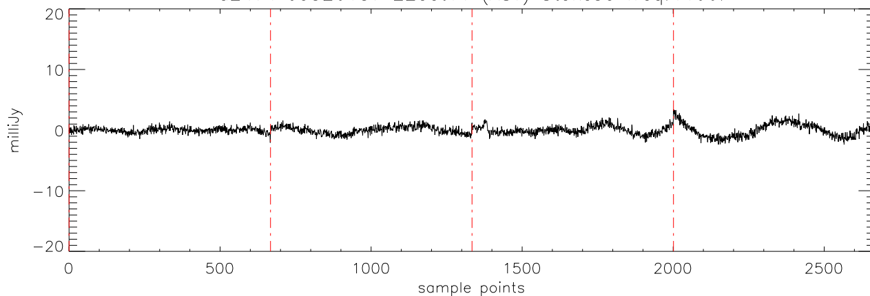
a2471 J0326137 22oct11 (AST) StokesU freq:4608.
