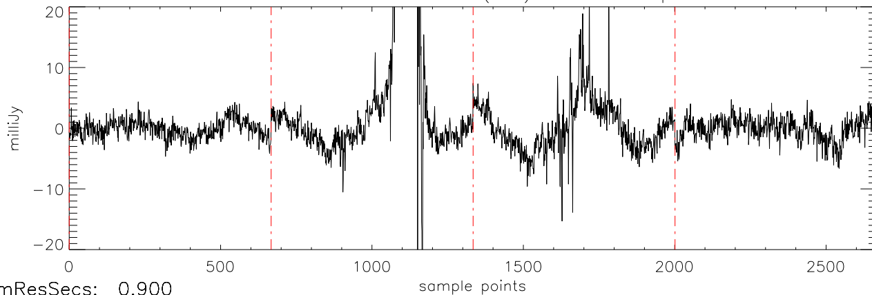
a2471 J0326137 22oct11 (AST) StokesQ freq:4466.
