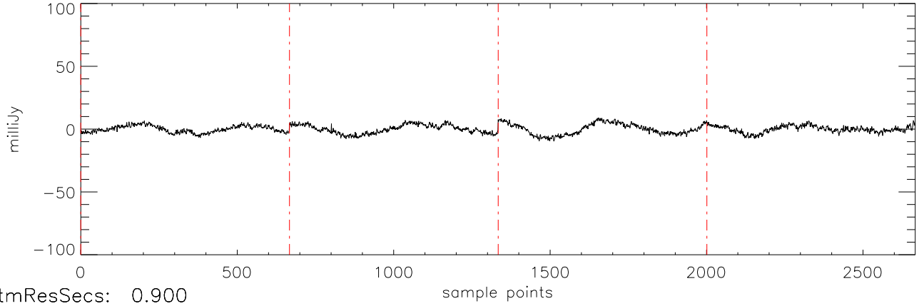
a2471 J0326137 22oct11 (AST) StokesI freq:5034.
