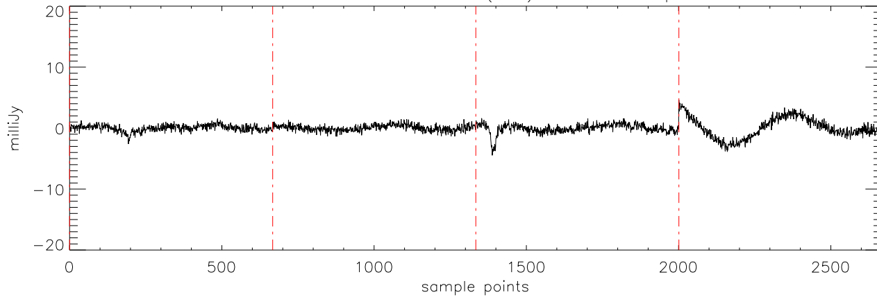
a2471 J0326137 22oct11 (AST) StokesU freq:4750.
