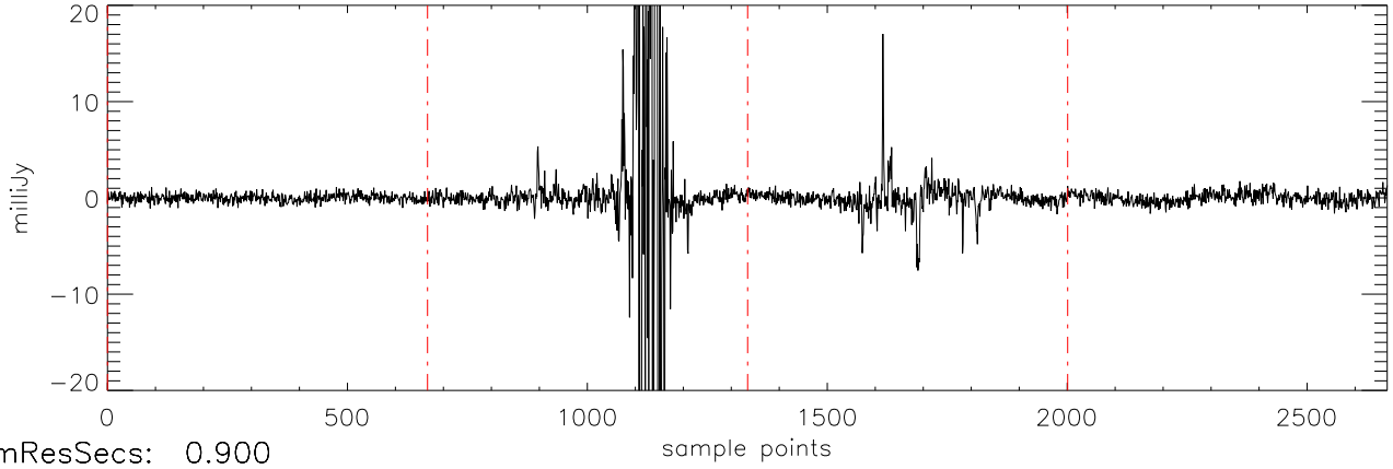
a2471 J0326137 22oct11 (AST) StokesV freq:4466.
