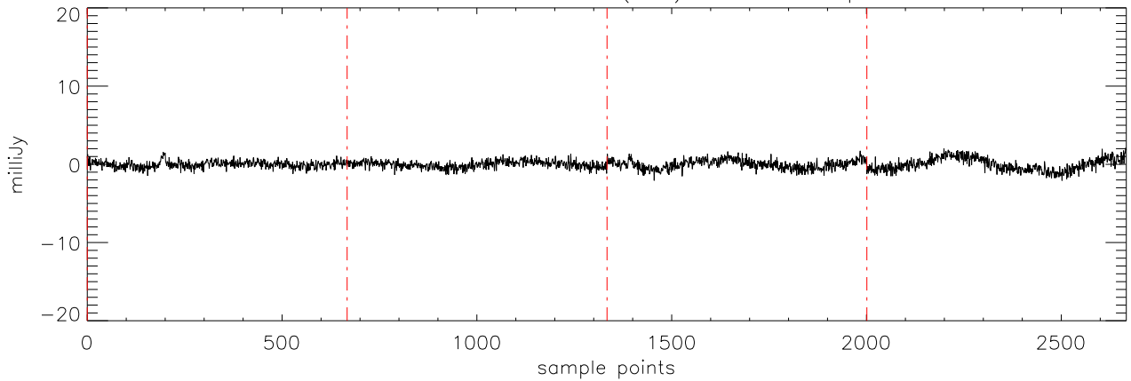
a2471 J0326137 22oct11 (AST) StokesV freq:4750.
