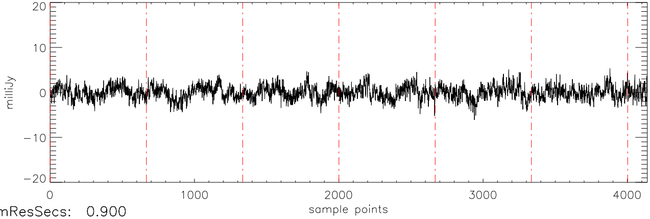
a2471 J00325937 17dec10 (AST) StokesQ freq:5034.
