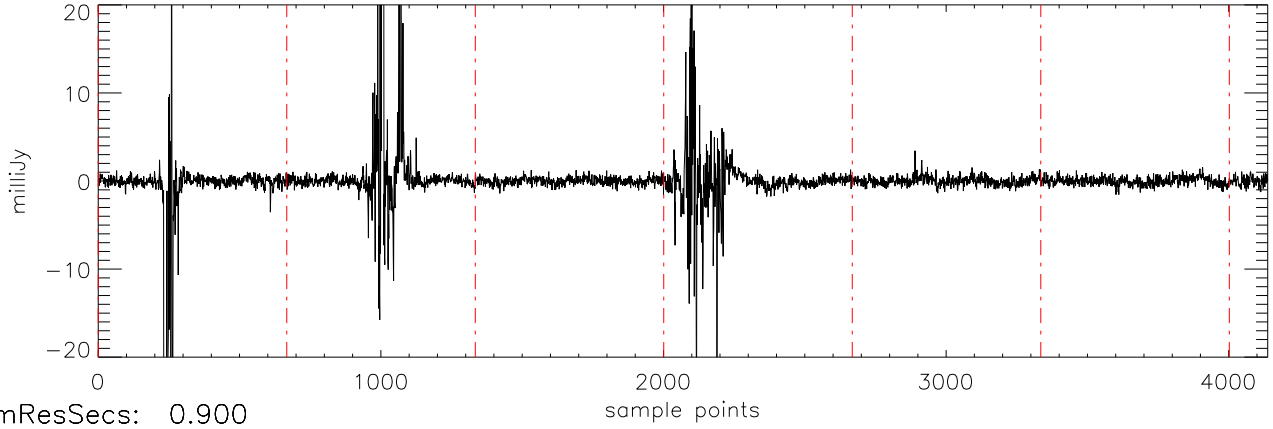
a2471 J00325937 17dec10 (AST) StokesV freq:4466.
