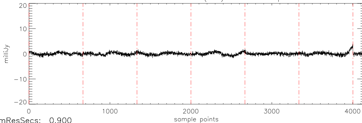
a2471 J00325937 17dec10 (AST) StokesU freq:5034.
