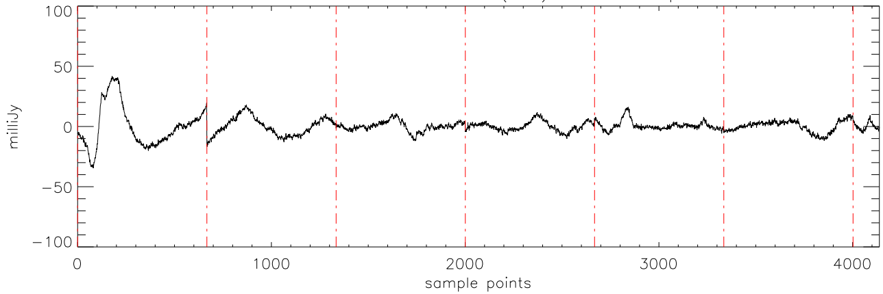
a2471 J00325937 17dec10 (AST) StokesI freq:4608.
