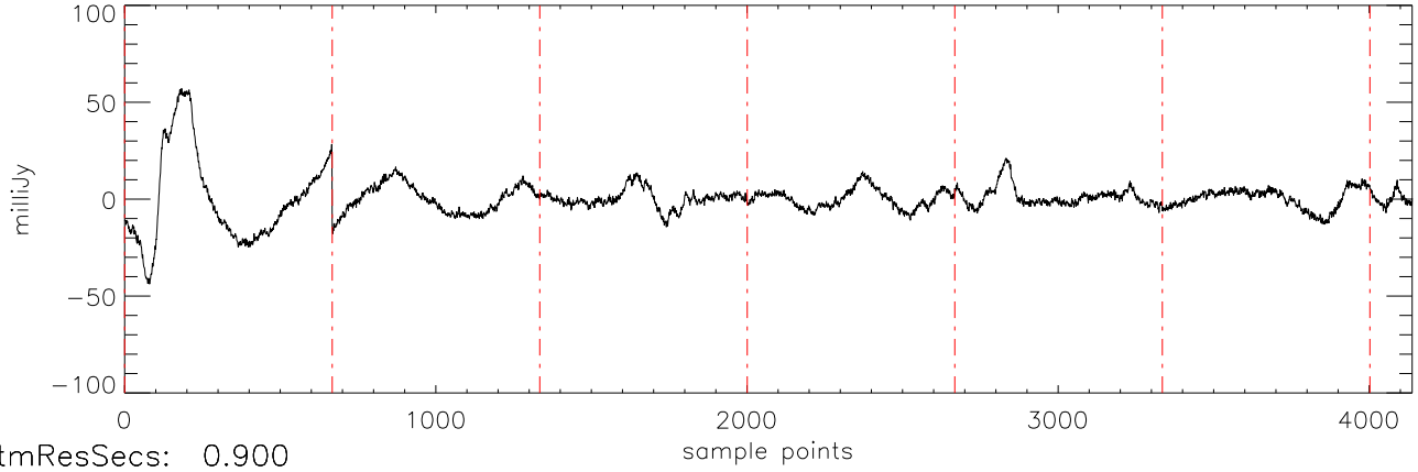
a2471 J00325937 17dec10 (AST) StokesI freq:5034.
