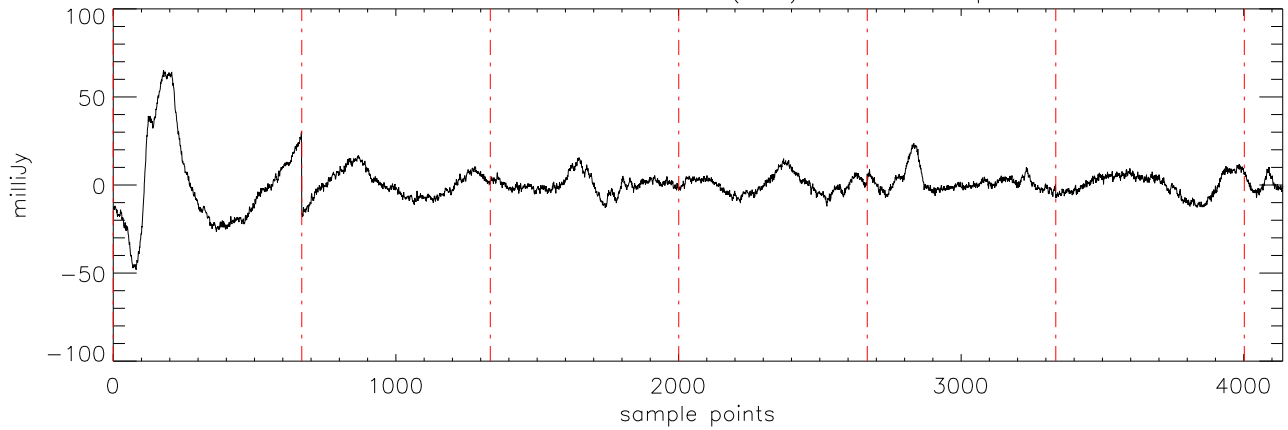
a2471 J00325937 17dec10 (AST) StokesI freq:5176.
