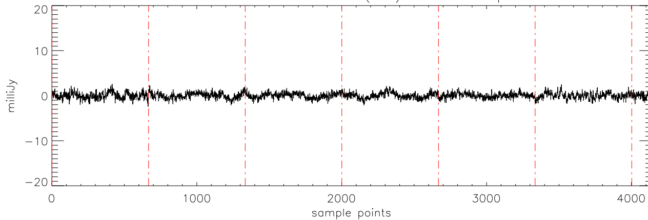
a2471 J00325937 17dec10 (AST) StokesU freq:5176.
