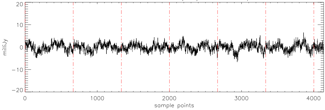
a2471 J00325937 17dec10 (AST) StokesQ freq:4750.
