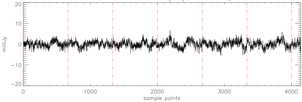
a2471 J00325937 17dec10 (AST) StokesQ freq:4608.
