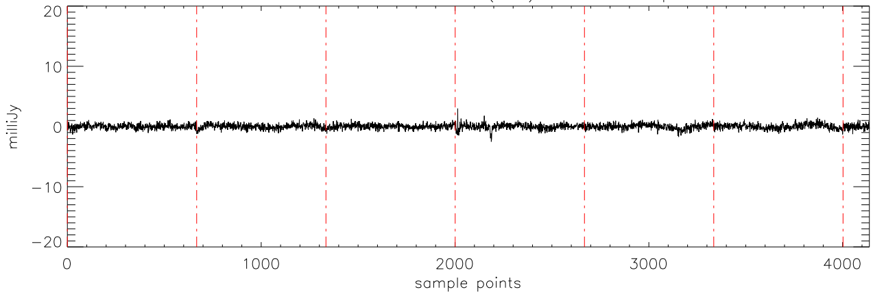
a2471 J00325937 17dec10 (AST) StokesV freq:4608.
