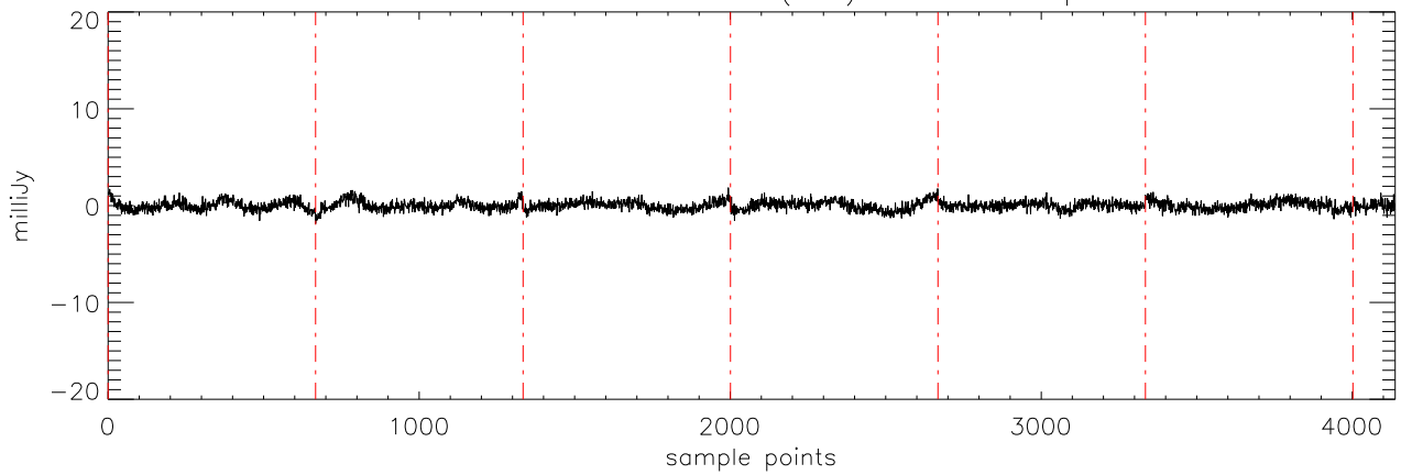
a2471 J00325937 17dec10 (AST) StokesU freq:4608.
