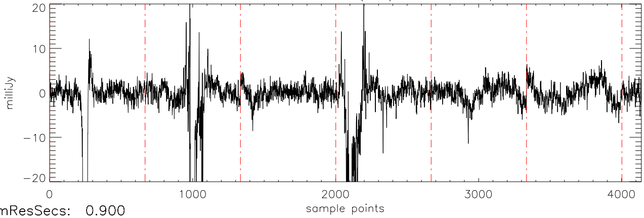
a2471 J00325937 17dec10 (AST) StokesQ freq:4466.
