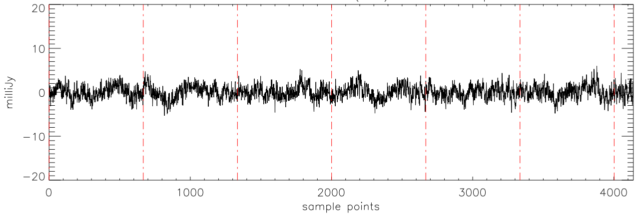
a2471 J00325937 17dec10 (AST) StokesQ freq:5176.
