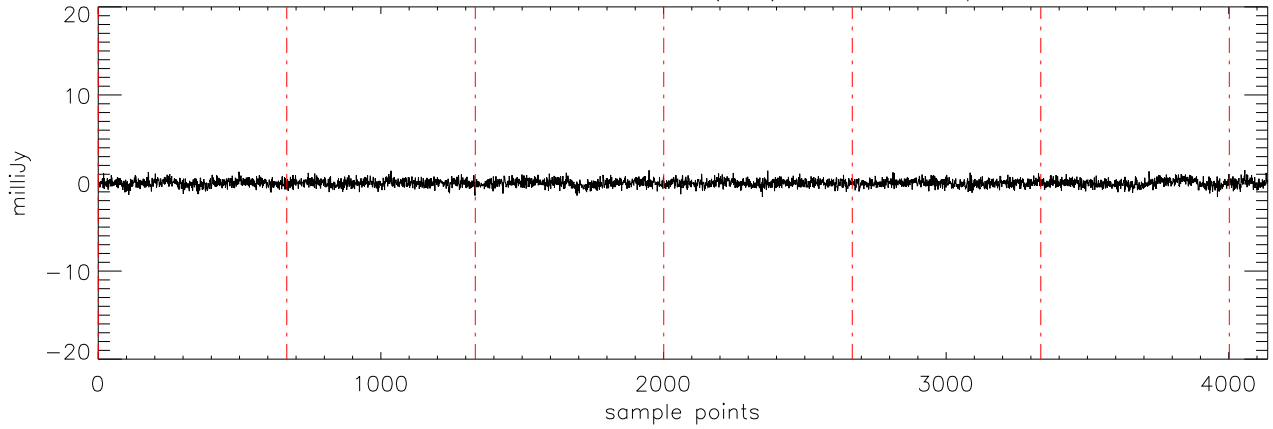
a2471 J00325937 17dec10 (AST) StokesV freq:4750.
