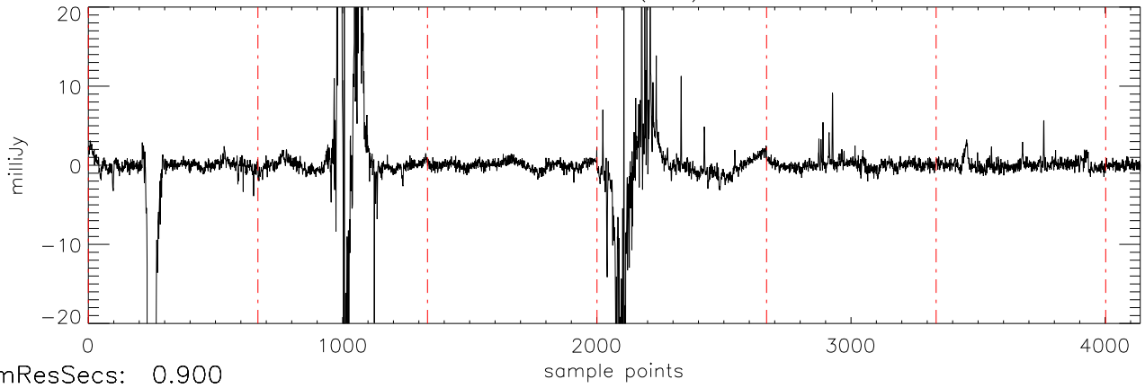
a2471 J00325937 17dec10 (AST) StokesU freq:4466.
