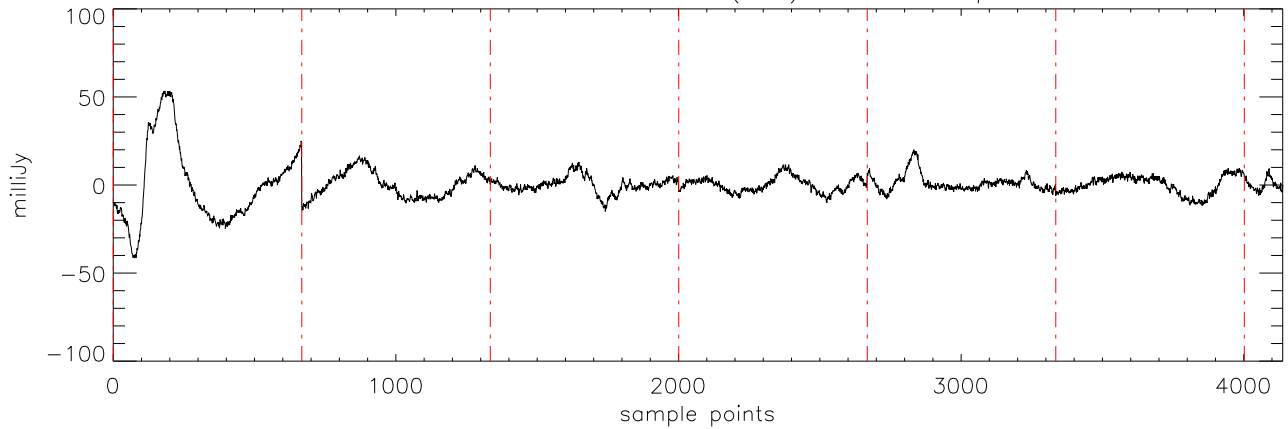
a2471 J00325937 17dec10 (AST) StokesI freq:4750.
