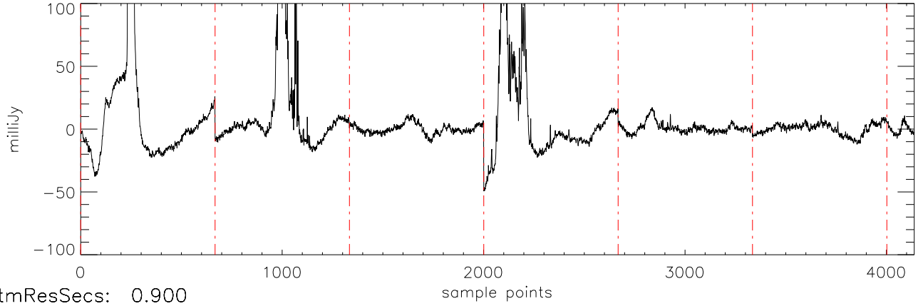
a2471 J00325937 17dec10 (AST) StokesI freq:4466.
