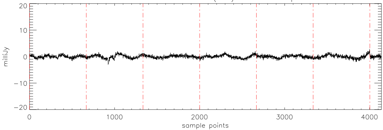
a2471 J00325937 17dec10 (AST) StokesU freq:4750.
