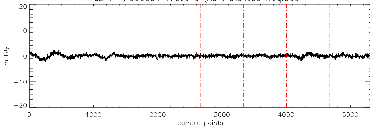
a2471 HD50554 17dec10 (AST) StokesU freq:5176.
