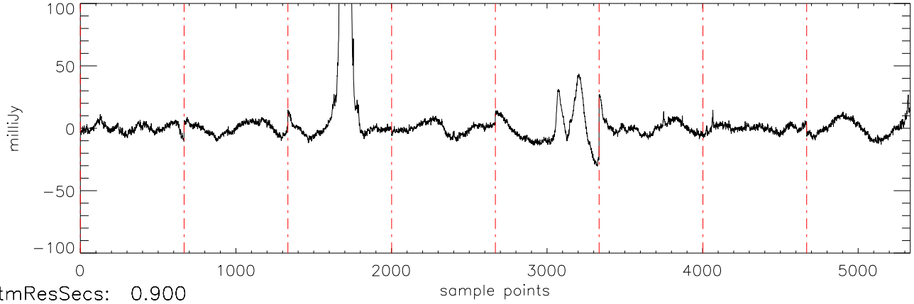
a2471 HD50554 17dec10 (AST) StokesI freq:4466.
