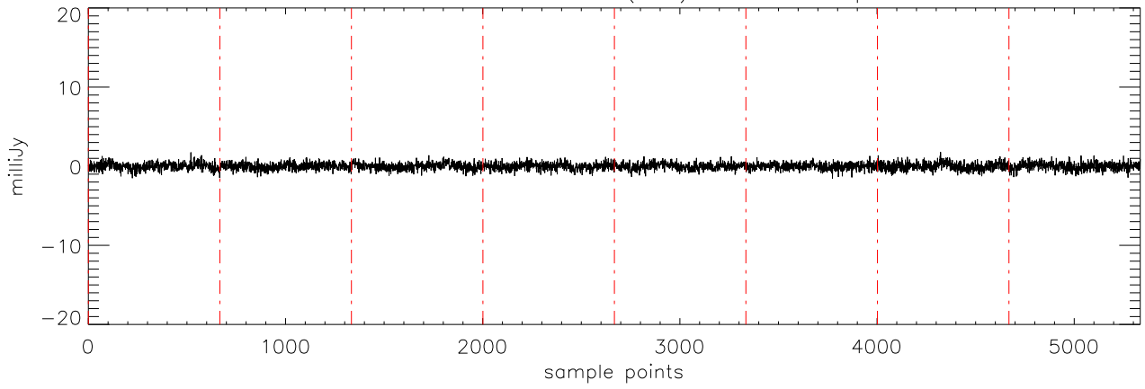
a2471 HD50554 17dec10 (AST) StokesV freq:5176.
