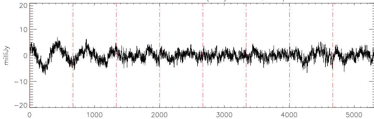
a2471 HD50554 17dec10 (AST) StokesQ freq:4608.
