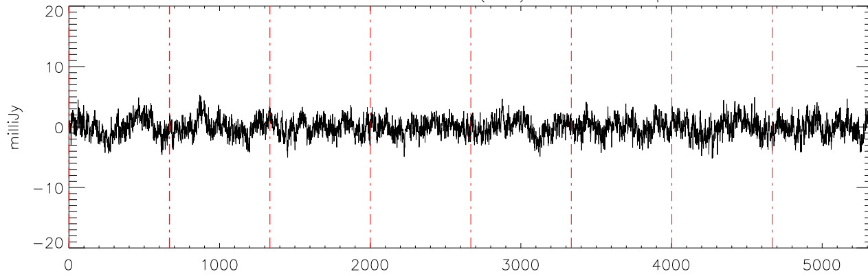
a2471 HD50554 17dec10 (AST) StokesQ freq:4750.
