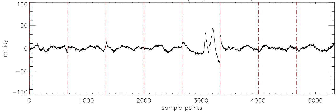
a2471 HD50554 17dec10 (AST) StokesI freq:4608.
