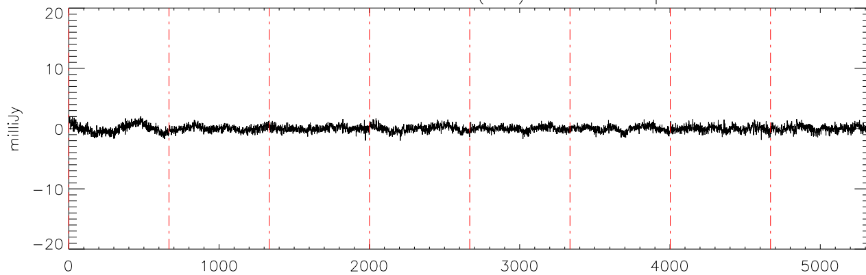
a2471 HD50554 17dec10 (AST) StokesU freq:4750.
