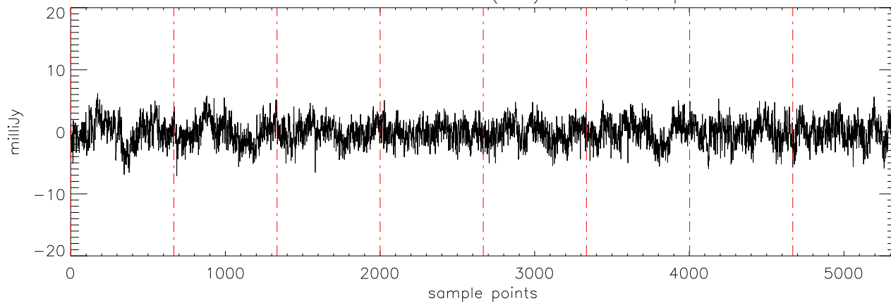
a2471 HD50554 17dec10 (AST) StokesQ freq:5176.
