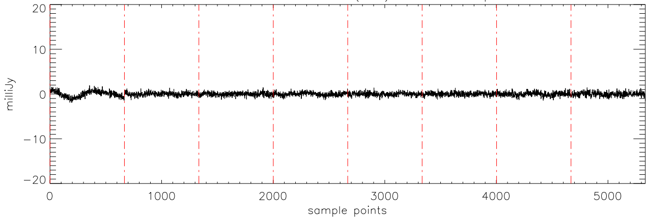
a2471 HD50554 17dec10 (AST) StokesV freq:4750.
