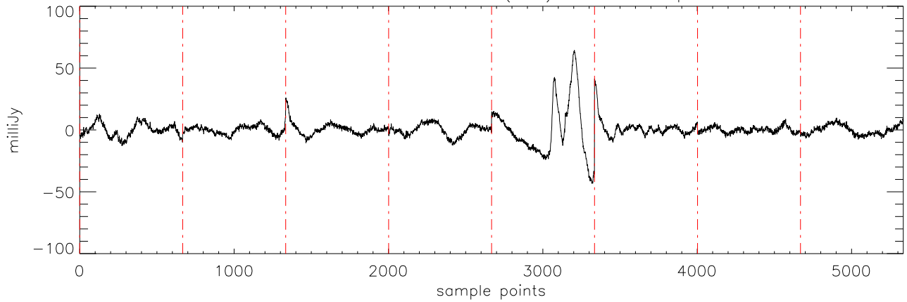
a2471 HD50554 17dec10 (AST) StokesI freq:5176.
