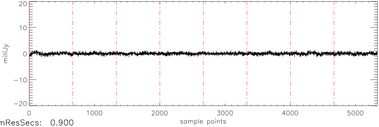
a2471 HD50554 17dec10 (AST) StokesV freq:5034.
