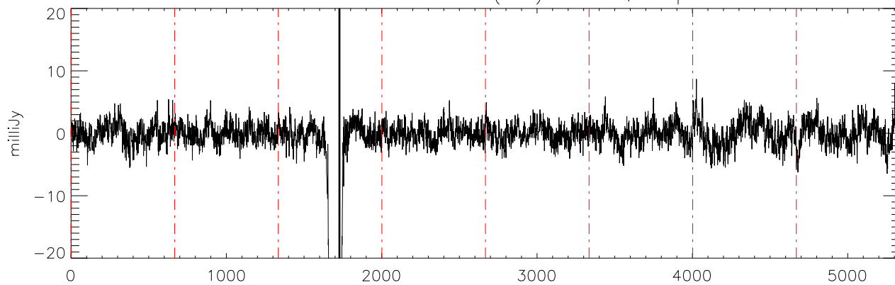
a2471 HD50554 17dec10 (AST) StokesQ freq:4325.
