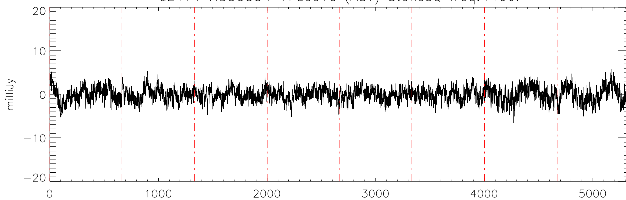
a2471 HD50554 17dec10 (AST) StokesQ freq:4466.
