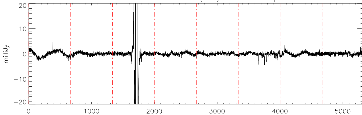
a2471 HD50554 17dec10 (AST) StokesU freq:4325.
