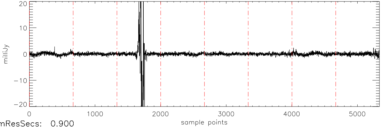
a2471 HD50554 17dec10 (AST) StokesV freq:4466.
