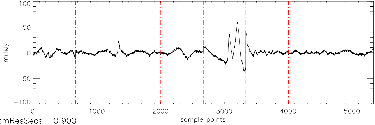
a2471 HD50554 17dec10 (AST) StokesI freq:5034.
