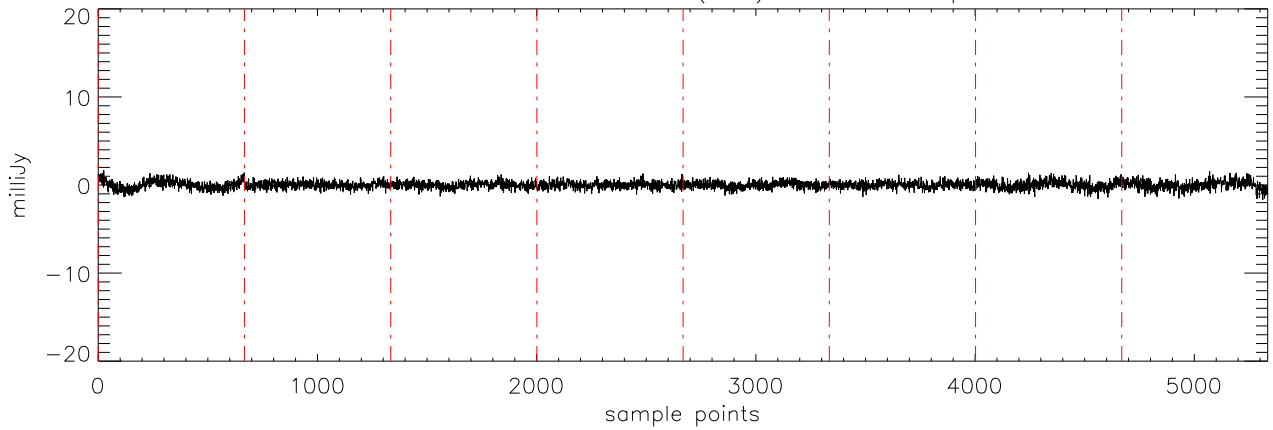
a2471 HD50554 17dec10 (AST) StokesV freq:4608.
