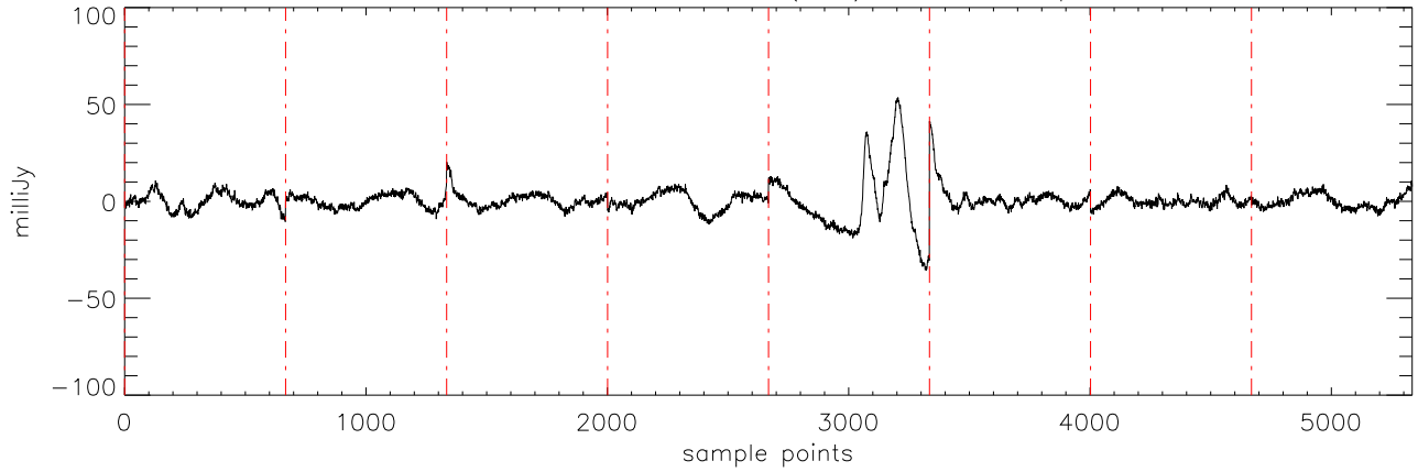
a2471 HD50554 17dec10 (AST) StokesI freq:4750.
