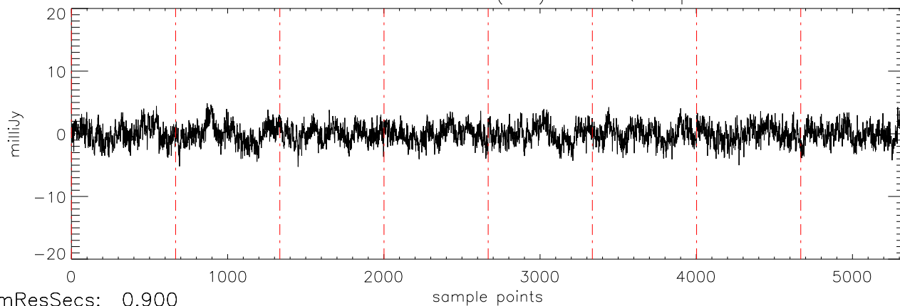
a2471 HD50554 17dec10 (AST) StokesQ freq:5034.
