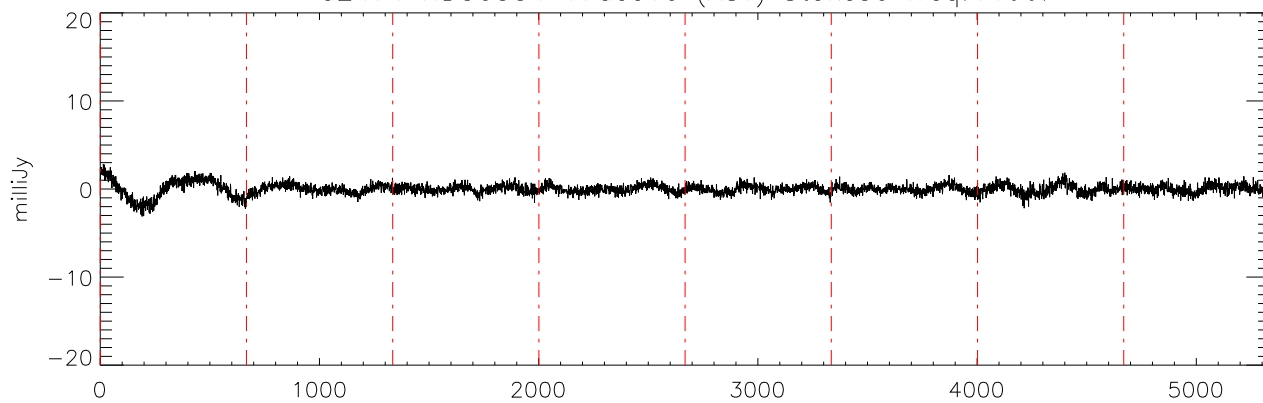
a2471 HD50554 17dec10 (AST) StokesU freq:4466.
