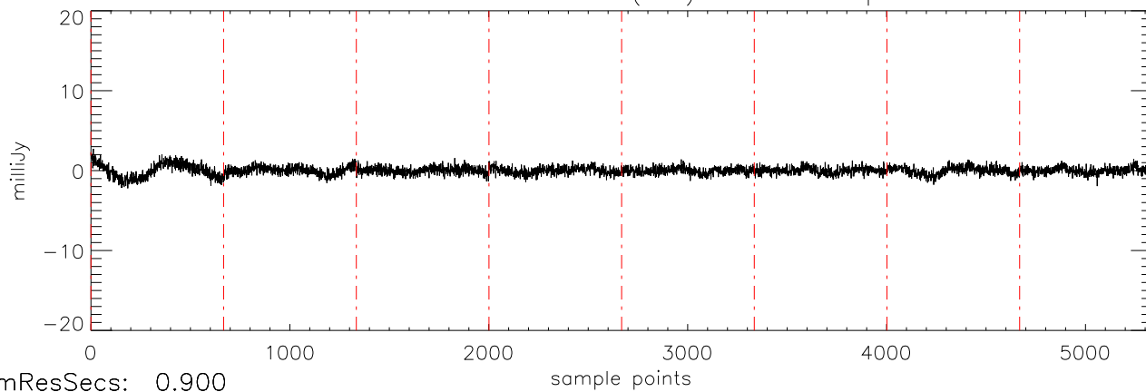
a2471 HD50554 17dec10 (AST) StokesU freq:5034.
