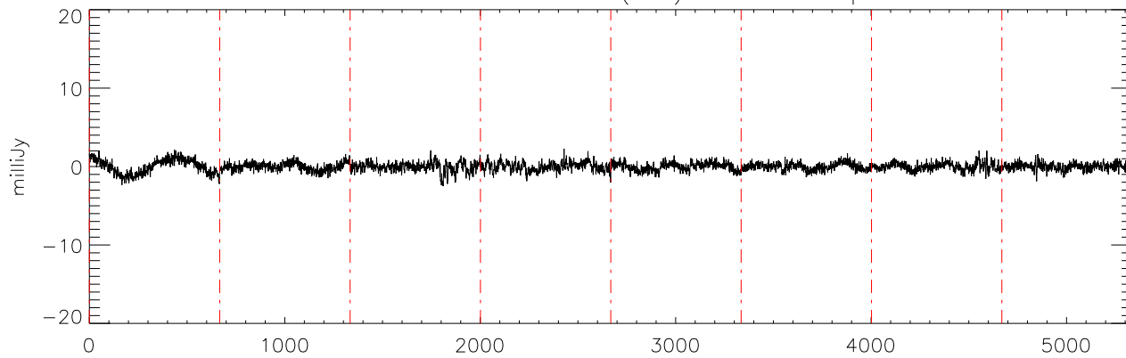
a2471 HD50554 17dec10 (AST) StokesU freq:4608.
