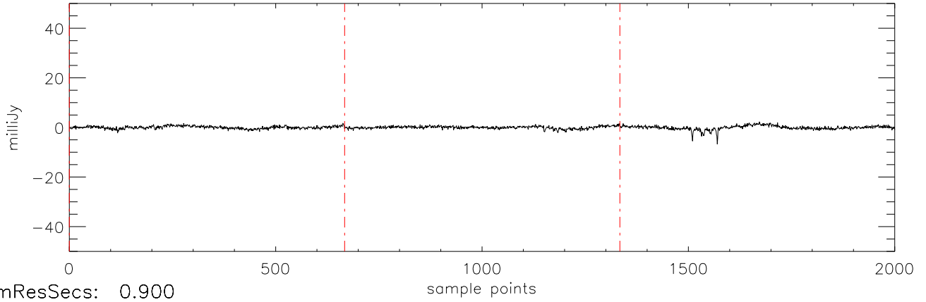
a2471 HD50554 08jan10 (AST) StokesU freq:4466.
