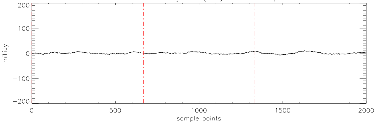
a2471 HD50554 08jan10 (AST) StokesI freq:4608.
