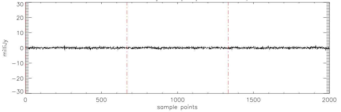
a2471 HD50554 08jan10 (AST) StokesV freq:5176.
