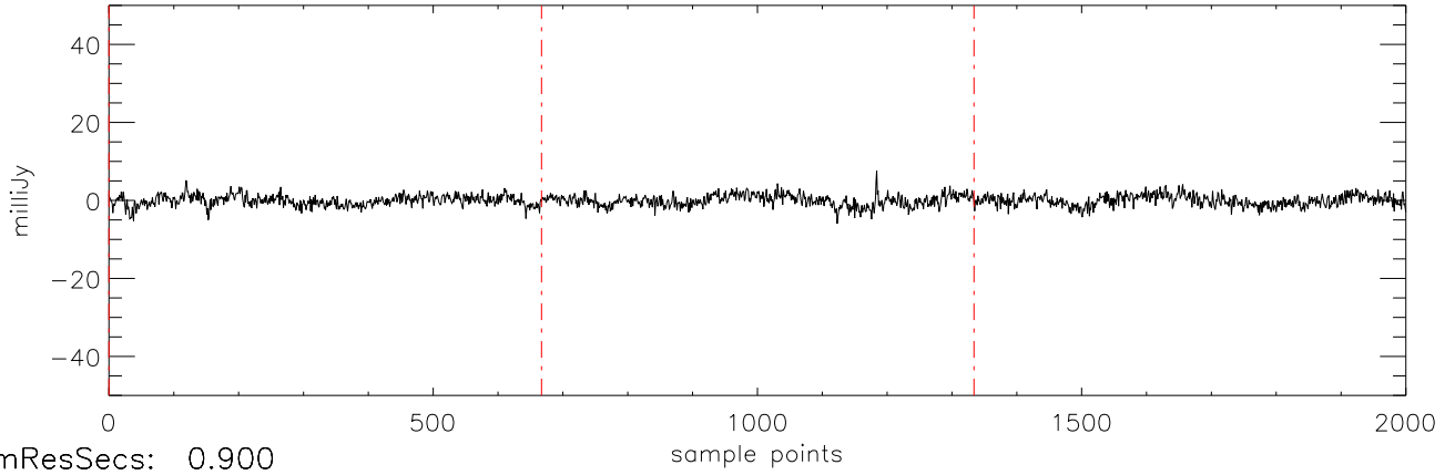
a2471 HD50554 08jan10 (AST) StokesQ freq:4466.
