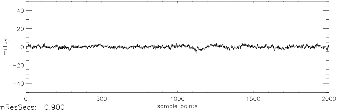
a2471 HD50554 08jan10 (AST) StokesQ freq:5034.
