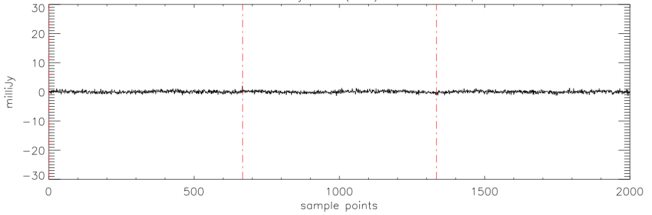
a2471 HD50554 08jan10 (AST) StokesV freq:4608.
