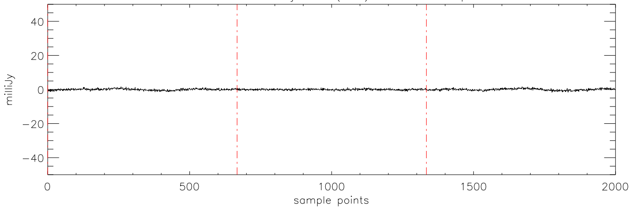
a2471 HD50554 08jan10 (AST) StokesU freq:4608.
