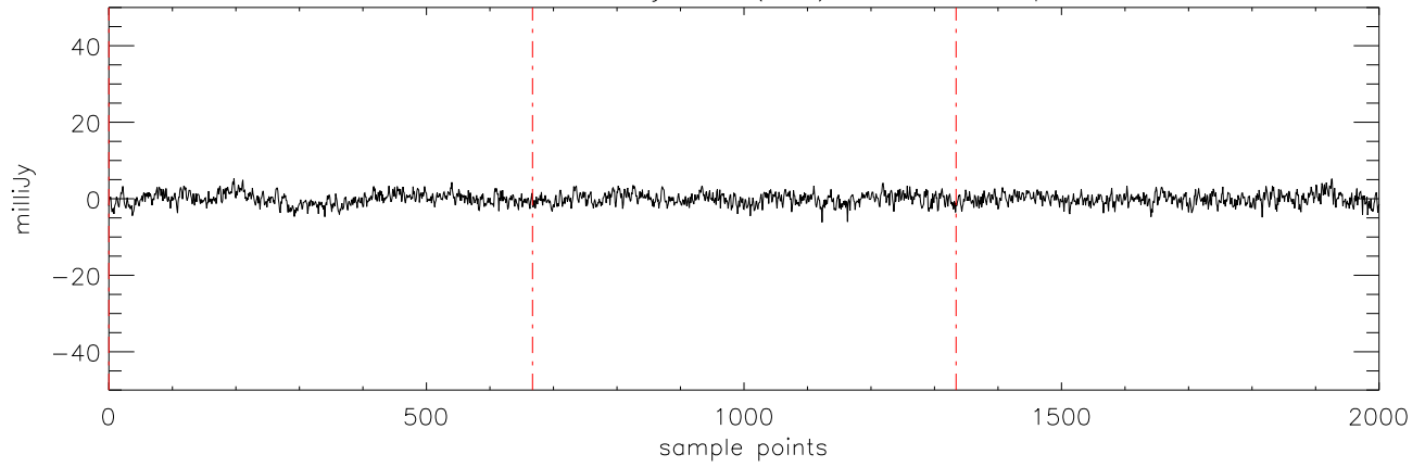
a2471 HD50554 08jan10 (AST) StokesQ freq:5176.
