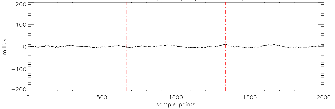
a2471 HD50554 08jan10 (AST) StokesI freq:4750.
