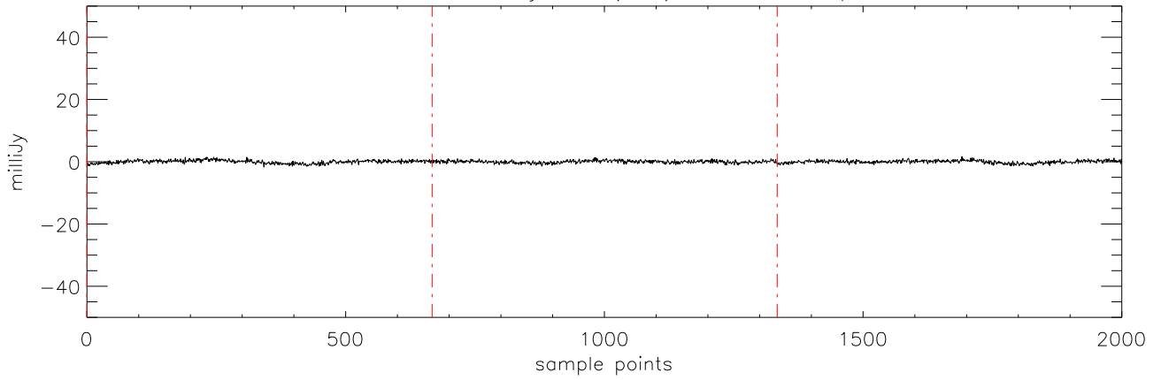
a2471 HD50554 08jan10 (AST) StokesU freq:4750.
