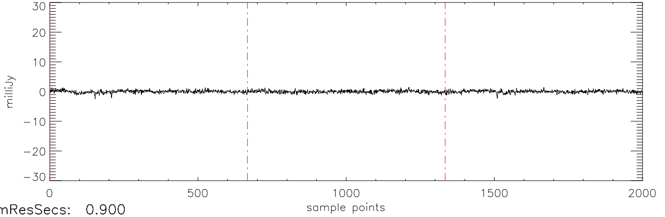
a2471 HD50554 08jan10 (AST) StokesV freq:4466.
