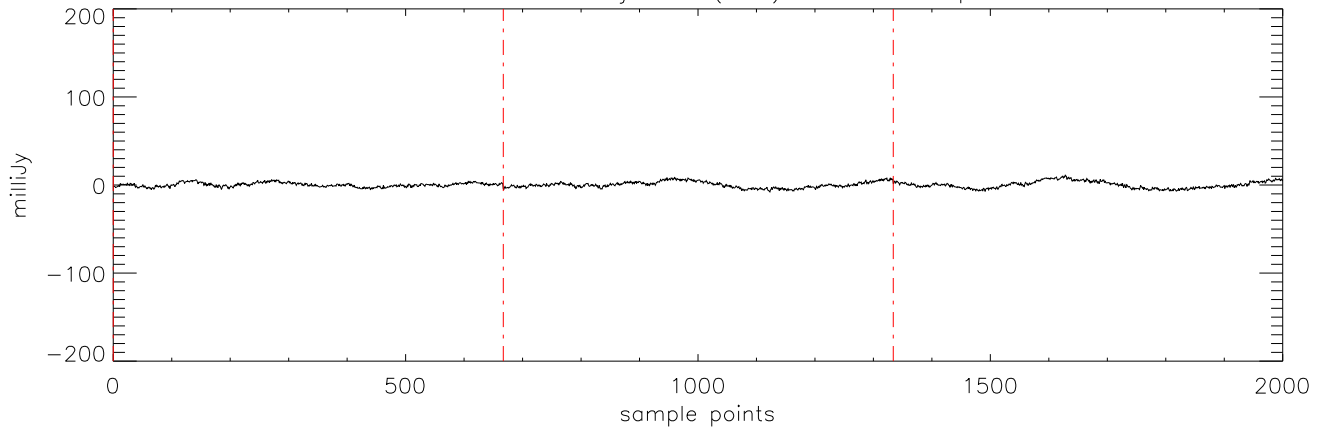
a2471 HD50554 08jan10 (AST) StokesI freq:5176.
