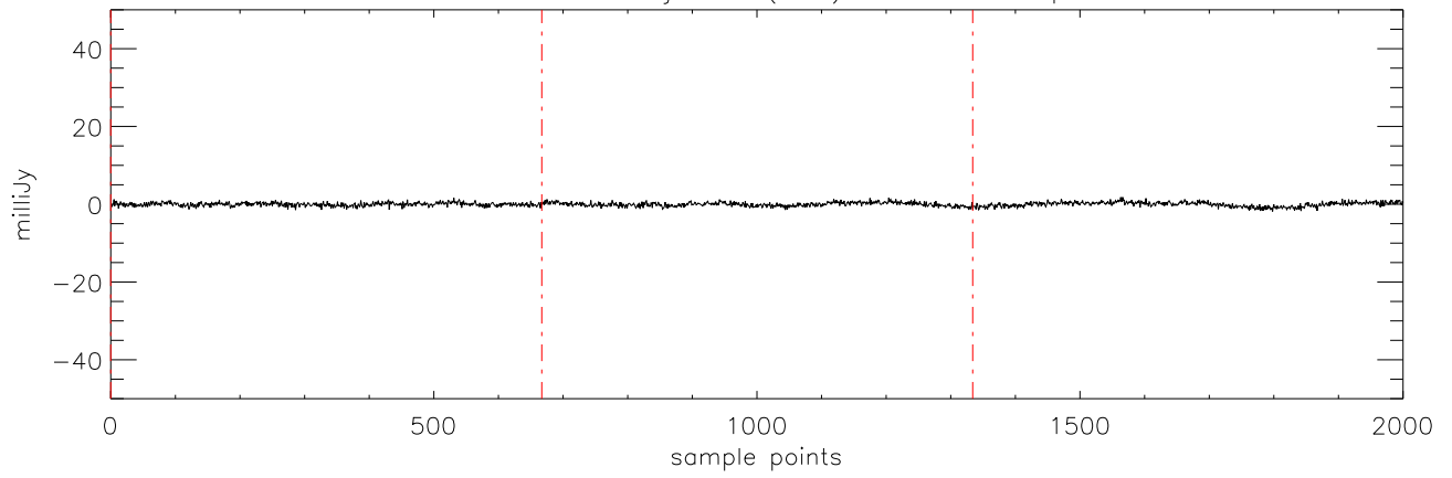
a2471 HD50554 08jan10 (AST) StokesU freq:5176.
