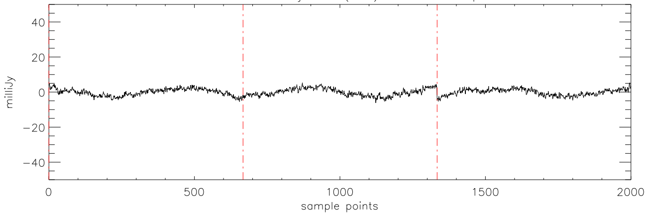
a2471 HD50554 08jan10 (AST) StokesQ freq:4608.
