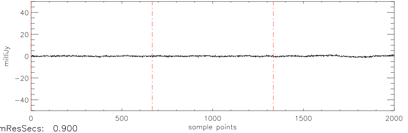
a2471 HD50554 08jan10 (AST) StokesU freq:5034.
