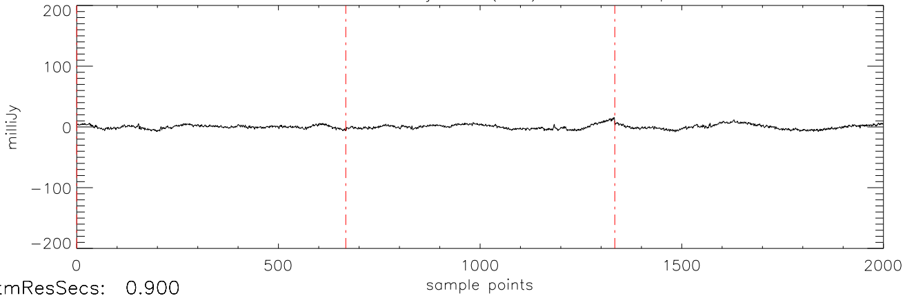
a2471 HD50554 08jan10 (AST) StokesI freq:4466.
