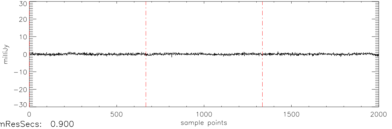
a2471 HD50554 08jan10 (AST) StokesV freq:5034.
