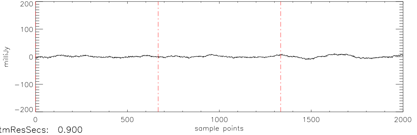
a2471 HD50554 08jan10 (AST) StokesI freq:5034.
