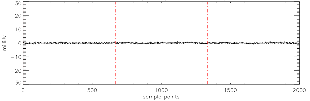
a2471 HD50554 08jan10 (AST) StokesV freq:4750.
