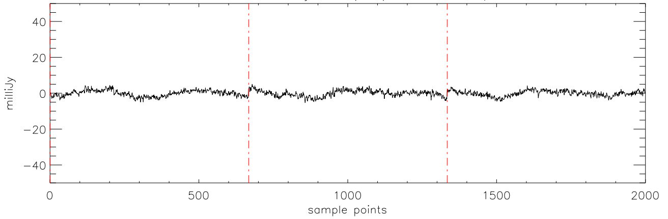
a2471 HD50554 08jan10 (AST) StokesQ freq:4750.
