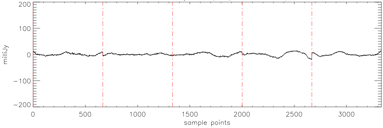
a2471 HD46375 09jan10 (AST) StokesI freq:4750.
