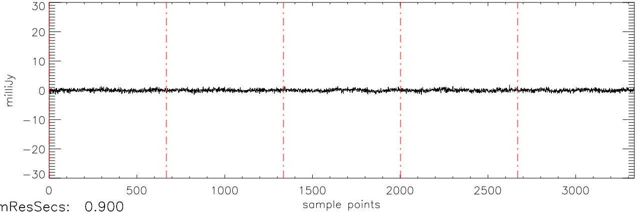
a2471 HD46375 09jan10 (AST) StokesV freq:5034.
