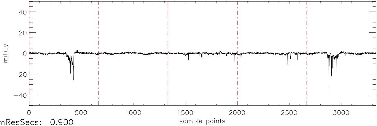
a2471 HD46375 09jan10 (AST) StokesU freq:4466.
