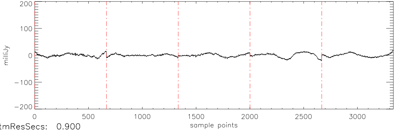
a2471 HD46375 09jan10 (AST) StokesI freq:5034.
