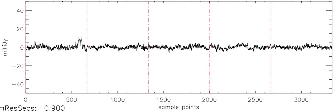
a2471 HD46375 09jan10 (AST) StokesQ freq:5034.
