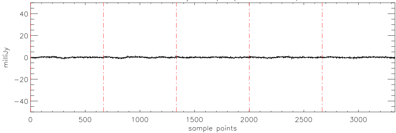
a2471 HD46375 09jan10 (AST) StokesU freq:4750.
