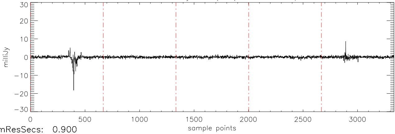
a2471 HD46375 09jan10 (AST) StokesV freq:4466.
