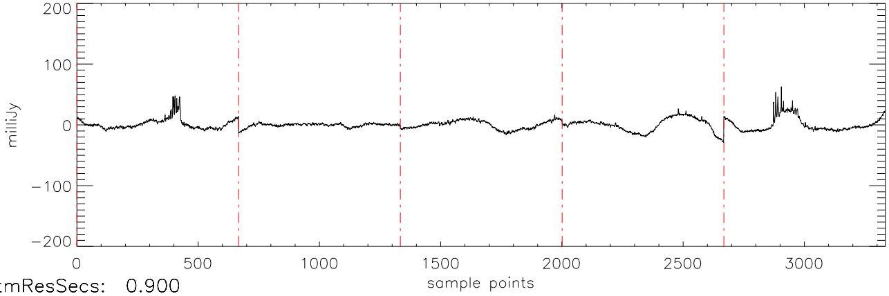
a2471 HD46375 09jan10 (AST) StokesI freq:4466.
