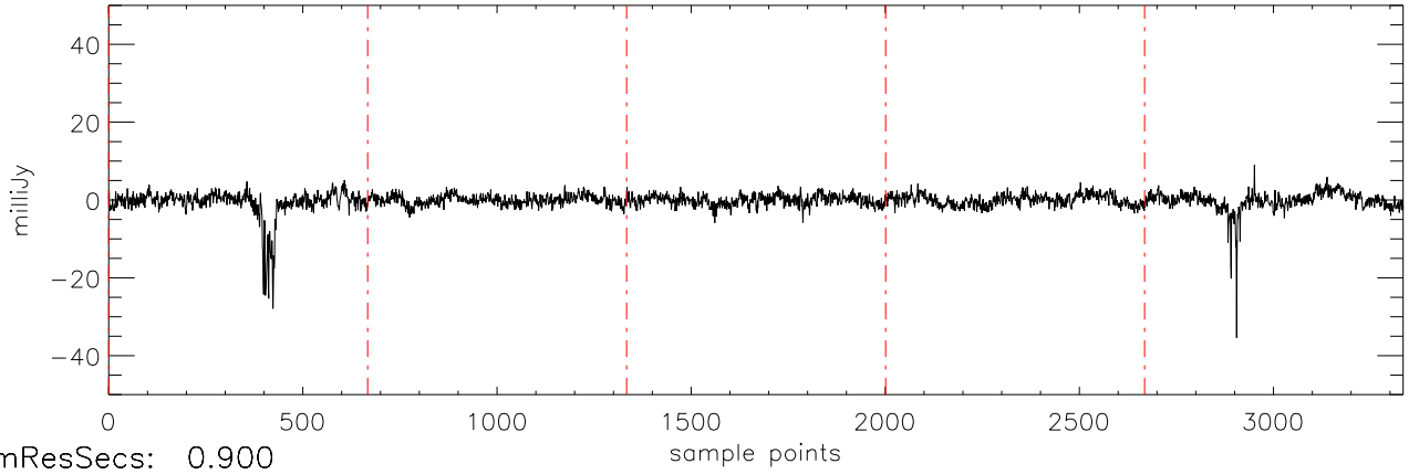
a2471 HD46375 09jan10 (AST) StokesQ freq:4466.
