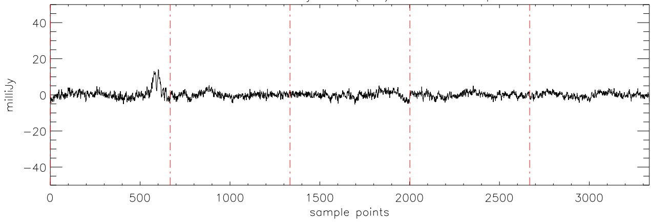
a2471 HD46375 09jan10 (AST) StokesQ freq:5176.
