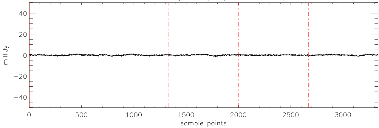
a2471 HD46375 09jan10 (AST) StokesU freq:4608.
