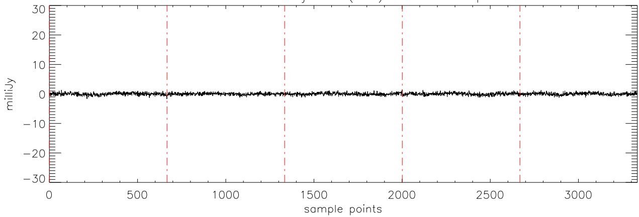
a2471 HD46375 09jan10 (AST) StokesV freq:4608.
