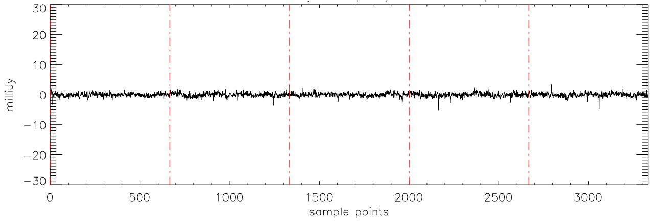
a2471 HD46375 09jan10 (AST) StokesV freq:5176.
