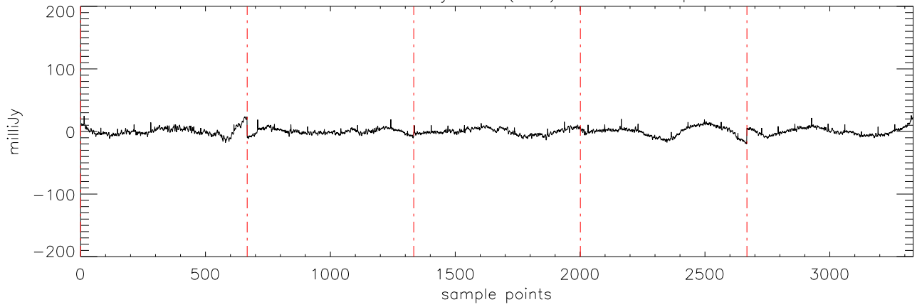
a2471 HD46375 09jan10 (AST) StokesI freq:5176.
