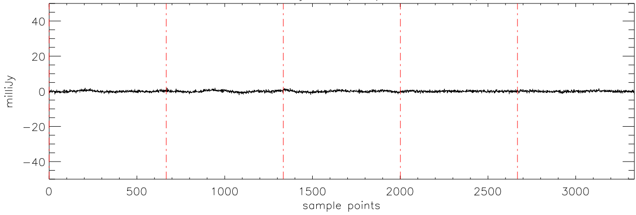
a2471 HD46375 09jan10 (AST) StokesU freq:5176.
