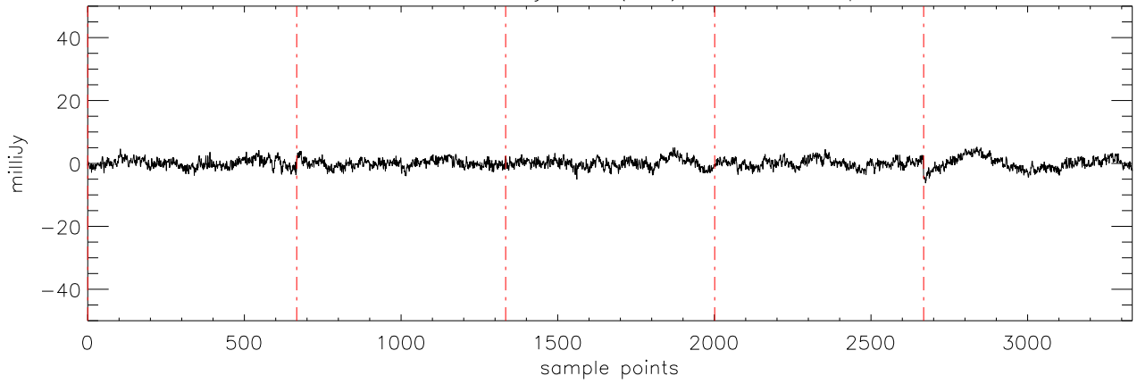
a2471 HD46375 09jan10 (AST) StokesQ freq:4750.
