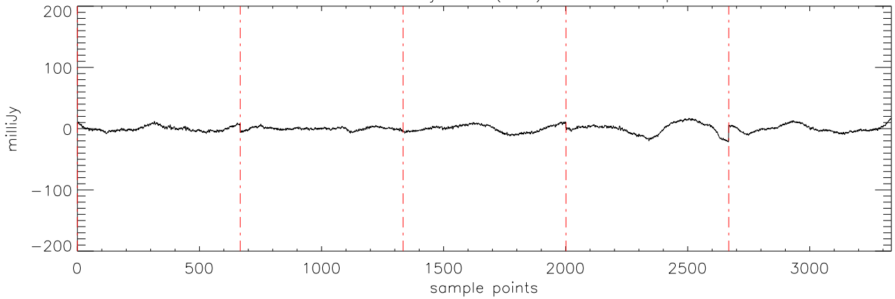
a2471 HD46375 09jan10 (AST) StokesI freq:4608.
