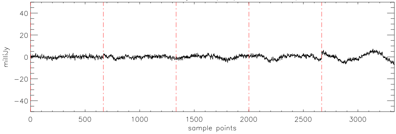
a2471 HD46375 09jan10 (AST) StokesQ freq:4608.
