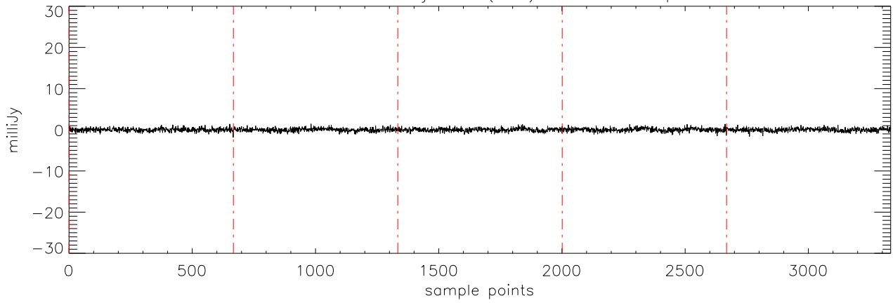
a2471 HD46375 09jan10 (AST) StokesV freq:4750.
