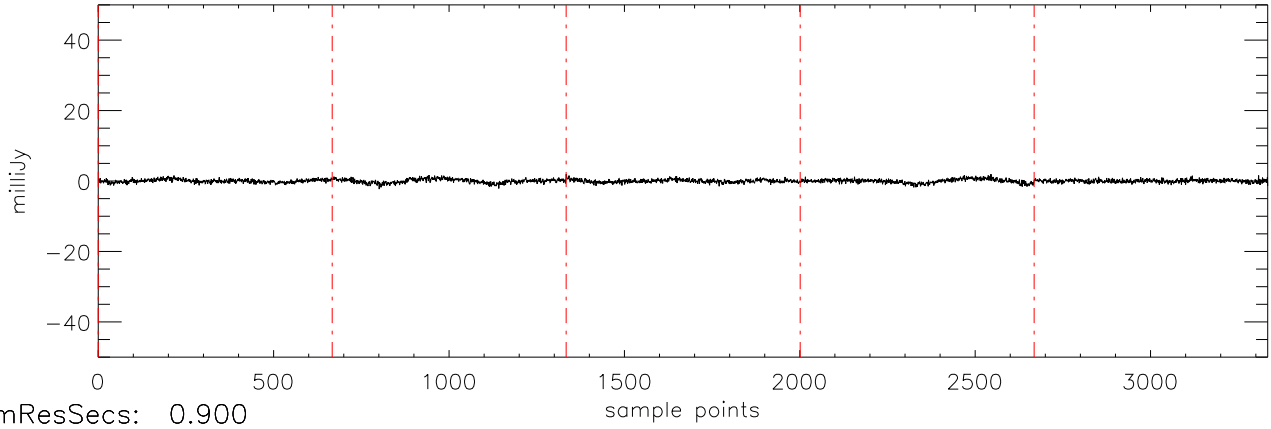
a2471 HD46375 09jan10 (AST) StokesU freq:5034.
