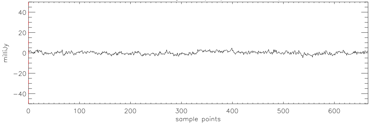
a2471 HD114762 07jan10 (AST) StokesQ freq:4750.
