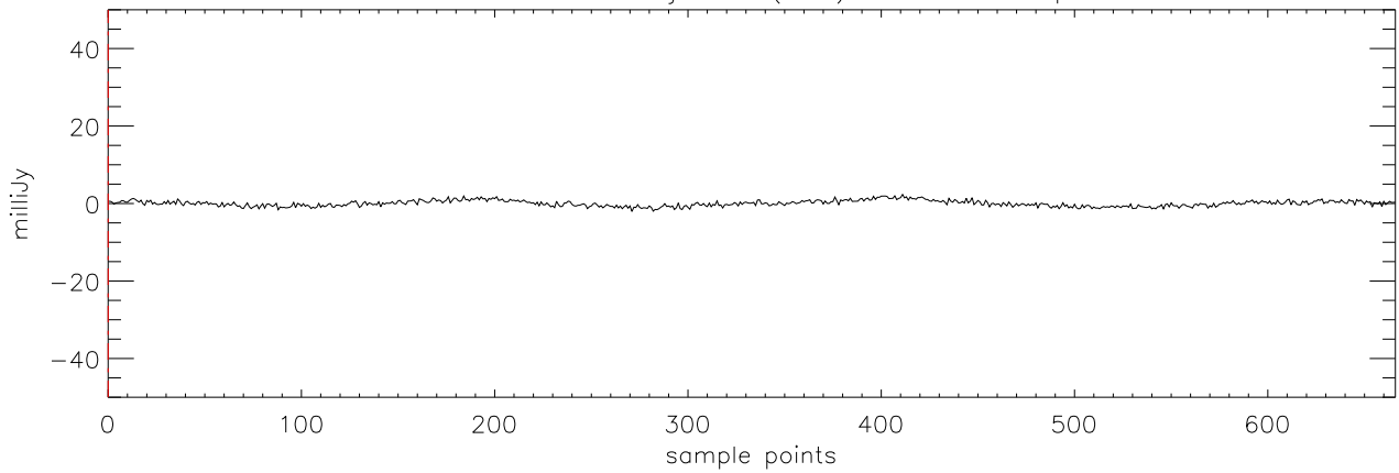
a2471 HD114762 07jan10 (AST) StokesU freq:4608.
