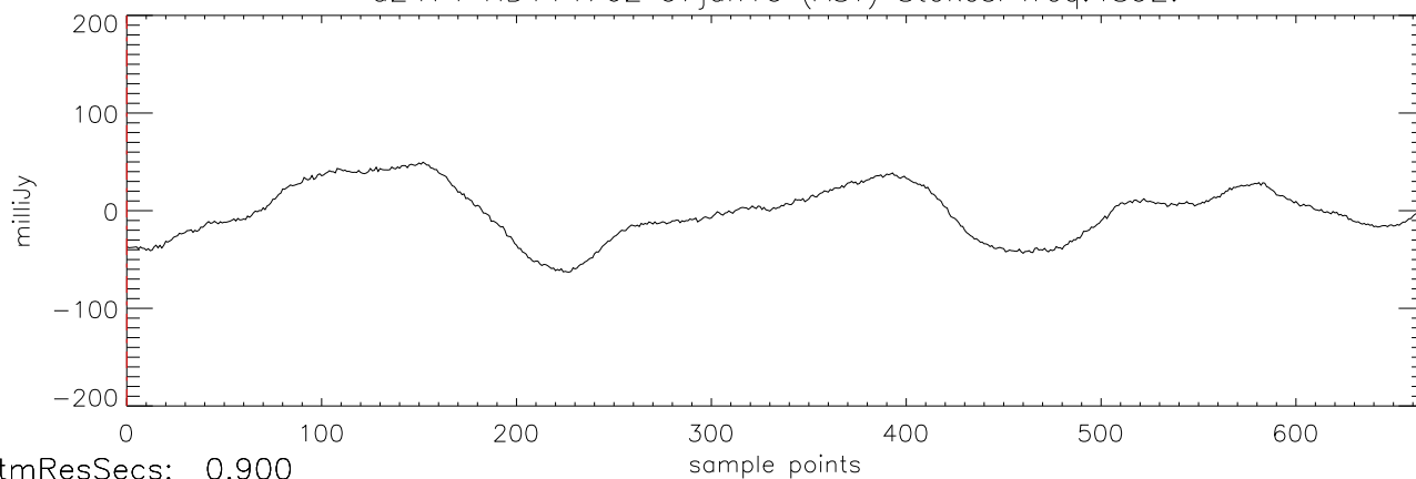
a2471 HD114762 07jan10 (AST) StokesI freq:5034.
