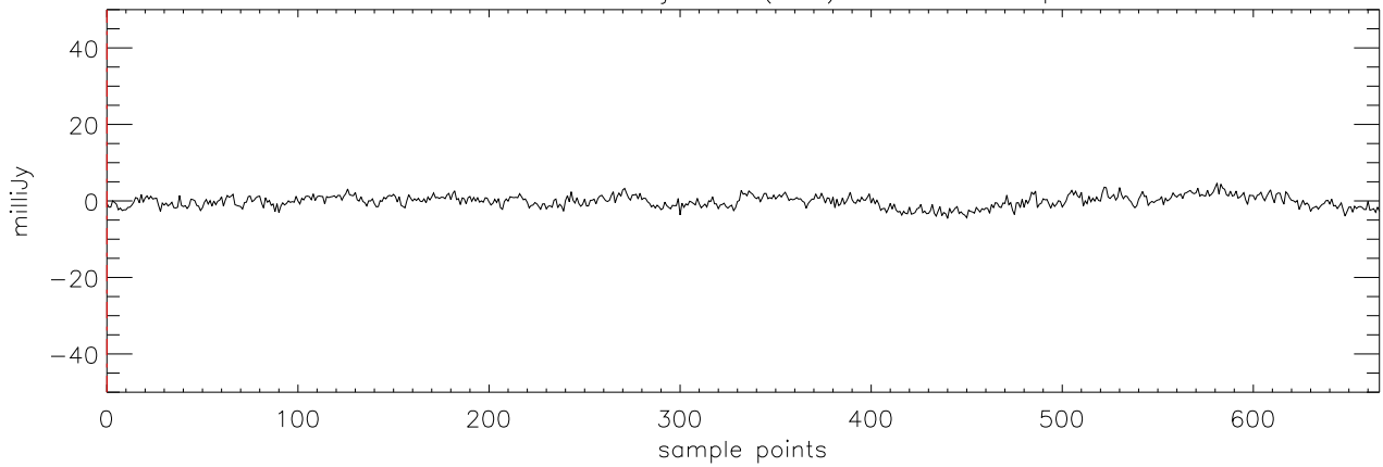
a2471 HD114762 07jan10 (AST) StokesQ freq:4608.
