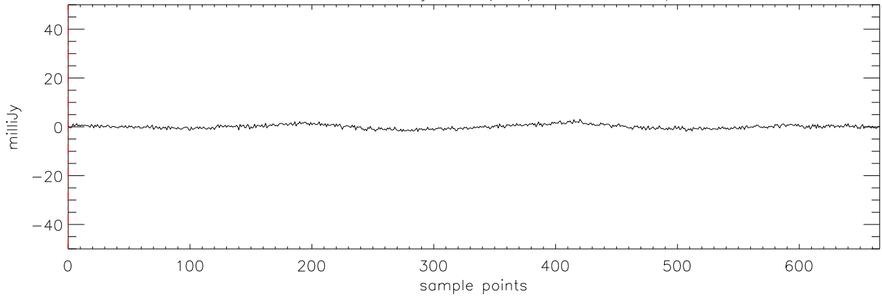
a2471 HD114762 07jan10 (AST) StokesU freq:4750.
