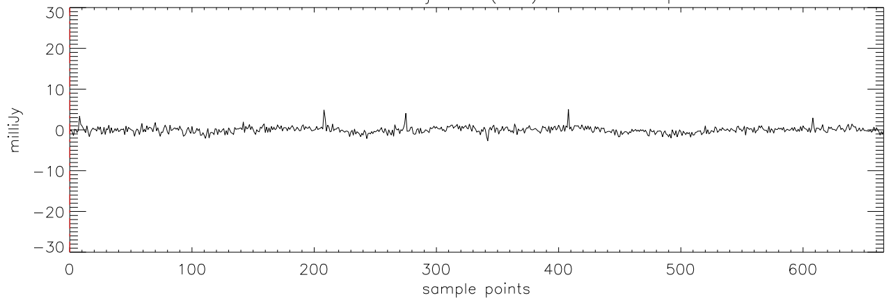
a2471 HD114762 07jan10 (AST) StokesV freq:5176.
