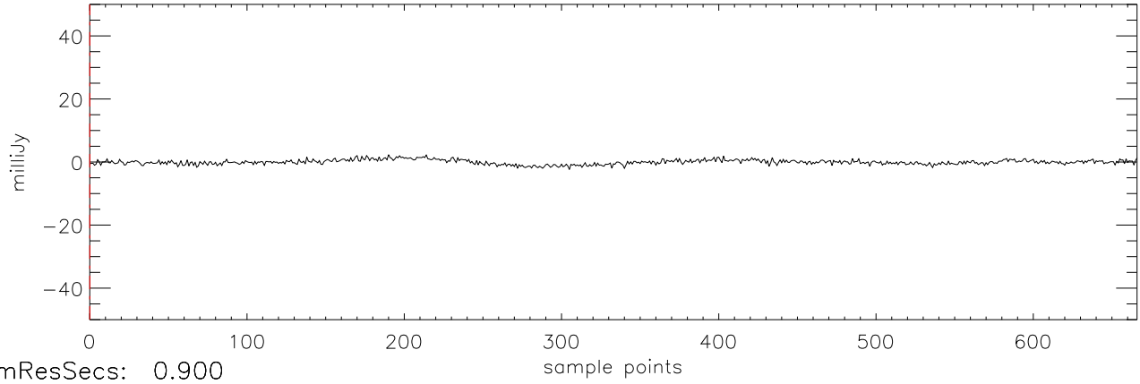
a2471 HD114762 07jan10 (AST) StokesU freq:5034.
