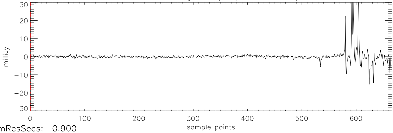
a2471 HD114762 07jan10 (AST) StokesV freq:4466.
