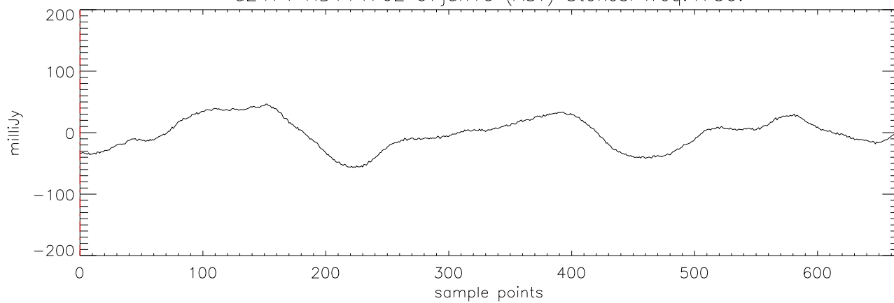
a2471 HD114762 07jan10 (AST) StokesI freq:4750.
