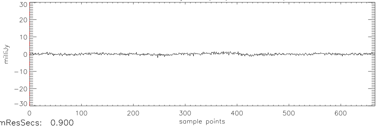
a2471 HD114762 07jan10 (AST) StokesV freq:5034.
