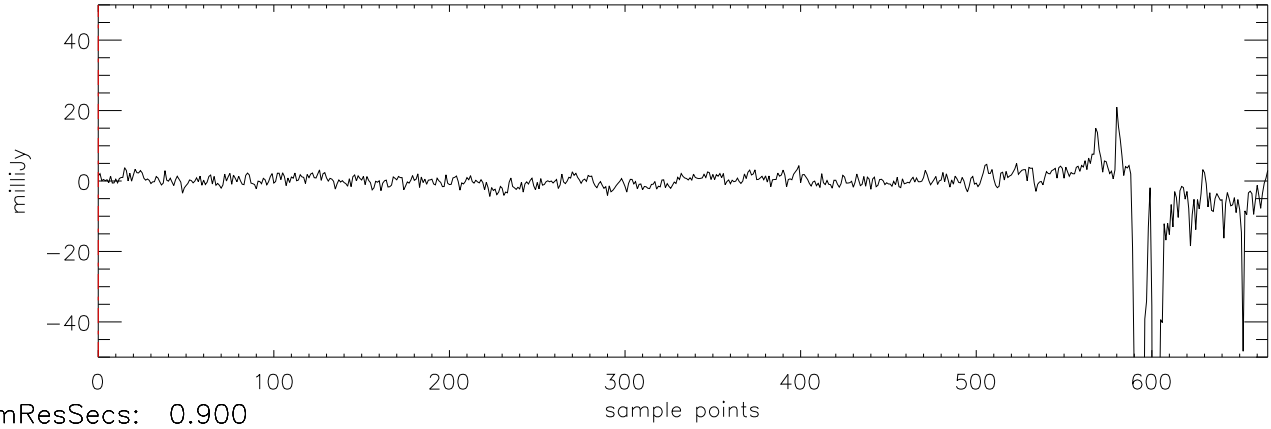
a2471 HD114762 07jan10 (AST) StokesQ freq:4466.
