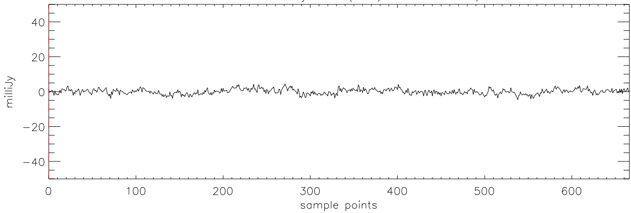
a2471 HD114762 07jan10 (AST) StokesQ freq:5176.
