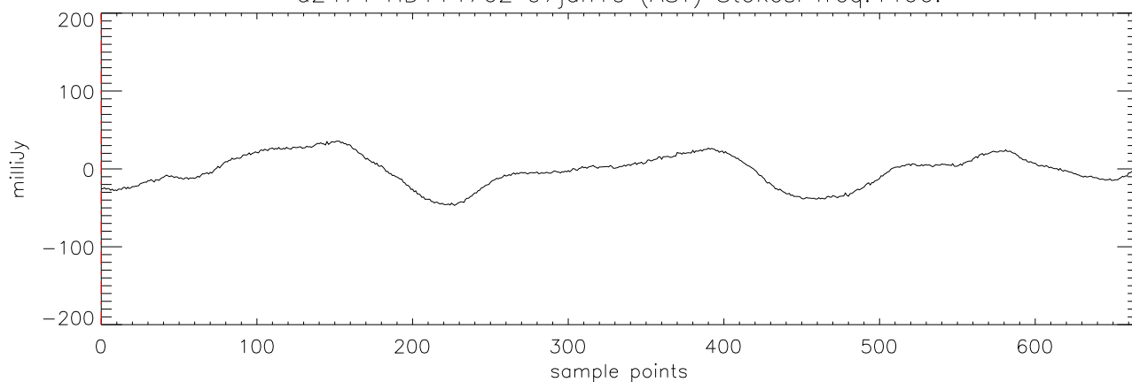
a2471 HD114762 07jan10 (AST) StokesI freq:4608.
