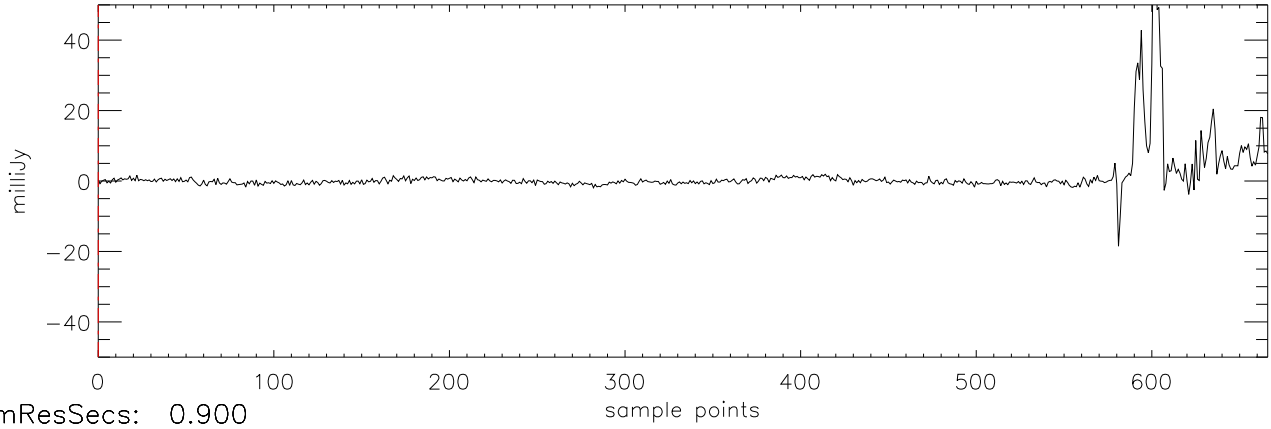
a2471 HD114762 07jan10 (AST) StokesU freq:4466.
