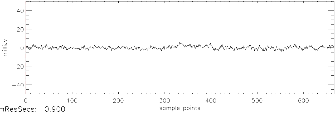
a2471 HD114762 07jan10 (AST) StokesQ freq:5034.
