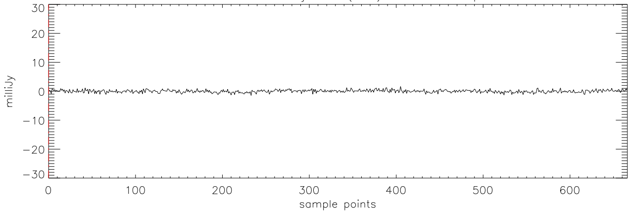
a2471 HD114762 07jan10 (AST) StokesV freq:4750.
