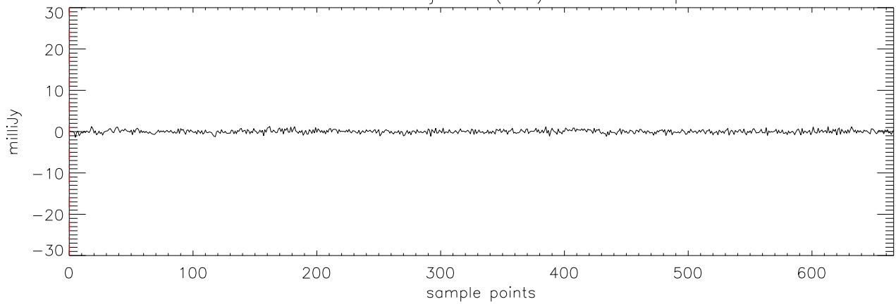
a2471 HD114762 07jan10 (AST) StokesV freq:4608.
