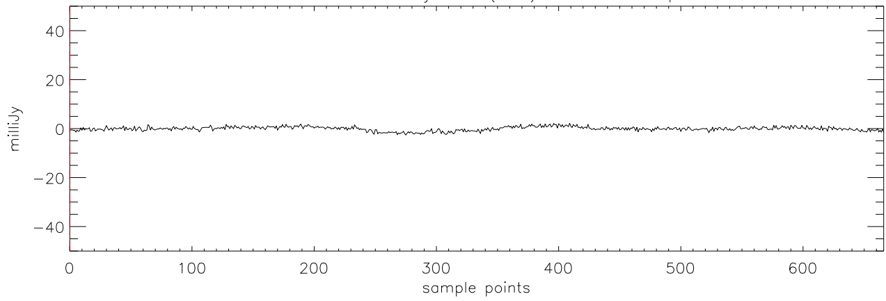
a2471 HD114762 07jan10 (AST) StokesU freq:5176.
