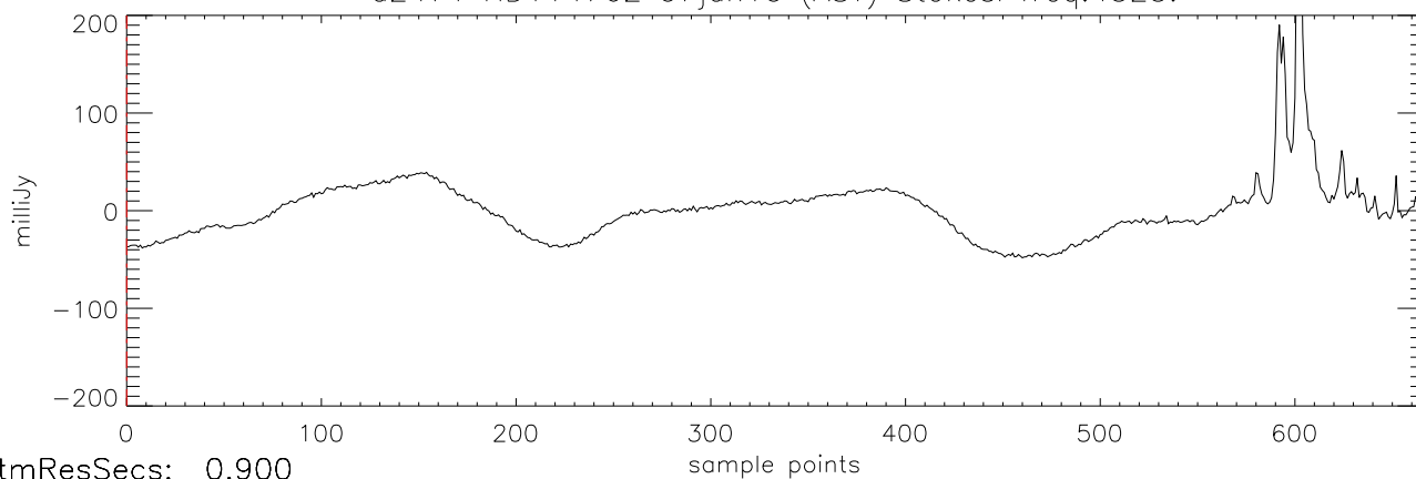
a2471 HD114762 07jan10 (AST) StokesI freq:4466.
