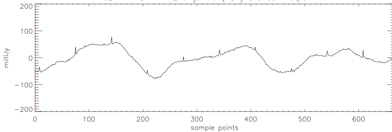
a2471 HD114762 07jan10 (AST) StokesI freq:5176.
