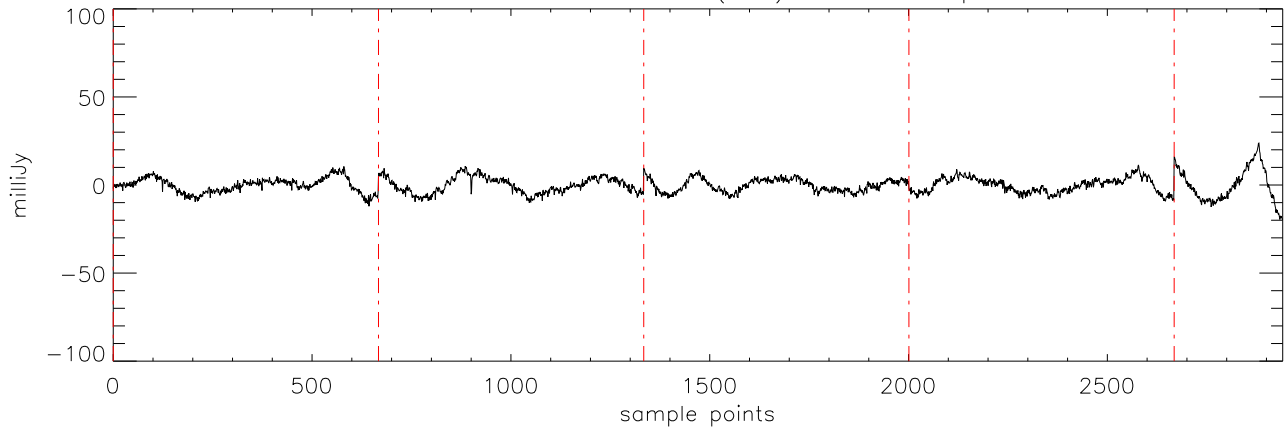
a2471 HD10697 20dec10 (AST) StokesI freq:5176.
