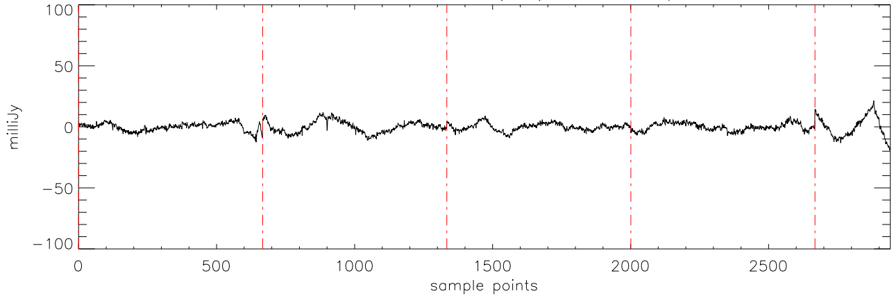
a2471 HD10697 20dec10 (AST) StokesI freq:4750.
