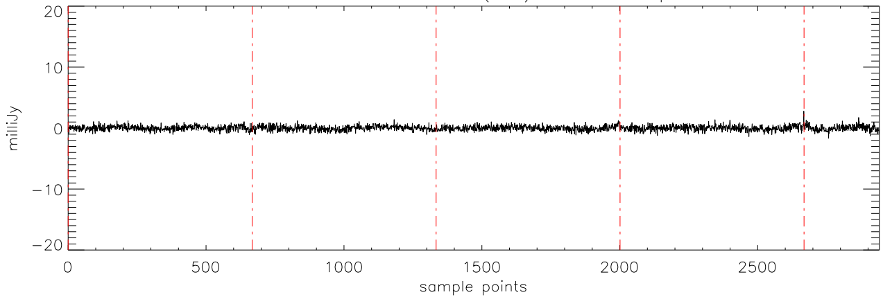
a2471 HD10697 20dec10 (AST) StokesV freq:4750.
