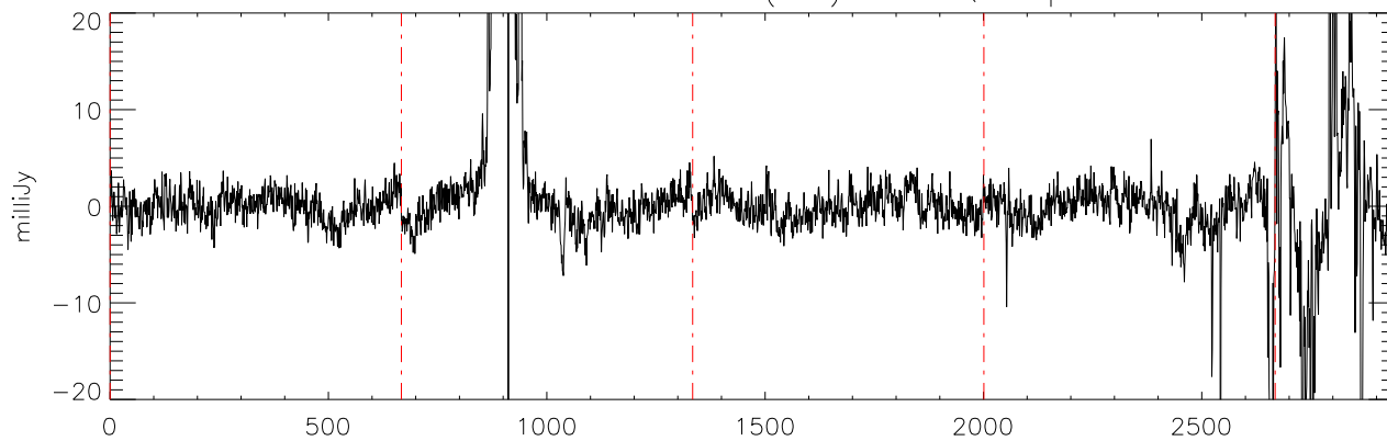
a2471 HD10697 20dec10 (AST) StokesQ freq:4325.
