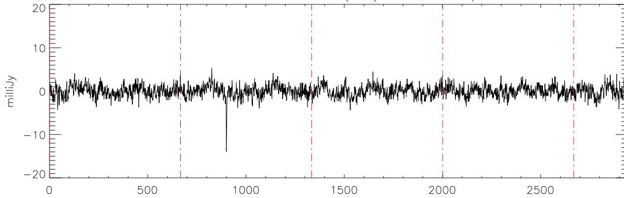
a2471 HD10697 20dec10 (AST) StokesQ freq:4750.
