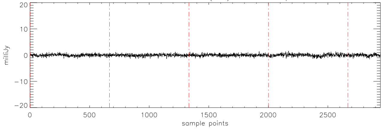
a2471 HD10697 20dec10 (AST) StokesV freq:5176.
