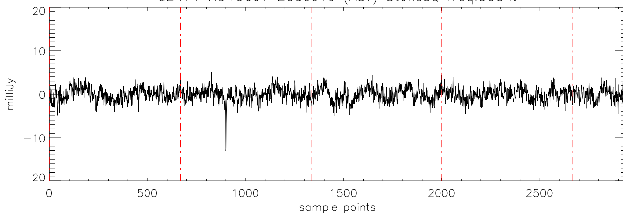
a2471 HD10697 20dec10 (AST) StokesQ freq:5176.
