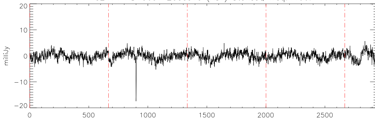
a2471 HD10697 20dec10 (AST) StokesQ freq:4466.
