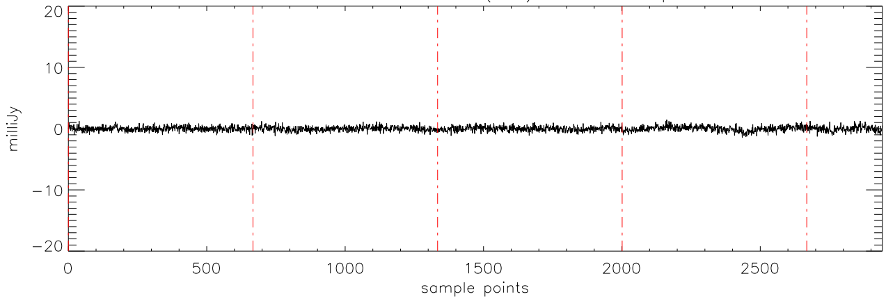
a2471 HD10697 20dec10 (AST) StokesV freq:4608.
