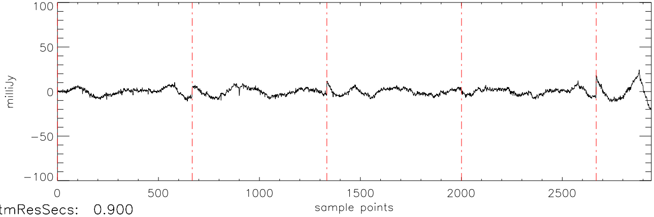
a2471 HD10697 20dec10 (AST) StokesI freq:5034.
