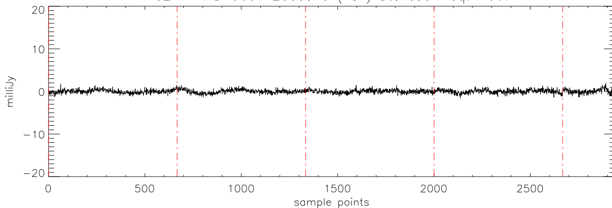
a2471 HD10697 20dec10 (AST) StokesU freq:4608.
