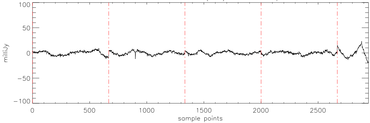
a2471 HD10697 20dec10 (AST) StokesI freq:4608.
