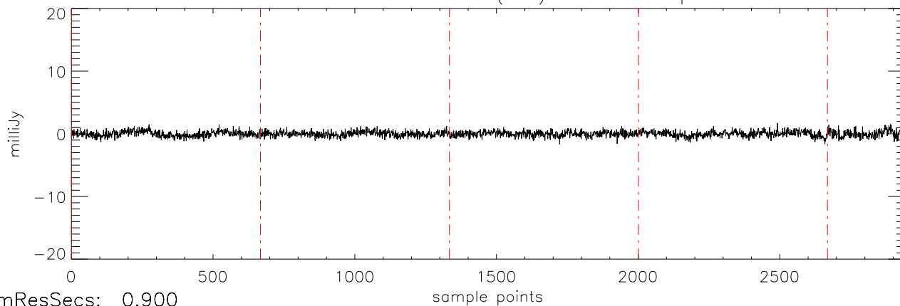
a2471 HD10697 20dec10 (AST) StokesU freq:5034.
