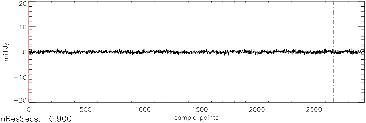
a2471 HD10697 20dec10 (AST) StokesV freq:5034.
