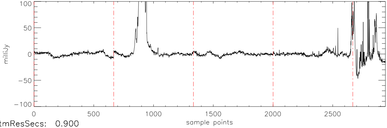
a2471 HD10697 20dec10 (AST) StokesI freq:4466.
