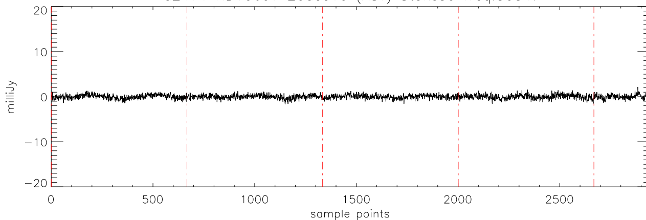
a2471 HD10697 20dec10 (AST) StokesU freq:5176.
