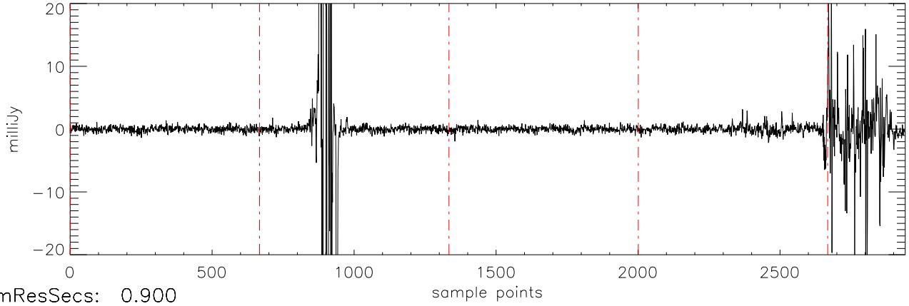
a2471 HD10697 20dec10 (AST) StokesV freq:4466.
