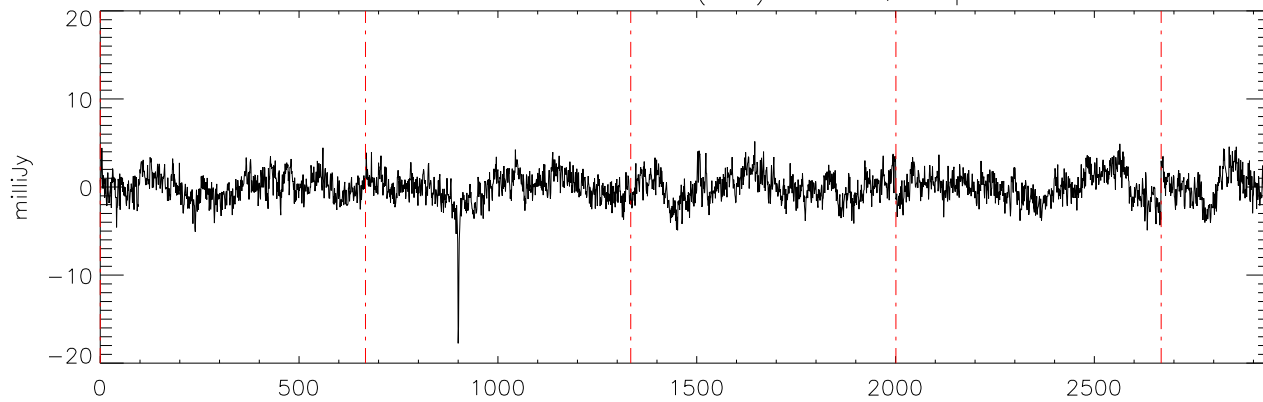
a2471 HD10697 20dec10 (AST) StokesQ freq:4608.
