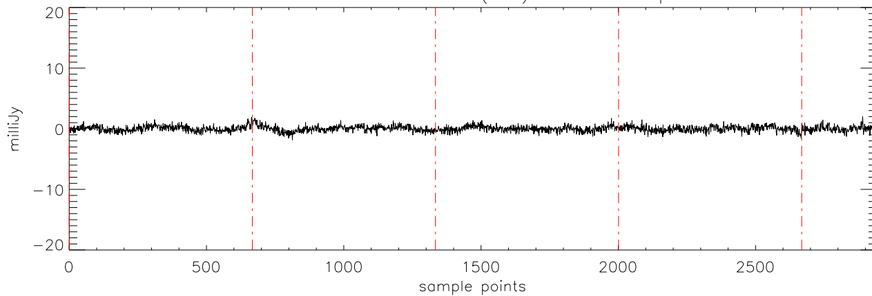
a2471 HD10697 20dec10 (AST) StokesU freq:4750.
