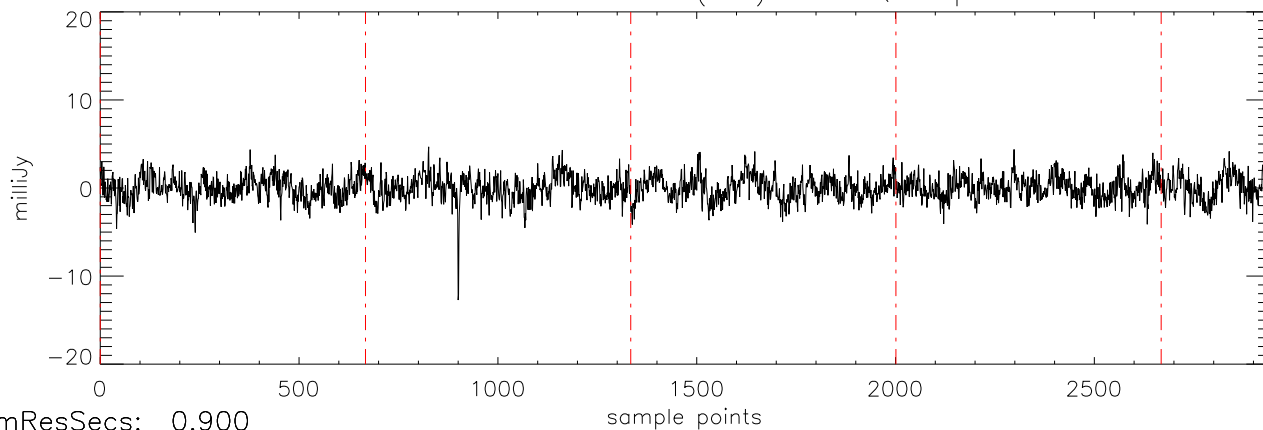
a2471 HD10697 20dec10 (AST) StokesQ freq:5034.
