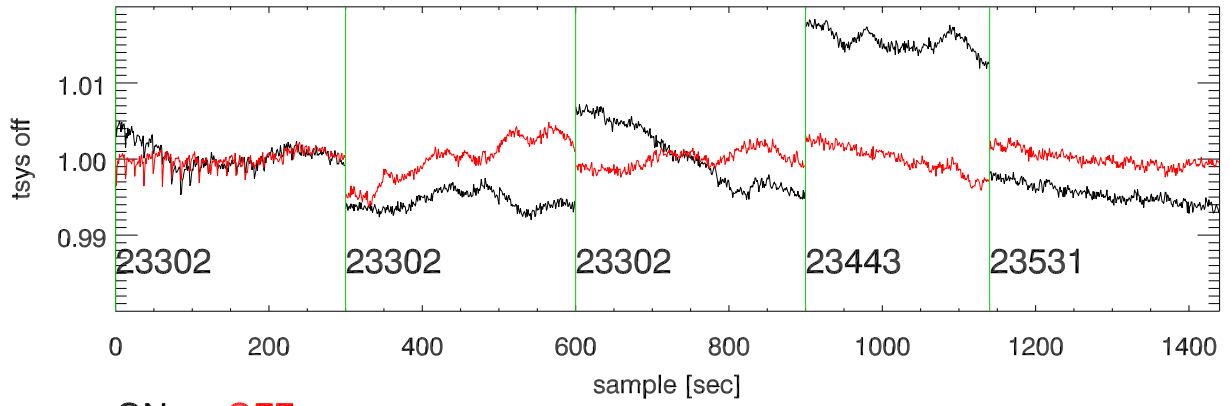
18mar11 a2335 on,offs overplotted. band 1 PoIA
