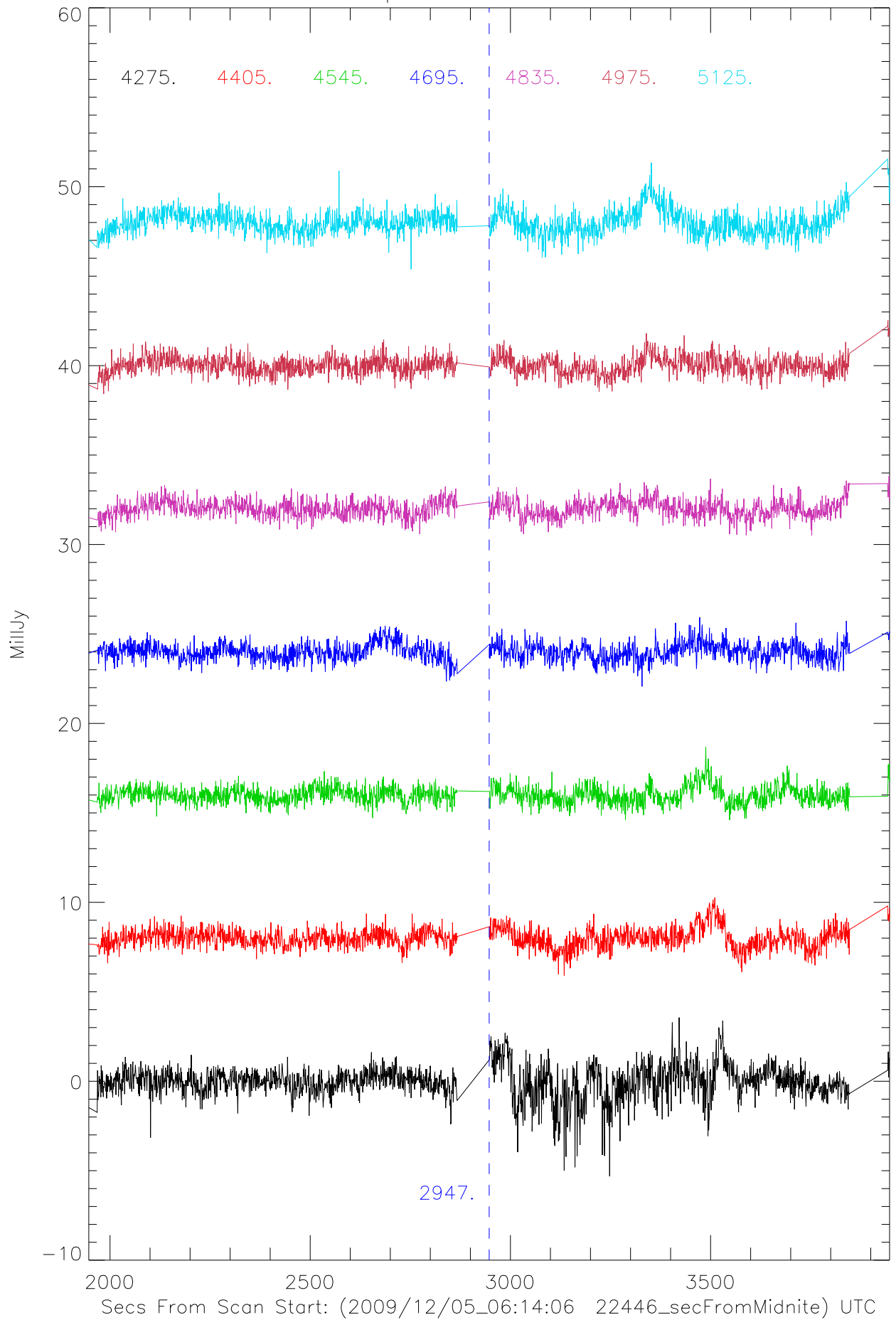
04dec09 cband blowup stokes V TP vs time for 2MASS0746
