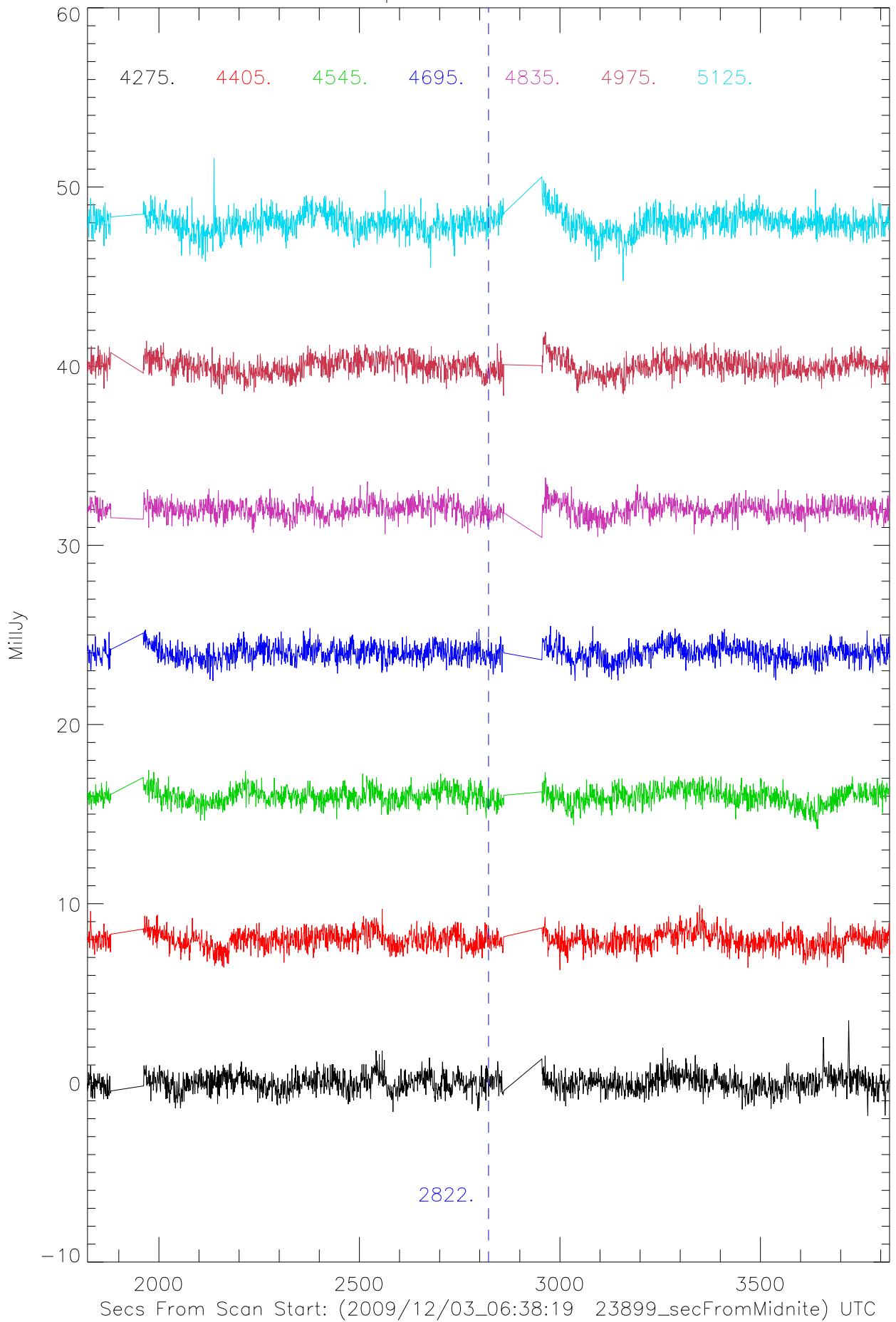
02dec09 cband blowup stokes V TP vs time for 2MASS0746
