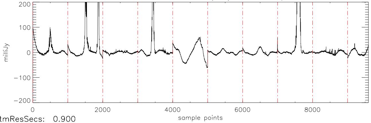
a2430 2MASS0036 02dec09 (AST) StokesI freq:4405.
