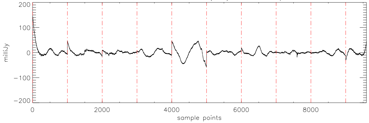
a2430 2MASS0036 02dec09 (AST) StokesI freq:5125.
