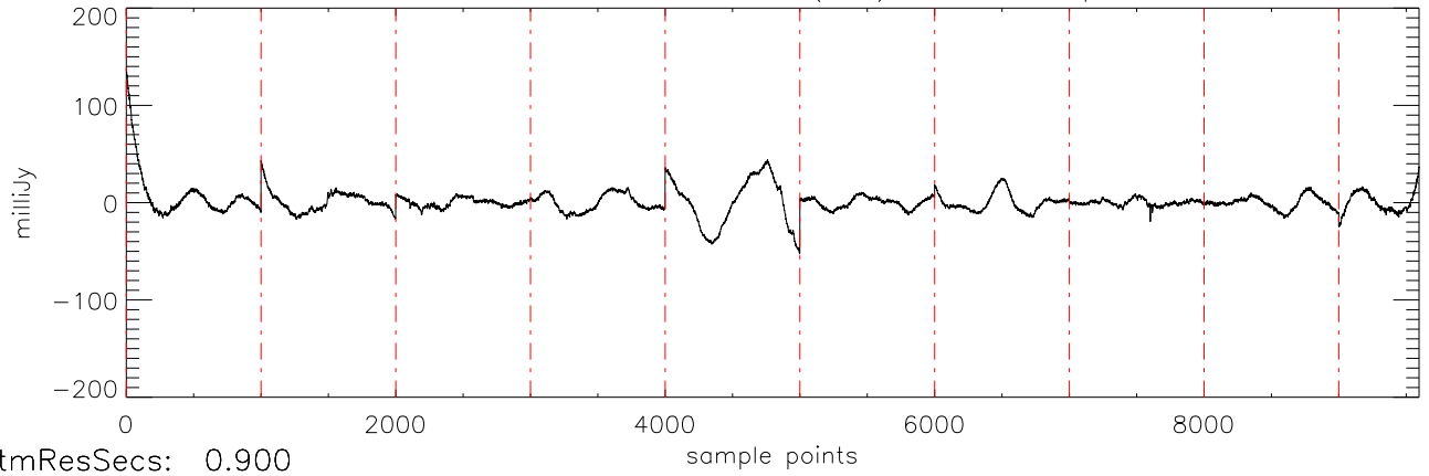
a2430 2MASS0036 02dec09 (AST) StokesI freq:4975.
