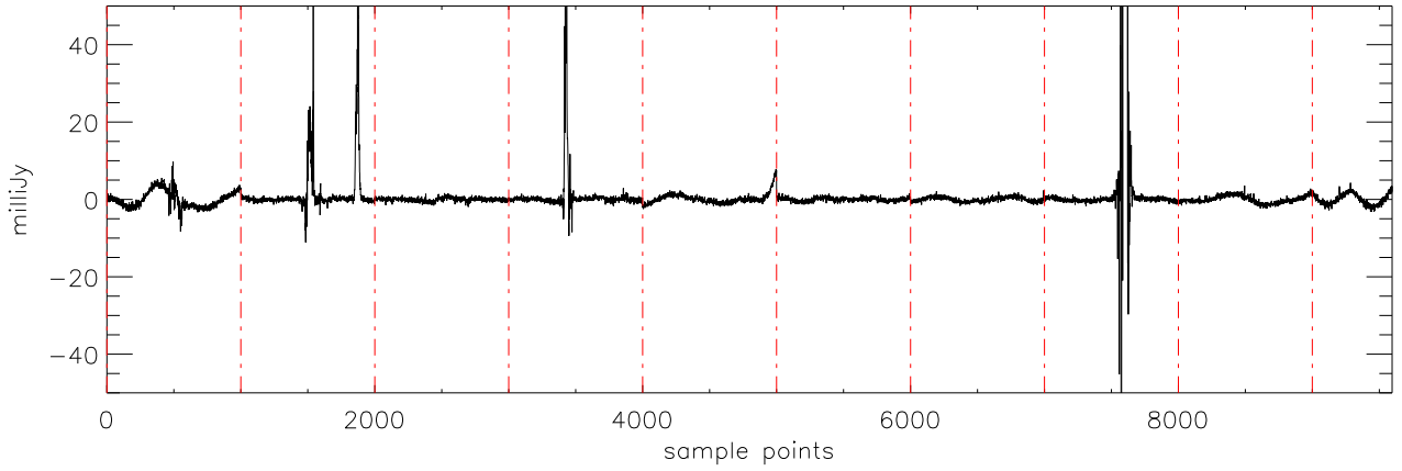
a2430 2MASS0036 02dec09 (AST) StokesU freq:4545.
