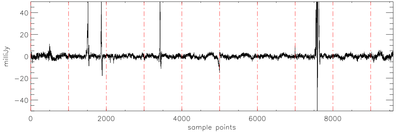
a2430 2MASS0036 02dec09 (AST) StokesQ freq:4545.
