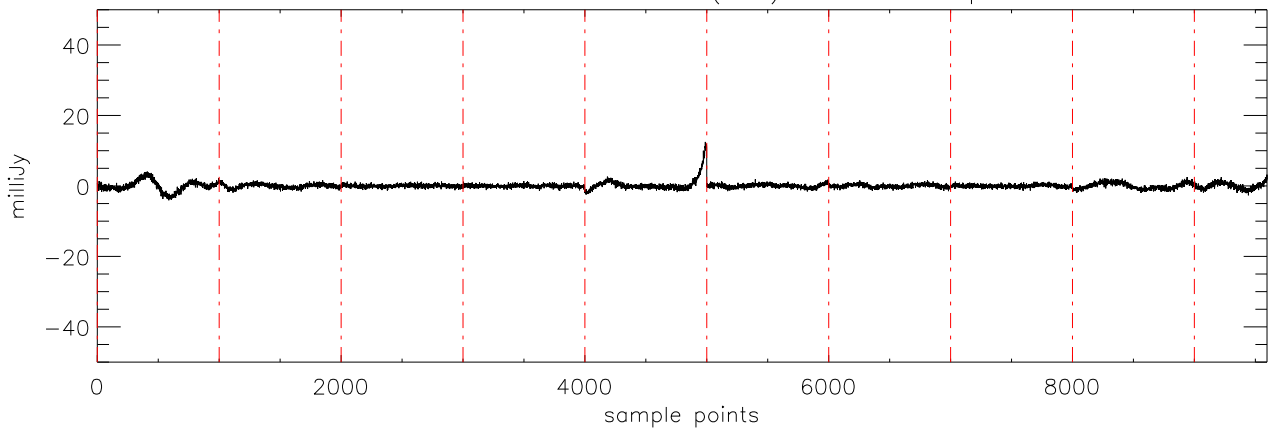
a2430 2MASS0036 02dec09 (AST) StokesU freq:4695.
