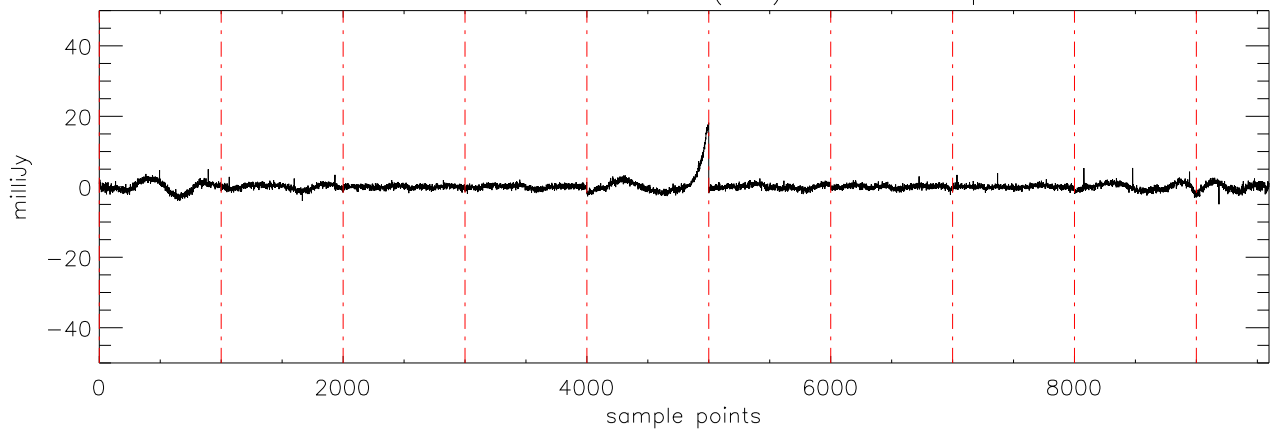
a2430 2MASS0036 02dec09 (AST) StokesU freq:5125.
