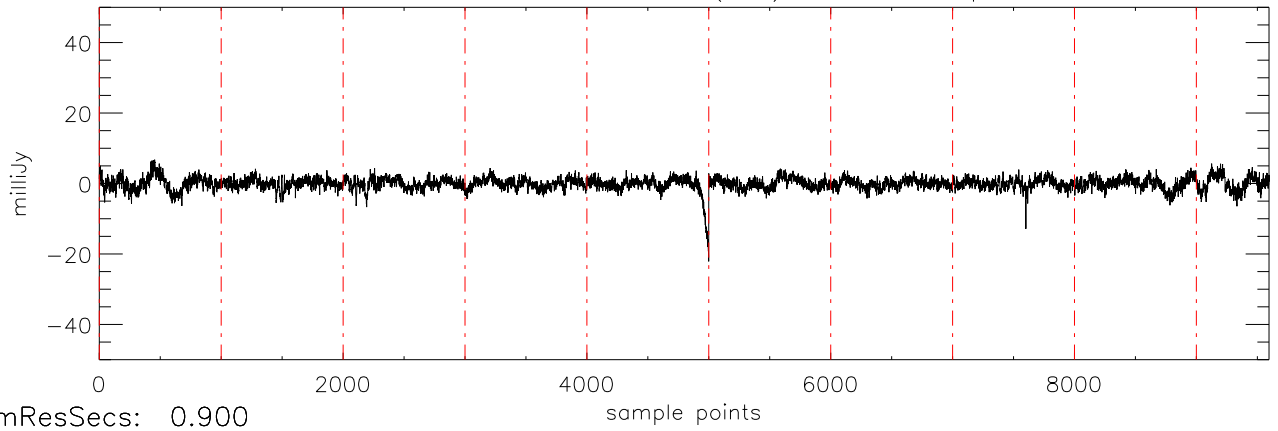
a2430 2MASS0036 02dec09 (AST) StokesQ freq:4975.
