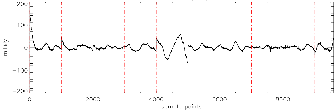
a2430 2MASS0036 02dec09 (AST) StokesI freq:5125.
