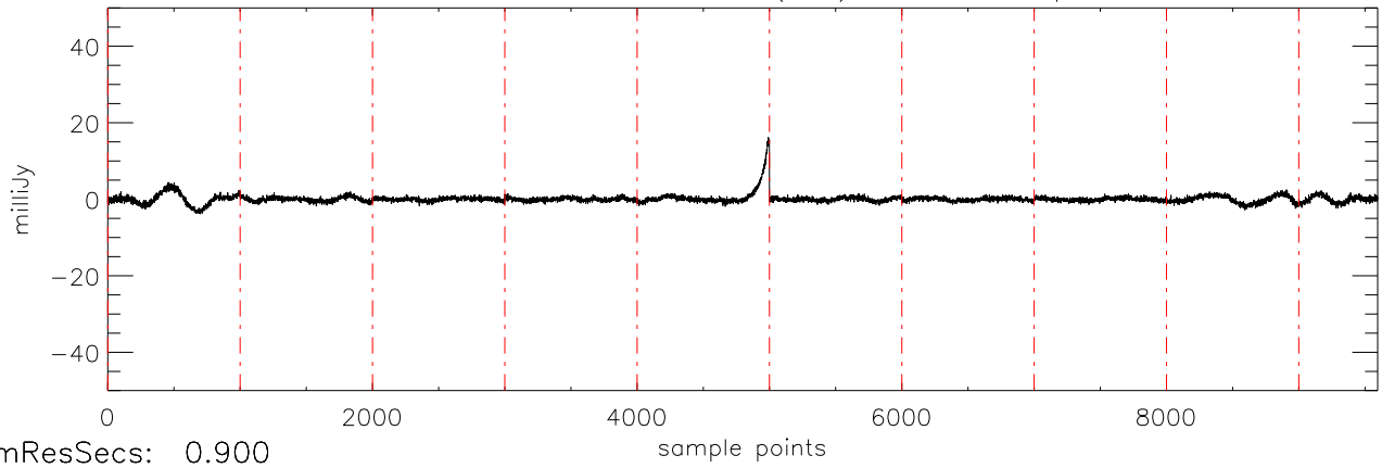
a2430 2MASS0036 02dec09 (AST) StokesU freq:4975.
