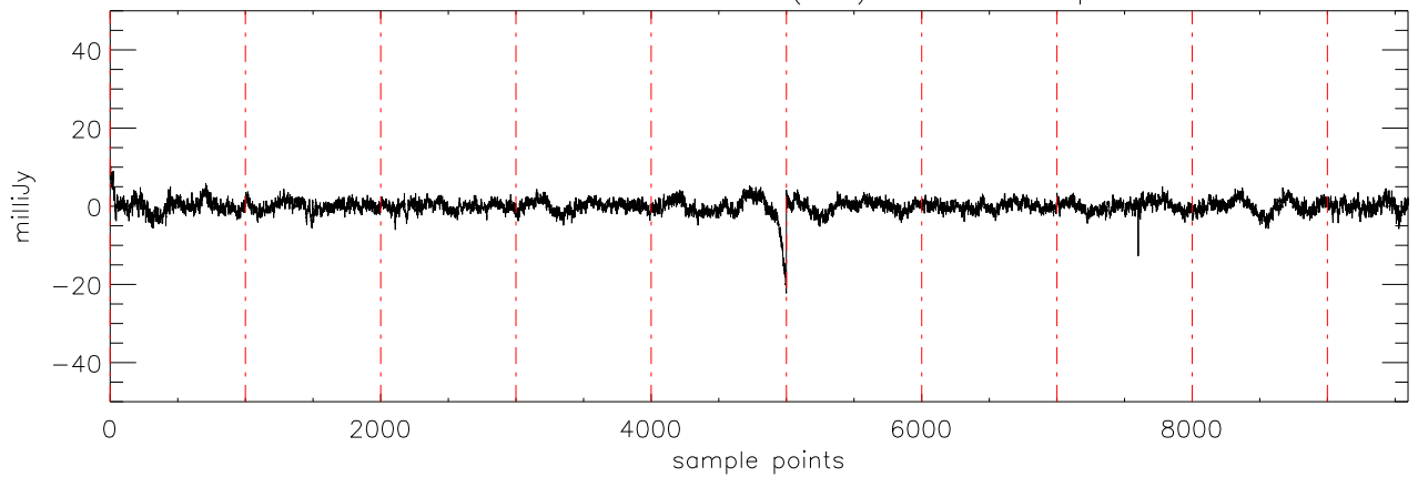
a2430 2MASS0036 02dec09 (AST) StokesQ freq:4695.
