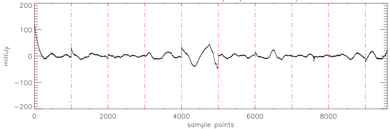
a2430 2MASS0036 02dec09 (AST) StokesI freq:4695.
