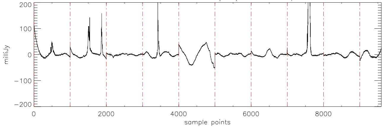
a2430 2MASS0036 02dec09 (AST) StokesI freq:4545.
