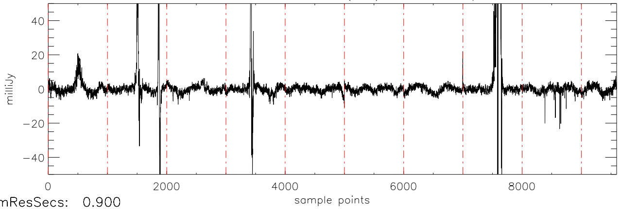
a2430 2MASS0036 02dec09 (AST) StokesQ freq:4405.
