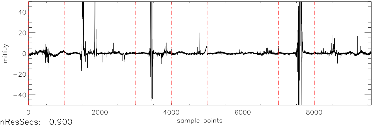
a2430 2MASS0036 02dec09 (AST) StokesU freq:4405.
