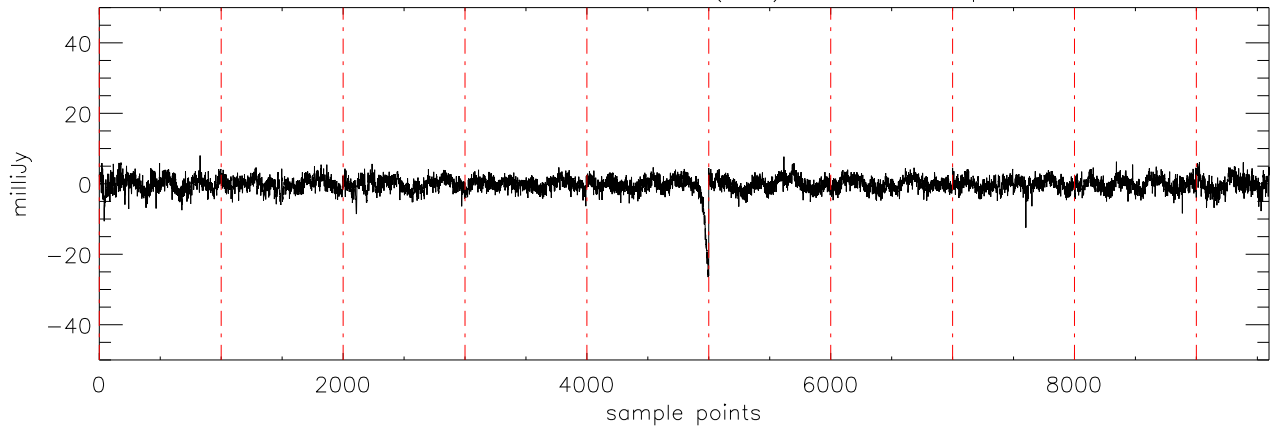
a2430 2MASS0036 02dec09 (AST) StokesQ freq:5125.
