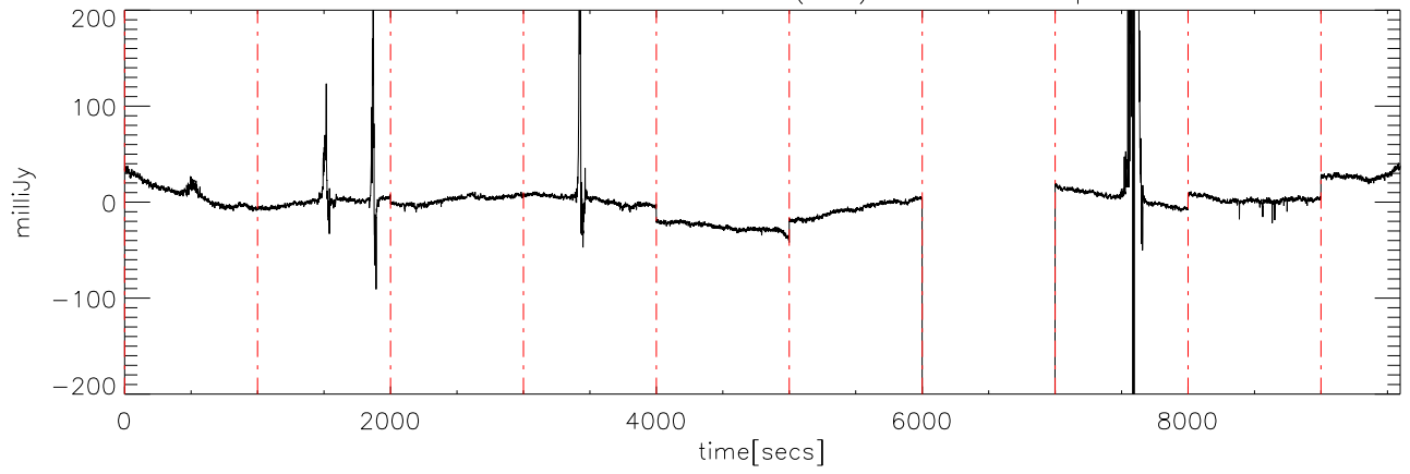
a2430 2MASS0036 02dec09 (AST) StokesQ freq:4405.
