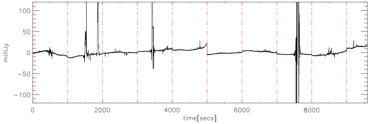
a2430 2MASS0036 02dec09 (AST) StokesU freq:4405.
