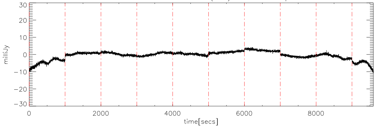
a2430 2MASS0036 02dec09 (AST) StokesV freq:4695.
