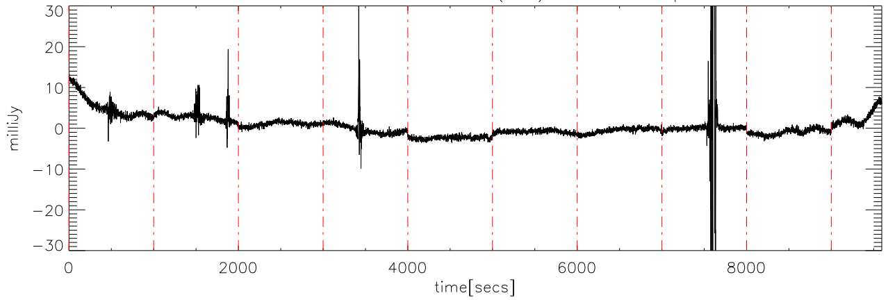
a2430 2MASS0036 02dec09 (AST) StokesV freq:4545.
