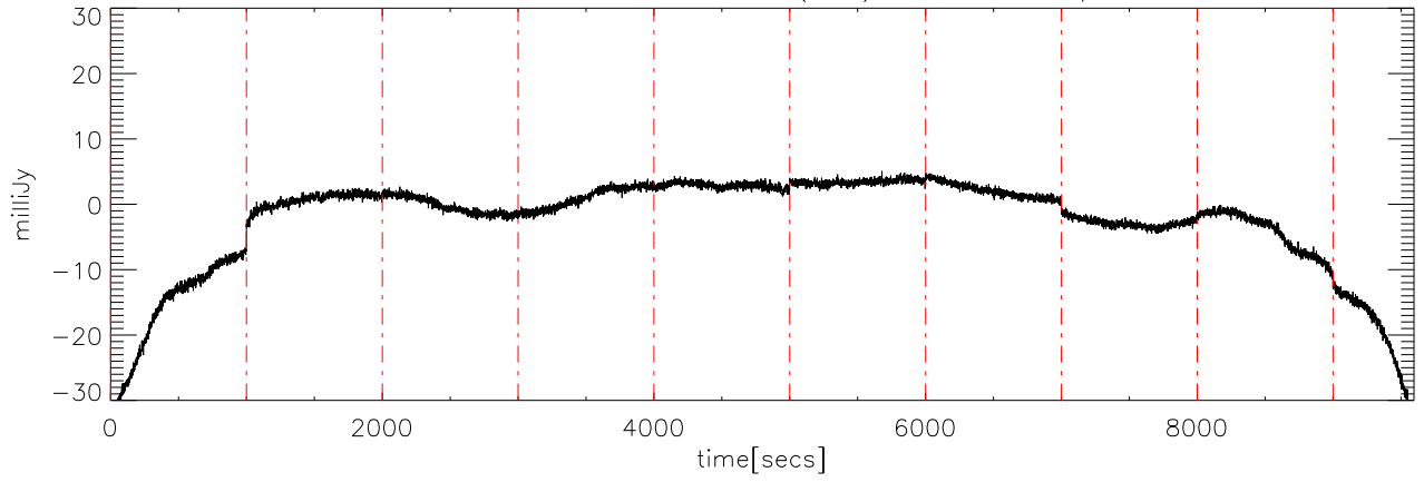
a2430 2MASS0036 02dec09 (AST) StokesV freq:4975.
