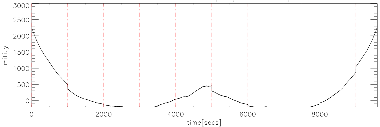
\alpha 2430 2MASS0036 02dec09 (AST) StokesI freq:4695.
