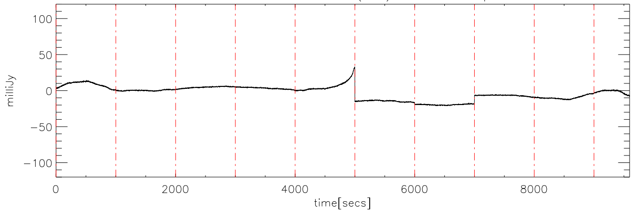
a2430 2MASS0036 02dec09 (AST) StokesU freq:5125.
