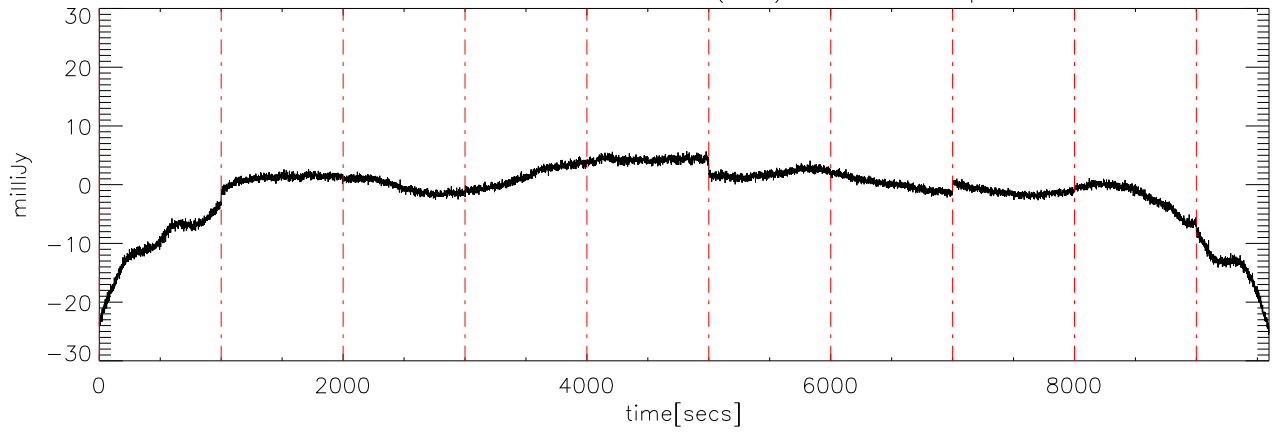
a2430 2MASS0036 02dec09 (AST) StokesV freq:5125.
