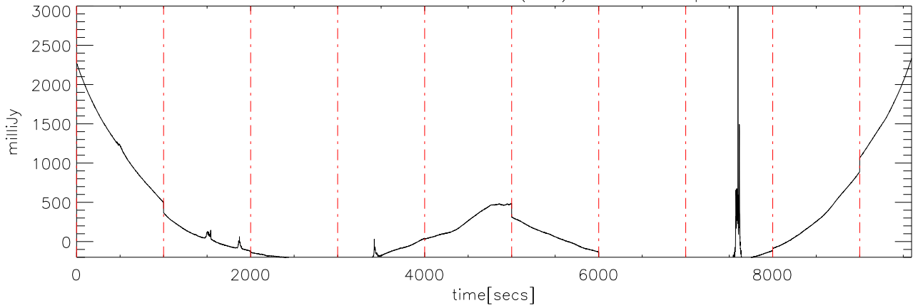
\alpha 2430 2MASS0036 02dec09 (AST) StokesI freq:4545.
