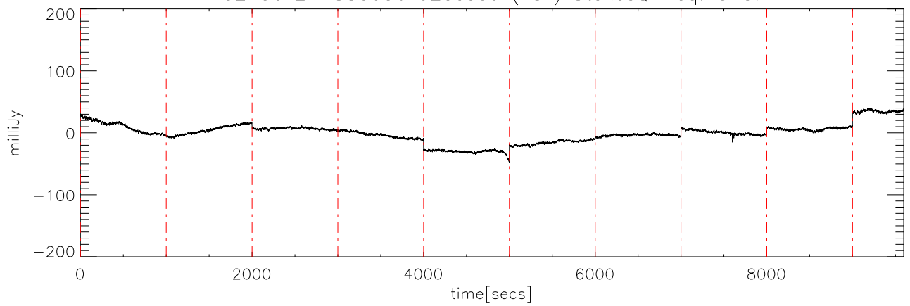
a2430 2MASS0036 02dec09 (AST) StokesQ freq:4695.
