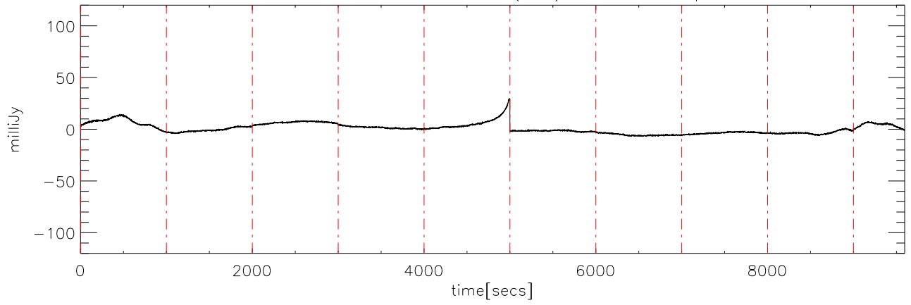
a2430 2MASS0036 02dec09 (AST) StokesU freq:4975.
