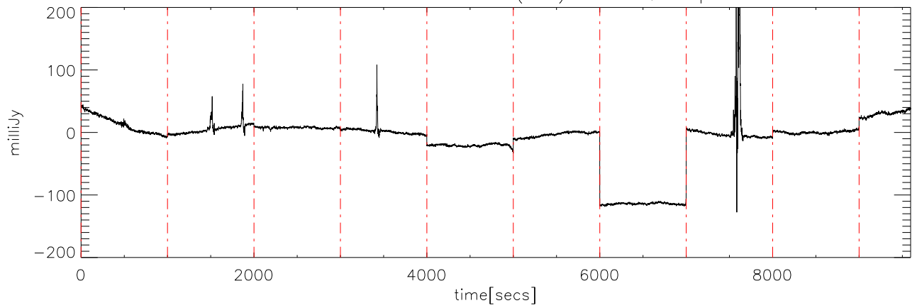
a2430 2MASS0036 02dec09 (AST) StokesQ freq:4545.
