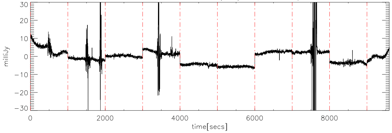
a2430 2MASS0036 02dec09 (AST) StokesV freq:4405.
