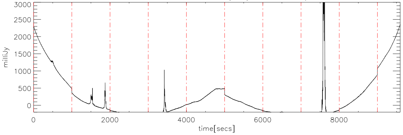
\alpha 2430 2MASS0036 02dec09 (AST) StokesI freq:4405.
