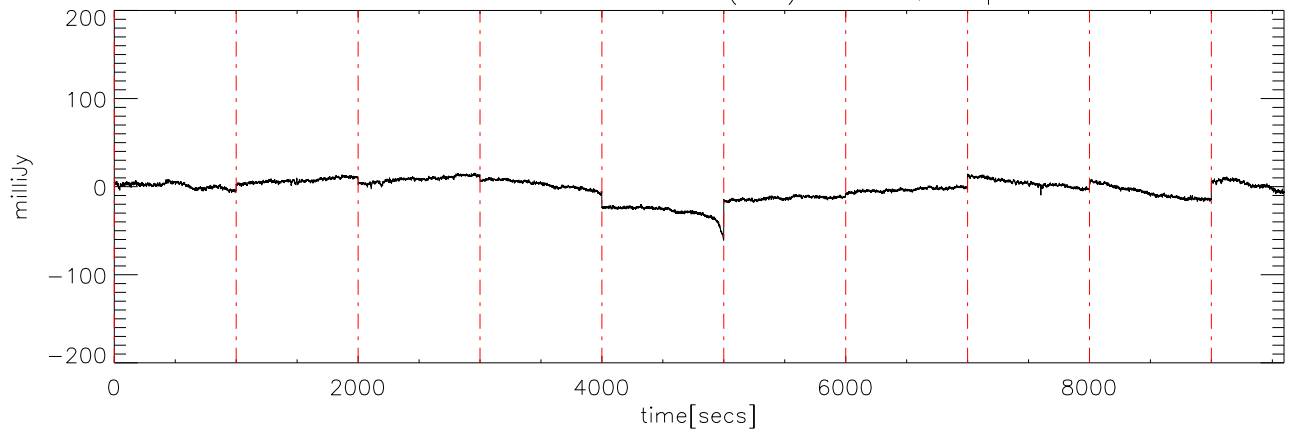
a2430 2MASS0036 02dec09 (AST) StokesQ freq:5125.
