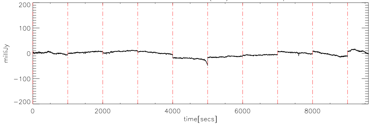
a2430 2MASS0036 02dec09 (AST) StokesQ freq:4975.
