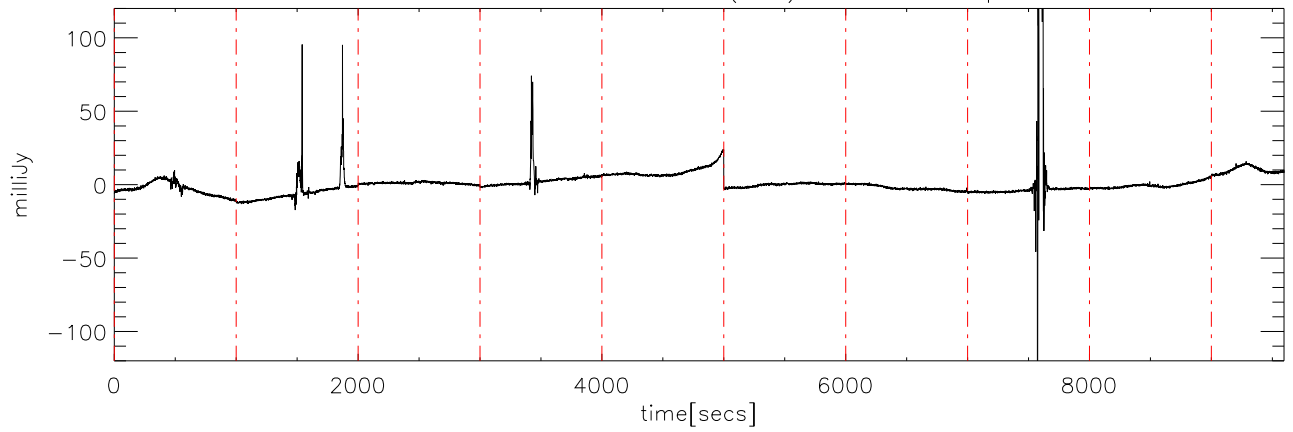
a2430 2MASS0036 02dec09 (AST) StokesU freq:4545.
