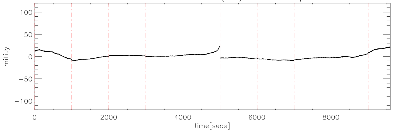
a2430 2MASS0036 02dec09 (AST) StokesU freq:4695.
