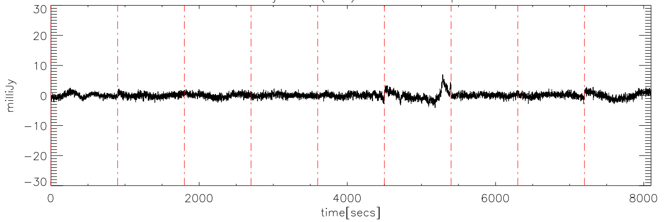
a2414 13jun09 (AST) StokesV freq:5125.
