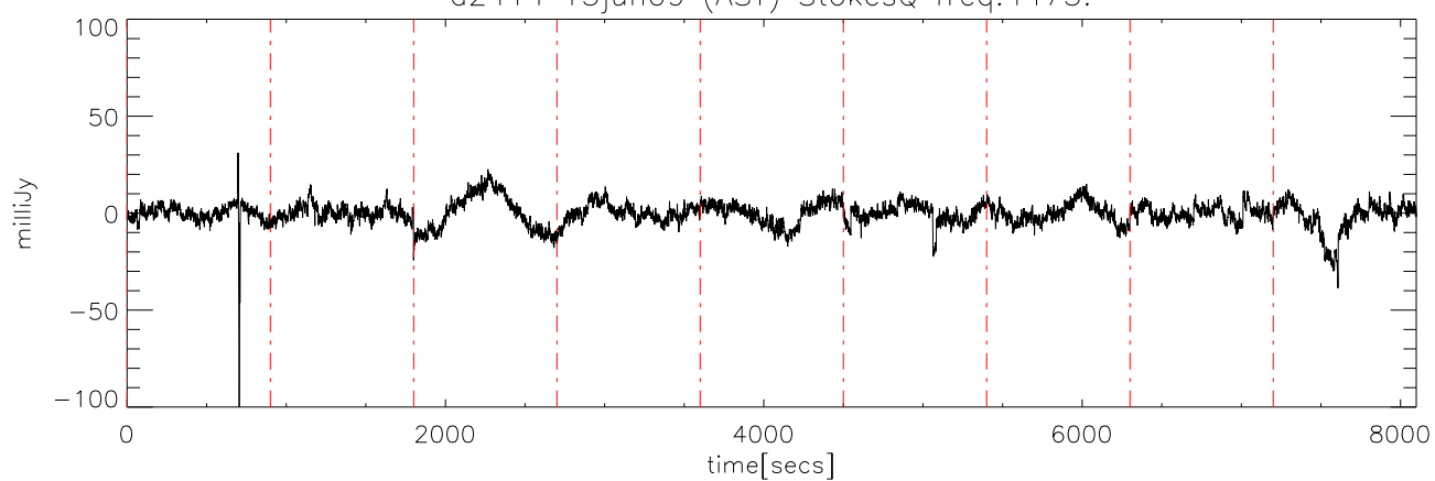
a2414 13jun09 (AST) StokesQ freq:4600.
