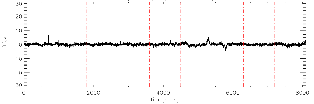
a2414 13jun09 (AST) StokesV freq:4600.
