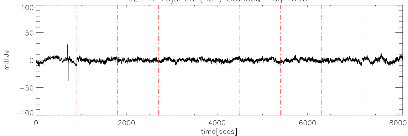
a2414 13jun09 (AST) StokesQ freq:4725.
