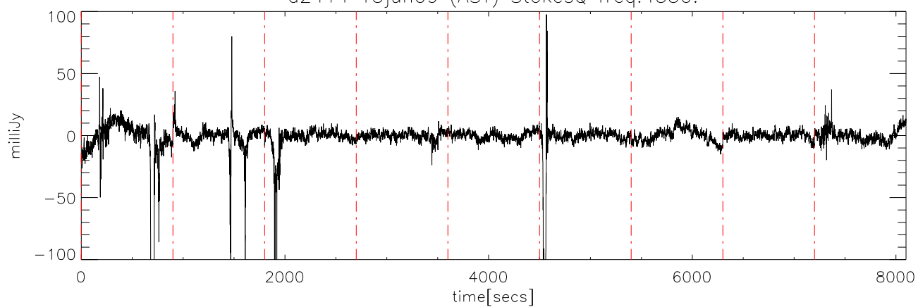
a2414 13jun09 (AST) StokesQ freq:4475.
