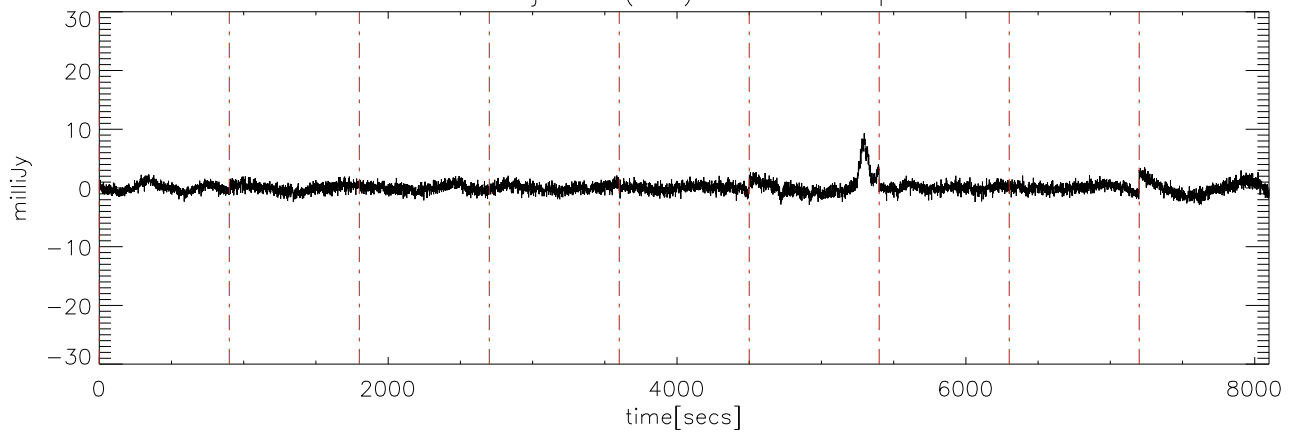
a2414 13jun09 (AST) StokesV freq:4725.
