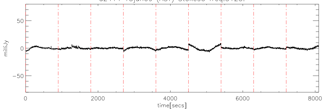
a2414 13jun09 (AST) StokesU freq:5250.
