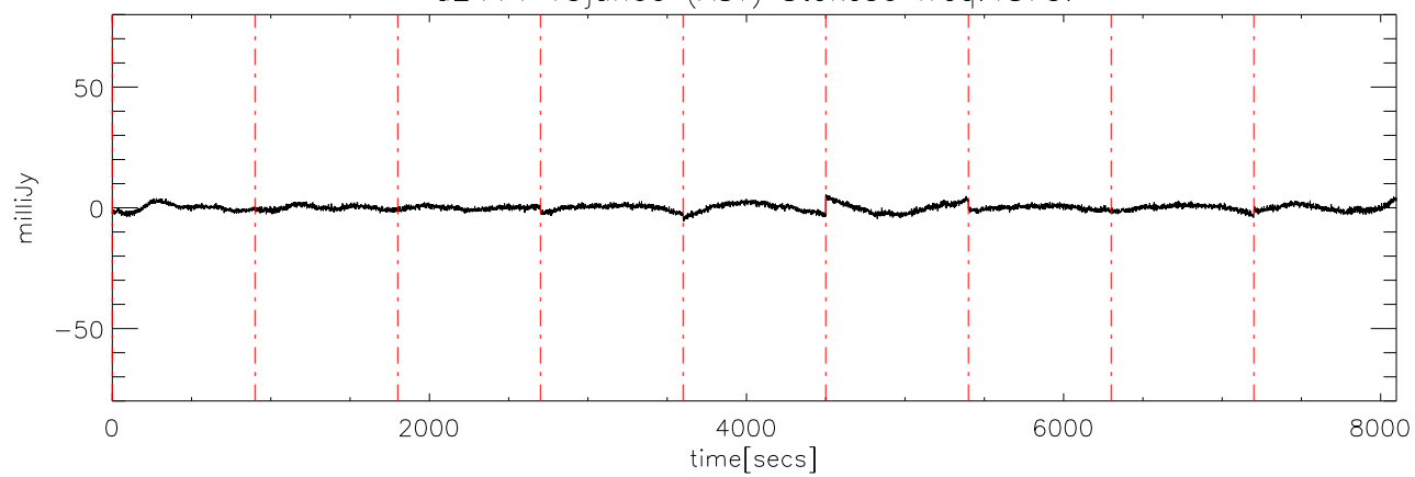
a2414 13jun09 (AST) StokesU freq:5000.
