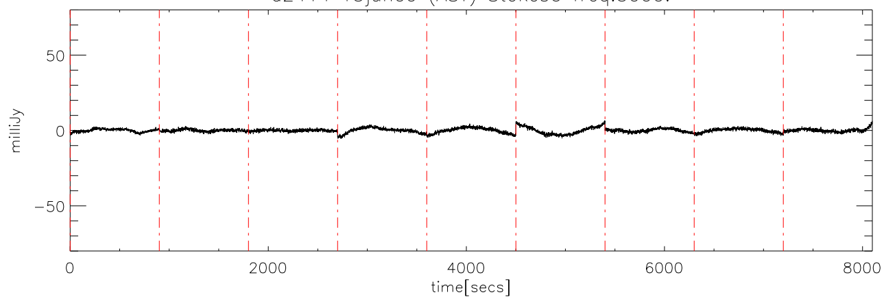
a2414 13jun09 (AST) StokesU freq:5125.
