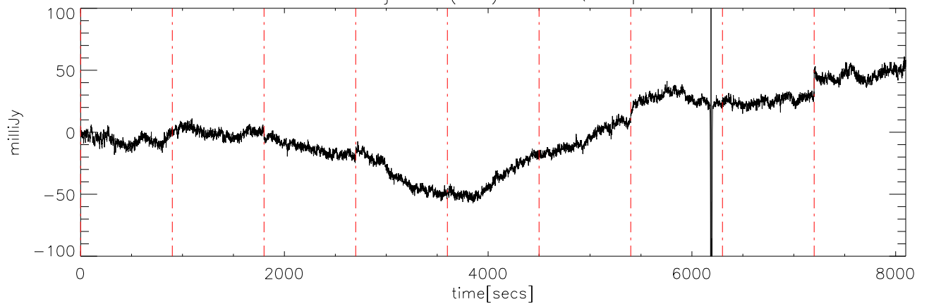
a2414 10jun09 (AST) StokesQ freq:4525.
