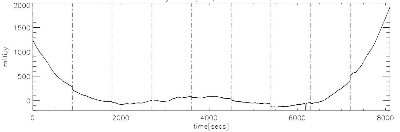
a2414 10jun09 (AST) StokesI freq:4925.
