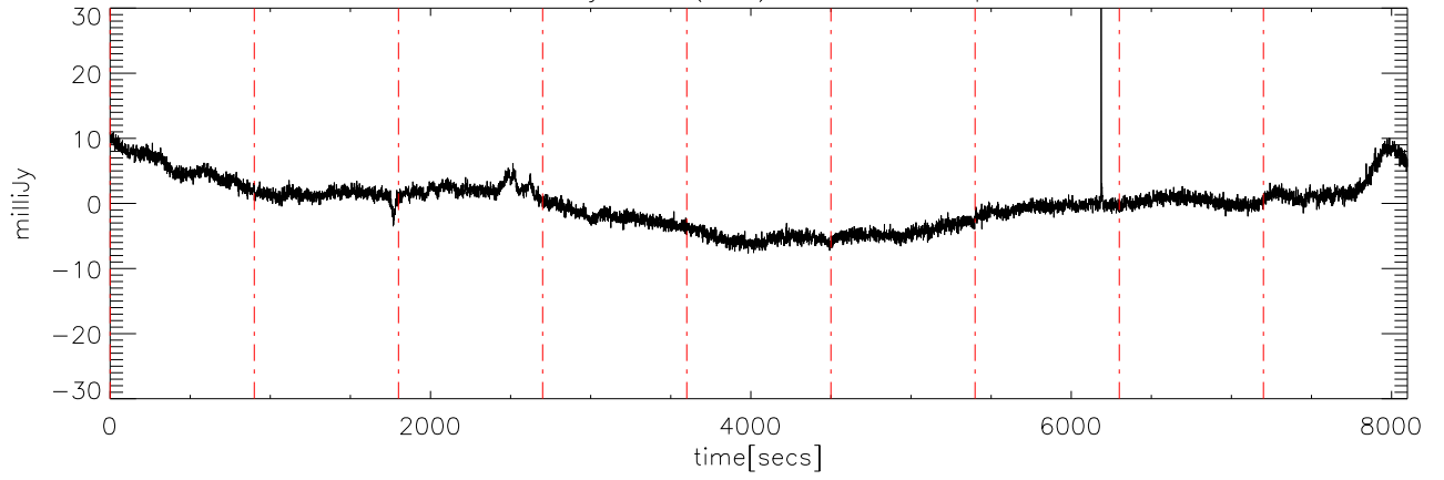
a2414 10jun09 (AST) StokesV freq:4800.
