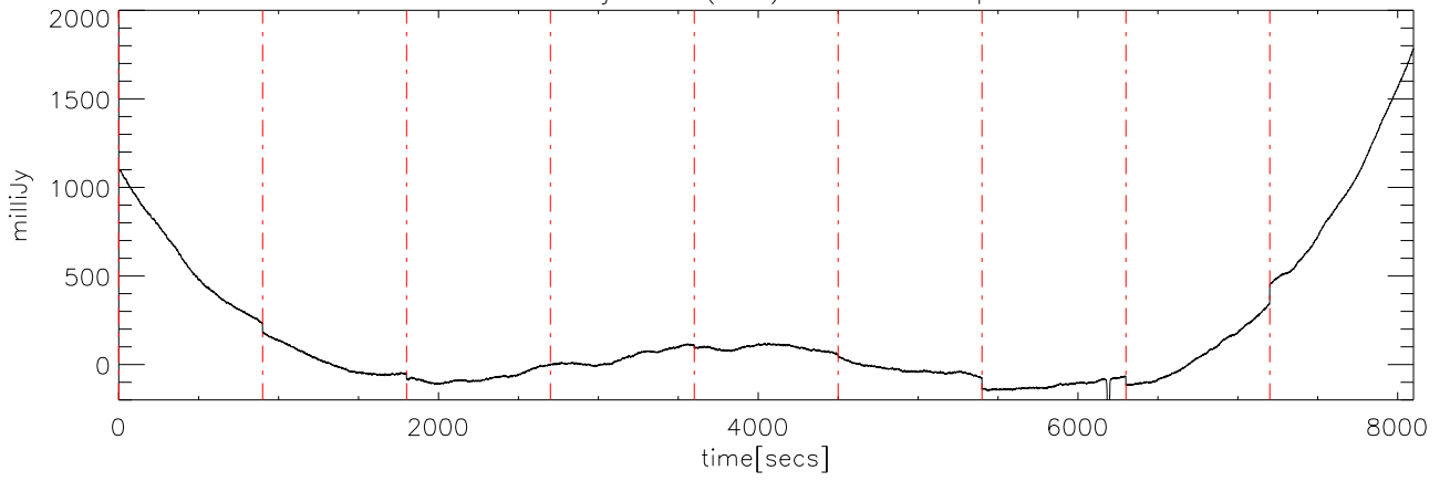
a2414 10jun09 (AST) StokesI freq:4800.
