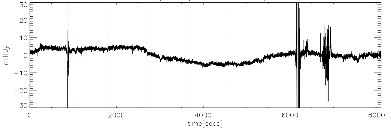
a2414 10jun09 (AST) StokesV freq:4400.
