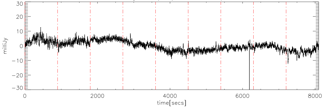
a2414 10jun09 (AST) StokesV freq:4275.
