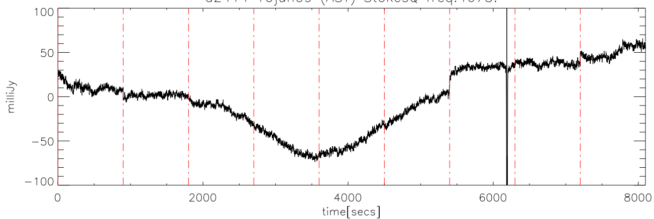
a2414 10jun09 (AST) StokesQ freq:4800.
