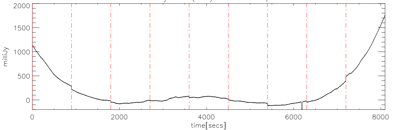
a2414 10jun09 (AST) StokesI freq:4525.
