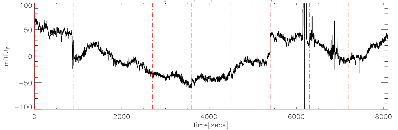
a2414 10jun09 (AST) StokesQ freq:4400.
