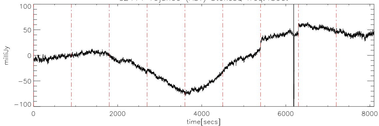
a2414 10jun09 (AST) StokesQ freq:4925.
