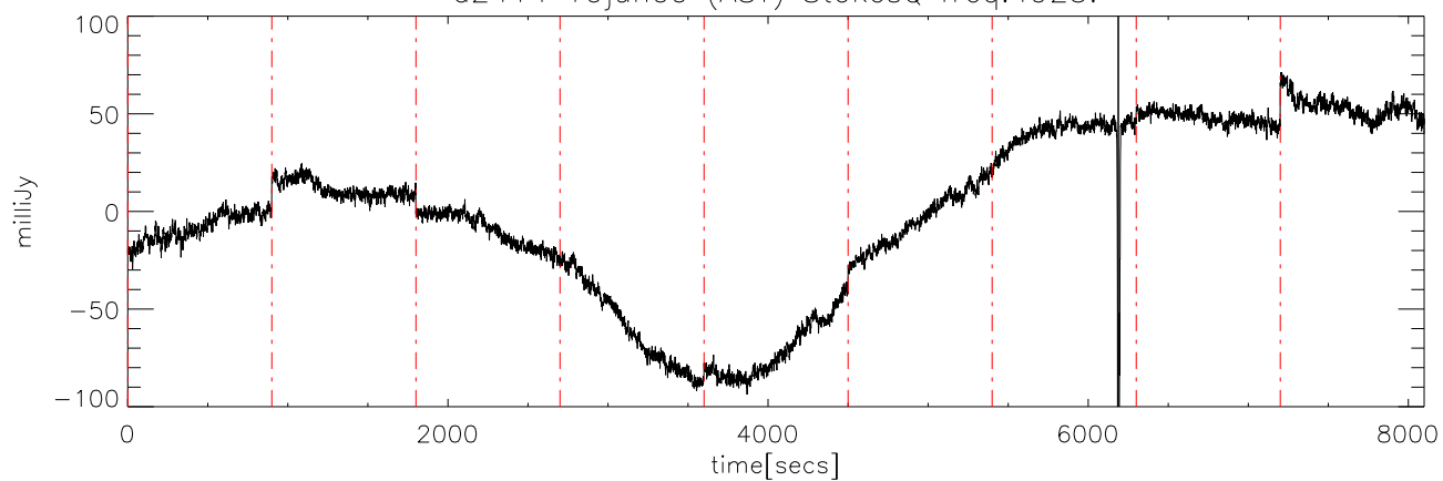
a2414 10jun09 (AST) StokesQ freq:5050.
