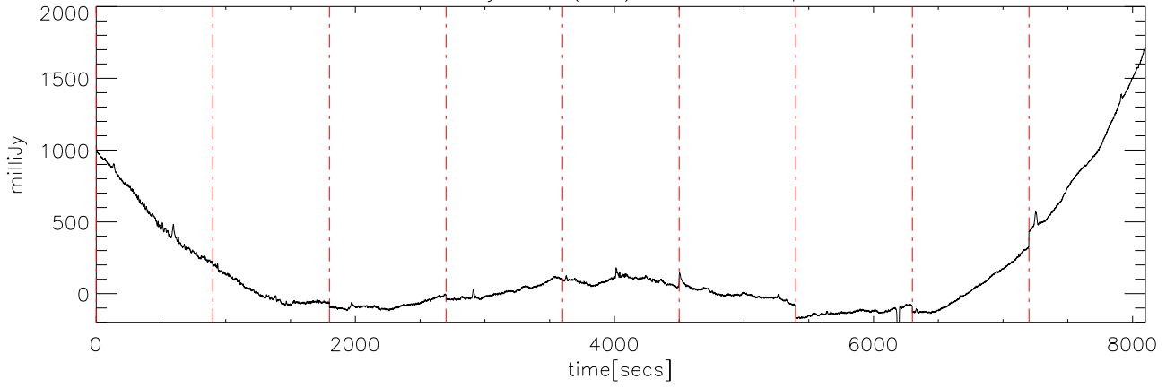
a2414 10jun09 (AST) StokesI freq:4275.
