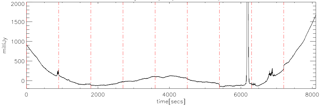
a2414 10jun09 (AST) StokesI freq:4400.
