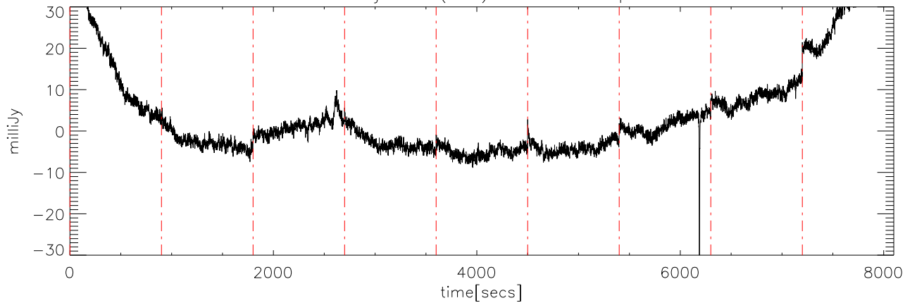
a2414 10jun09 (AST) StokesV freq:5050.
