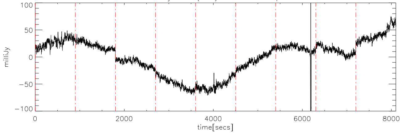
a2414 10jun09 (AST) StokesQ freq:4275.
