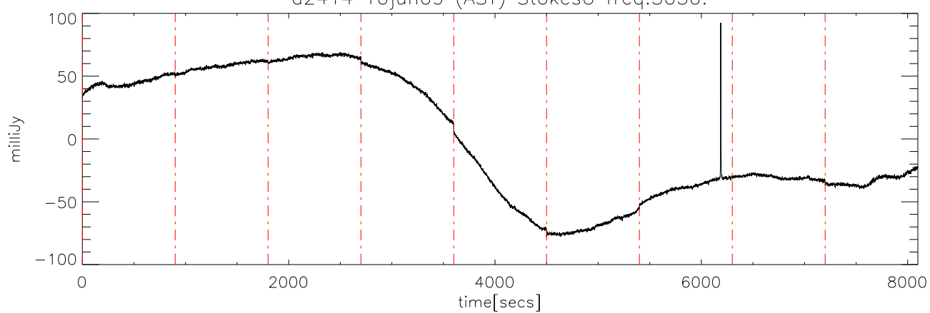
a2414 10jun09 (AST) StokesU freq:5050.
