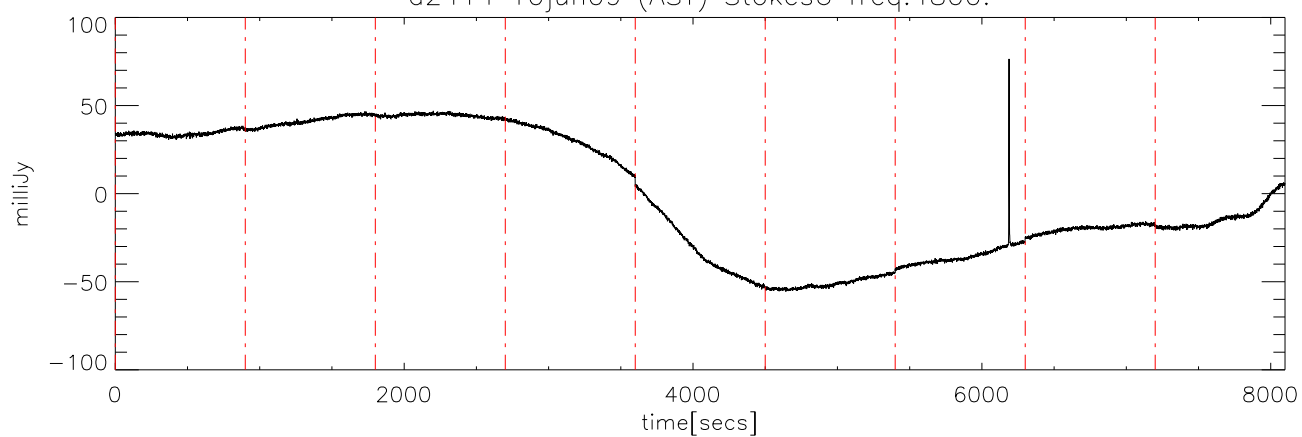
a2414 10jun09 (AST) StokesU freq:4925.
