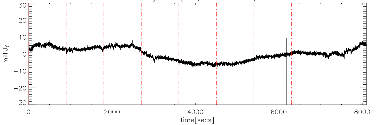
a2414 10jun09 (AST) StokesV freq:4525.
