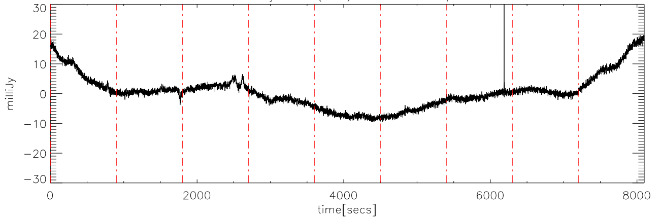
a2414 10jun09 (AST) StokesV freq:4925.
