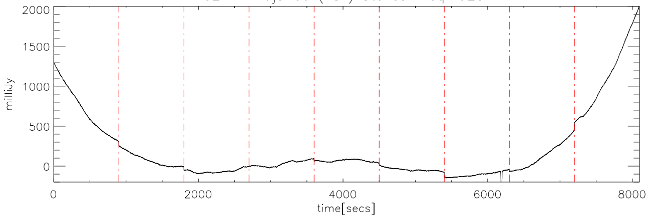
a2414 10jun09 (AST) StokesI freq:5050.
