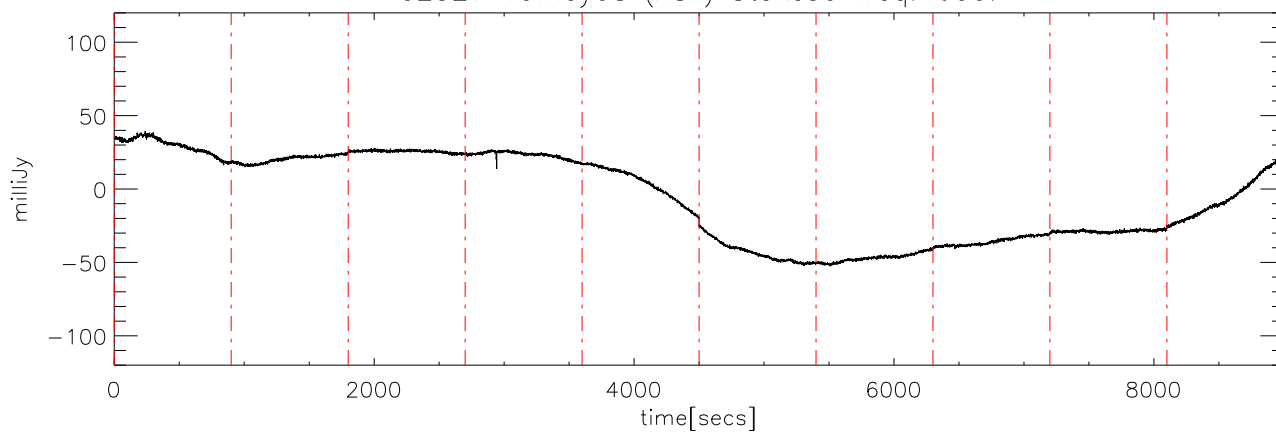
a2327 19may08 (AST) StokesU freq:4725.
