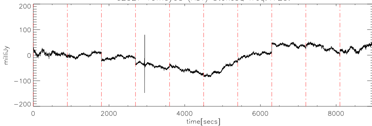
a2327 19may08 (AST) StokesQ freq:4725.
