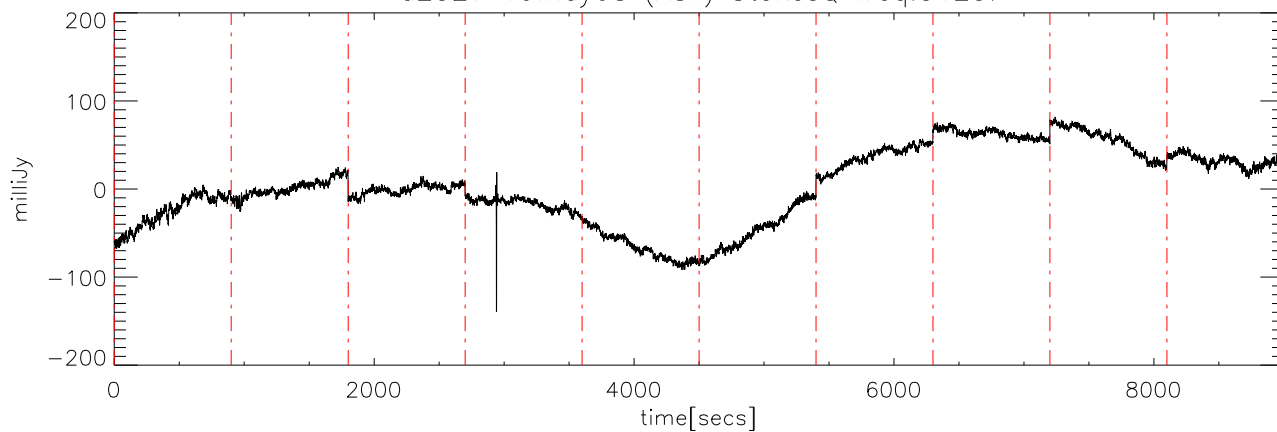
a2327 19may08 (AST) StokesQ freq:5250.
