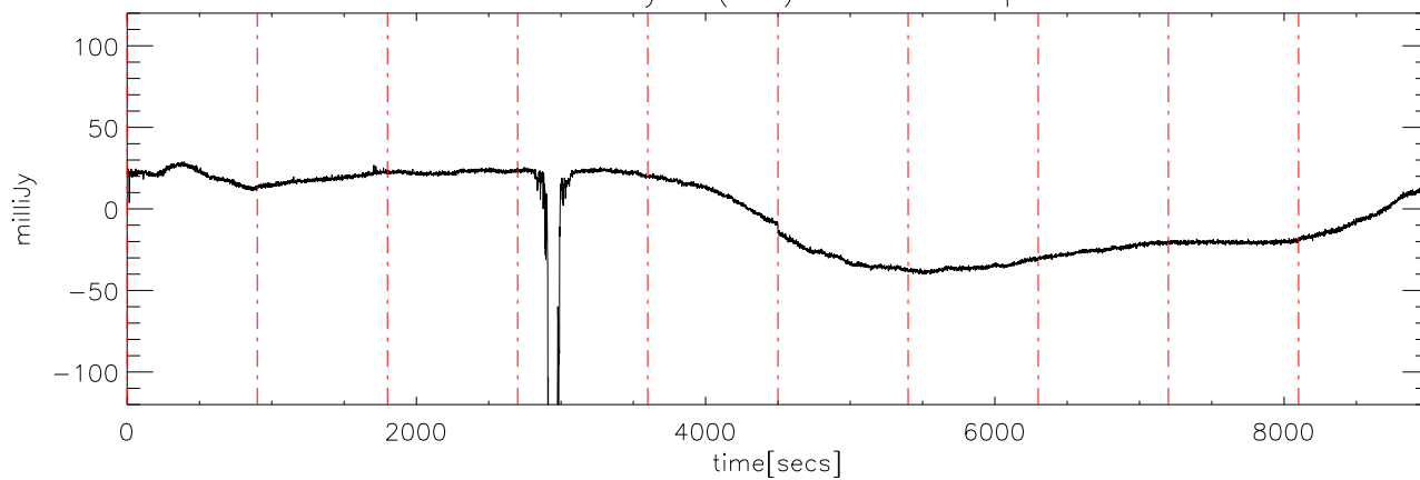
a2327 19may08 (AST) StokesU freq:4475.
