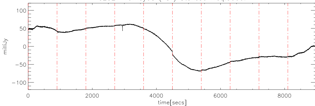
a2327 19may08 (AST) StokesU freq:5125.
