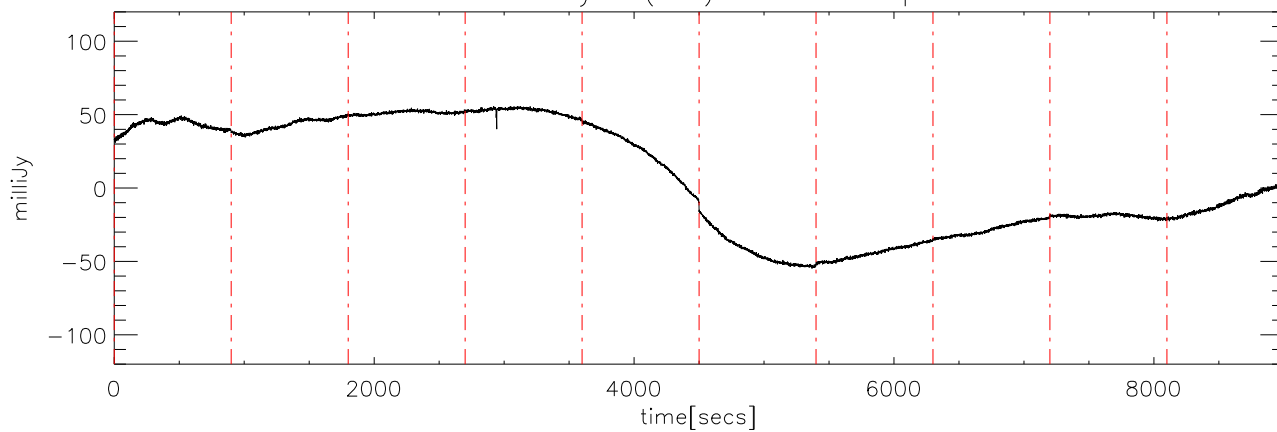
a2327 19may08 (AST) StokesU freq:5000.
