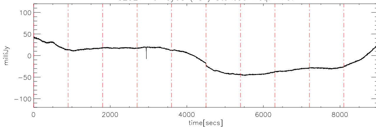
a2327 19may08 (AST) StokesU freq:4600.
