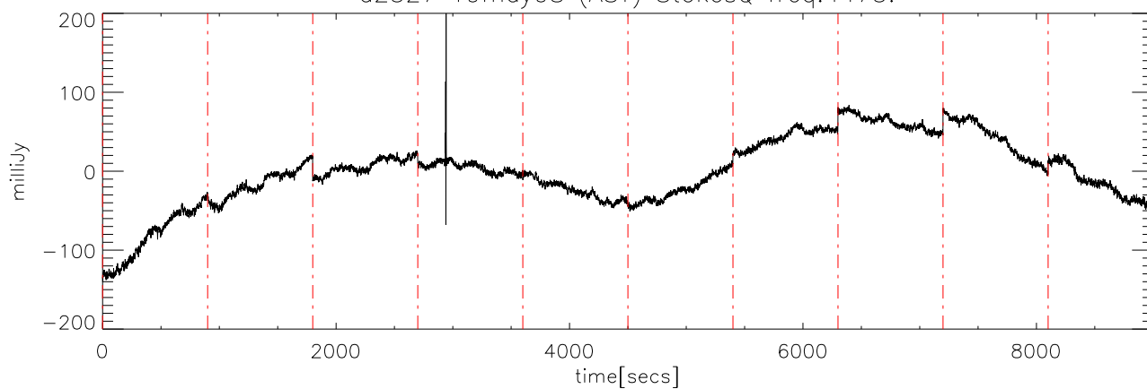
a2327 19may08 (AST) StokesQ freq:4600.
