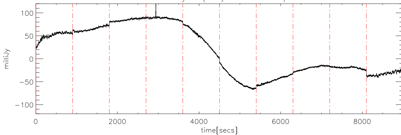
a2327 19may08 (AST) StokesU freq:5250.
