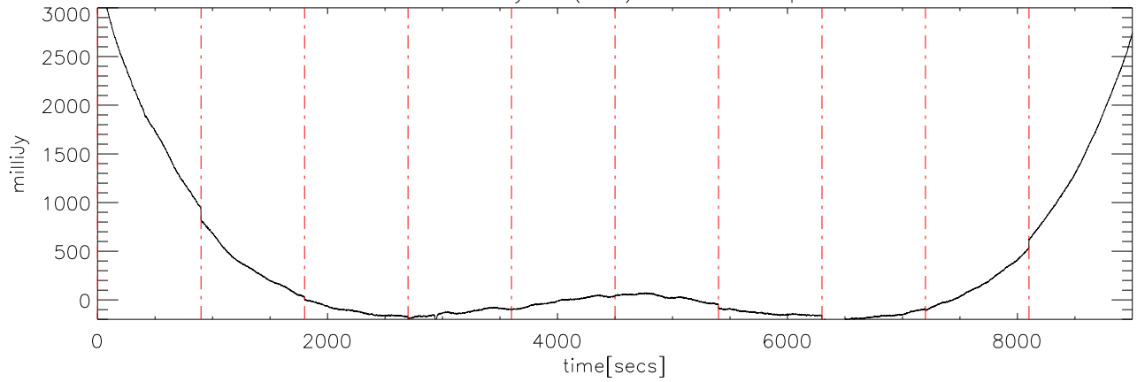
a2327 19may08 (AST) StokesI freq:5250.
