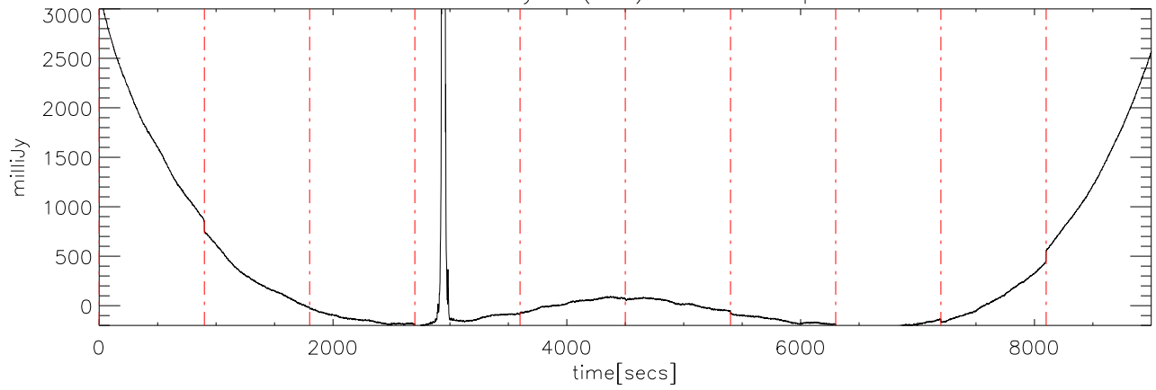
a2327 19may08 (AST) StokesI freq:4475.
