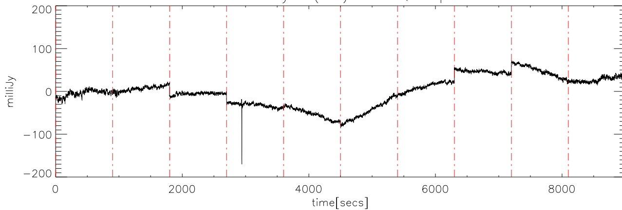
a2327 19may08 (AST) StokesQ freq:5000.
