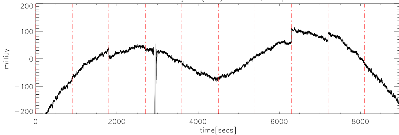
a2327 19may08 (AST) StokesQ freq:4475.
