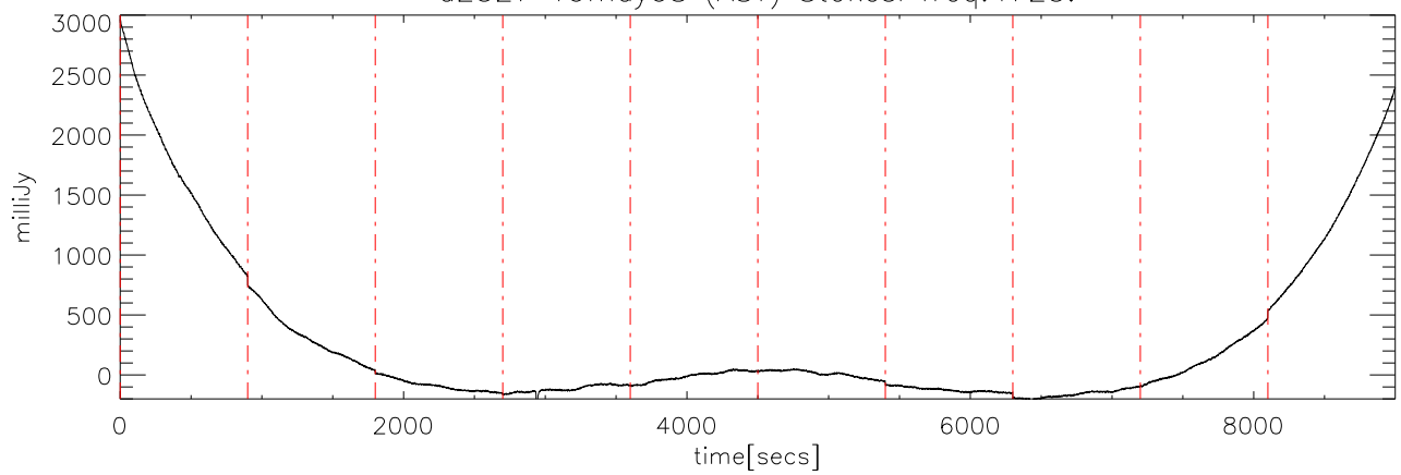
a2327 19may08 (AST) StokesI freq:4725.
