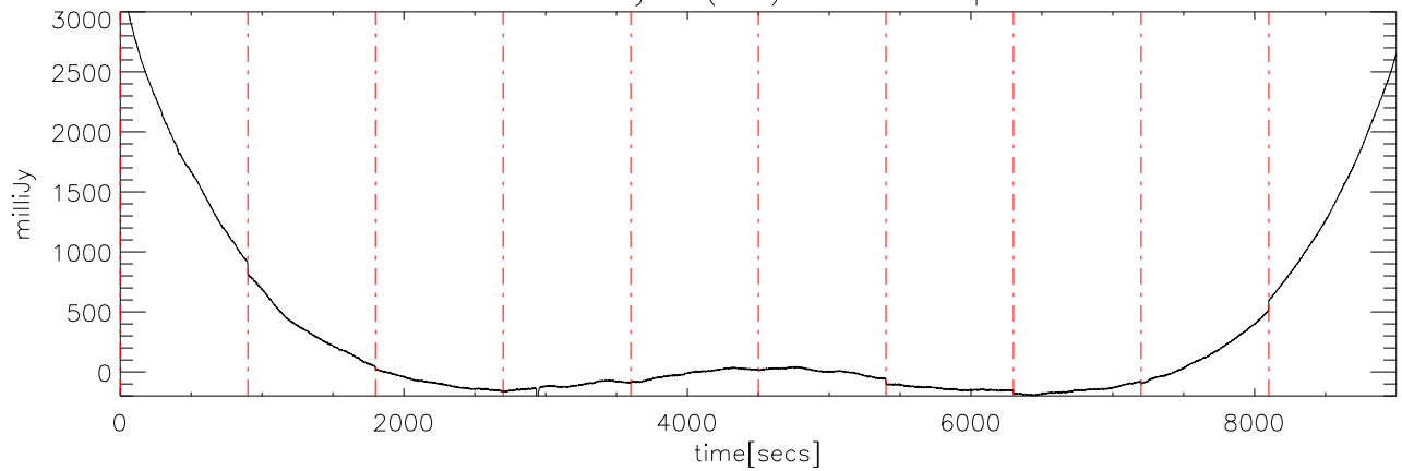
a2327 19may08 (AST) StokesI freq:5125.
