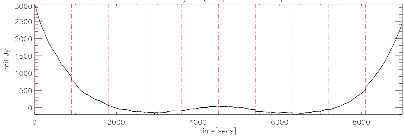
a2327 19may08 (AST) StokesI freq:4600.
