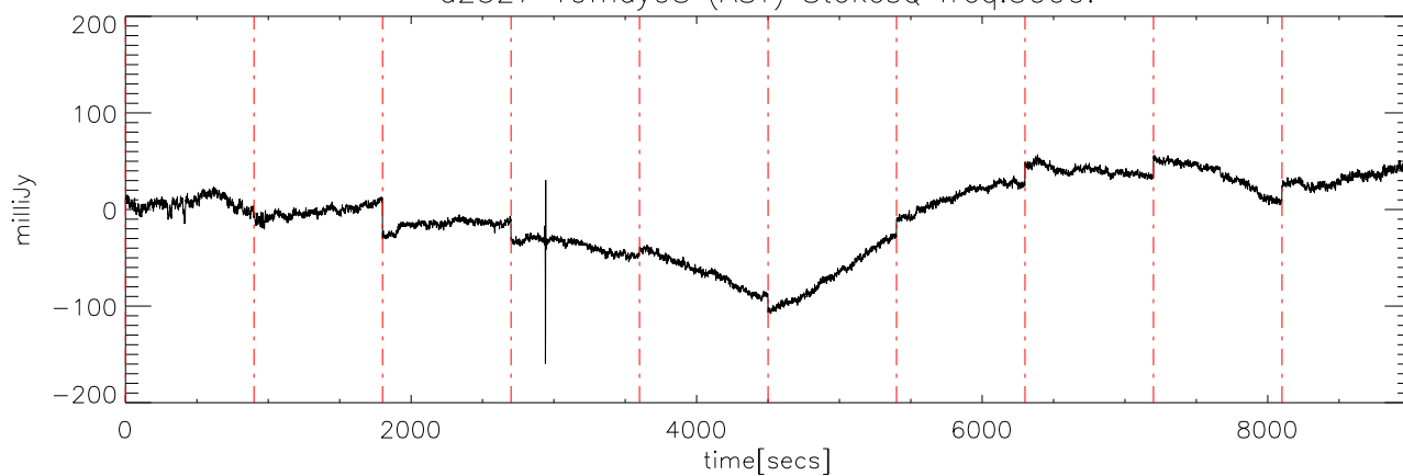
a2327 19may08 (AST) StokesQ freq:5125.
