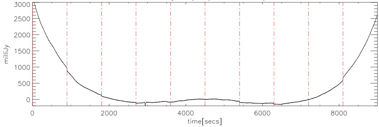
a2327 19may08 (AST) StokesI freq:5000.
