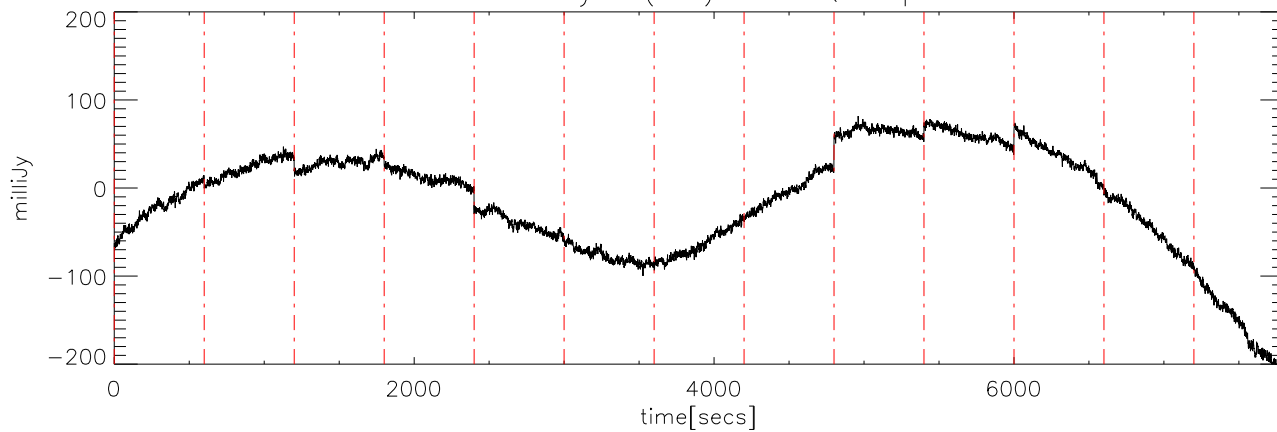
a2327 17may08 (AST) StokesQ freq:4475.
