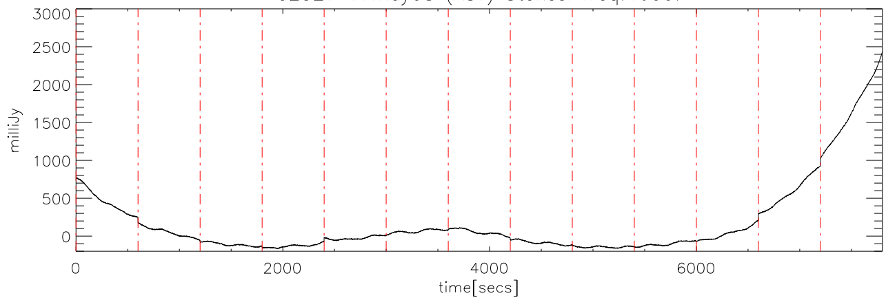
a2327 17may08 (AST) StokesI freq:4725.
