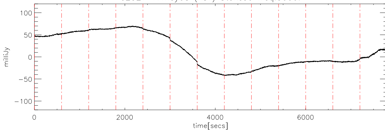
a2327 17may08 (AST) StokesU freq:5125.
