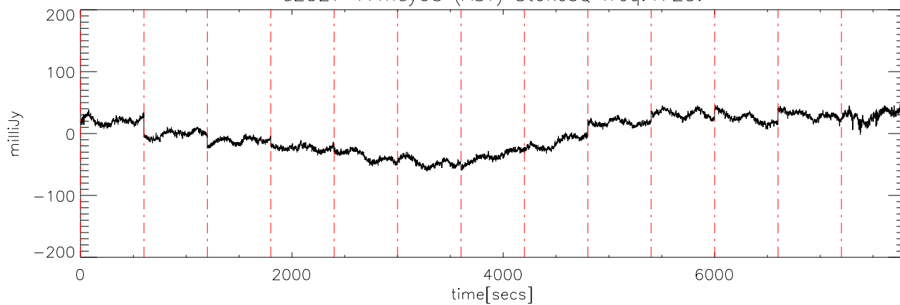
a2327 17may08 (AST) StokesQ freq:4725.
