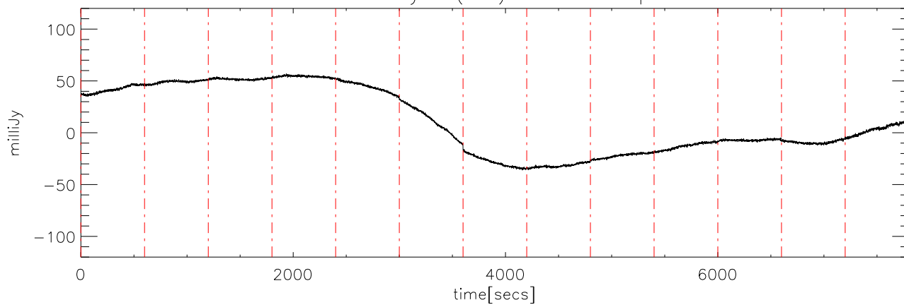
a2327 17may08 (AST) StokesU freq:5000.
