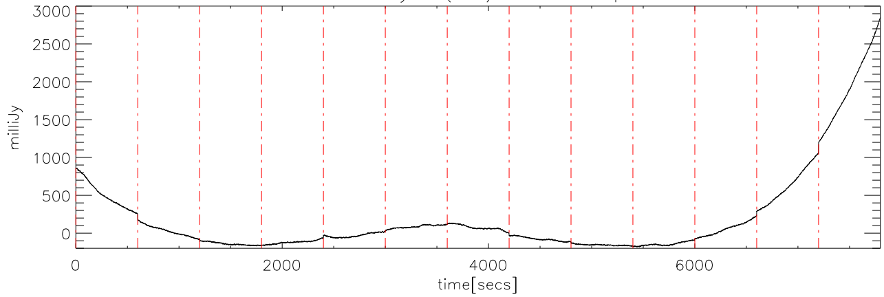
a2327 17may08 (AST) StokesI freq:5250.
