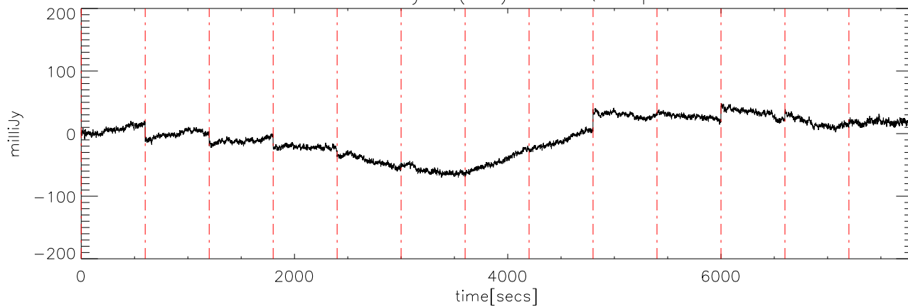
a2327 17may08 (AST) StokesQ freq:5000.
