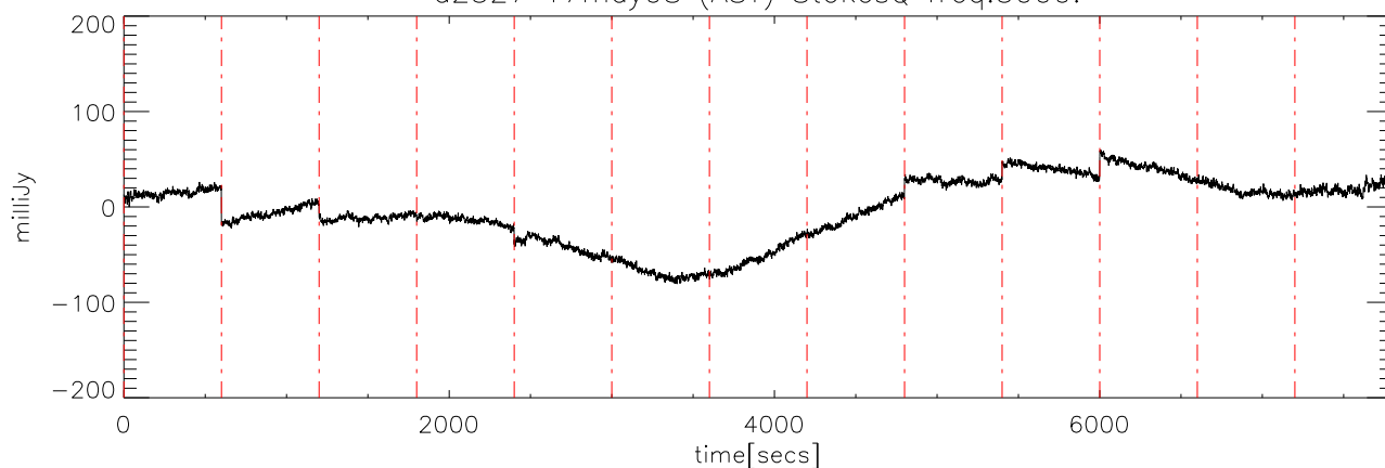
a2327 17may08 (AST) StokesQ freq:5125.
