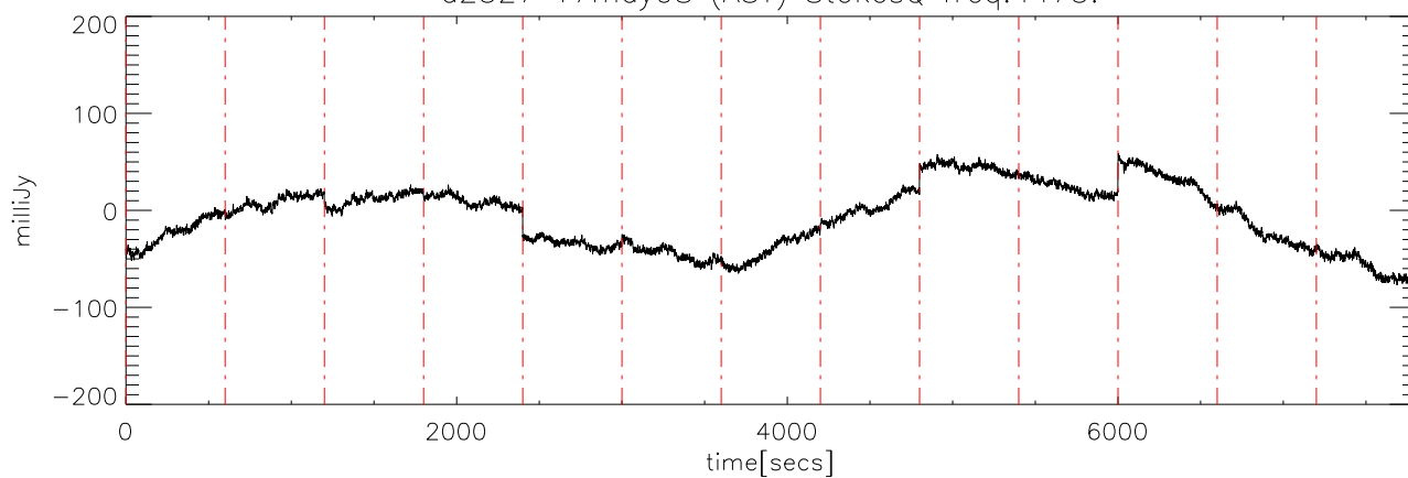
a2327 17may08 (AST) StokesQ freq:4600.
