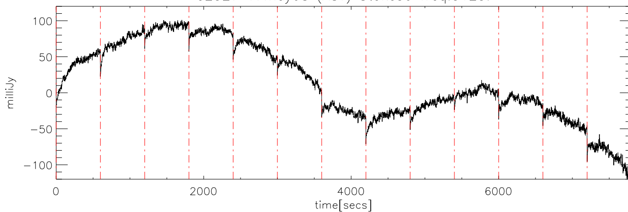
a2327 17may08 (AST) StokesU freq:5250.
