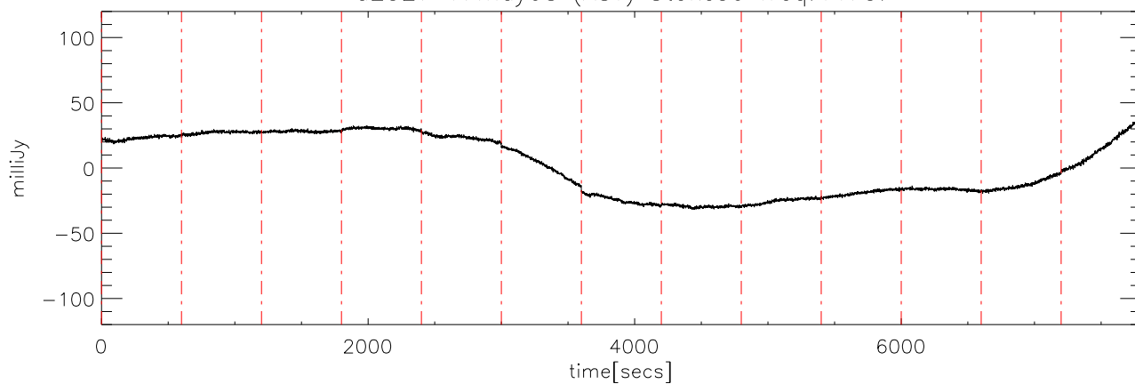
a2327 17may08 (AST) StokesU freq:4600.
