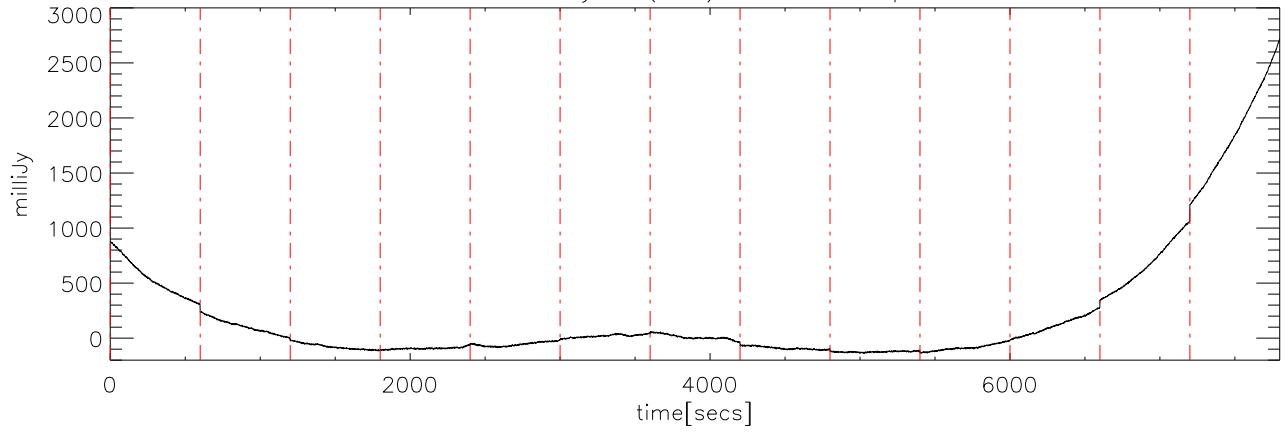
a2327 17may08 (AST) StokesI freq:5000.
