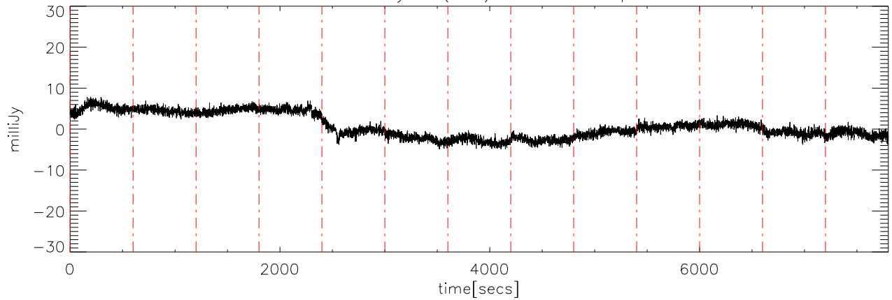
a2327 17may08 (AST) StokesV freq:4600.
