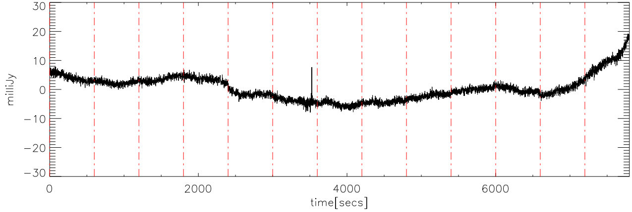
a2327 17may08 (AST) StokesV freq:4475.
