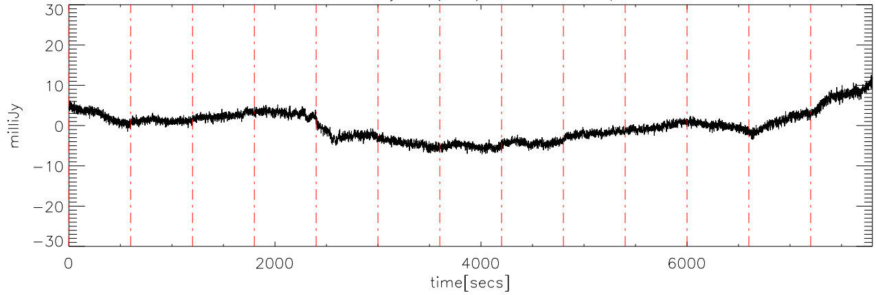
a2327 17may08 (AST) StokesV freq:4725.
