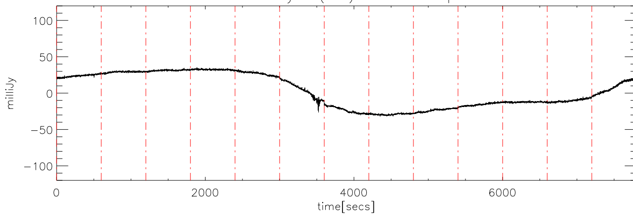
a2327 17may08 (AST) StokesU freq:4475.
