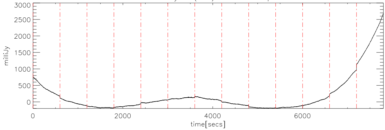
a2327 17may08 (AST) StokesI freq:4475.
