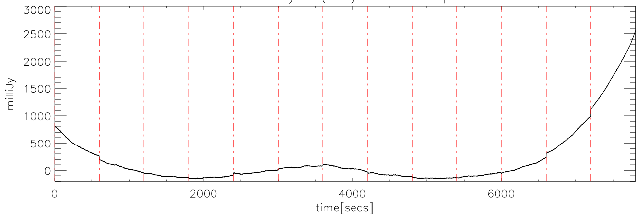
a2327 17may08 (AST) StokesI freq:4600.
