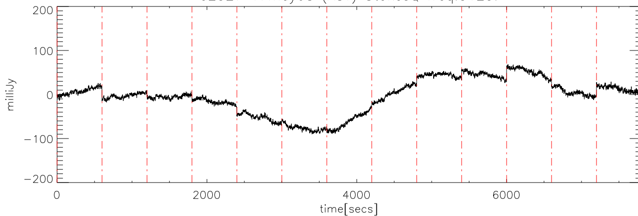
a2327 17may08 (AST) StokesQ freq:5250.
