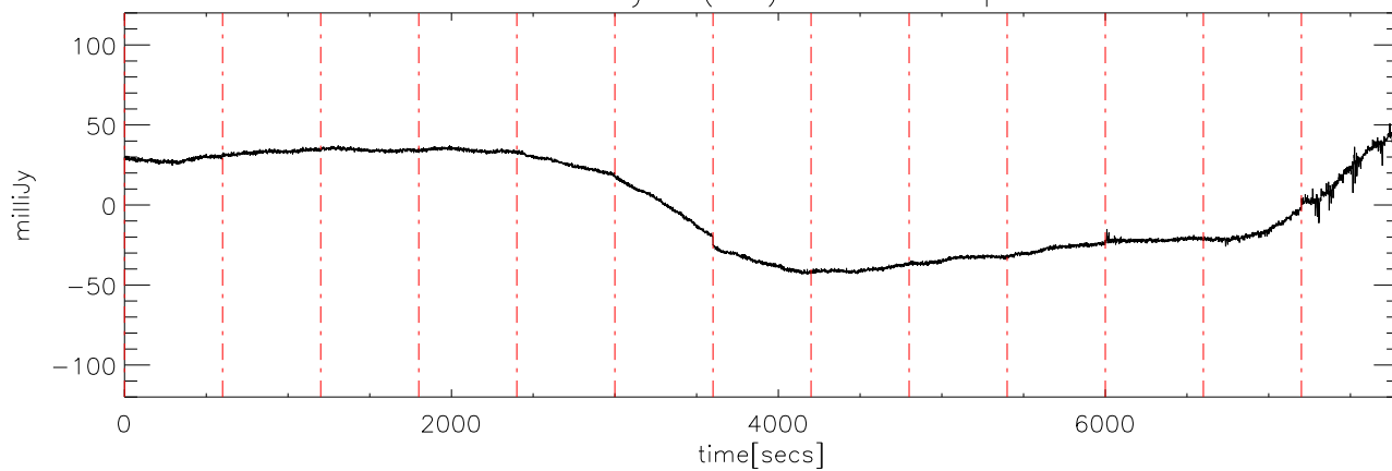
a2327 17may08 (AST) StokesU freq:4725.
