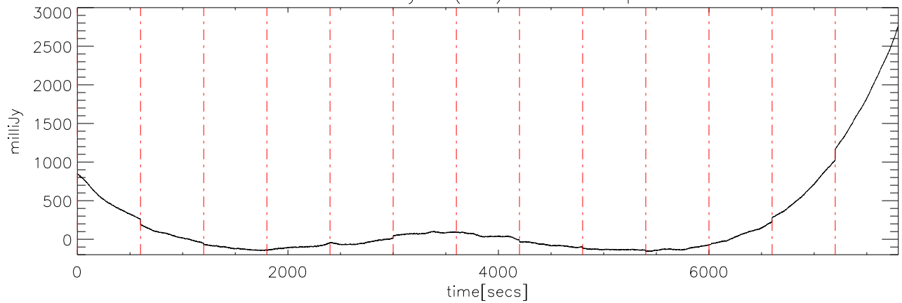
a2327 17may08 (AST) StokesI freq:5125.
