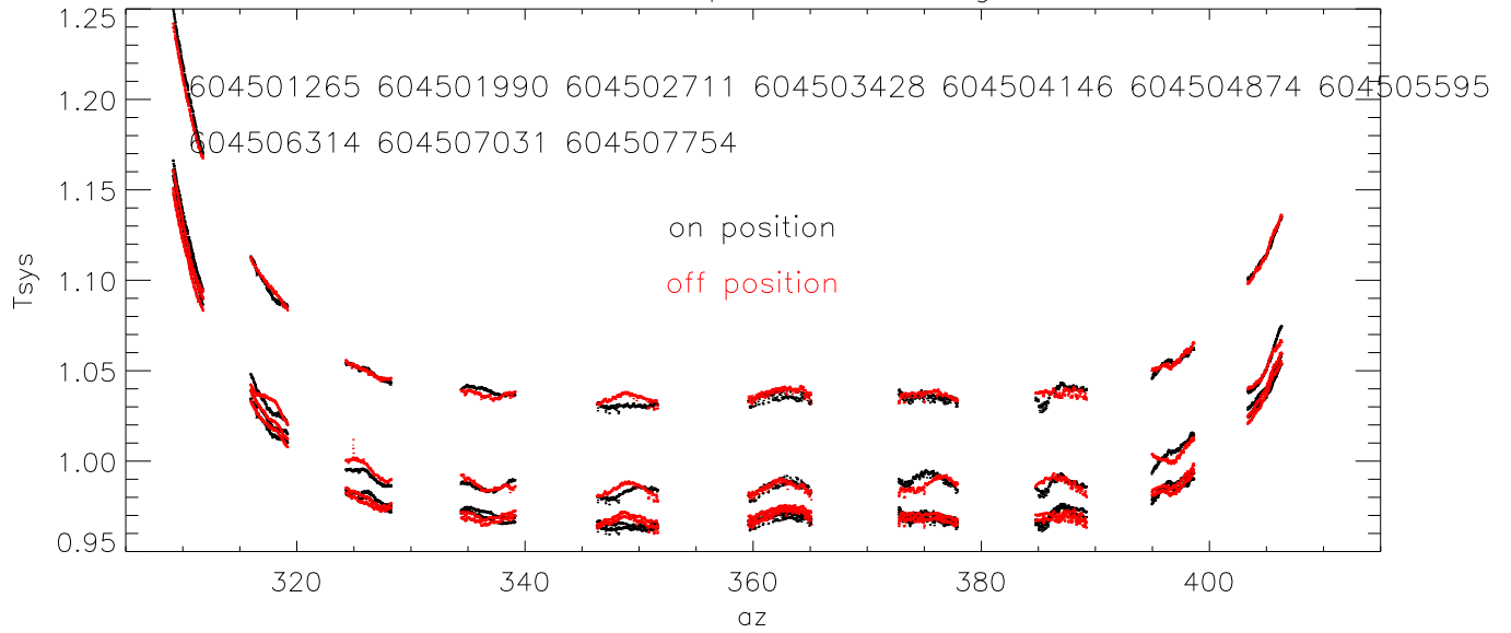
08mar06: Total power vs az avgPols
