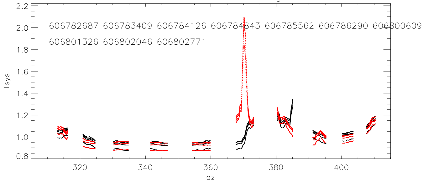
03apr06: Total power vs az avgPols
