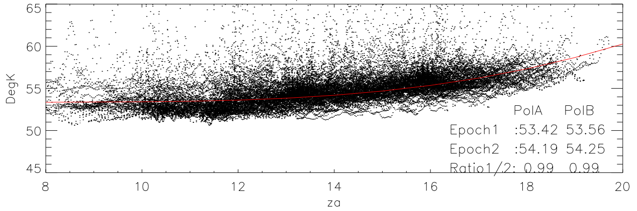
PolB data Epoch 1 data and fit.
