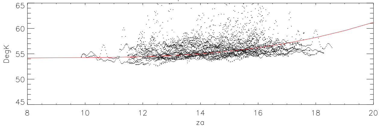
PolB data Epoch 2 data and fit.
