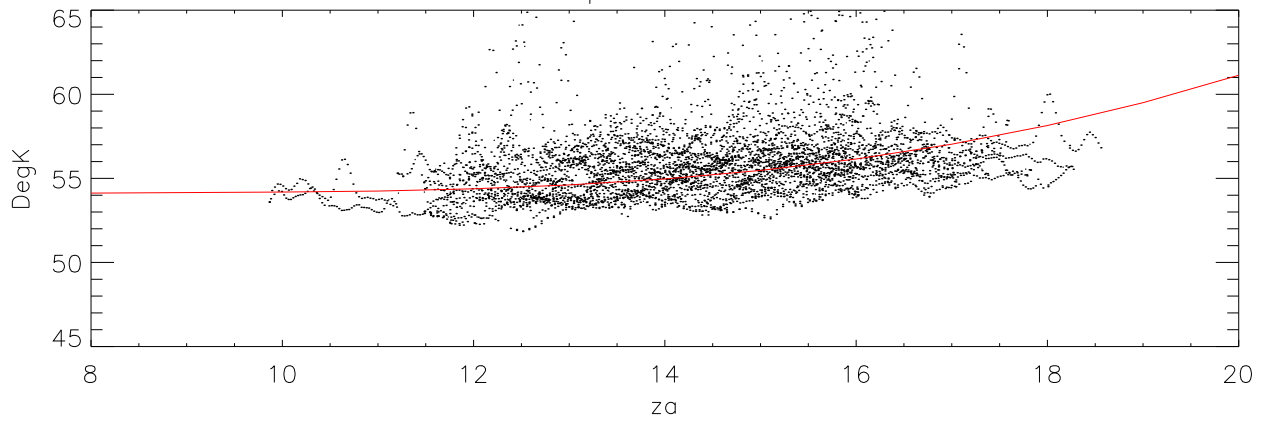
PolB data Epoch 2 data and fit.
