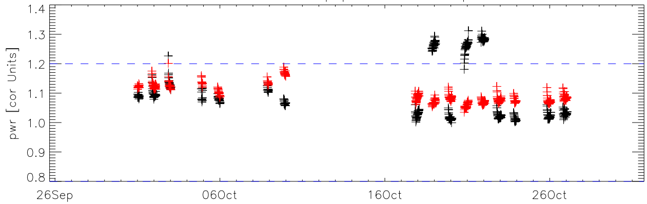
a2010 median strip power vs date. pixel:6
