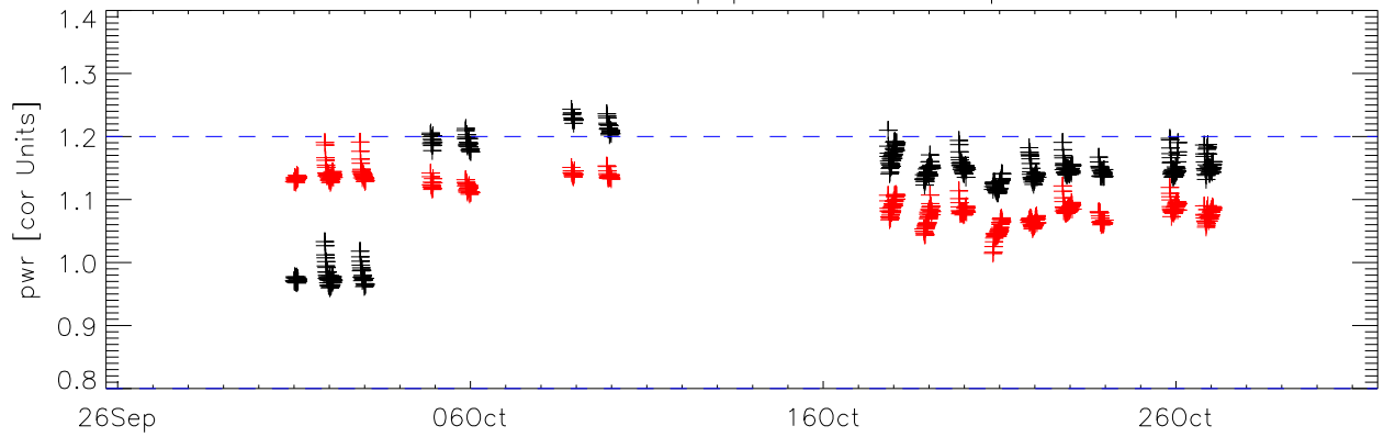
a2010 median strip power vs date. pixel:2
