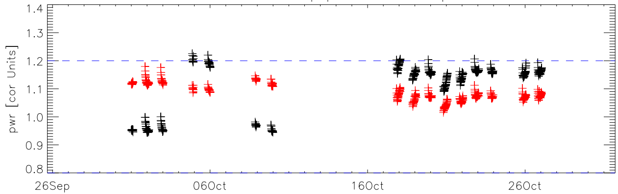
a2010 median strip power vs date. pixel:3
