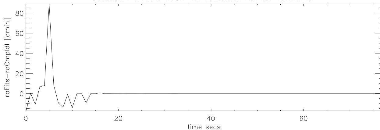
28sep04 a1956 scan 427228229. dec vs time
