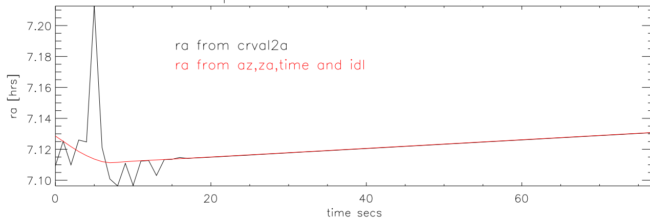
28sep04 a1956 scan 427228229. RaFits-raIdlCmp
