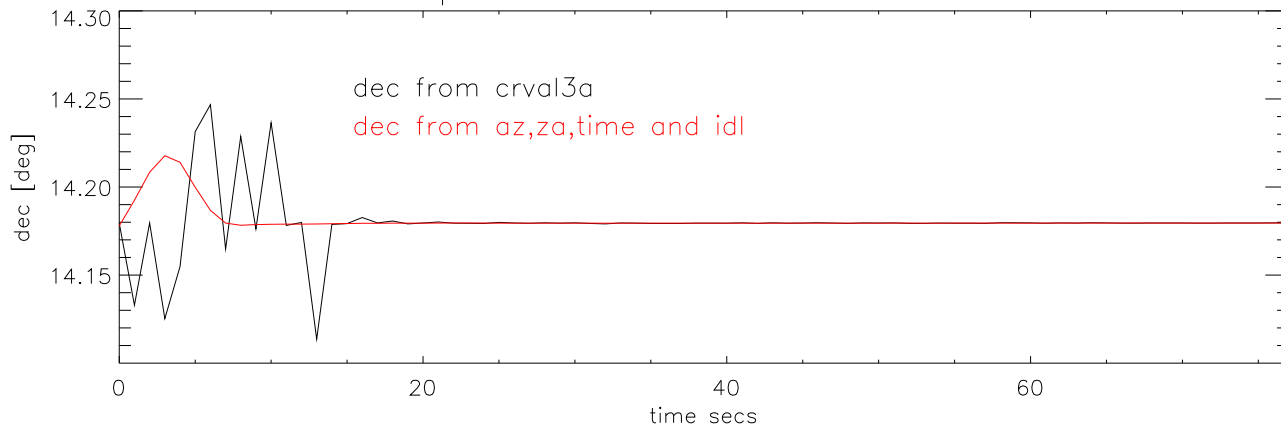
28sep04 a1956 scan 427228229. decFitsHdr-decIdlCmp
