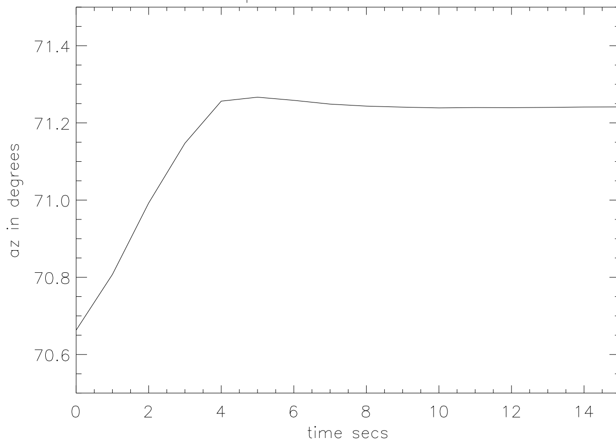
azimuth position for scan 427228229
