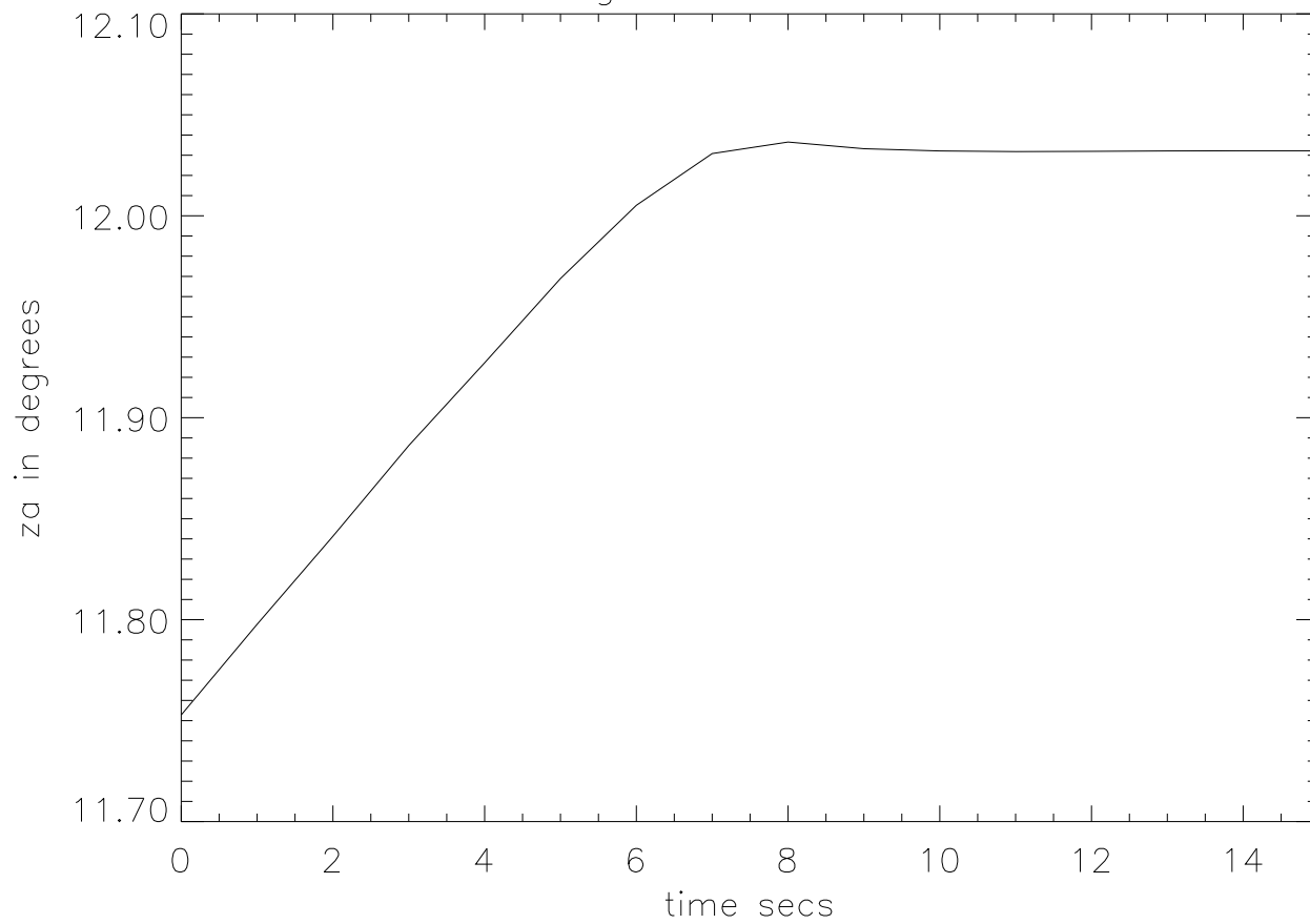
zenith angle for scan 427228229
