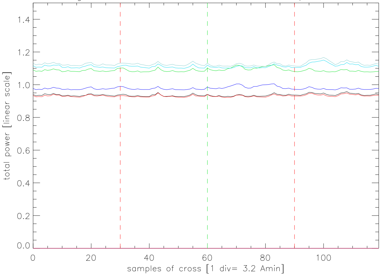
19aug04 A1946 alfa CROSSA0 src:J1311+18 polB beams
