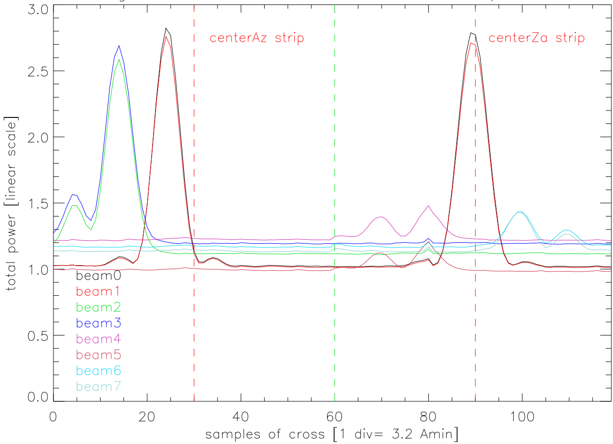
19aug04 A1946 alfa CROSSA0 src:B1345+125 polB beams
