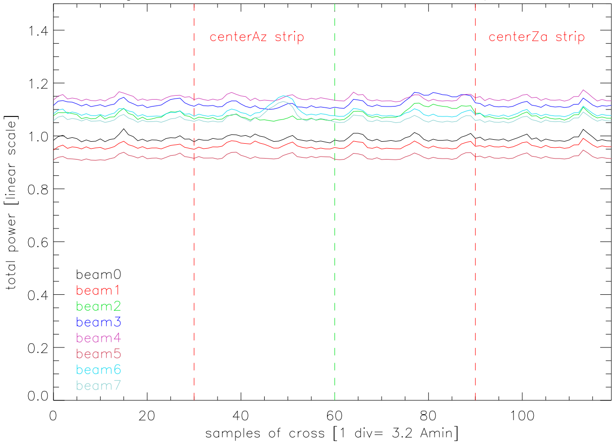
19aug04 A1946 alfa CROSSA2 src:J1311+18 polB beams
