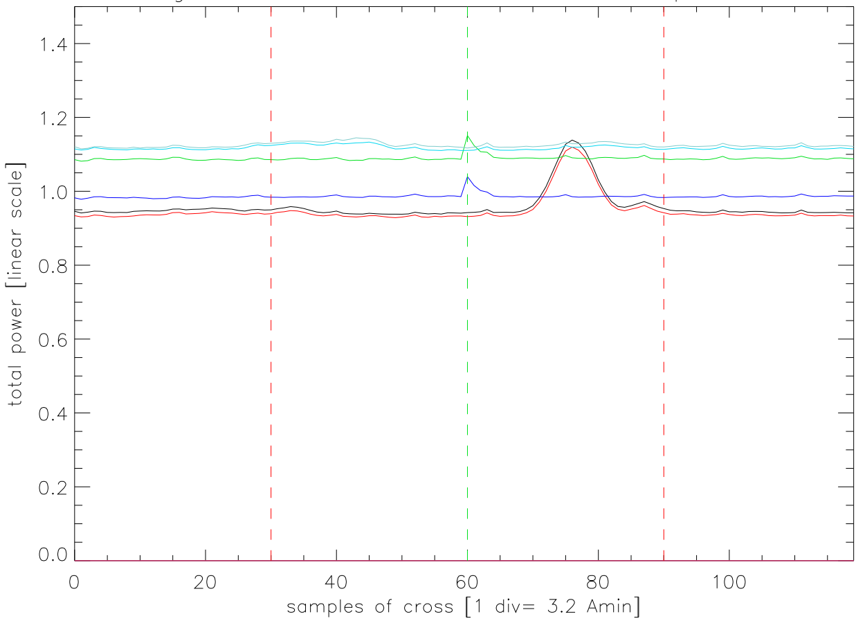
19aug04 A1946 alfa CROSSA1 src:J1311+18 polB beams
