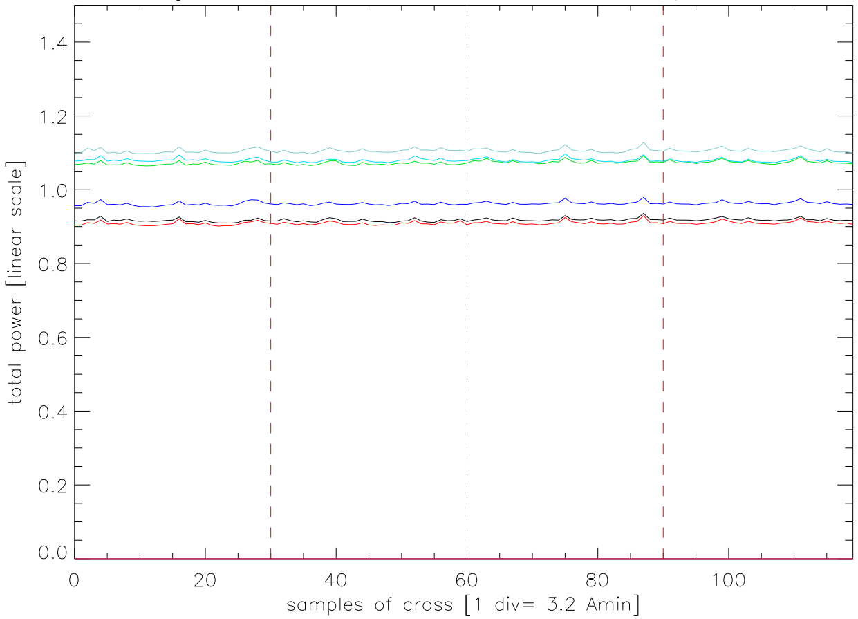
19aug04 A1946 alfa CROSSA5 src:J1257+18 polB beams
