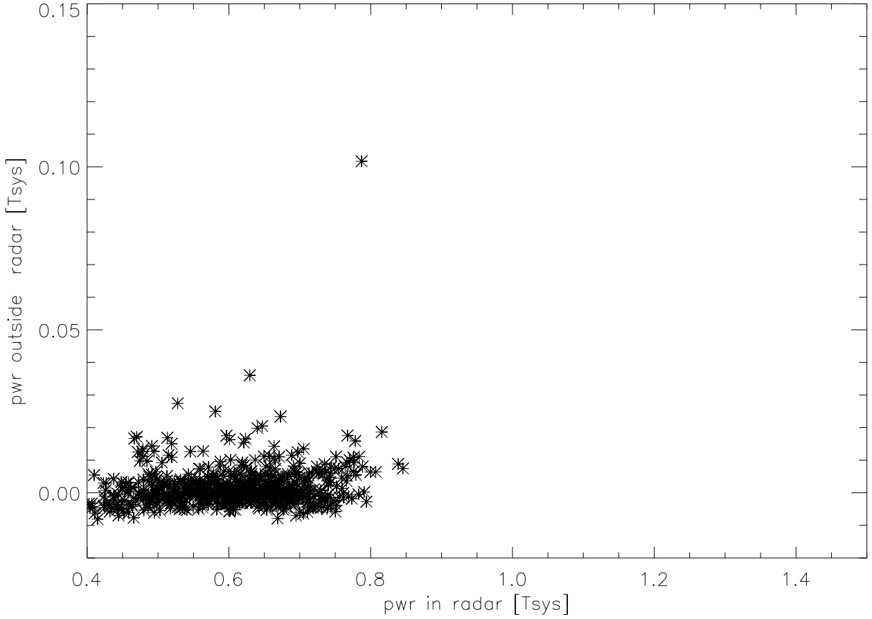
Strength outside radar band vs strength radar Pixel 4 polB
