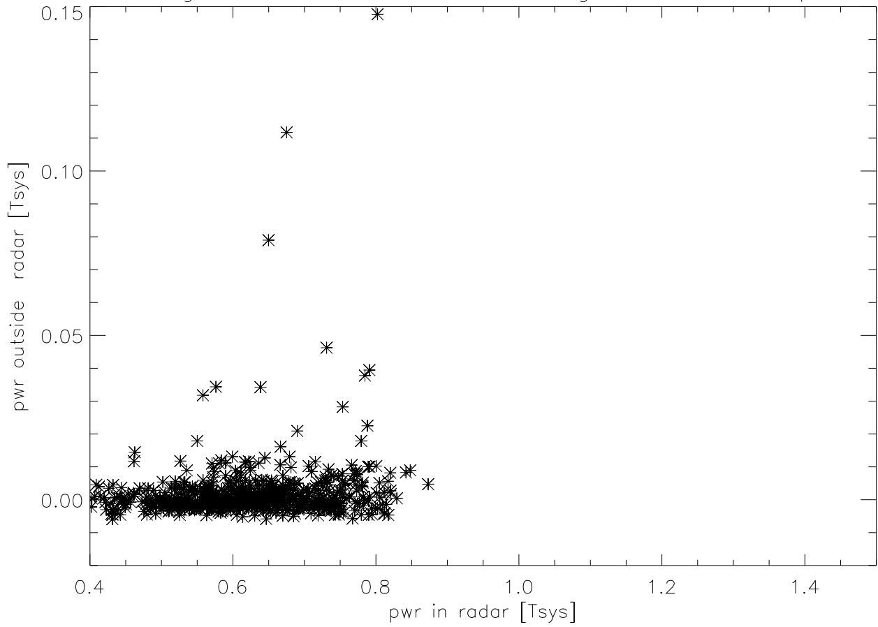
Strength outside radar band vs strength radar Pixel 5 polB
