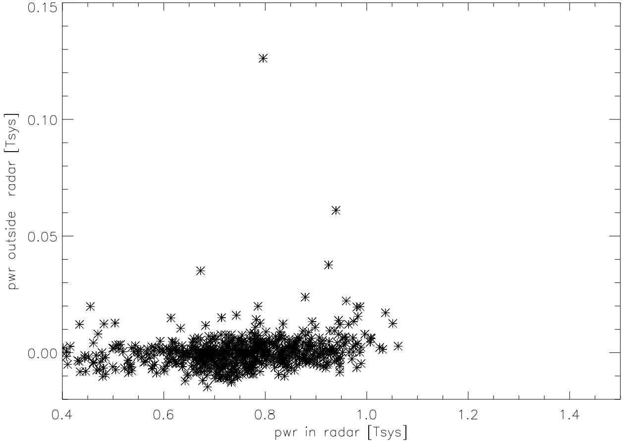
Strength outside radar band vs strength radar Pixel 0 polB
