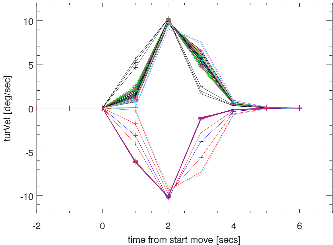
Turret velocity during sband tx<-->rx moves
