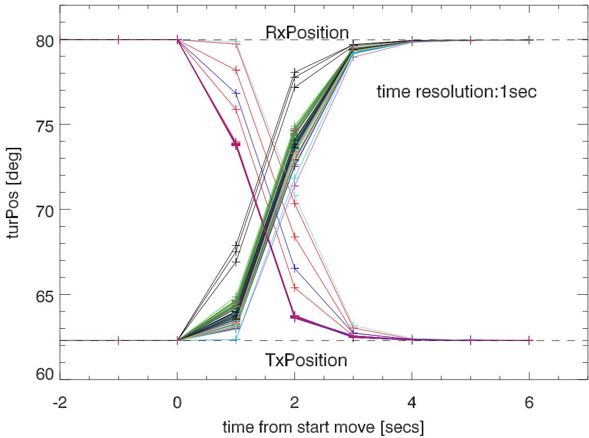
7may20:Turret positions during sband tx<-->rx moves
