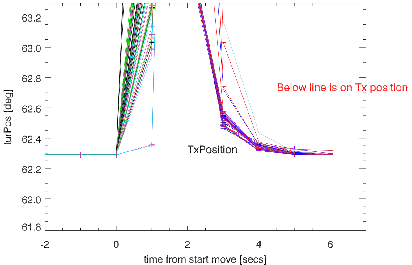
moving rx to tx. On position when within .5 deg
