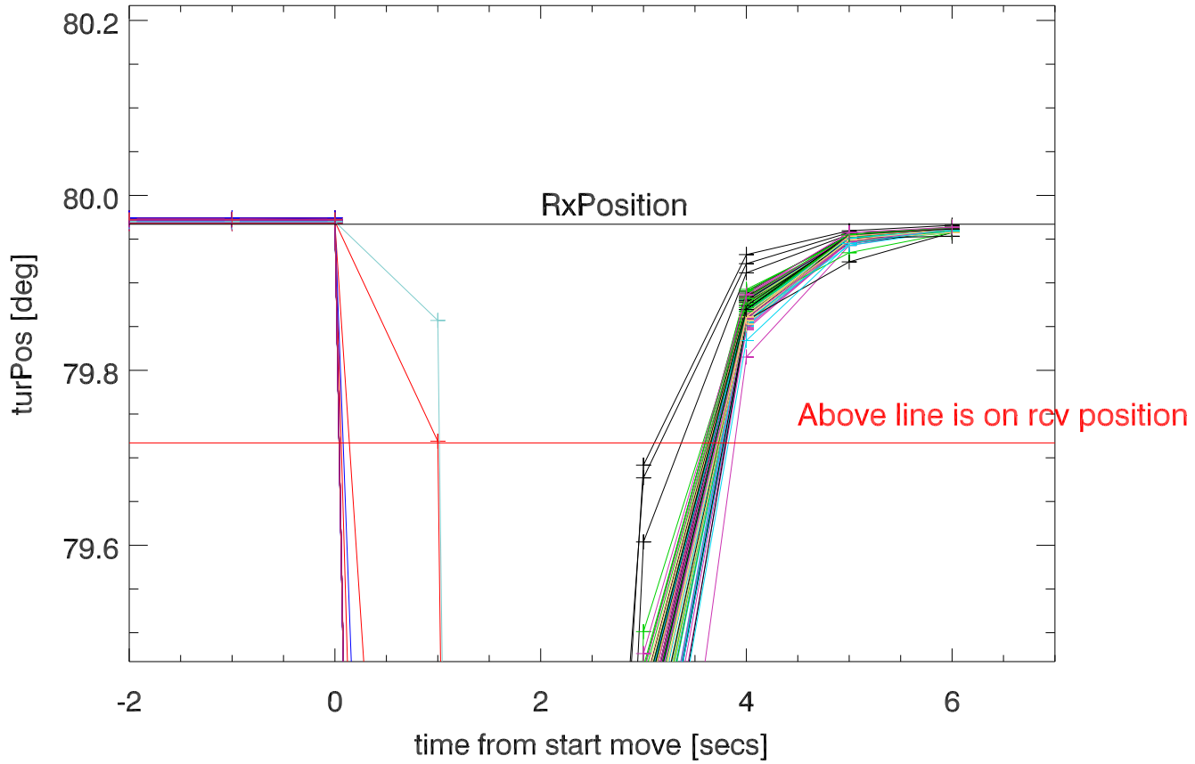
moving tx to rx. On position when within .25 deg
