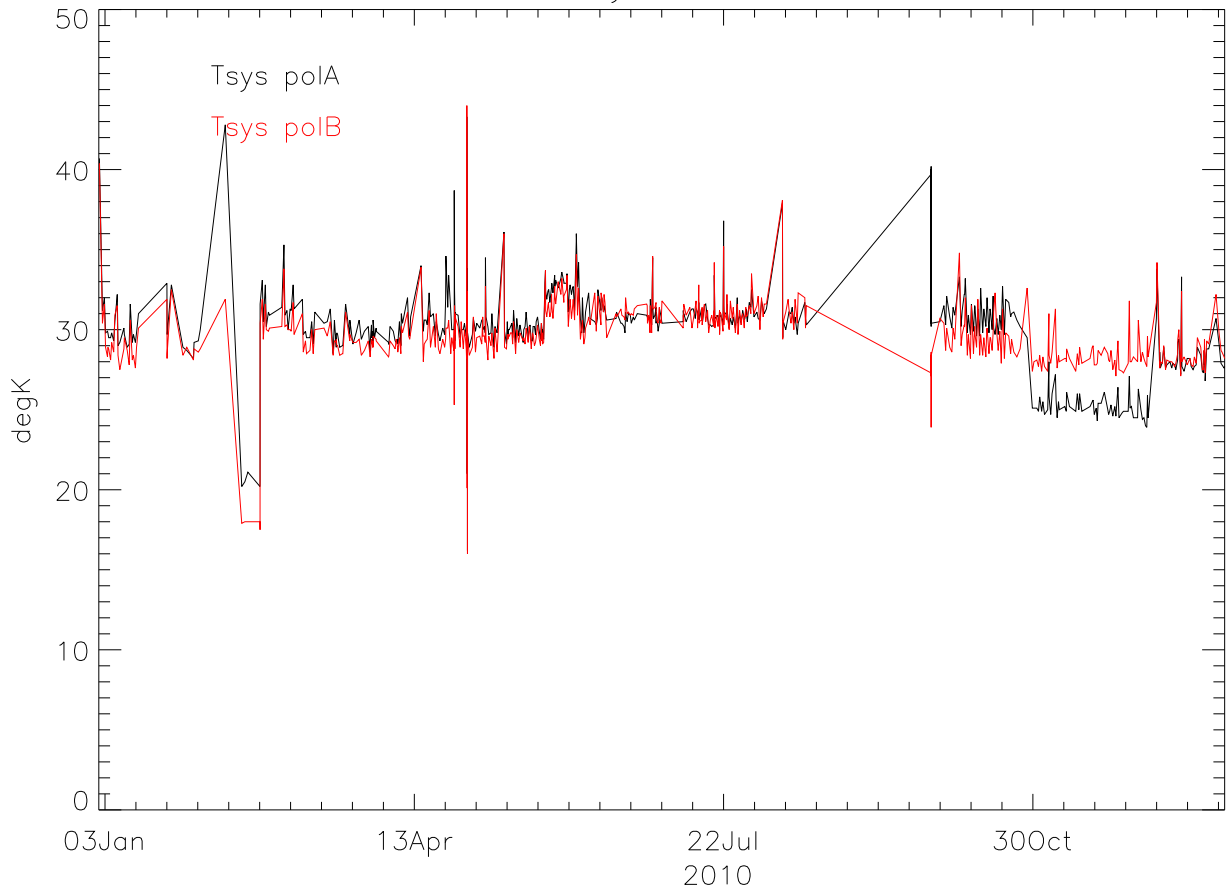
lbw TsysA-TsysB 2010
