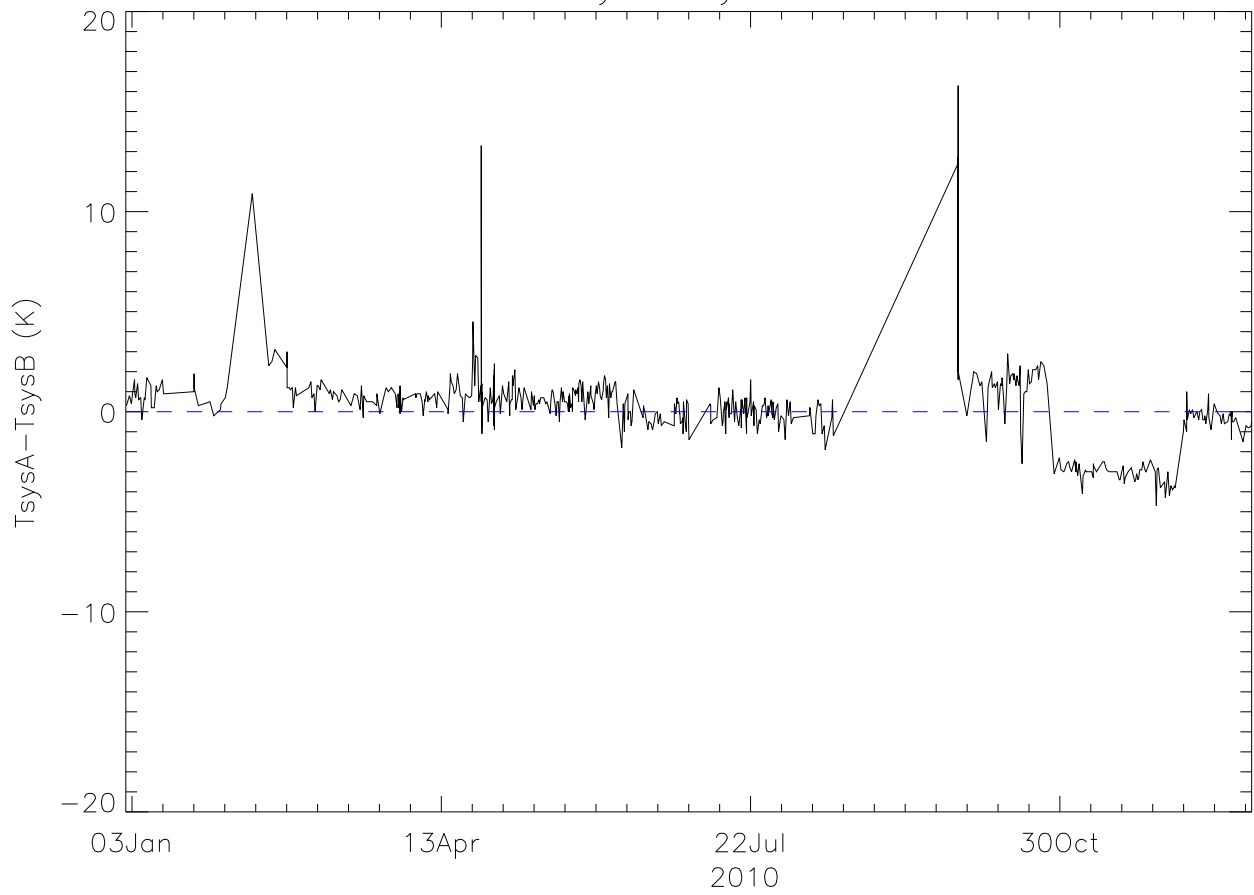
lbw TsysA-TsysB 2010
