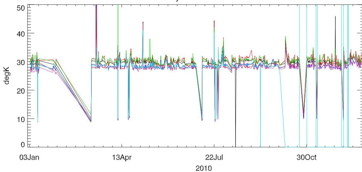
alfa Tsys for 2010 PoIB
