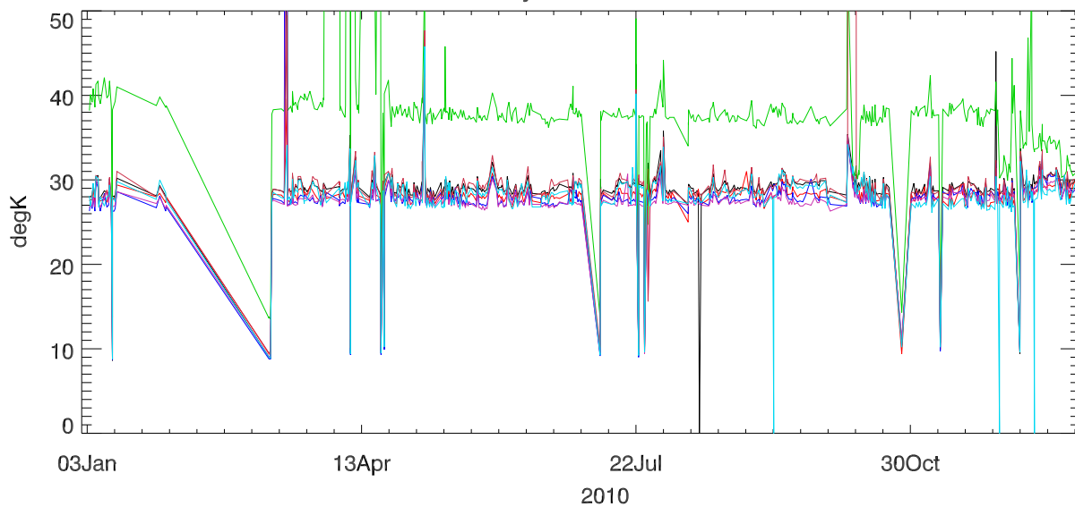
alfa Tsys for 2010 PoIA
