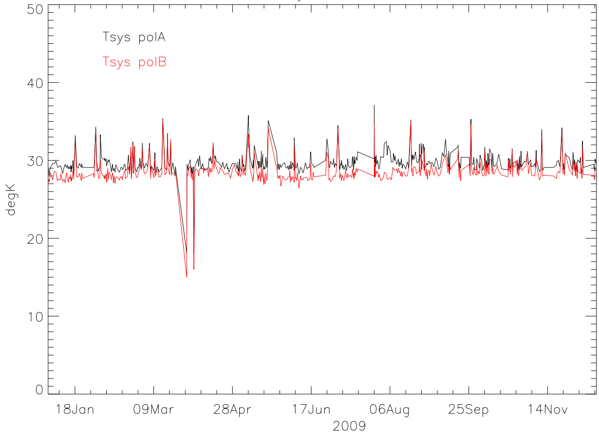
lbw TsysA-TsysB 2009
