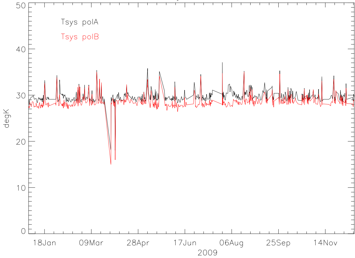
lbw TsysA-TsysB 2009
