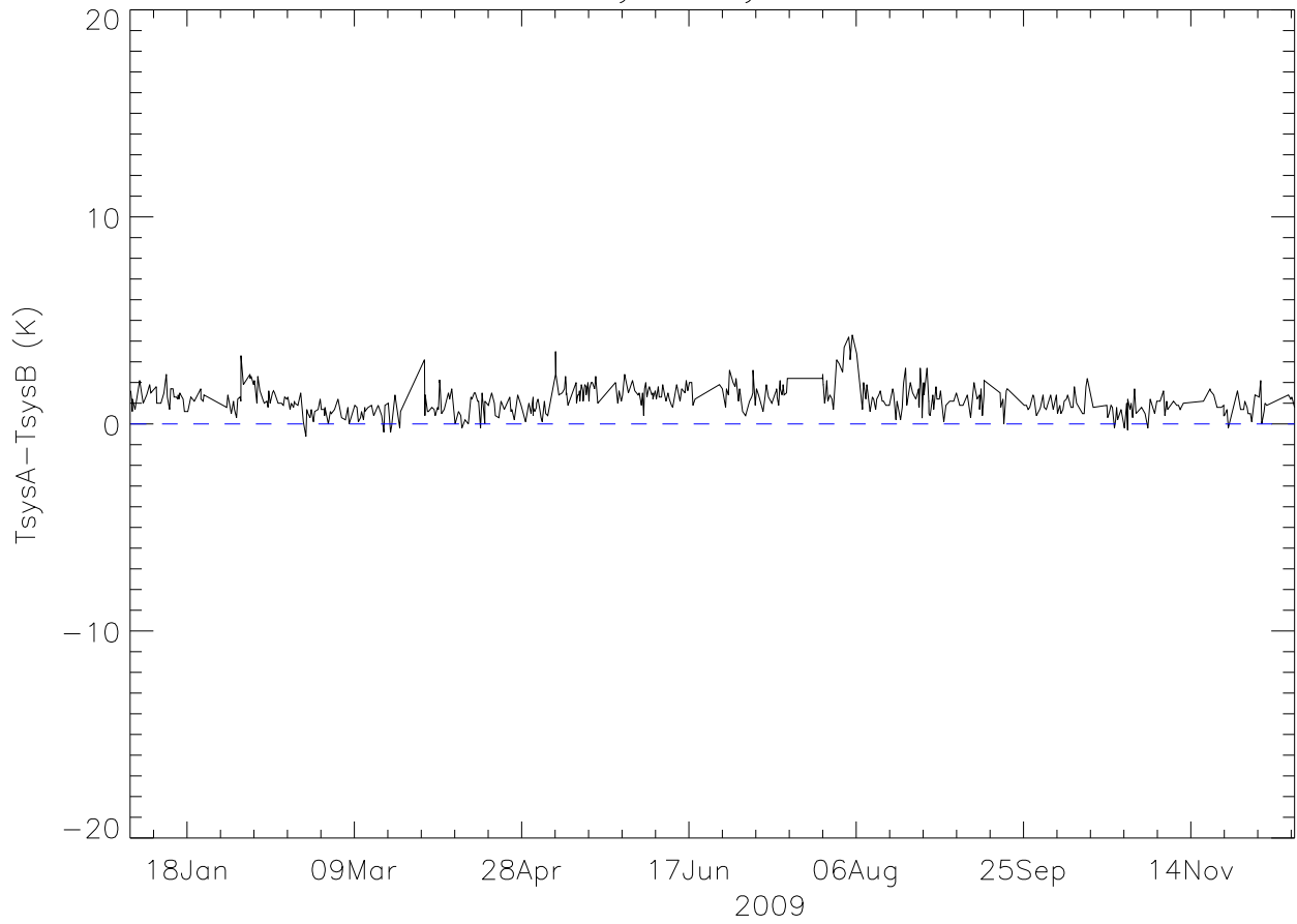
lbw TsysA-TsysB 2009
