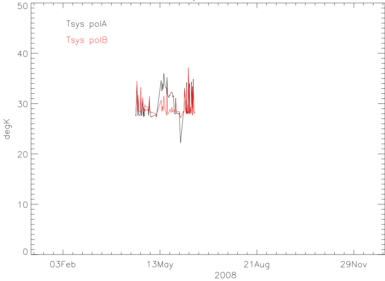
sbh TsysA-TsysB 2008
