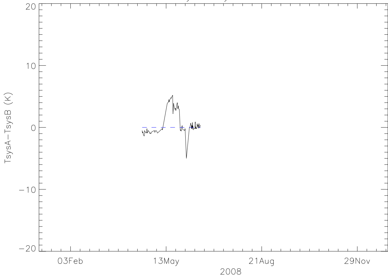
sbh TsysA-TsysB 2008
