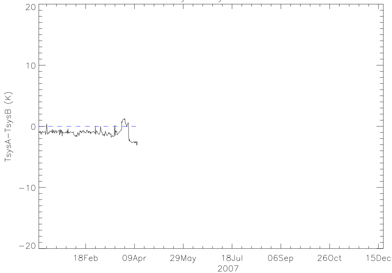
xb TsysA - TsysB 2007
