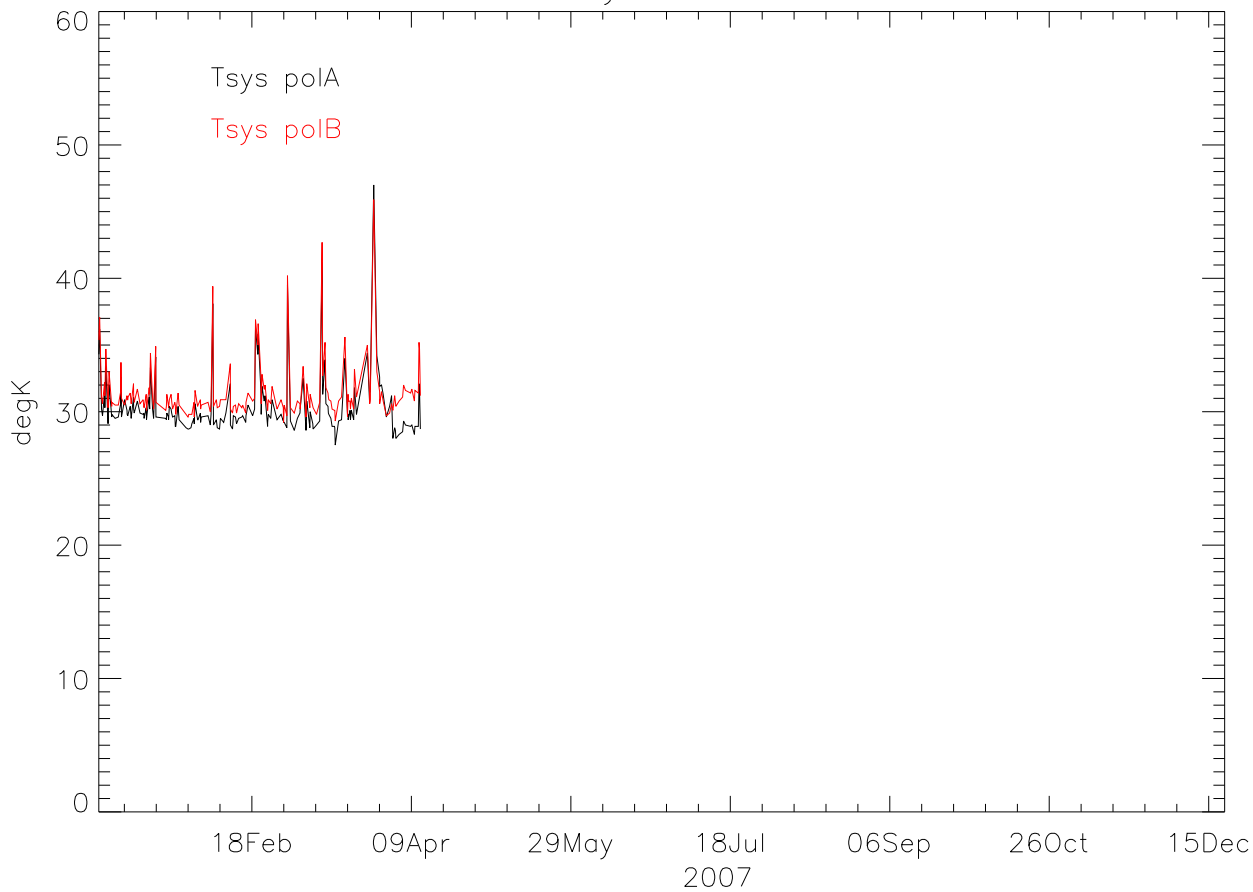
xb TsysA - TsysB 2007
