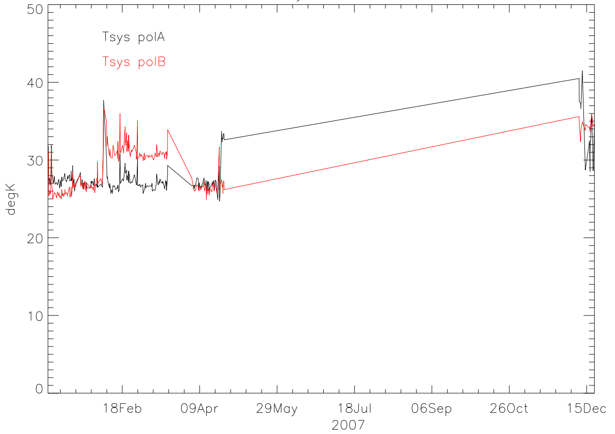
lbw TsysA-TsysB 2007
