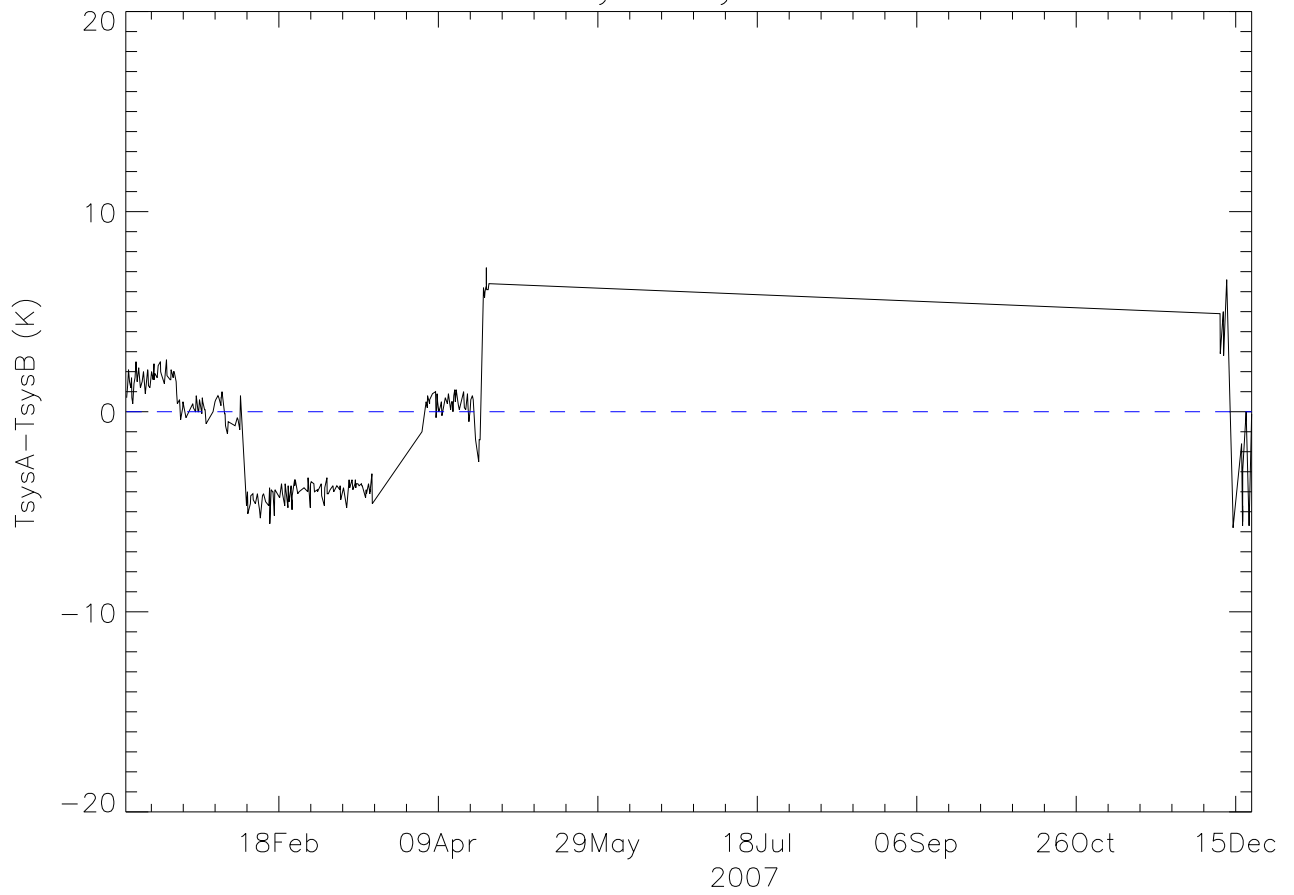
lbw TsysA-TsysB 2007
