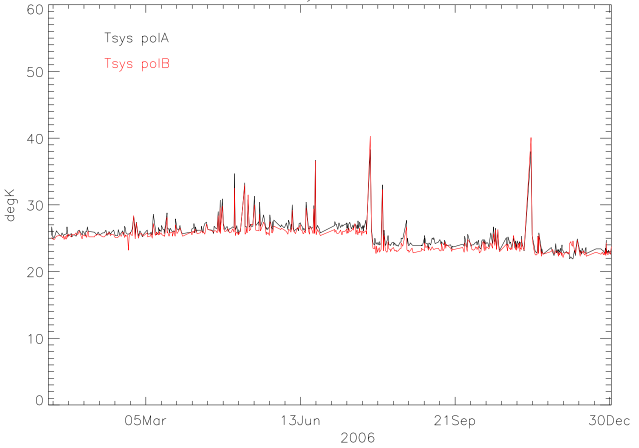
sbw TsysA-TsysB 2006
