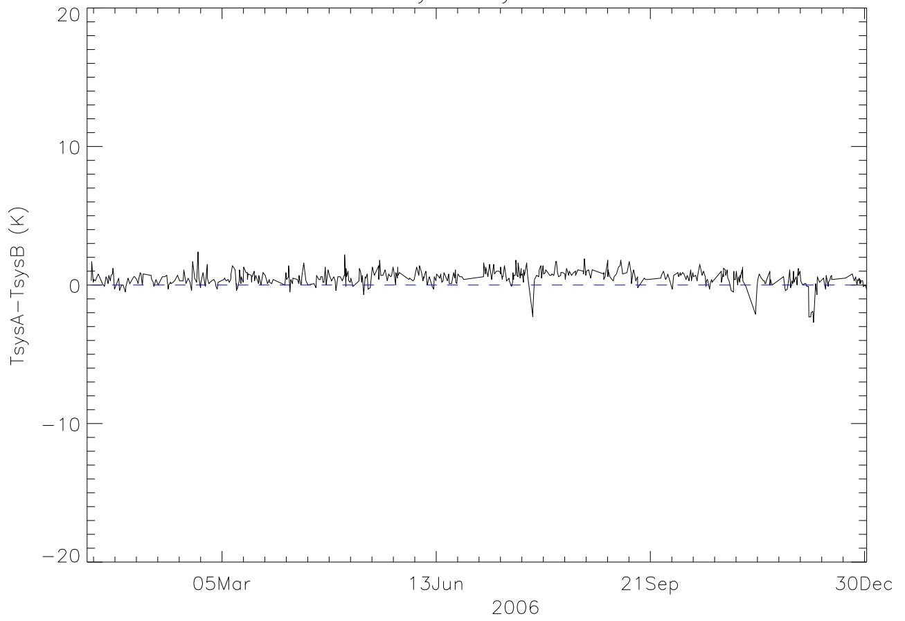
sbw TsysA-TsysB 2006
