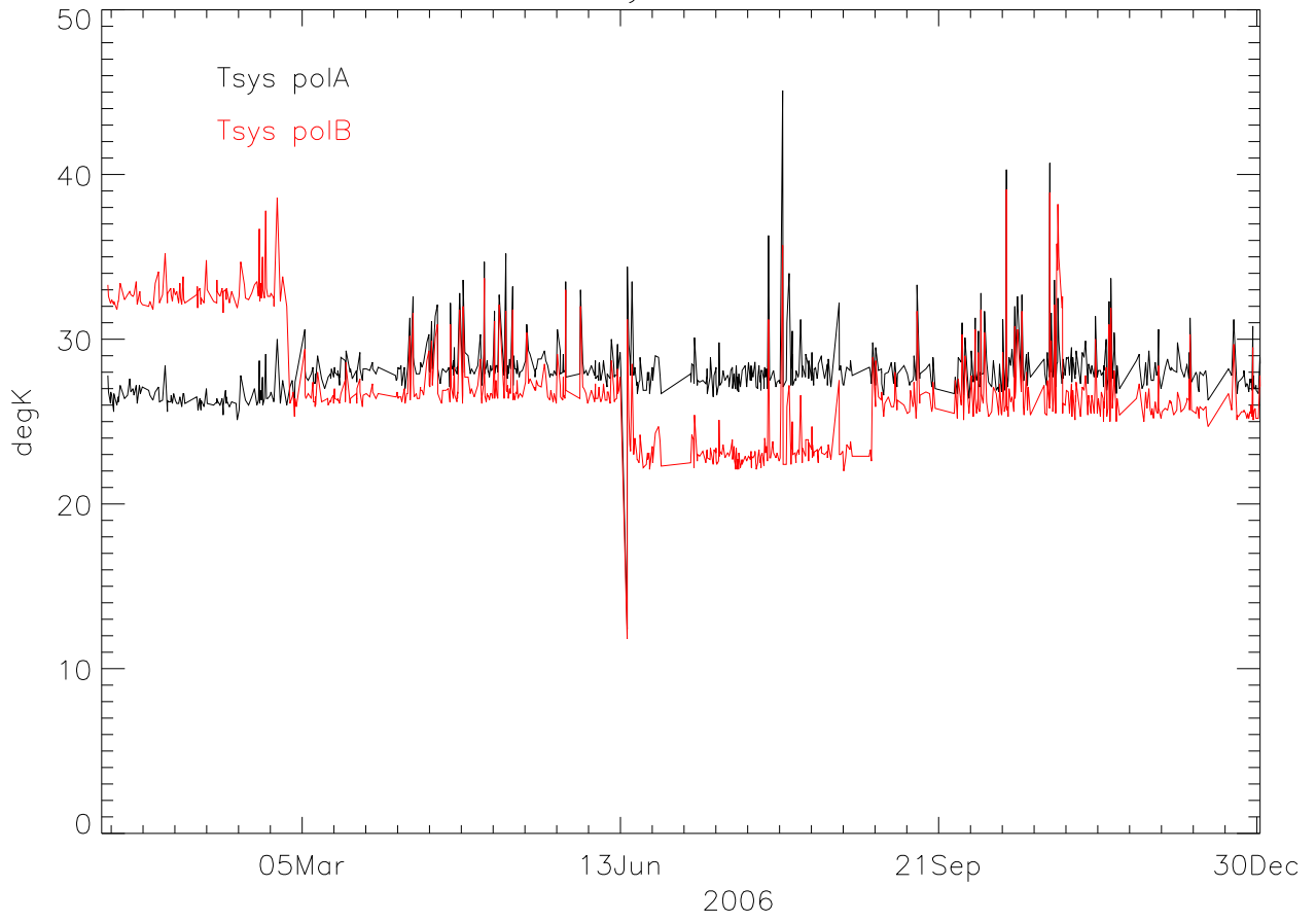
lbw TsysA-TsysB 2006
