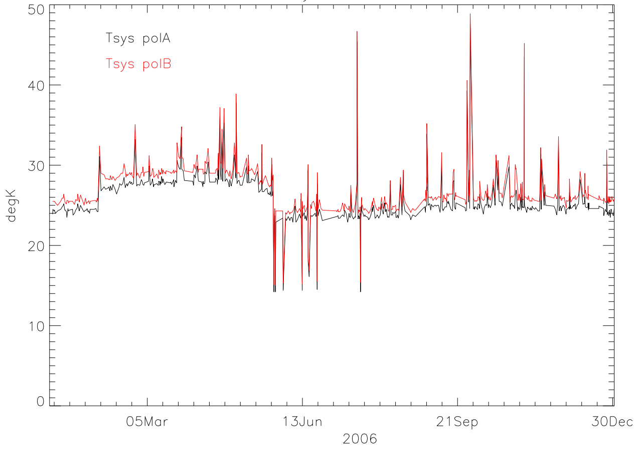
cb TsysA-TsysB 2006
