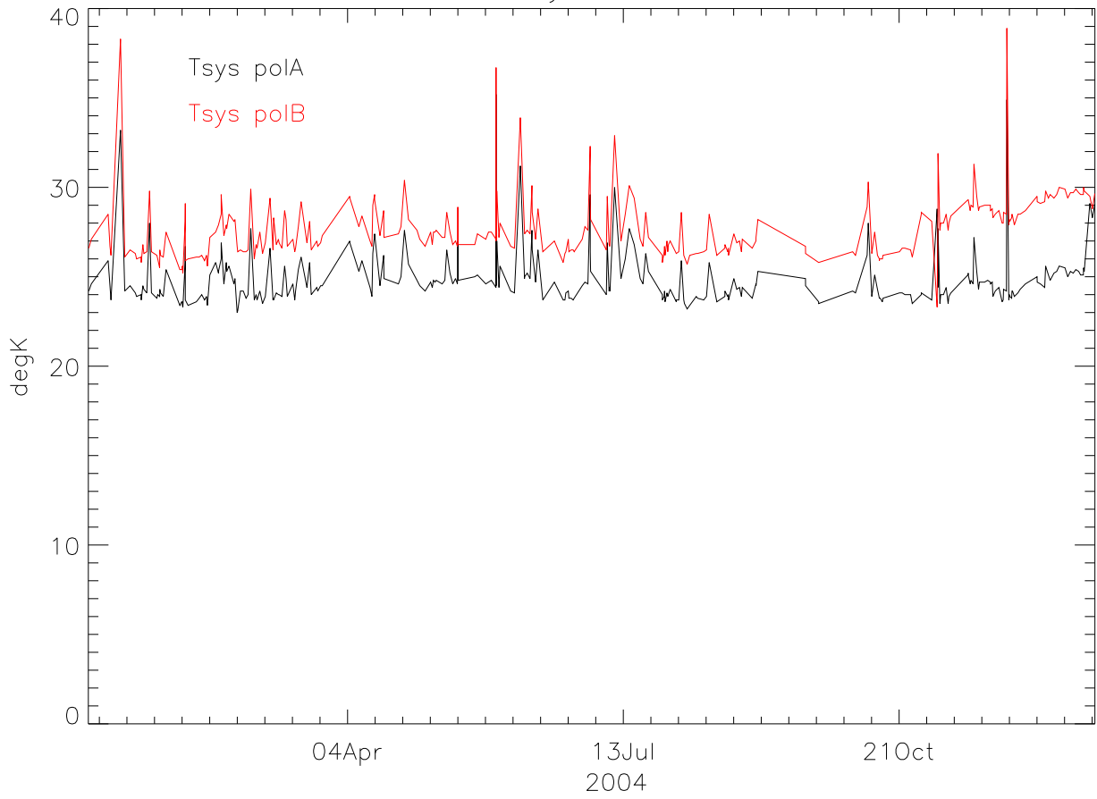
sbn TsysA-TsysB 2004
