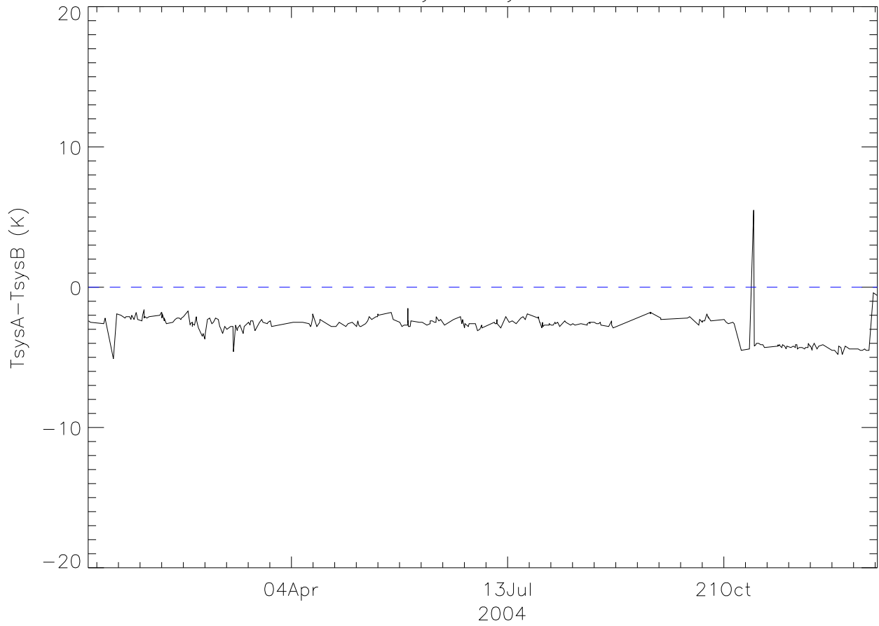
sbn TsysA-TsysB 2004
