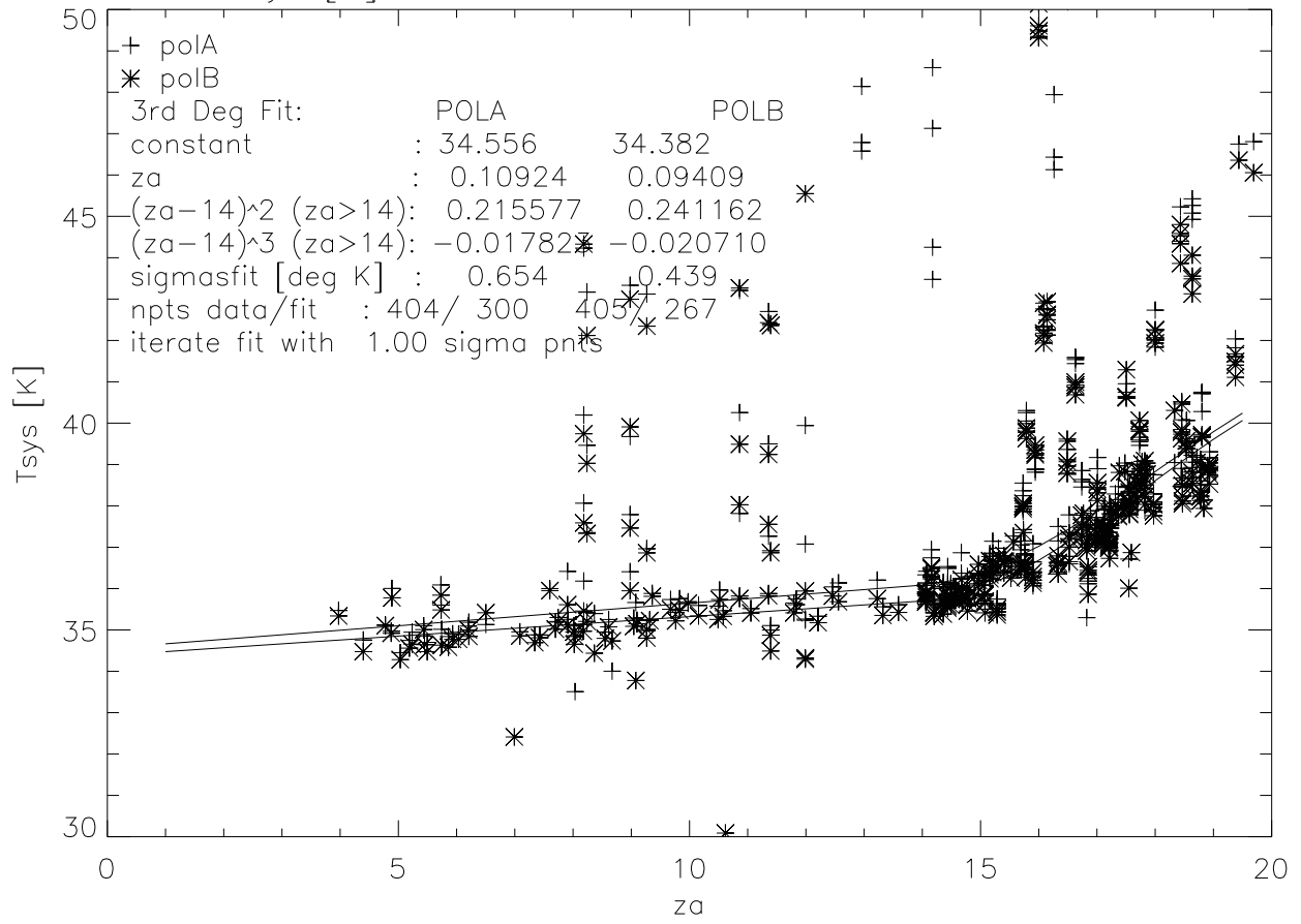
Tsys [K] vs Za LBW 1650–1670 MHZ, APR–JUL00
