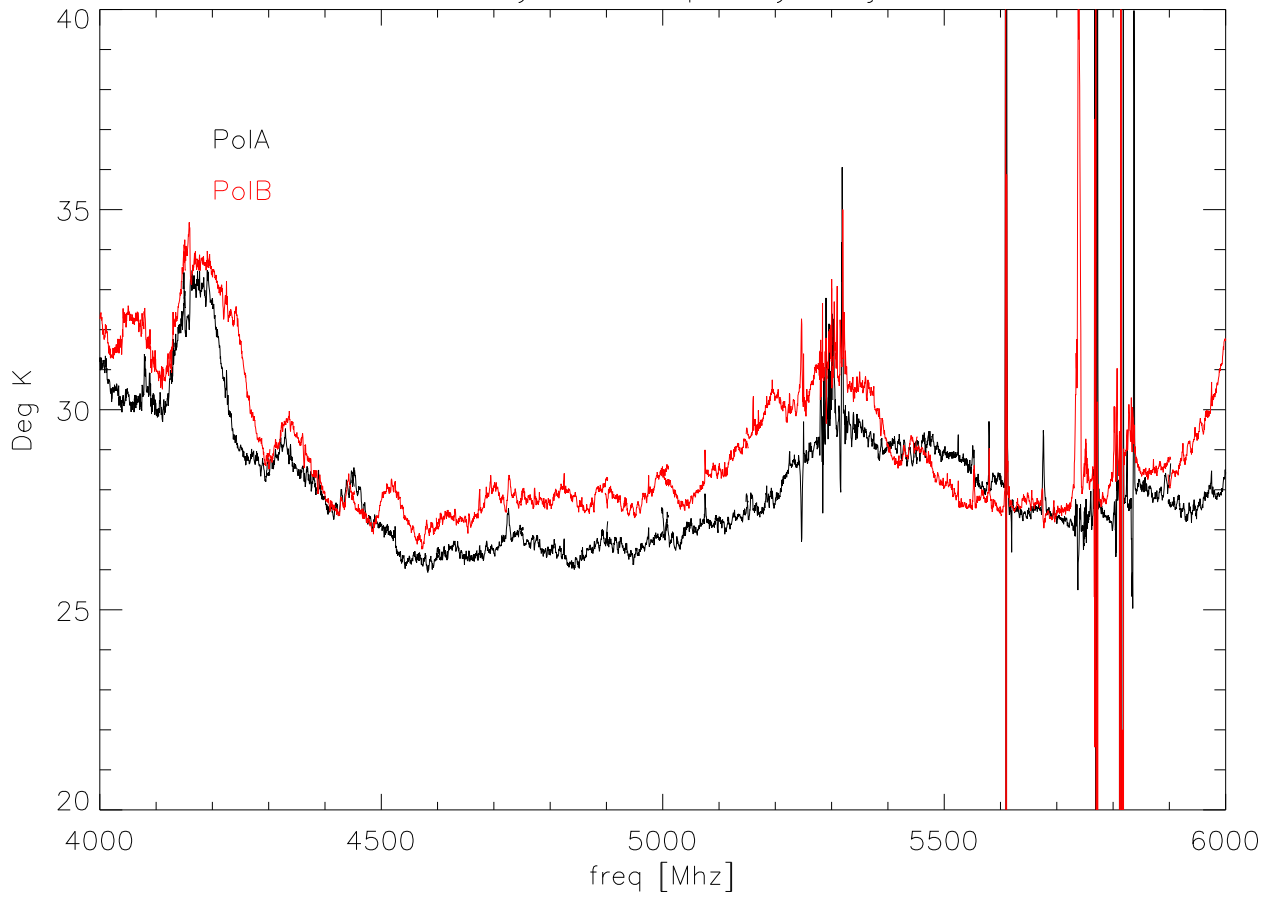
cband high correlated cal vs frequency
