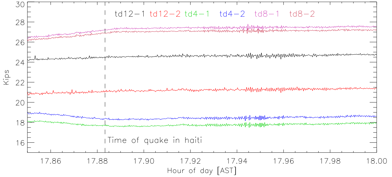
Remove mean tension each cable
